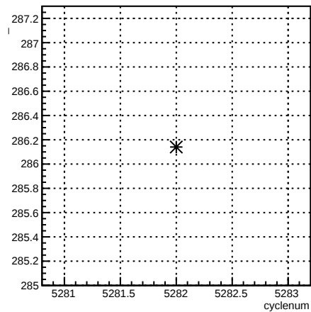
4eX_coil7:cyclenum {run == 5962}
