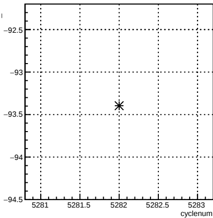
usl_4eY:cyclenum {run == 5962}
