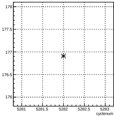
4eY_coil4:cyclenum {run == 5962}
