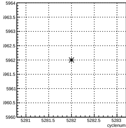
run:cyclenum {run == 5962}
