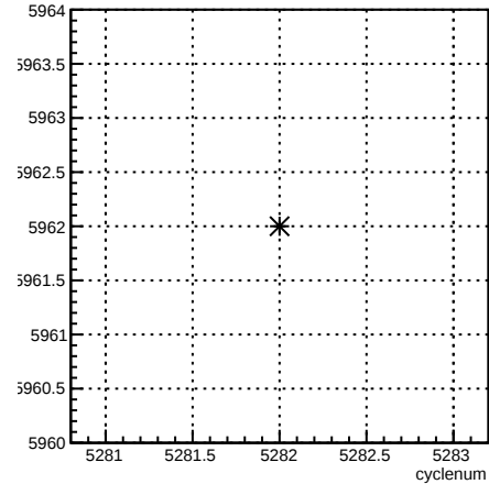
run:cyclenum {run == 5962}
