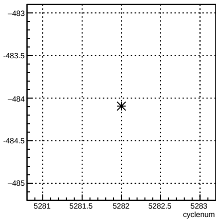
12X_coil7:cyclenum {run == 5962}
