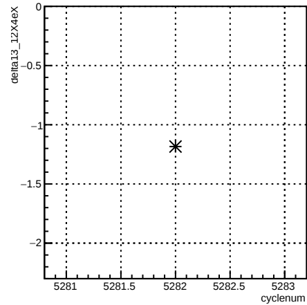
delta13_12X4eX:cyclenum {run == 5962}
