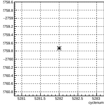
usr_coil7:cyclenum {run == 5962}
