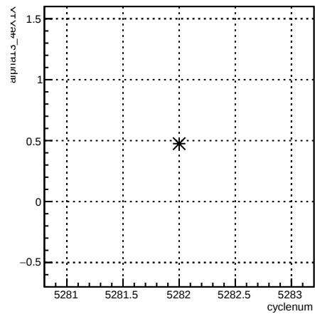
alpha13_4eX1X:cyclenum {run == 5962}
