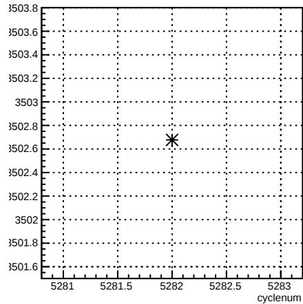
usl_coil3:cyclenum {run == 5962}
