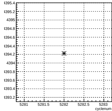
usl_coil4:cyclenum {run == 5962}
