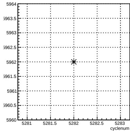
run:cyclenum {run == 5962}
