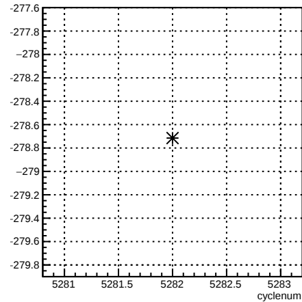
1X_coil1:cyclenum {run == 5962}
