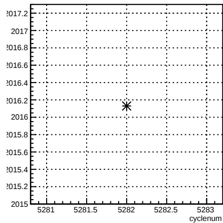
usl_coil7:cyclenum {run == 5962}
