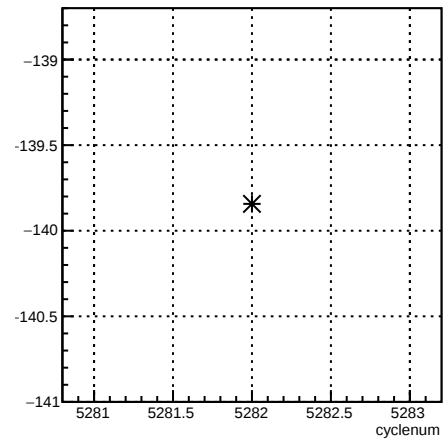
usr_4eY:cyclenum {run == 5962}
