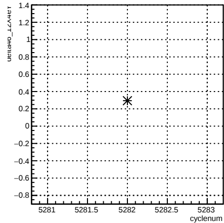
delta46_12X4eY:cyclenum {run == 5962}
