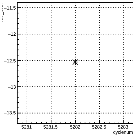
4eY_coil7:cyclenum {run == 5962}
