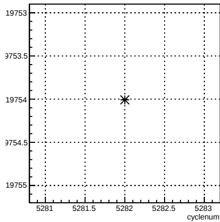
usr_coil6:cyclenum {run == 5962}
