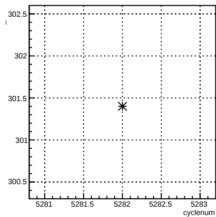
1X_coil7:cyclenum {run == 5962}
