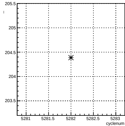
usr_4eX:cyclenum {run == 5962}
