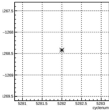
usl_coil6:cyclenum {run == 5962}
