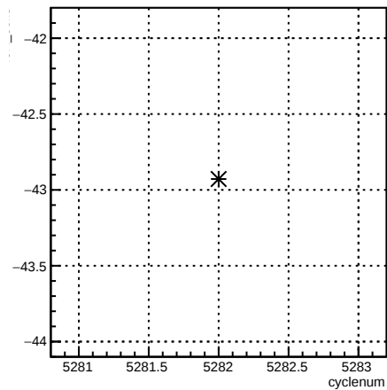
4eX_coil3:cyclenum {run == 5962}
