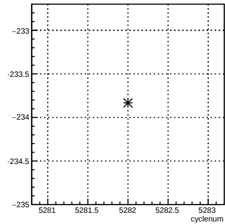
12X_coil6:cyclenum {run == 5962}
