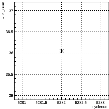
4eY_coil6:cyclenum {run == 5962}
