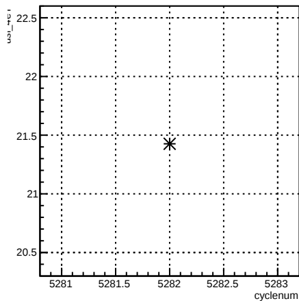
usl_4eY:cyclenum {run == 5962}
