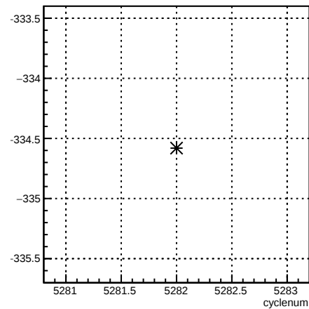
4eX_coil1:cyclenum {run == 5962}
