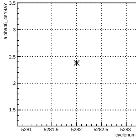
alpha46_4eY4aY:cyclenum {run == 5962}
