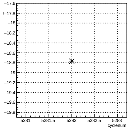
1X_coil3:cyclenum {run == 5962}
