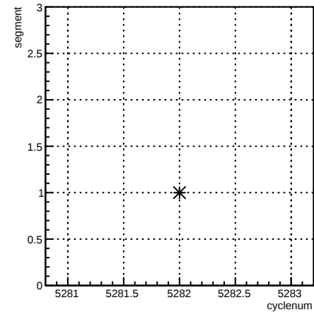
segment:cyclenum {run == 5962}
