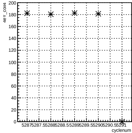
4eY_coil4:cyclenum {run == 5963}
