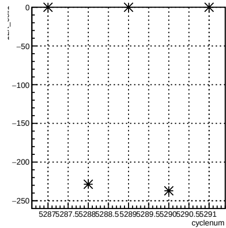
12X_coil1:cyclenum {run == 5963}
