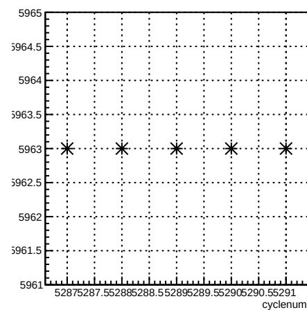
run:cyclenum {run == 5963}
