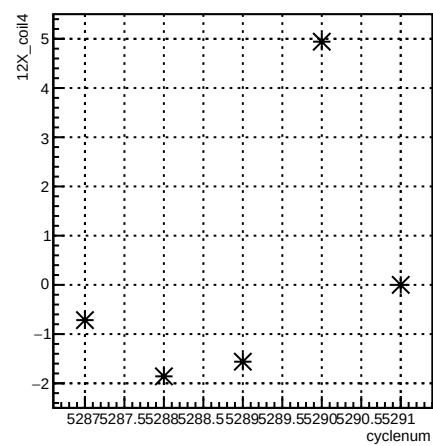
12X_coil4:cyclenum {run == 5963}
