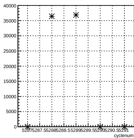
usr_coil7:cyclenum {run == 5963}
