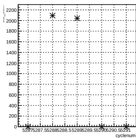
usl_coil7:cyclenum {run == 5963}
