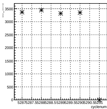
usl_coil3:cyclenum {run == 5963}
