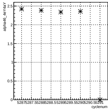
alpha46_4eY4aY:cyclenum {run == 5963}
