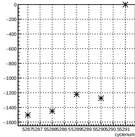
usl_coil6:cyclenum {run == 5963}
