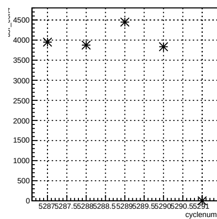
usr_coil4:cyclenum {run == 5963}
