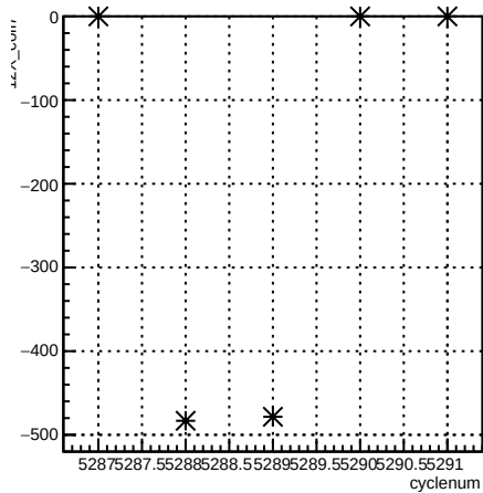
12X_coil7:cyclenum {run == 5963}
