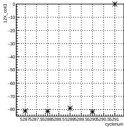
12X_coil3:cyclenum {run == 5963}
