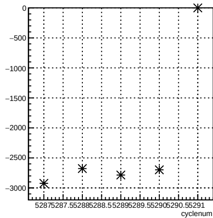
usr_coil3:cyclenum {run == 5963}
