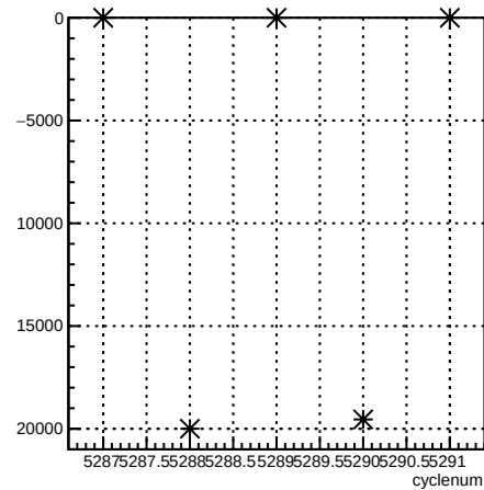
usr_coil1:cyclenum {run == 5963}
