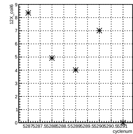
12X_coil6:cyclenum {run == 5963}
