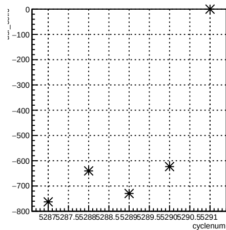
usr_coil6:cyclenum {run == 5963}
