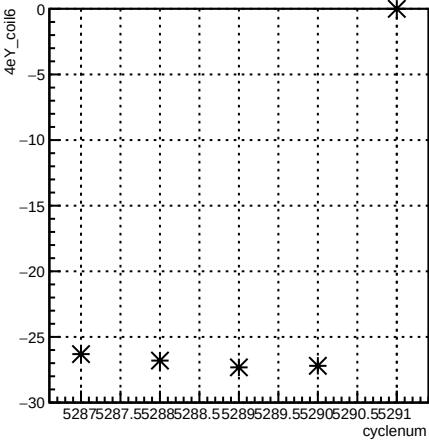
4eY_coil6:cyclenum {run == 5963}
