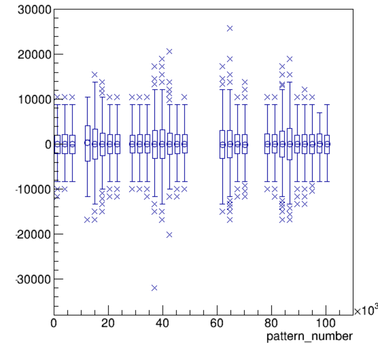
asym_sam3/ppm:pattern_number {ErrorFlag==0}
