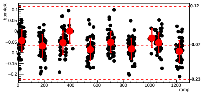
bmod_trim6,cyc=5290
