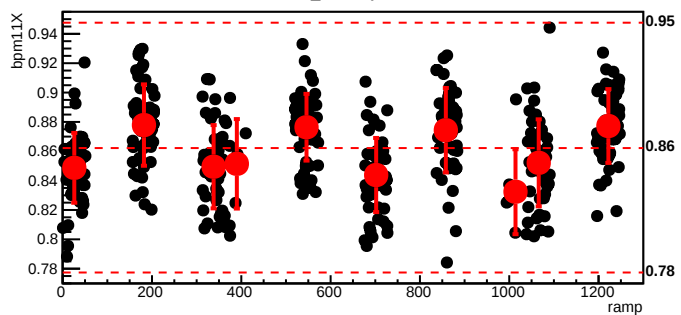
bmod_trim4,cyc=5290
