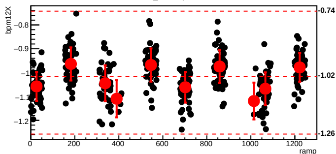
bmod_trim6,cyc=5290
