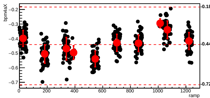
bmod_trim3,cyc=5290
