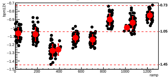
bmod_trim3,cyc=5290
