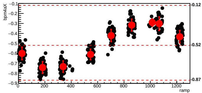
bmod_trim1,cyc=5290
