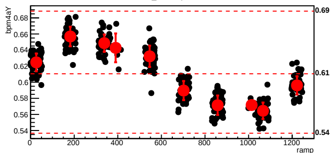
bmod_trim6,cyc=5290
