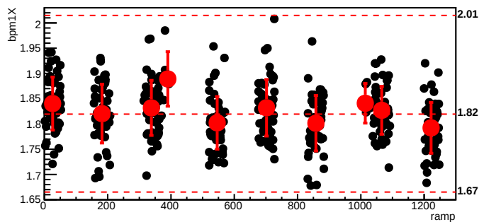
bmod_trim6,cyc=5290
