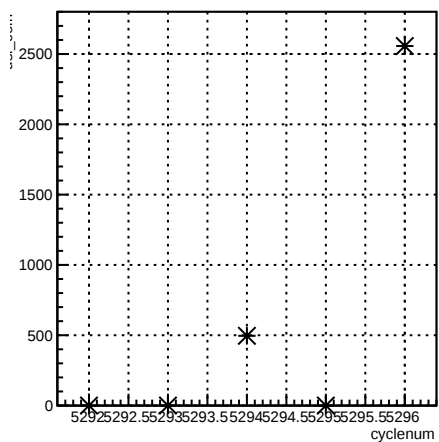
usl_coil7:cyclenum {run == 5964}
