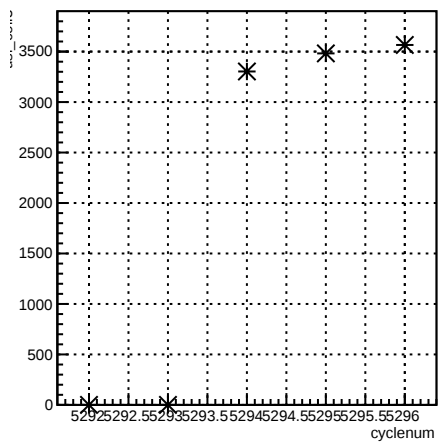
usl_coil3:cyclenum {run == 5964}
