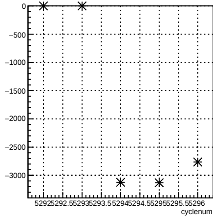
usr_coil3:cyclenum {run == 5964}
