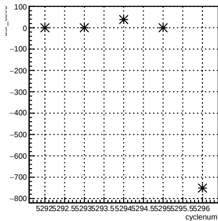
usr_coil6:cyclenum {run == 5964}
