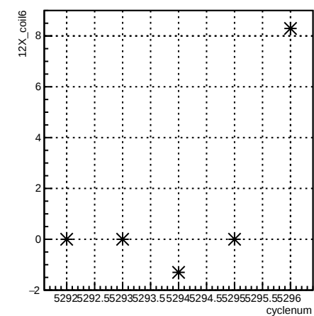
12X_coil6:cyclenum {run == 5964}
