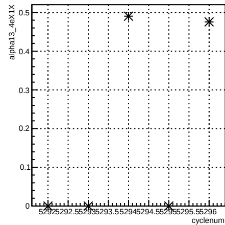
alpha13_4eX1X:cyclenum {run == 5964}
