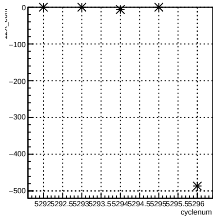
12X_coil7:cyclenum {run == 5964}
