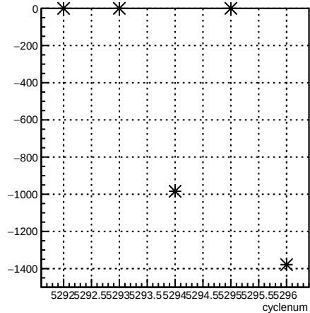
usl_coil6:cyclenum {run == 5964}
