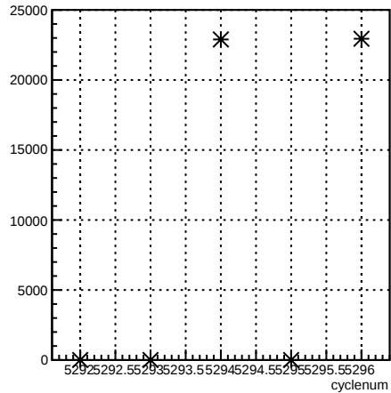
usl_coil1:cyclenum {run == 5964}
