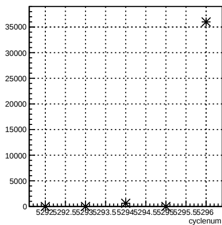
usr_coil7:cyclenum {run == 5964}
