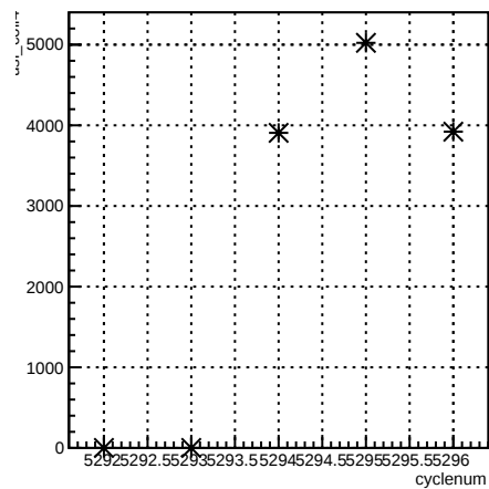
usl_coil4:cyclenum {run == 5964}
