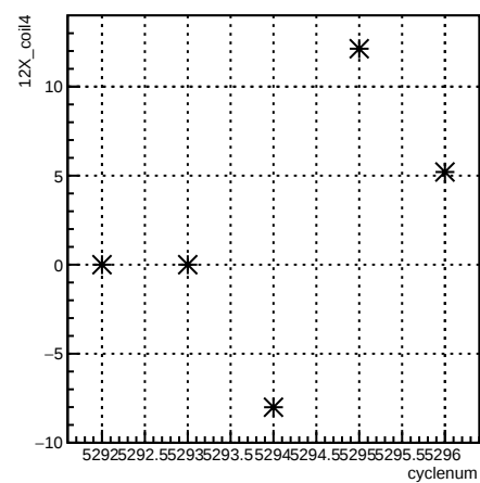
12X_coil4:cyclenum {run == 5964}
