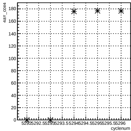
4aY_coil4:cyclenum {run == 5964}
