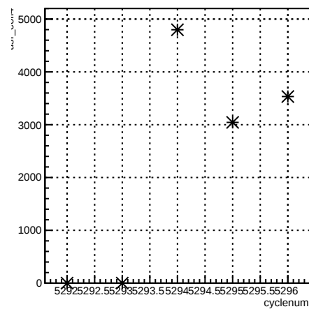
usr_coil4:cyclenum {run == 5964}
