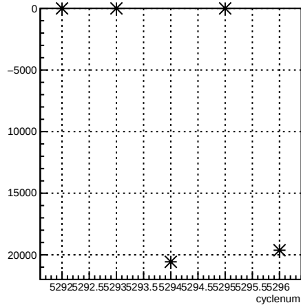
usr_coil1:cyclenum {run == 5964}
