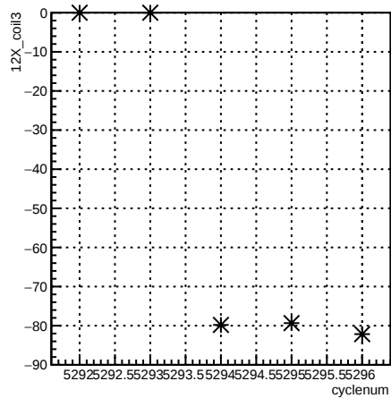
12X_coil3:cyclenum {run == 5964}
