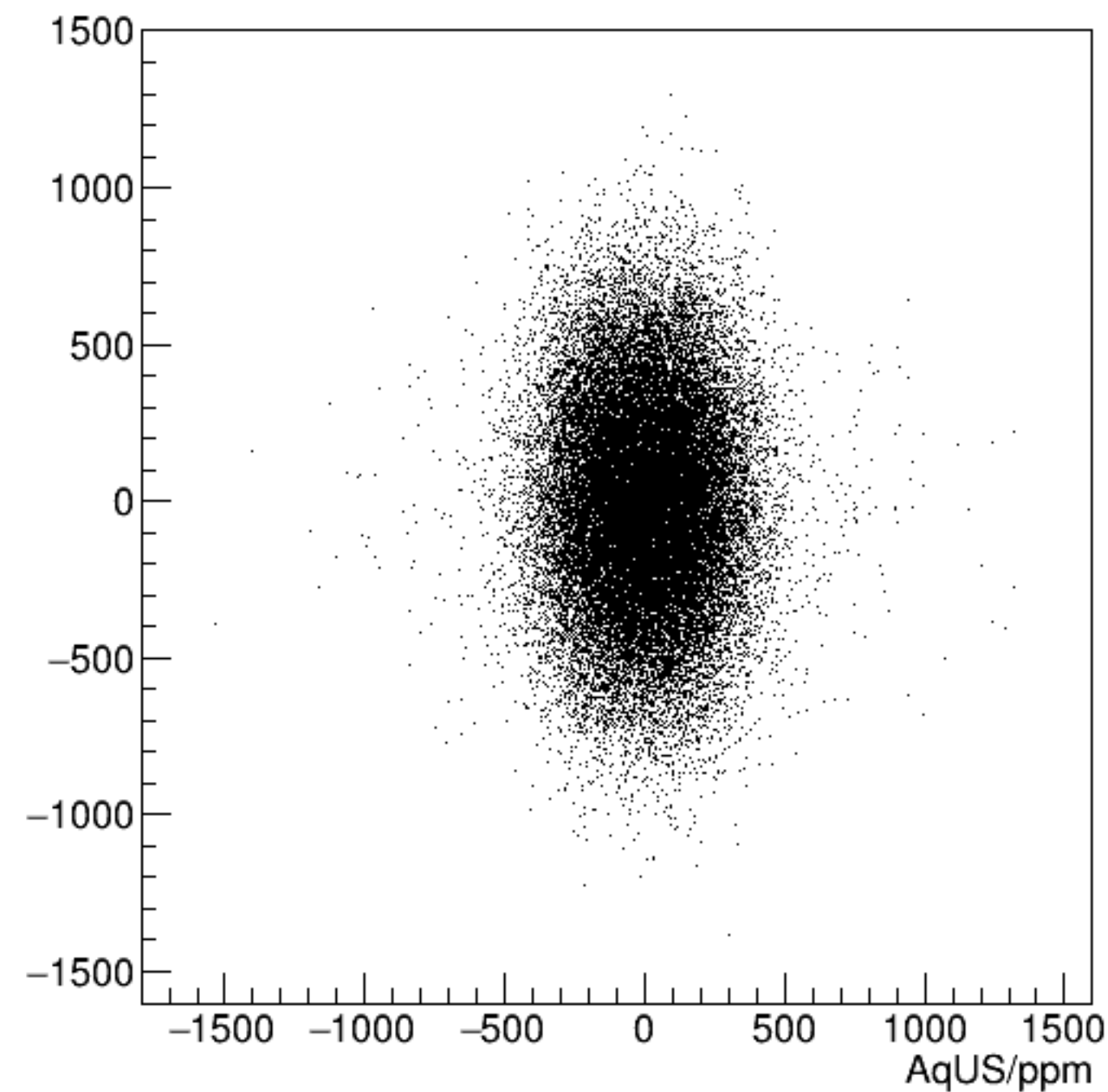
reg_asym_dsl/ppm:AqUS/ppm {ok_cut}
