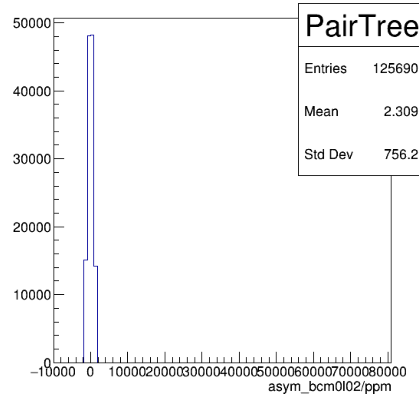
asym_bcm0l02/ppm {ErrorFlag==0}
