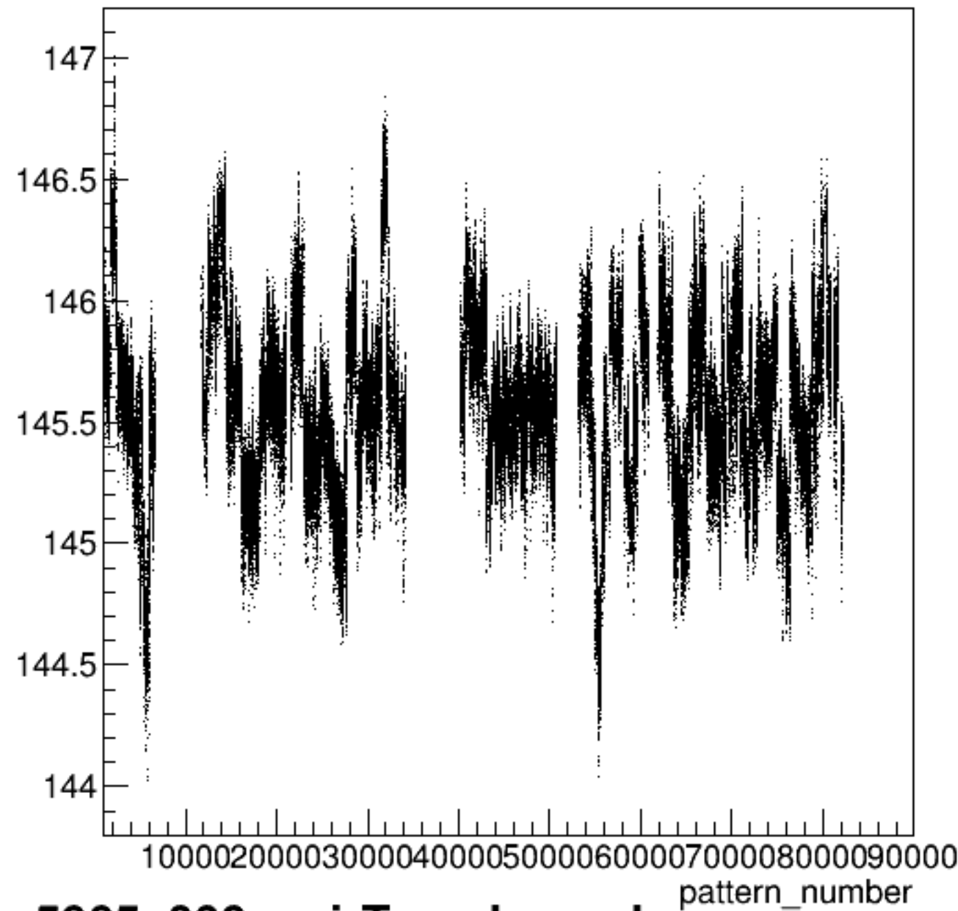
yield_bcm_dg_us:pattern_number {ErrorFlag==0}
