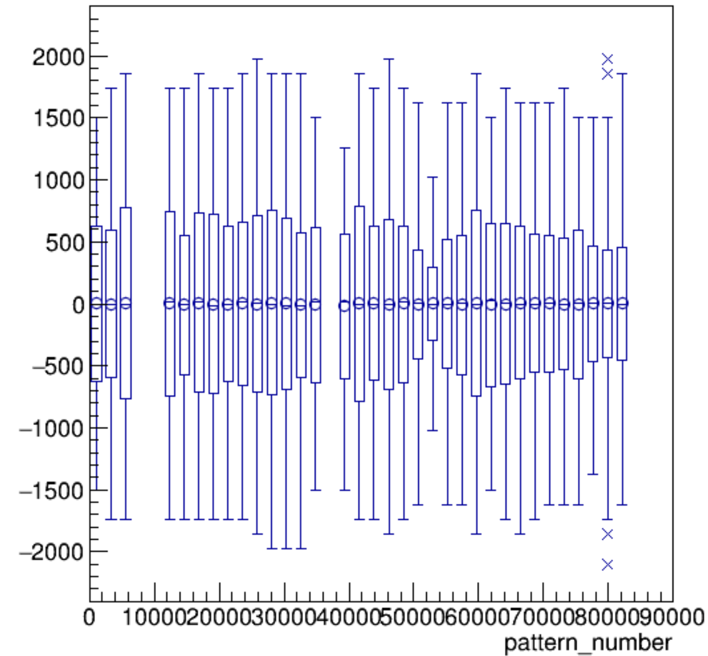
asym_bcm_dg_us/ppm:pattern_number {ErrorFlag==0}
