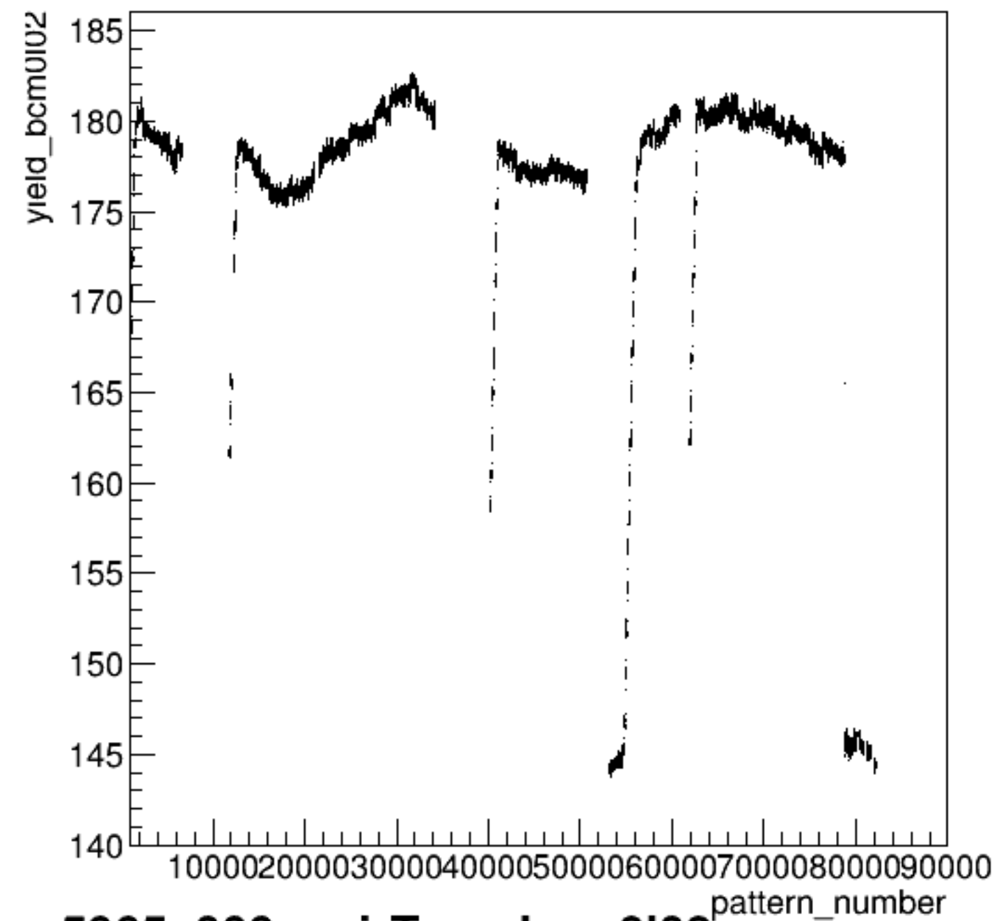
yield_bcm0l02:pattern_number {ErrorFlag==0}
