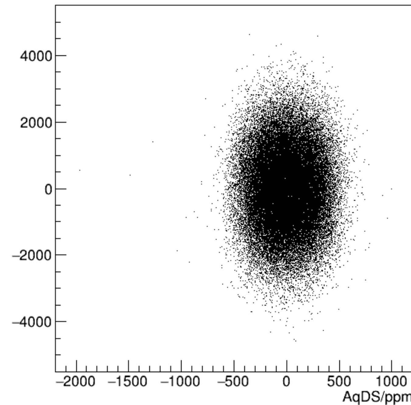
reg_asym_usr/ppm:AqDS/ppm {ok_cut}
