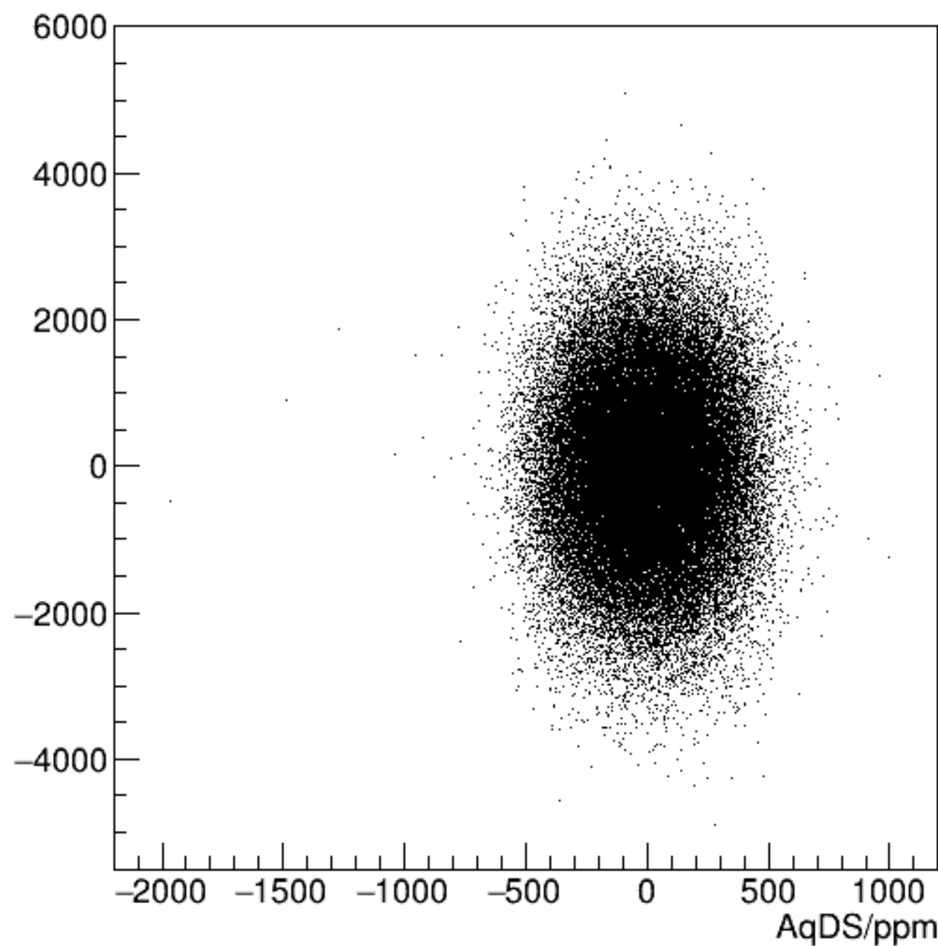
reg_asym_usl/ppm:AqDS/ppm {ok_cut}
