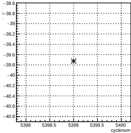
4eX_coil3:cyclenum {run == 6089}
