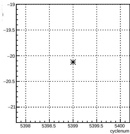
1X_coil3:cyclenum {run == 6089}
