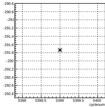
1X_coil1:cyclenum {run == 6089}
