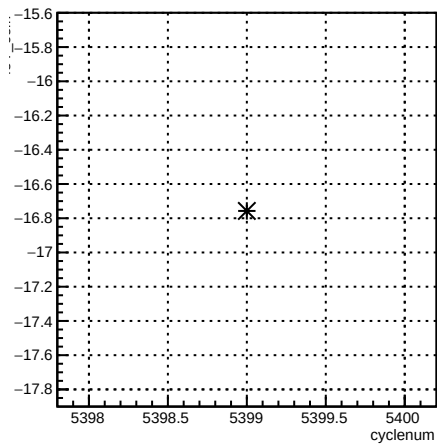
4eY_coil7:cyclenum {run == 6089}
