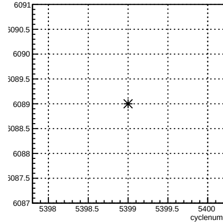
run:cyclenum {run == 6089}
