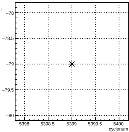
usl_4eY:cyclenum {run == 6089}
