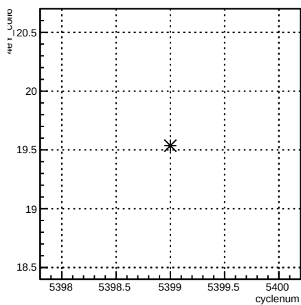
4eY_coil6:cyclenum {run == 6089}
