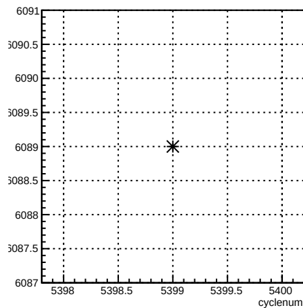
run:cyclenum {run == 6089}
