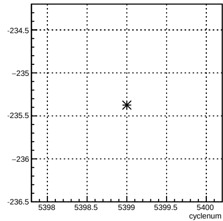
12X_coil6:cyclenum {run == 6089}
