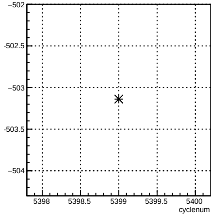
12X_coil7:cyclenum {run == 6089}
