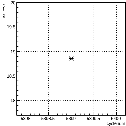
usl_4eY:cyclenum {run == 6089}
