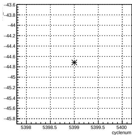
usr_12X:cyclenum {run == 6089}
