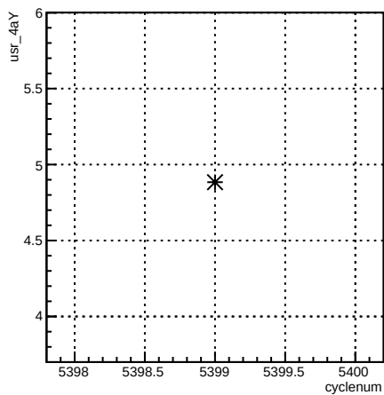
usr_4aY:cyclenum {run == 6089}
