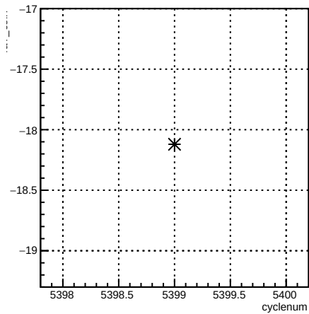
4aY_coil7:cyclenum {run == 6089}
