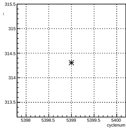
1X_coil7:cyclenum {run == 6089}
