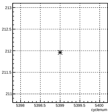
4eY_coil4:cyclenum {run == 6089}
