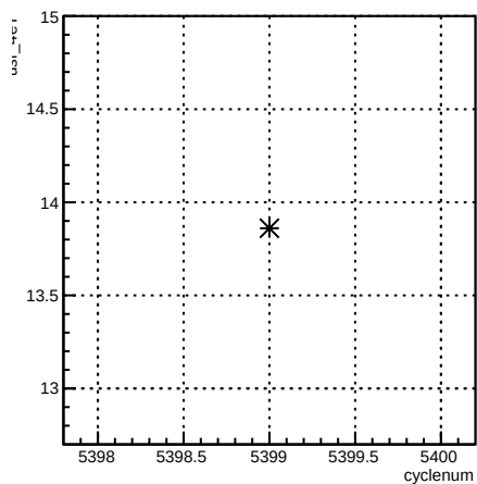
usr_4eY:cyclenum {run == 6089}
