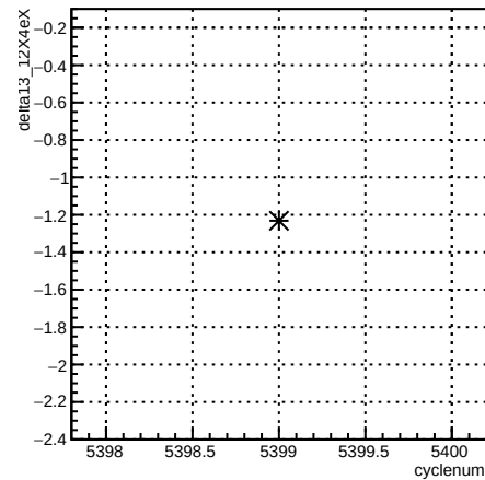
segment:cyclenum {run == 6089}
