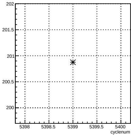
4aY_coil4:cyclenum {run == 6089}
