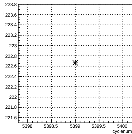
usr_4eX:cyclenum {run == 6089}
