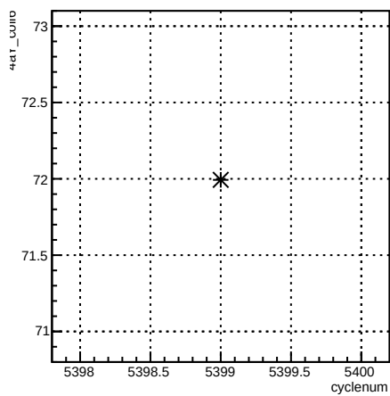
4aY_coil6:cyclenum {run == 6089}
