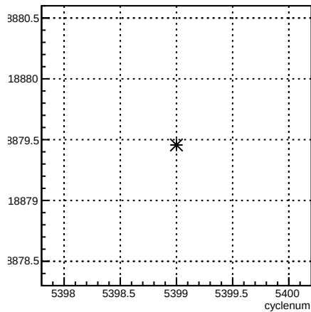
usl_coil6:cyclenum {run == 6089}
