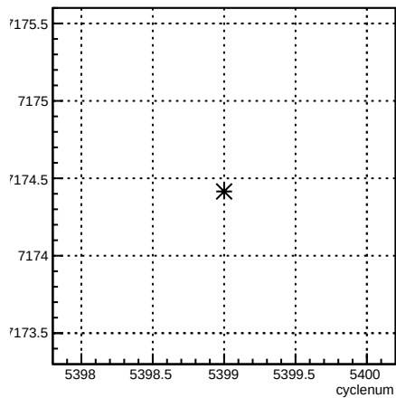
usl_coil7:cyclenum {run == 6089}
