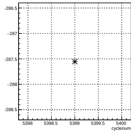
4eX_coil1:cyclenum {run == 6089}
