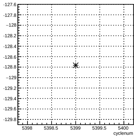
usr_1X:cyclenum {run == 6089}
