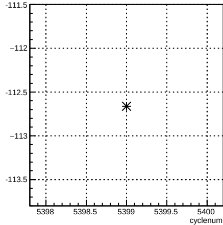
usr_coil6:cyclenum {run == 6089}
