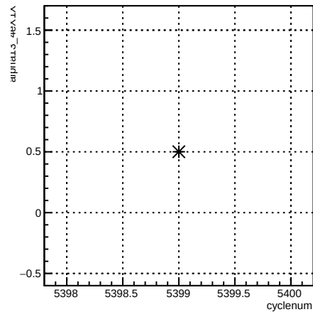
delta46_12X4eY:cyclenum {run == 6089}
