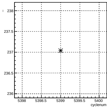
4eX_coil7:cyclenum {run == 6089}
