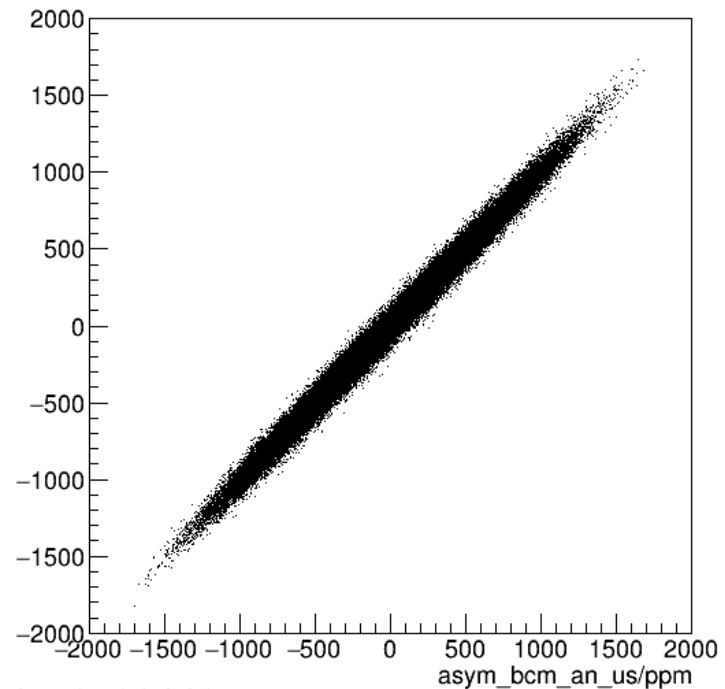
run6090_000_asym_bcm_dg_ds_vs_asym_bcm_an_us_pr.png
