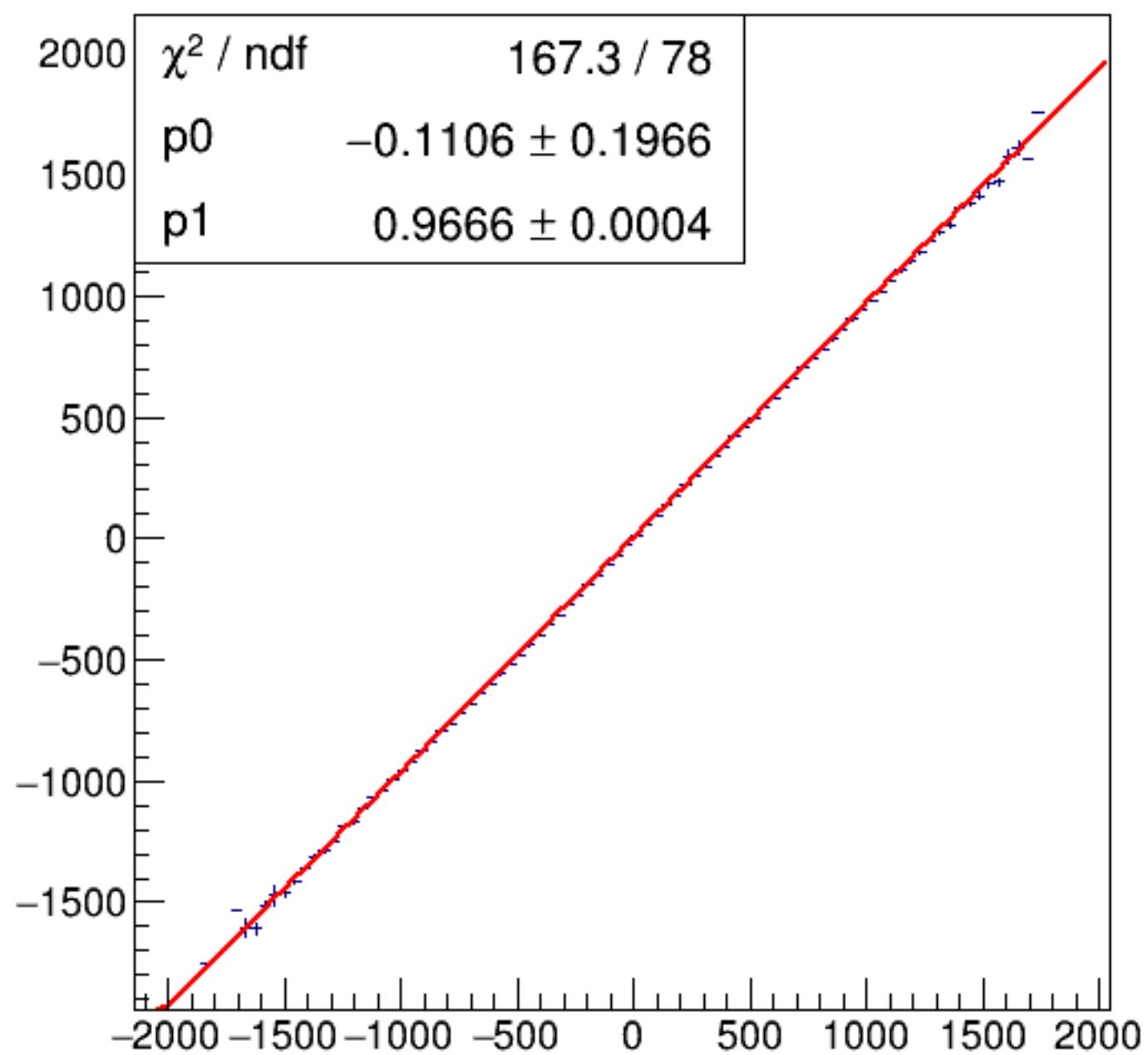
run6090_000_asym_bcm_dg_us_vs_asym_bcm_dg_ds_pr.png
