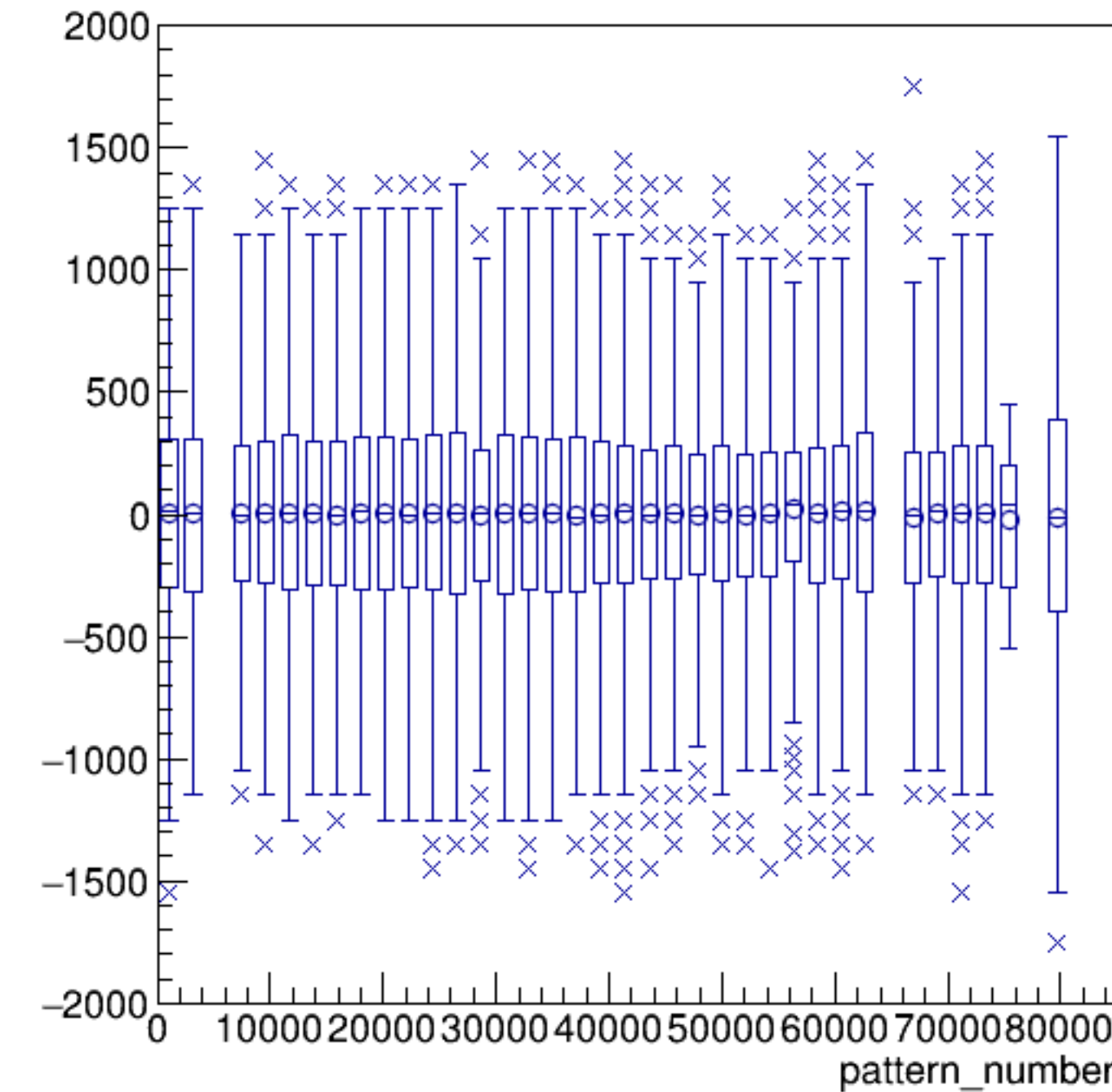
asym_bcm0l02/ppm:pattern_number {ErrorFlag==0}
