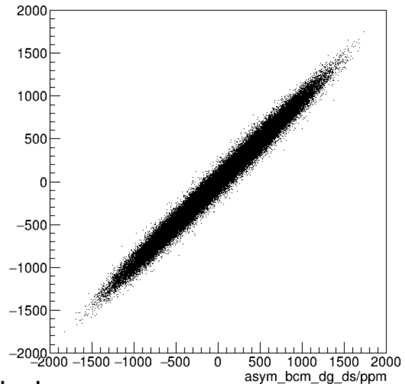
run6090_000_asym_bcm_dg_us_vs_asym_bcm_dg_ds_pr.png
