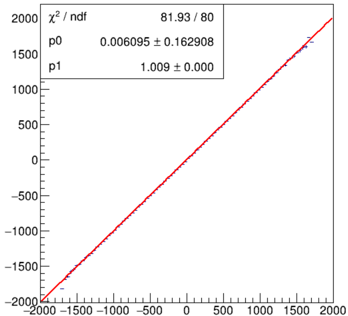
run6090_000_asym_bcm_dg_ds_vs_asym_bcm_an_us_pr.png
