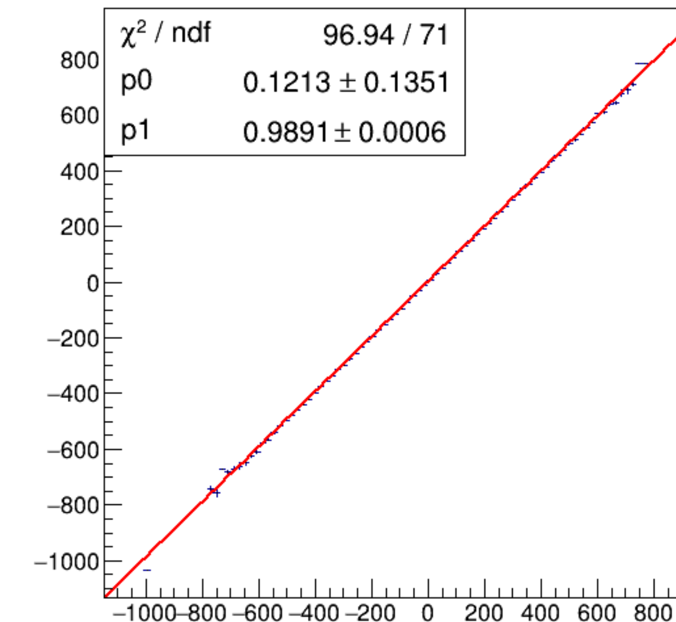
run6091_000_asym_bcm_an_us_vs_asym_bcm_an_ds3_mul.png
