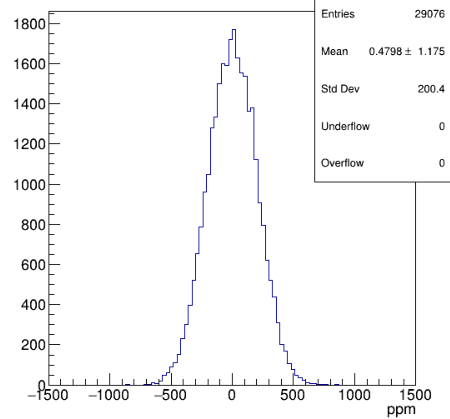
asym_bcm0l02
