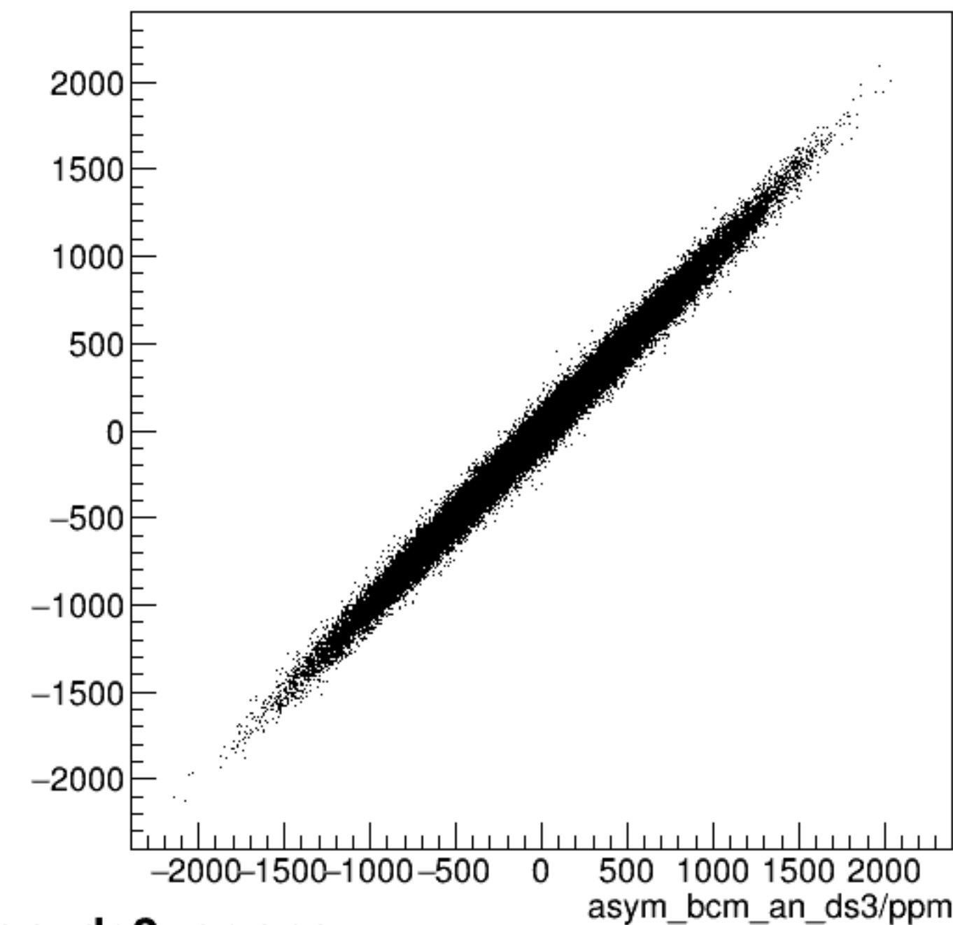
run6091_000_asym_bcm_dg_us_vs_asym_bcm_an_ds3_pr.png
