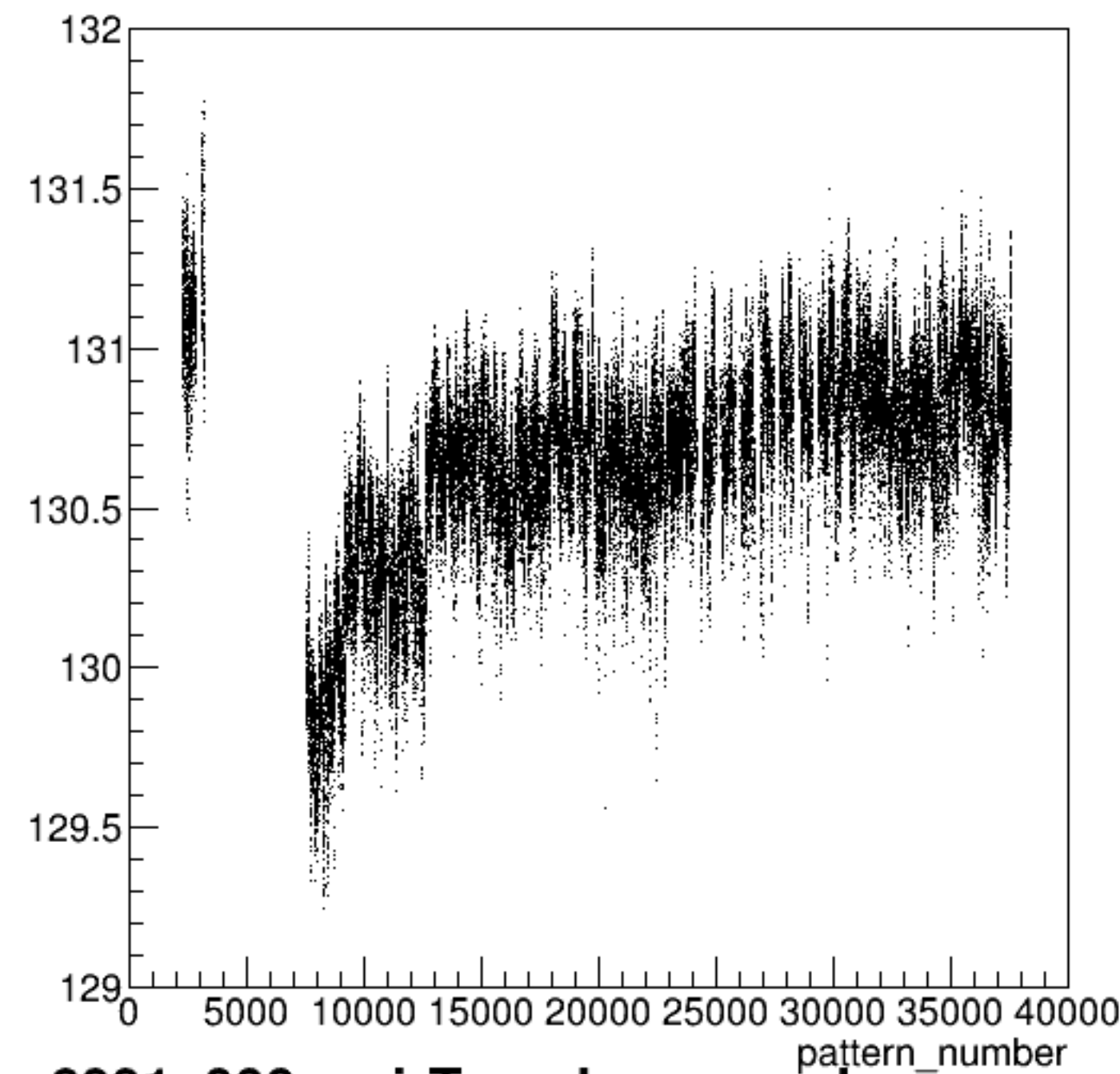
yield_bcm_an_ds:pattern_number {ErrorFlag==0}
