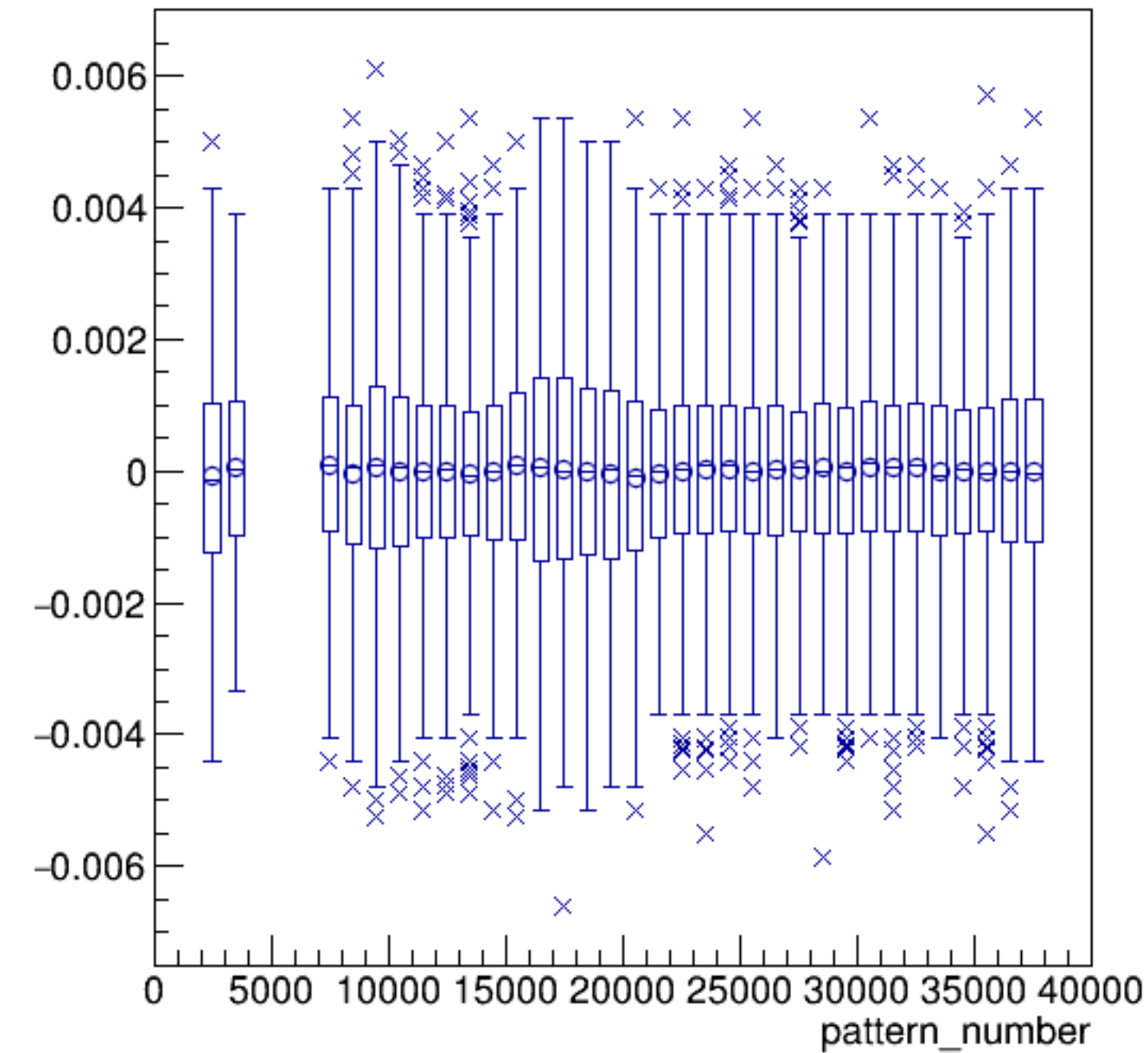
asym_bcm_an_diff*yield_bcm_an_diff:pattern_number {ErrorFlag==0}
