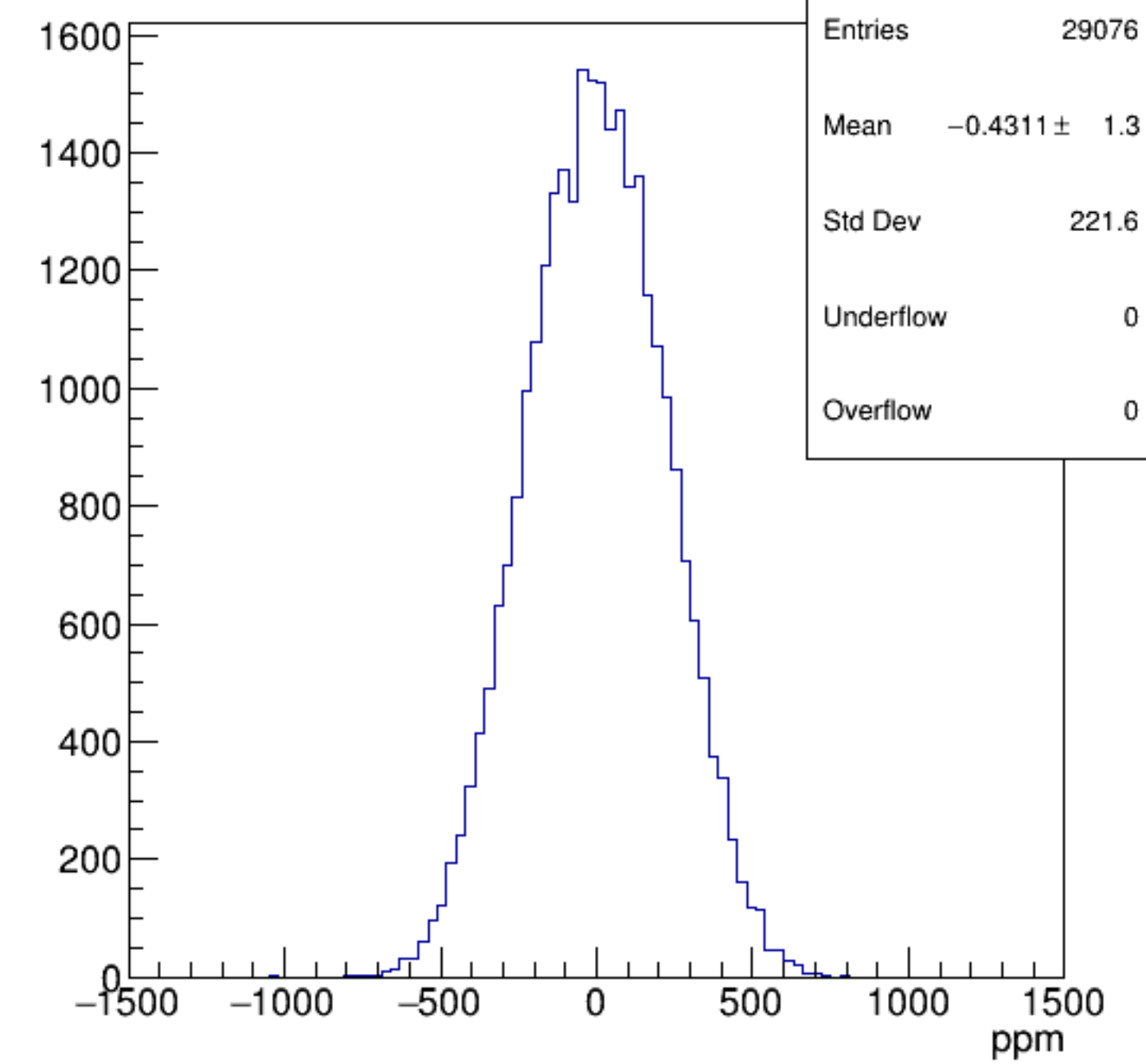
asym_bcm_an_us
