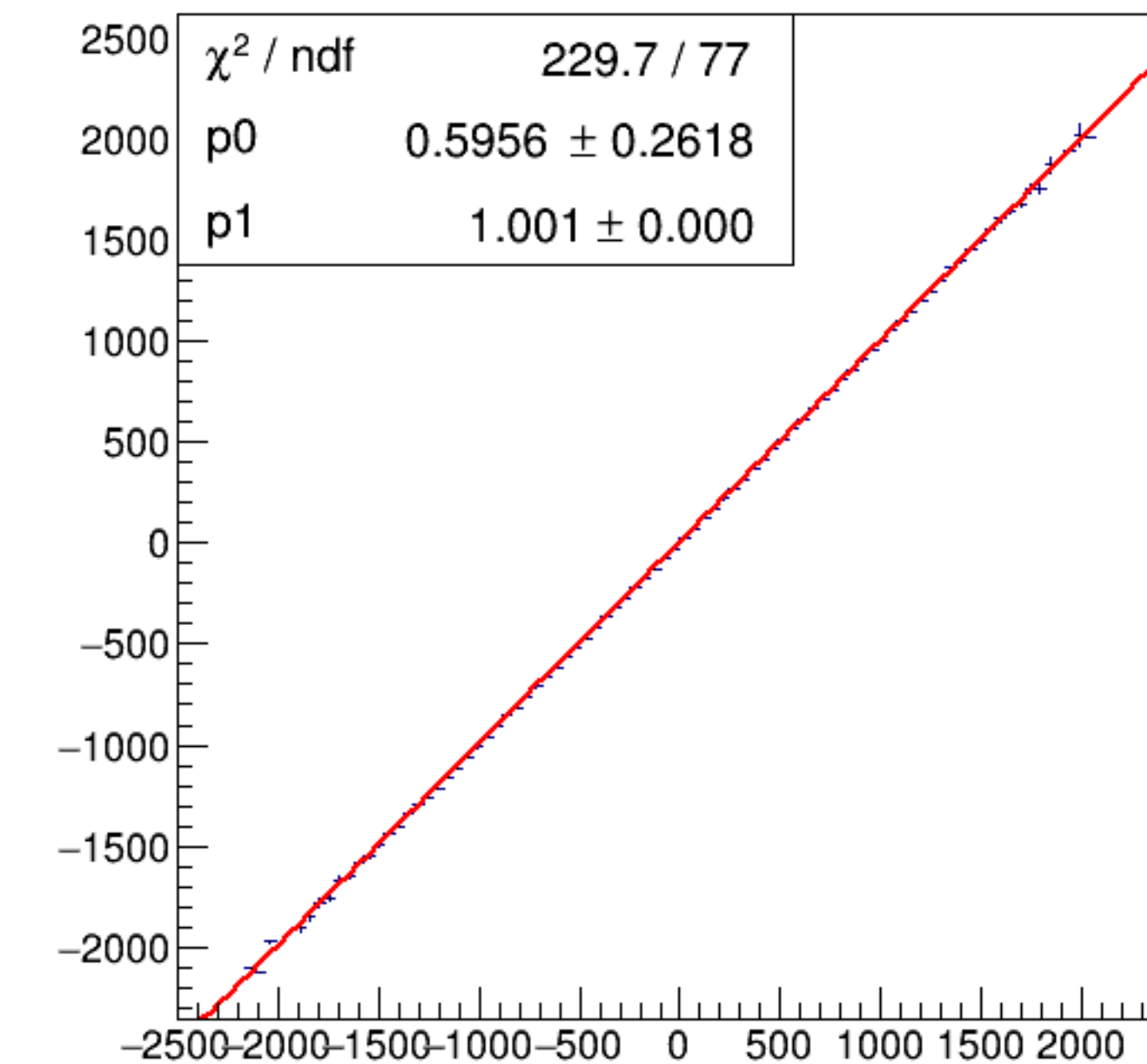
run6091_000_asym_bcm_dg_us_vs_asym_bcm_an_ds3_pr.png
