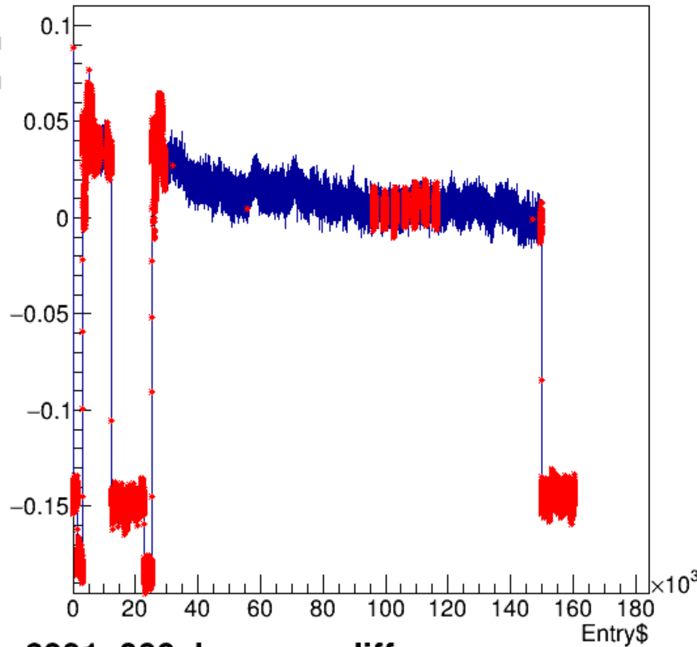
bcm_an_diff:Entry$
