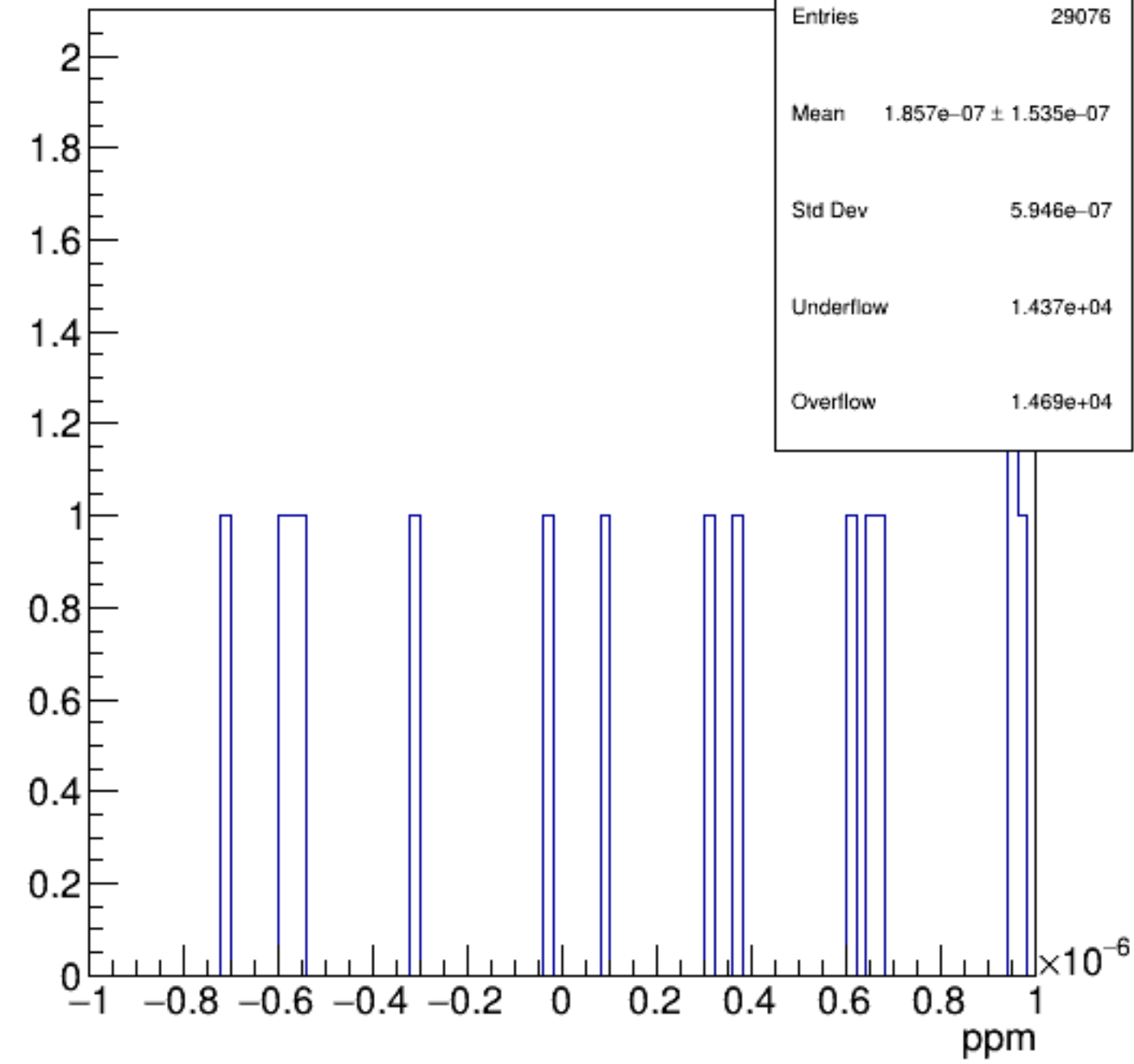
asym_bcm_an_diff
