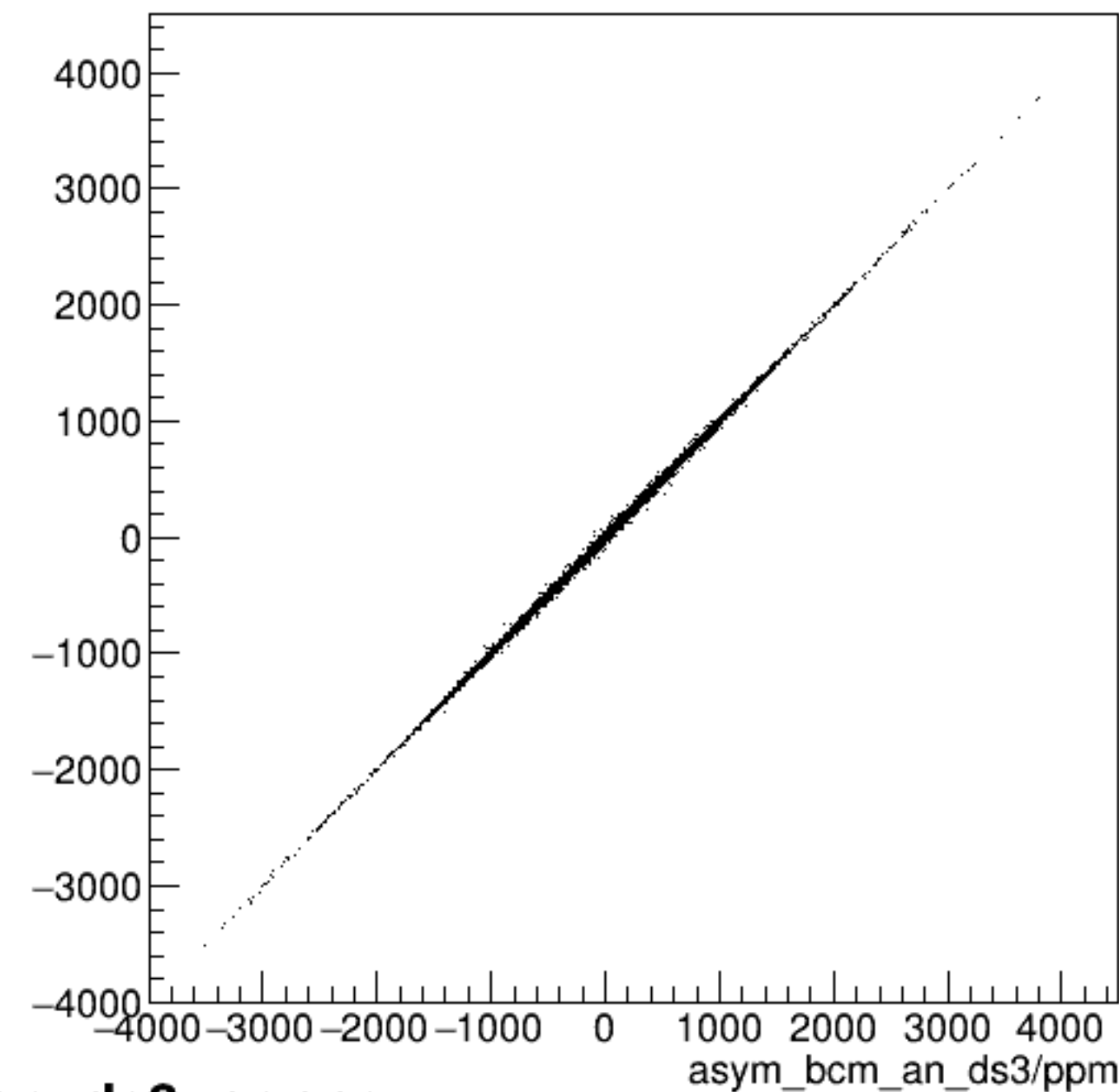
run6093_000_asym_bcm_an_ds_vs_asym_bcm_an_ds3_pr.png
