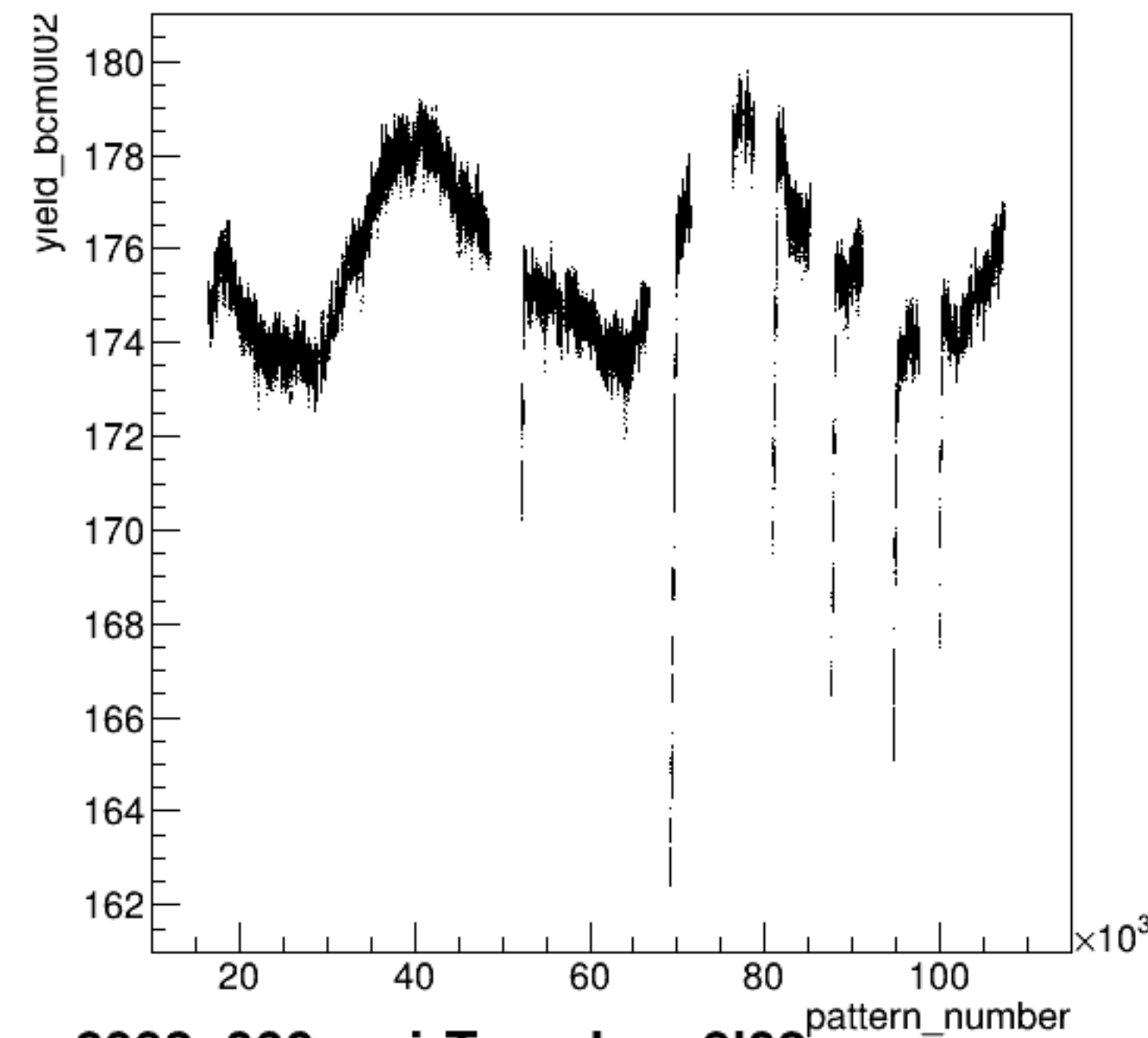
yield_bcm0l02:pattern_number {ErrorFlag==0}
