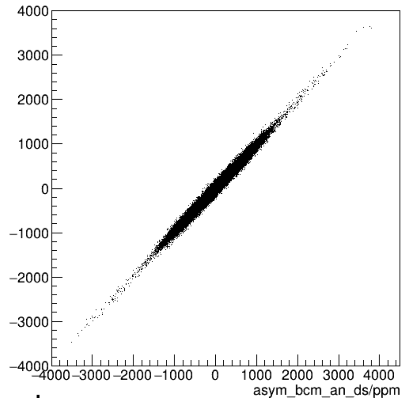
run6093_000_asym_bcm_dg_us_vs_asym_bcm_an_ds_pr.png
