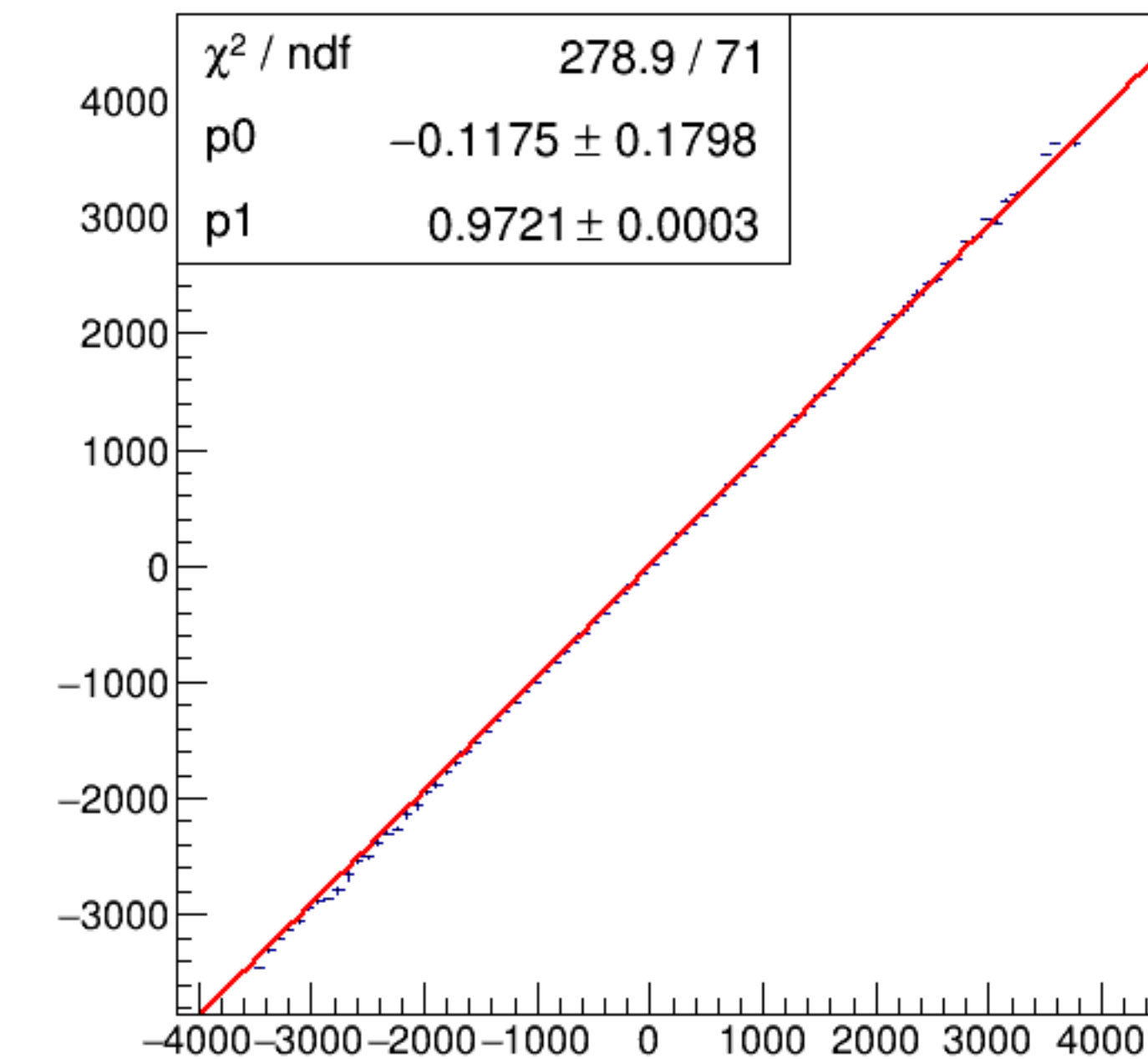
run6093_000_asym_bcm_dg_us_vs_asym_bcm_an_ds3_pr.png
