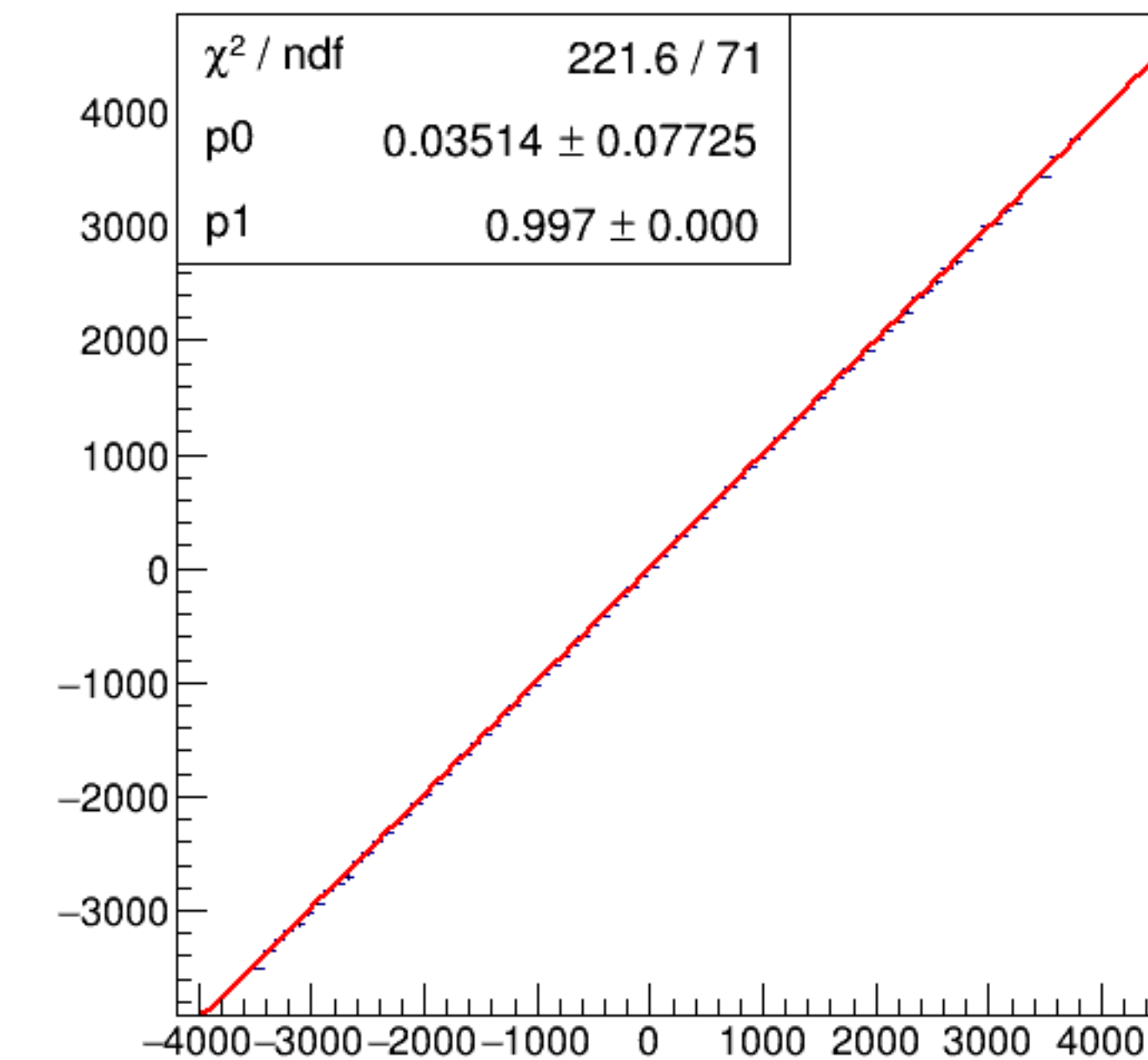
run6093_000_asym_bcm_an_ds_vs_asym_bcm_an_ds3_pr.png
