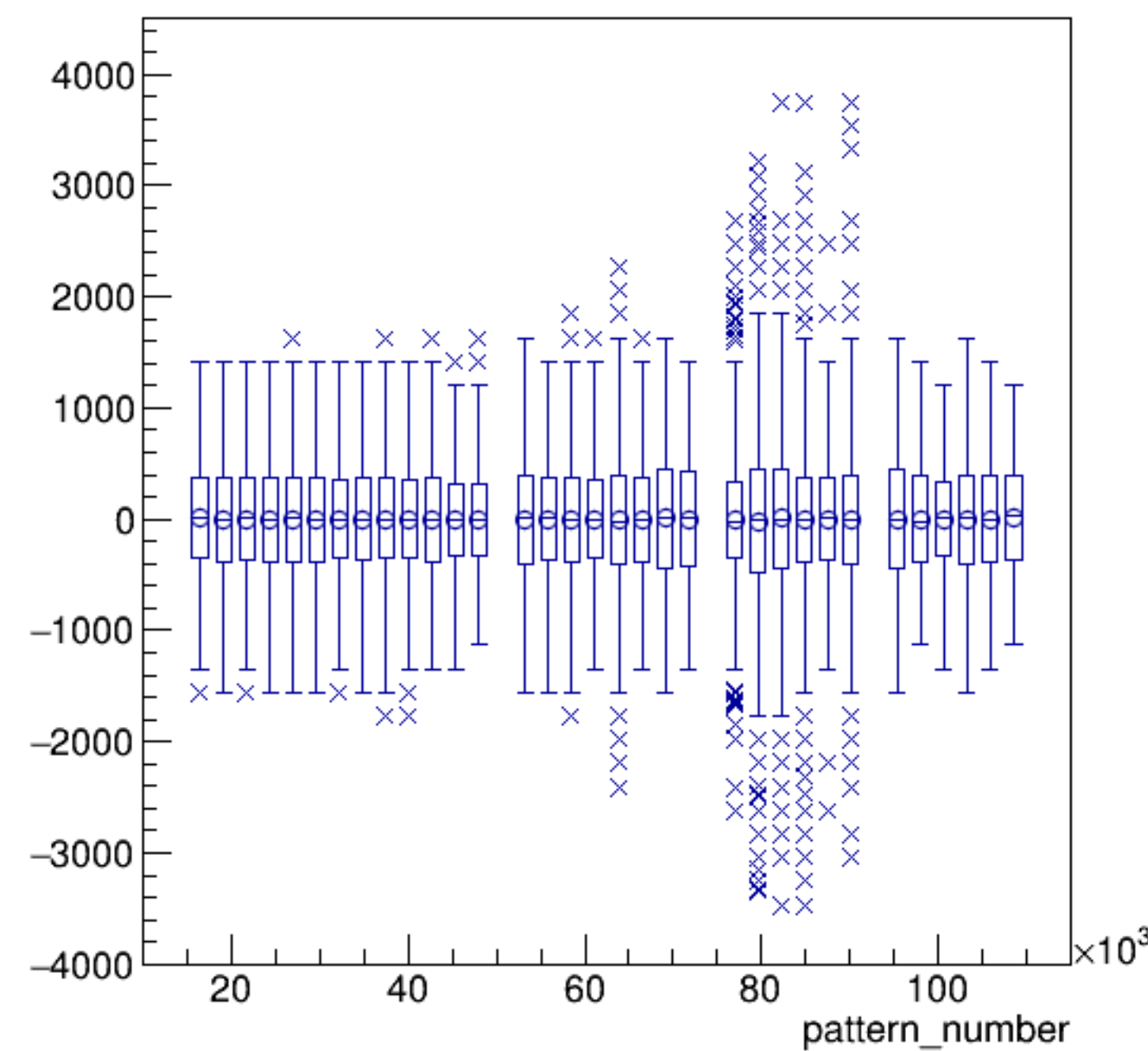
asym_bcm_dg_ds/ppm:pattern_number {ErrorFlag==0}
