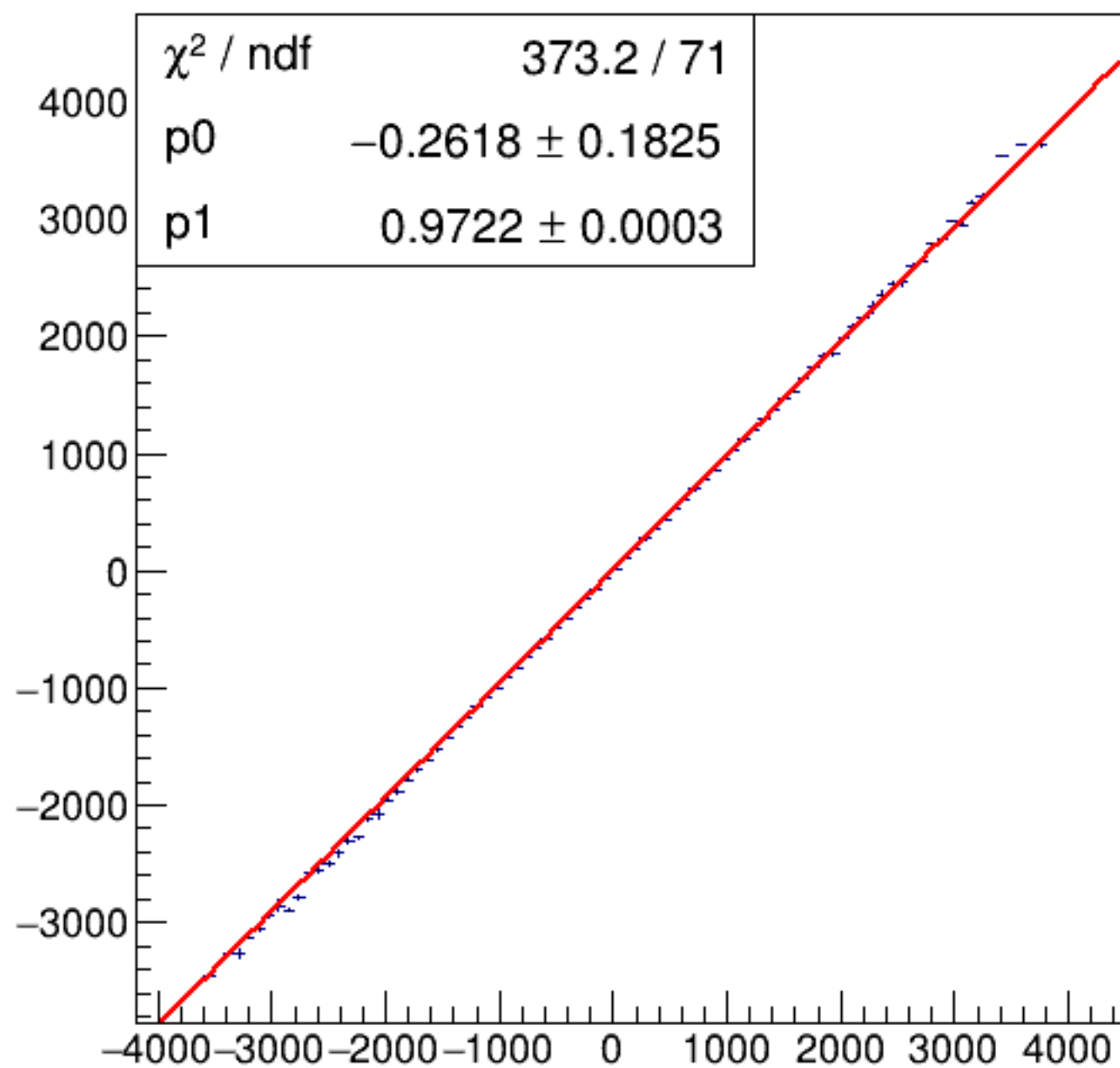
run6093_000_asym_bcm_dg_us_vs_asym_bcm_an_ds_pr.png
