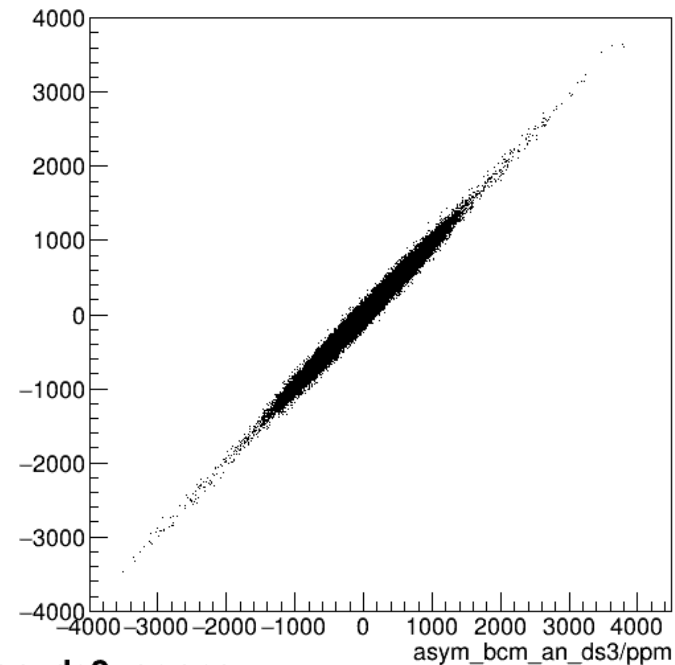
run6093_000_asym_bcm_dg_us_vs_asym_bcm_an_ds3_pr.png
