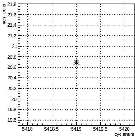
4eY_coil6:cyclenum {run == 6094}
