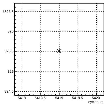
1X_coil7:cyclenum {run == 6094}
