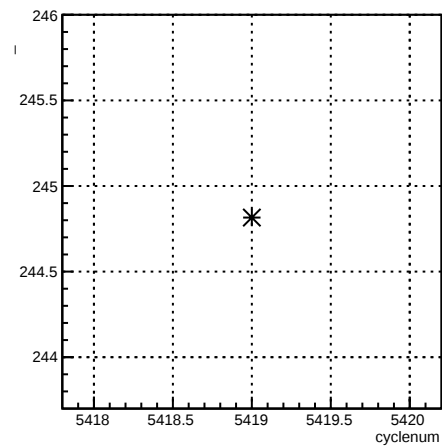
4eX_coil7:cyclenum {run == 6094}
