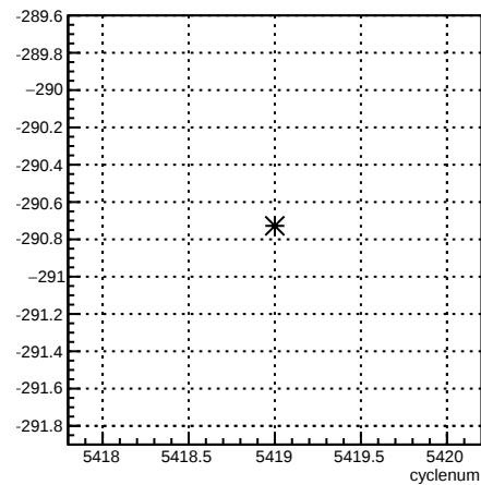
1X_coil1:cyclenum {run == 6094}
