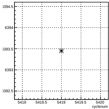
usl_coil7:cyclenum {run == 6094}
