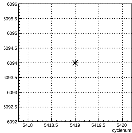
run:cyclenum {run == 6094}
