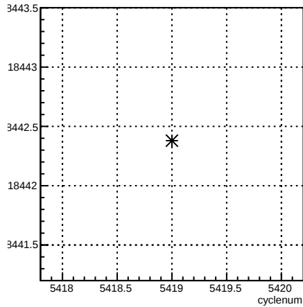
usl_coil1:cyclenum {run == 6094}
