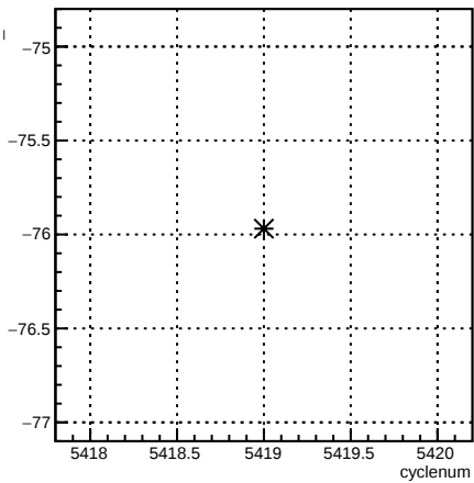
usl_4eY:cyclenum {run == 6094}
