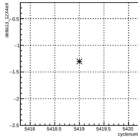
delta13_12X4eX:cyclenum {run == 6094}
