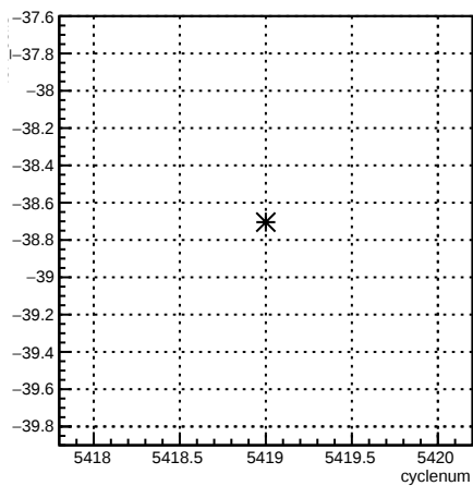
4eX_coil3:cyclenum {run == 6094}
