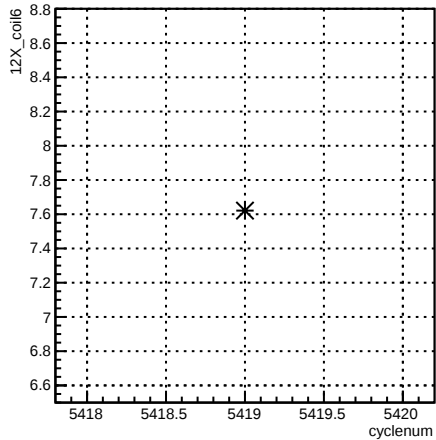
12X_coil6:cyclenum {run == 6094}
