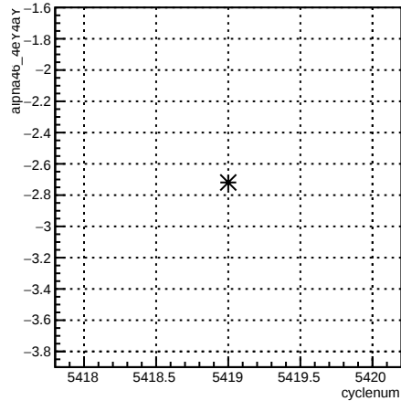
alpha46_4eY4aY:cyclenum {run == 6094}
