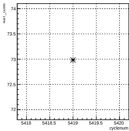
4aY_coil6:cyclenum {run == 6094}
