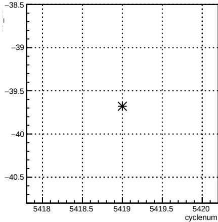
usl_12X:cyclenum {run == 6094}
