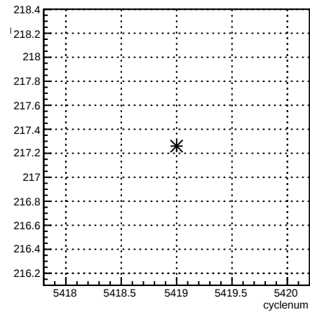
usr_4eX:cyclenum {run == 6094}
