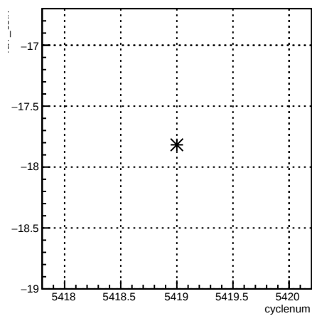
4aY_coil7:cyclenum {run == 6094}
