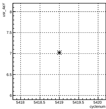
usr_4aY:cyclenum {run == 6094}
