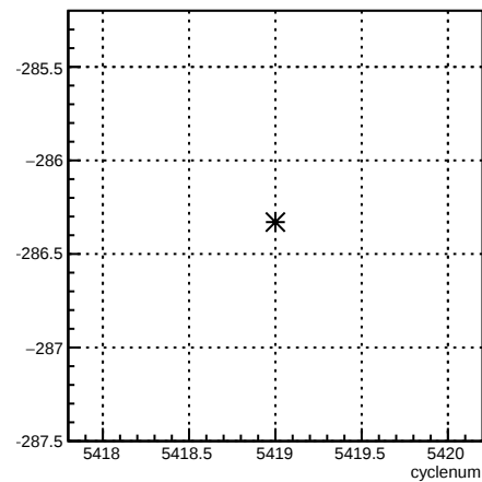
4eX_coil1:cyclenum {run == 6094}
