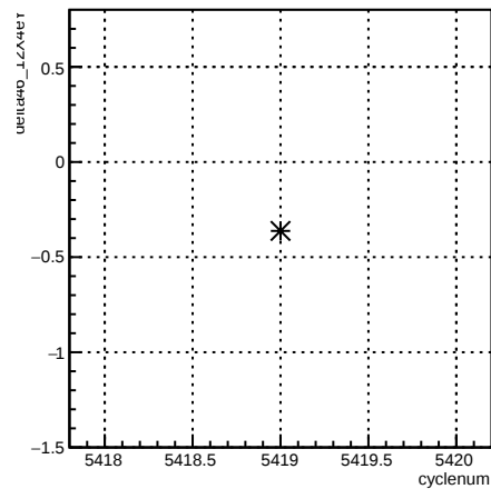
delta46_12X4eY:cyclenum {run == 6094}
