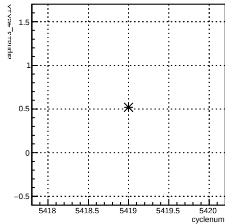
alpha13_4eX1X:cyclenum {run == 6094}
