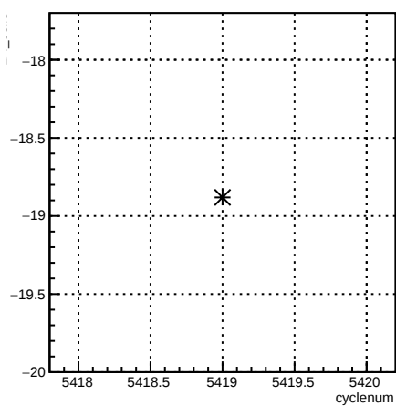
1X_coil3:cyclenum {run == 6094}
