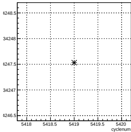
usr_coil7:cyclenum {run == 6094}
