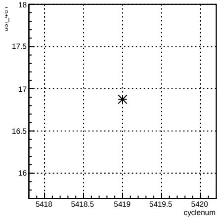
usl_4eY:cyclenum {run == 6094}
