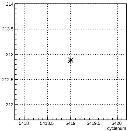
4eY_coil4:cyclenum {run == 6094}
