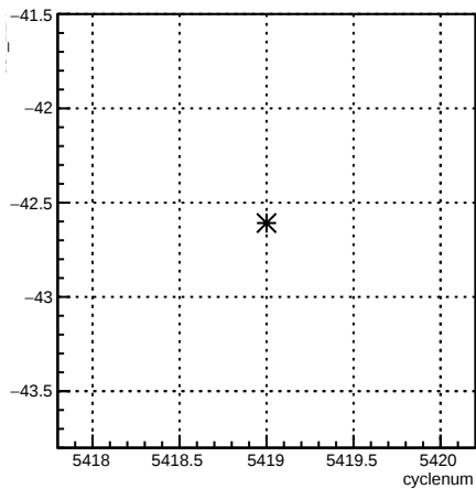
usr_12X:cyclenum {run == 6094}
