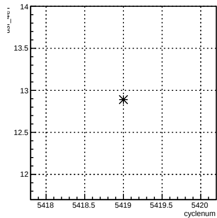
usr_4eY:cyclenum {run == 6094}
