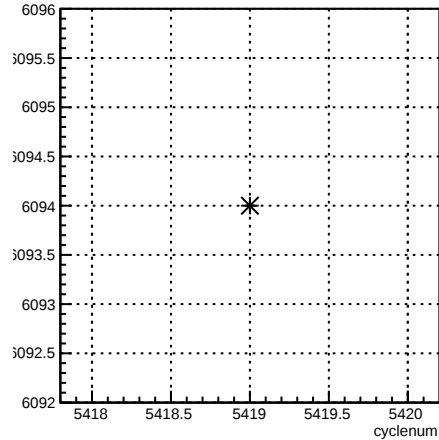
run:cyclenum {run == 6094}
