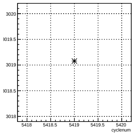
usl_coil3:cyclenum {run == 6094}
