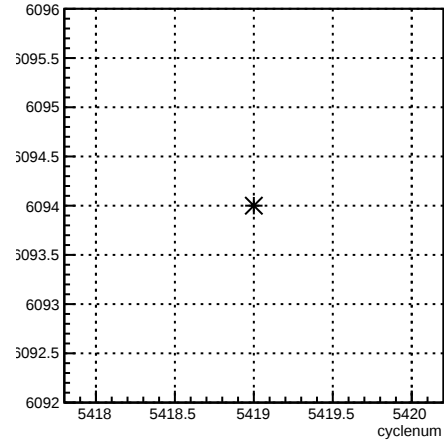
run:cyclenum {run == 6094}
