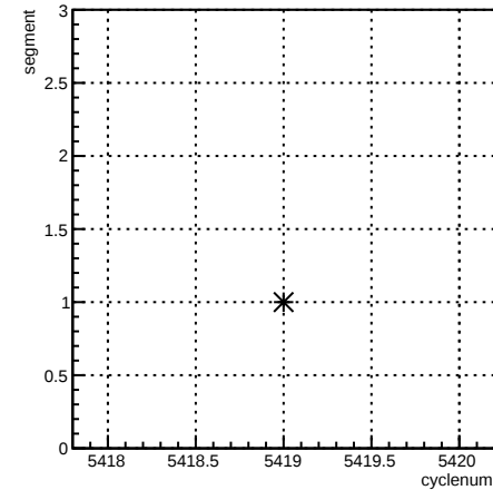
segment:cyclenum {run == 6094}
