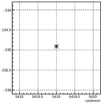
12X_coil6:cyclenum {run == 6094}
