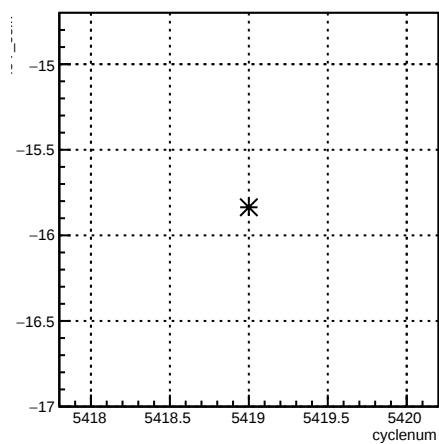
4eY_coil7:cyclenum {run == 6094}
