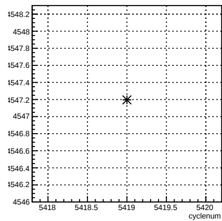
usl_coil4:cyclenum {run == 6094}
