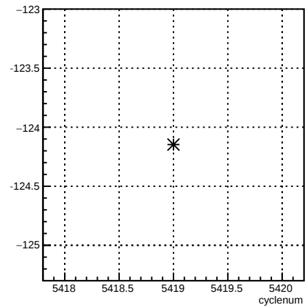
usr_1X:cyclenum {run == 6094}
