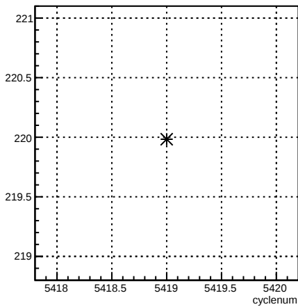
usl_coil6:cyclenum {run == 6094}
