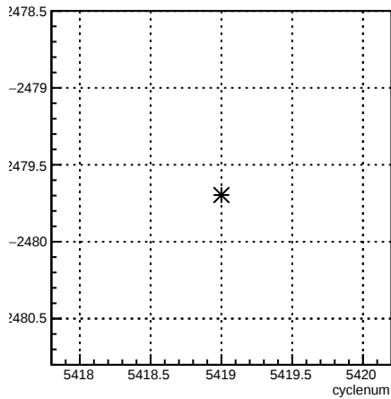
usr_coil3:cyclenum {run == 6094}
