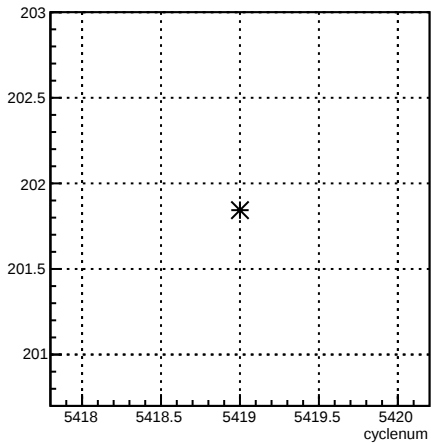
4aY_coil4:cyclenum {run == 6094}
