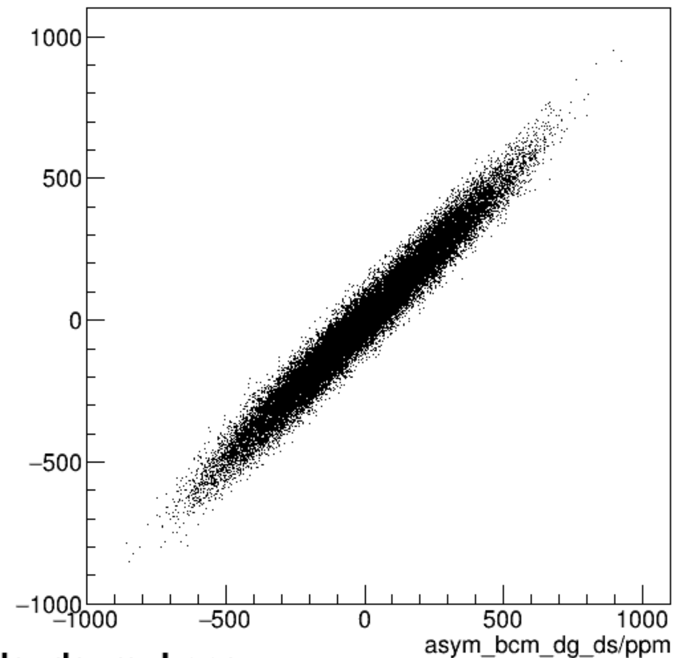
run6094_000_asym_bcm_dg_us_vs_asym_bcm_dg_ds_mul.png
