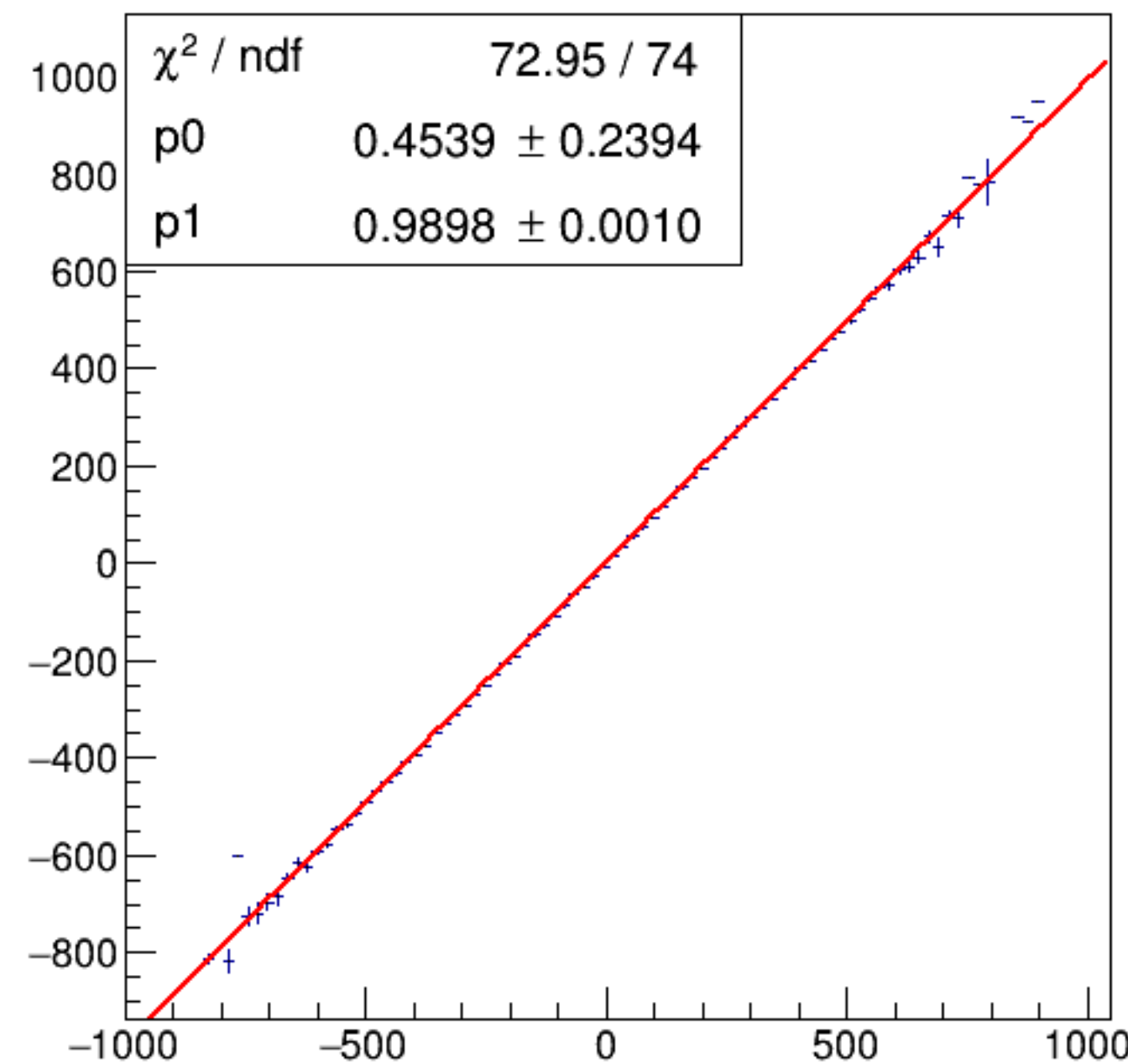
run6094_000_asym_bcm_dg_us_vs_asym_bcm_an_ds3_mul.png
