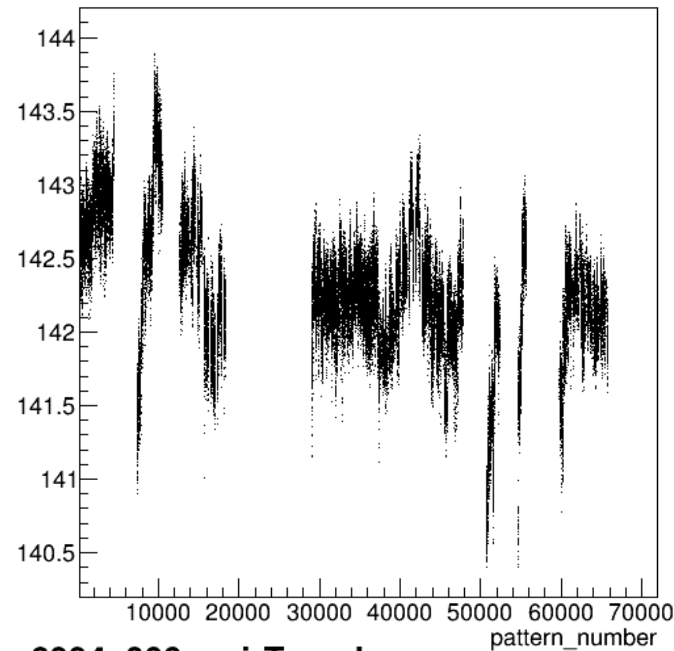
yield_bcm_an_us:pattern_number {ErrorFlag==0}
