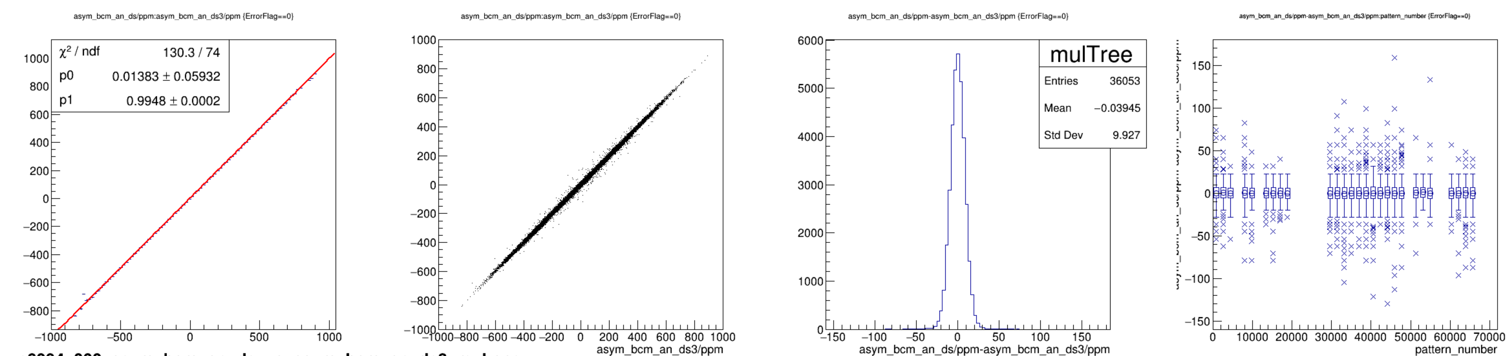
run6094_000_asym_bcm_an_ds_vs_asym_bcm_an_ds3_mul.png
