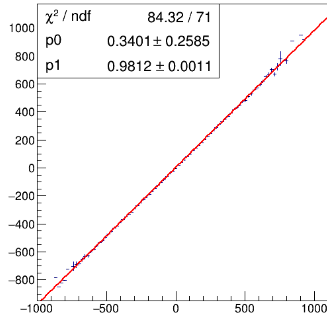
run6094_000_asym_bcm_dg_us_vs_asym_bcm_dg_ds_mul.png
