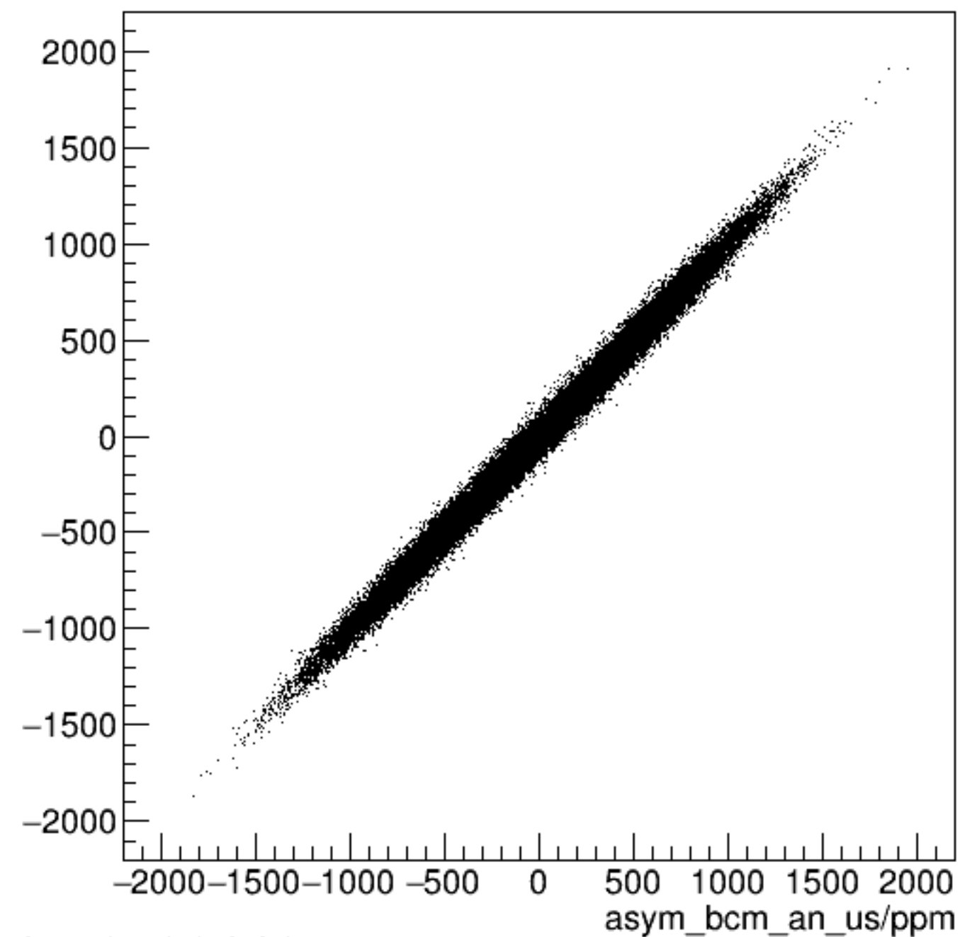
run6094_000_asym_bcm_dg_ds_vs_asym_bcm_an_us_pr.png
