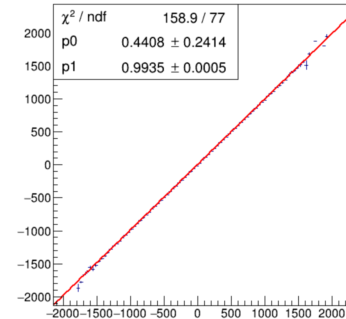
run6094_000_asym_bcm_dg_us_vs_asym_bcm_an_ds3_pr.png
