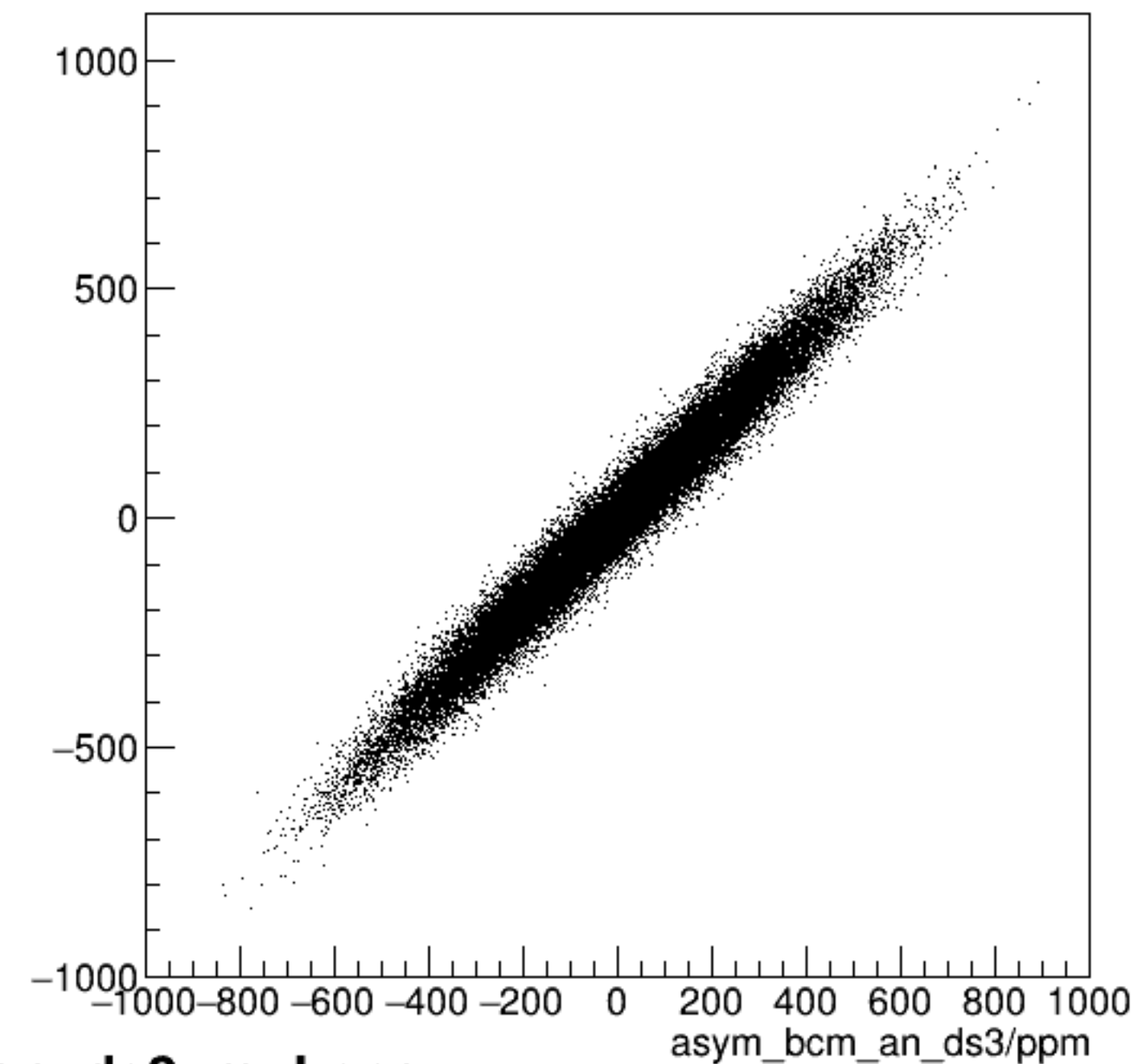
run6094_000_asym_bcm_dg_us_vs_asym_bcm_an_ds3_mul.png
