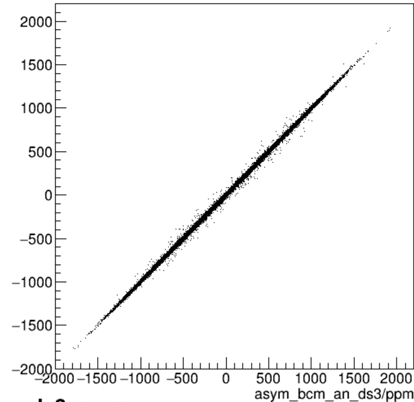
run6094_000_asym_bcm_an_ds_vs_asym_bcm_an_ds3_pr.png
