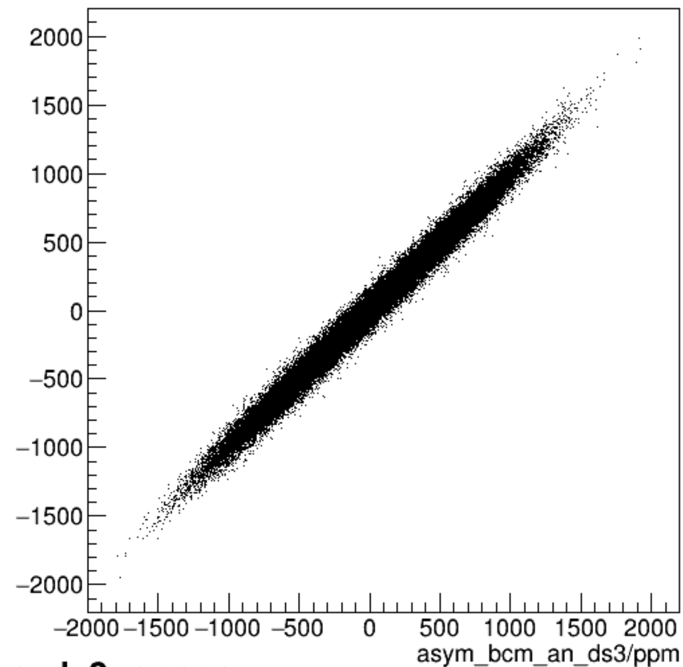
run6094_000_asym_bcm_dg_us_vs_asym_bcm_an_ds3_pr.png
