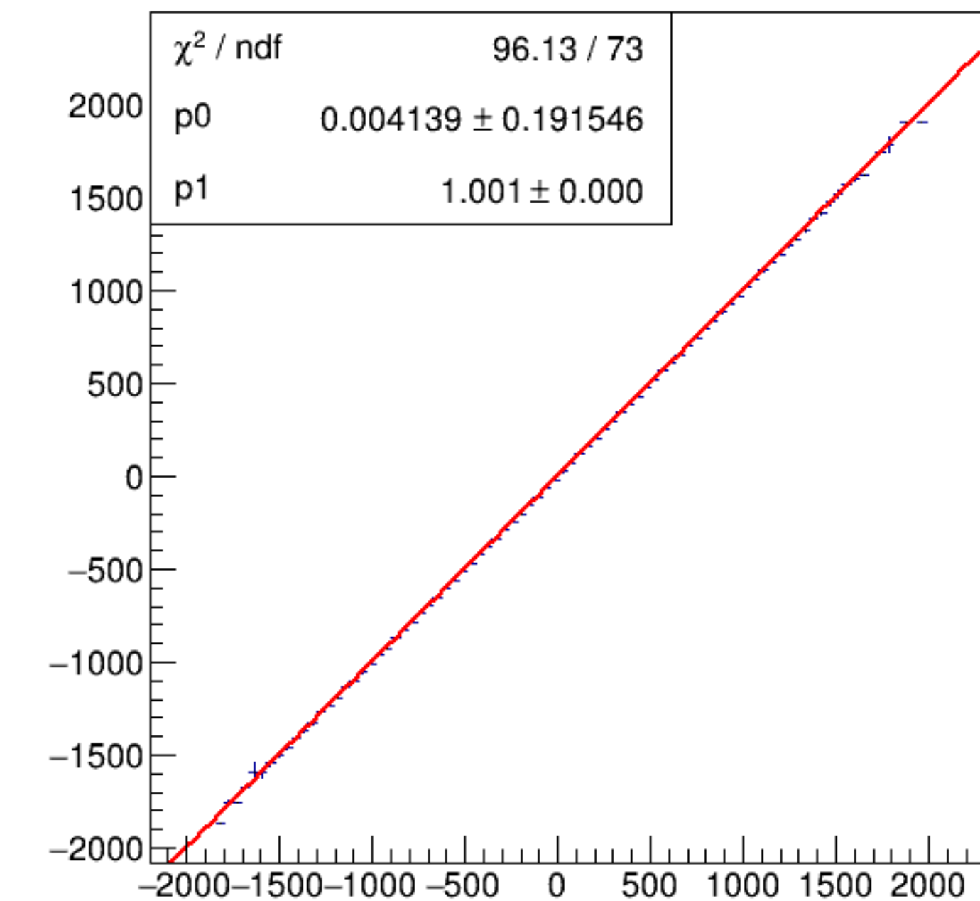
run6094_000_asym_bcm_dg_ds_vs_asym_bcm_an_us_pr.png
