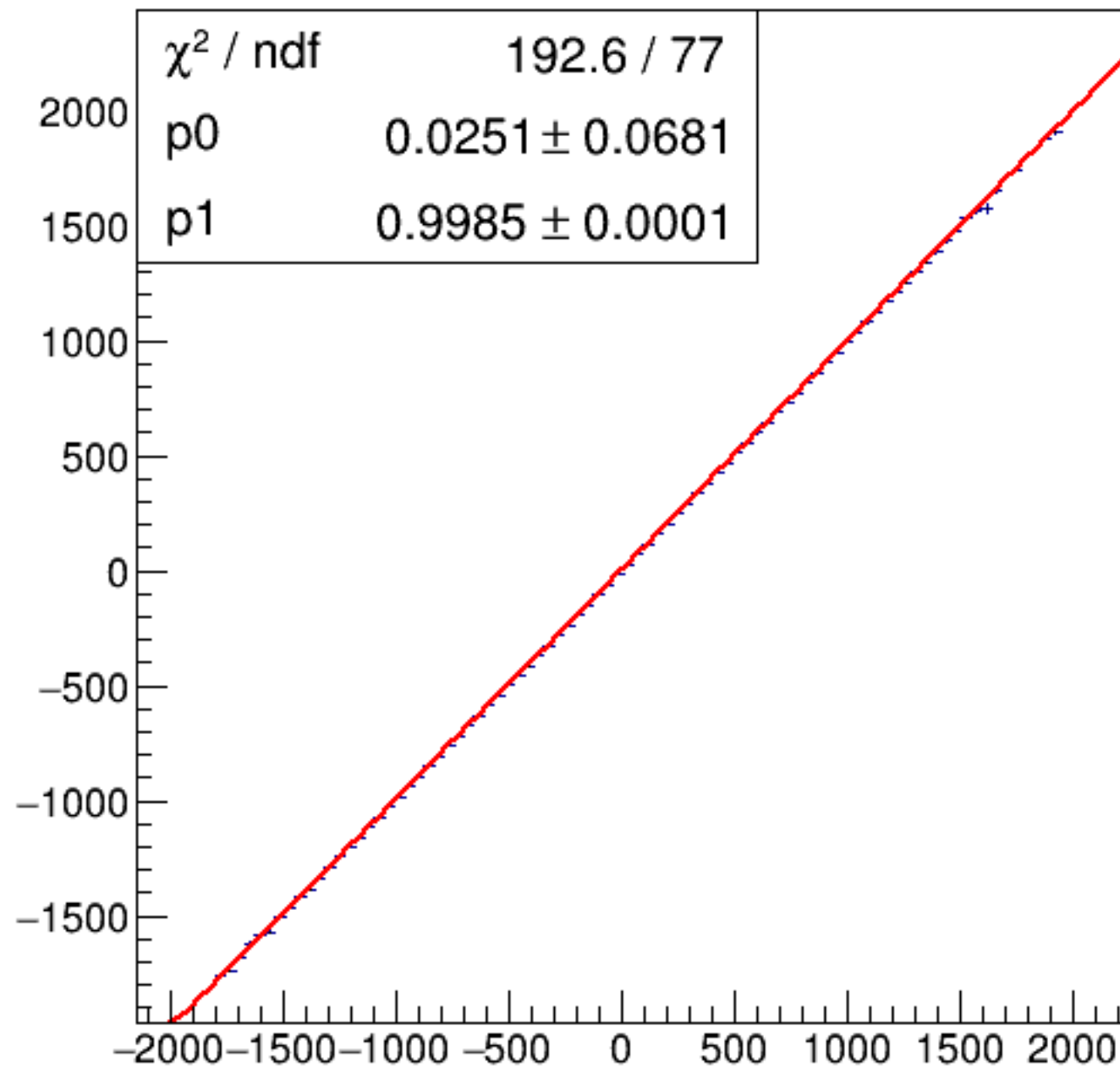
run6094_000_asym_bcm_an_ds_vs_asym_bcm_an_ds3_pr.png
