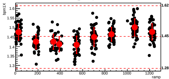
bmod_trim3,cyc=5420
