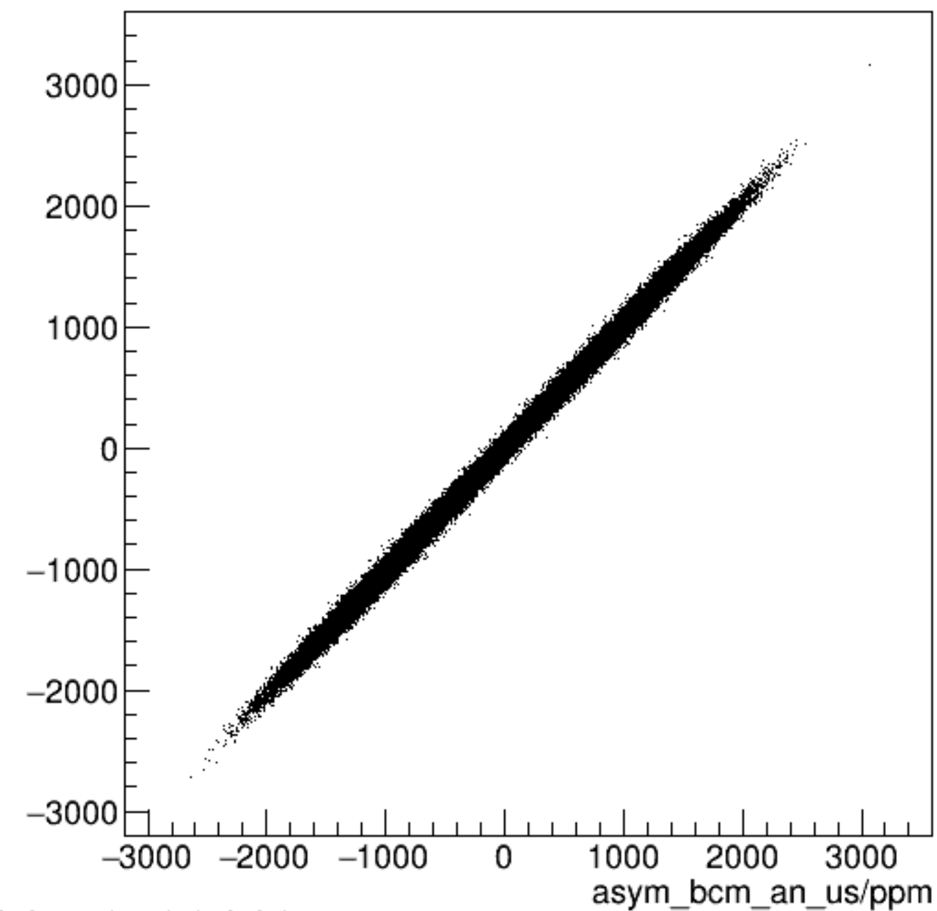
run6098_000_asym_bcm_dg_ds_vs_asym_bcm_an_us_pr.png
