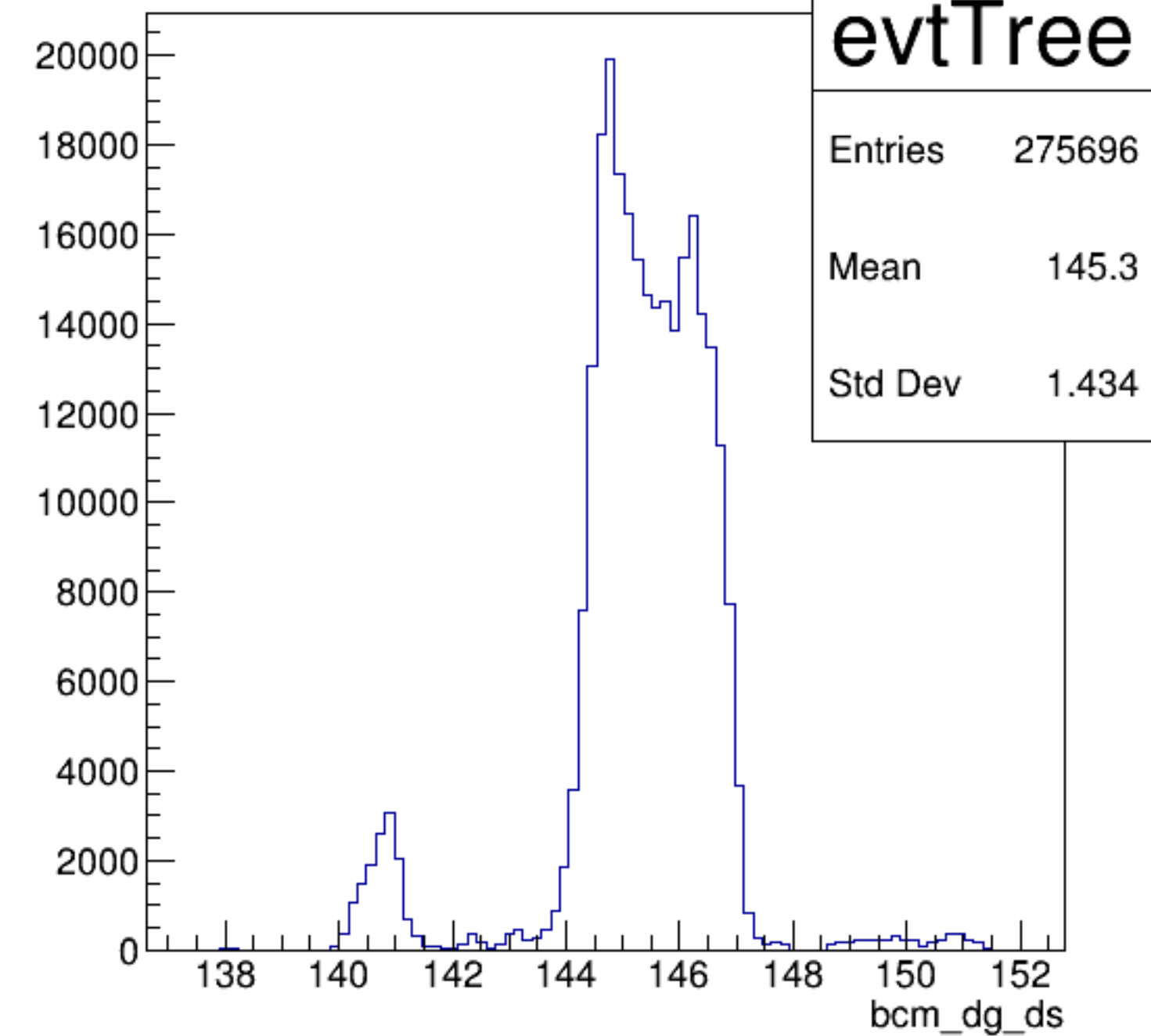
bcm_dg_ds {ErrorFlag==0}
