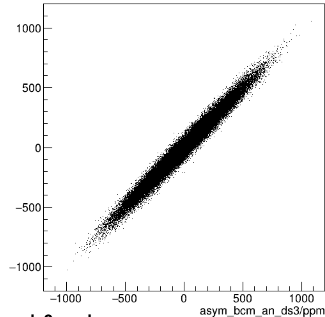
run6098_000_asym_bcm_dg_us_vs_asym_bcm_an_ds3_mul.png
