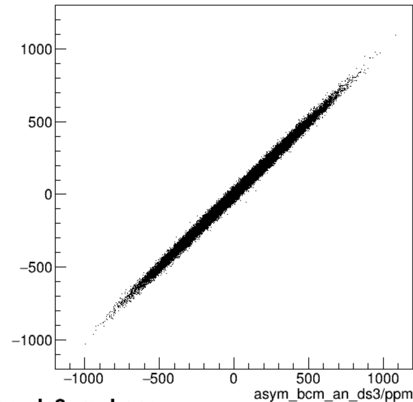
run6098_000_asym_bcm_an_us_vs_asym_bcm_an_ds3_mul.png
