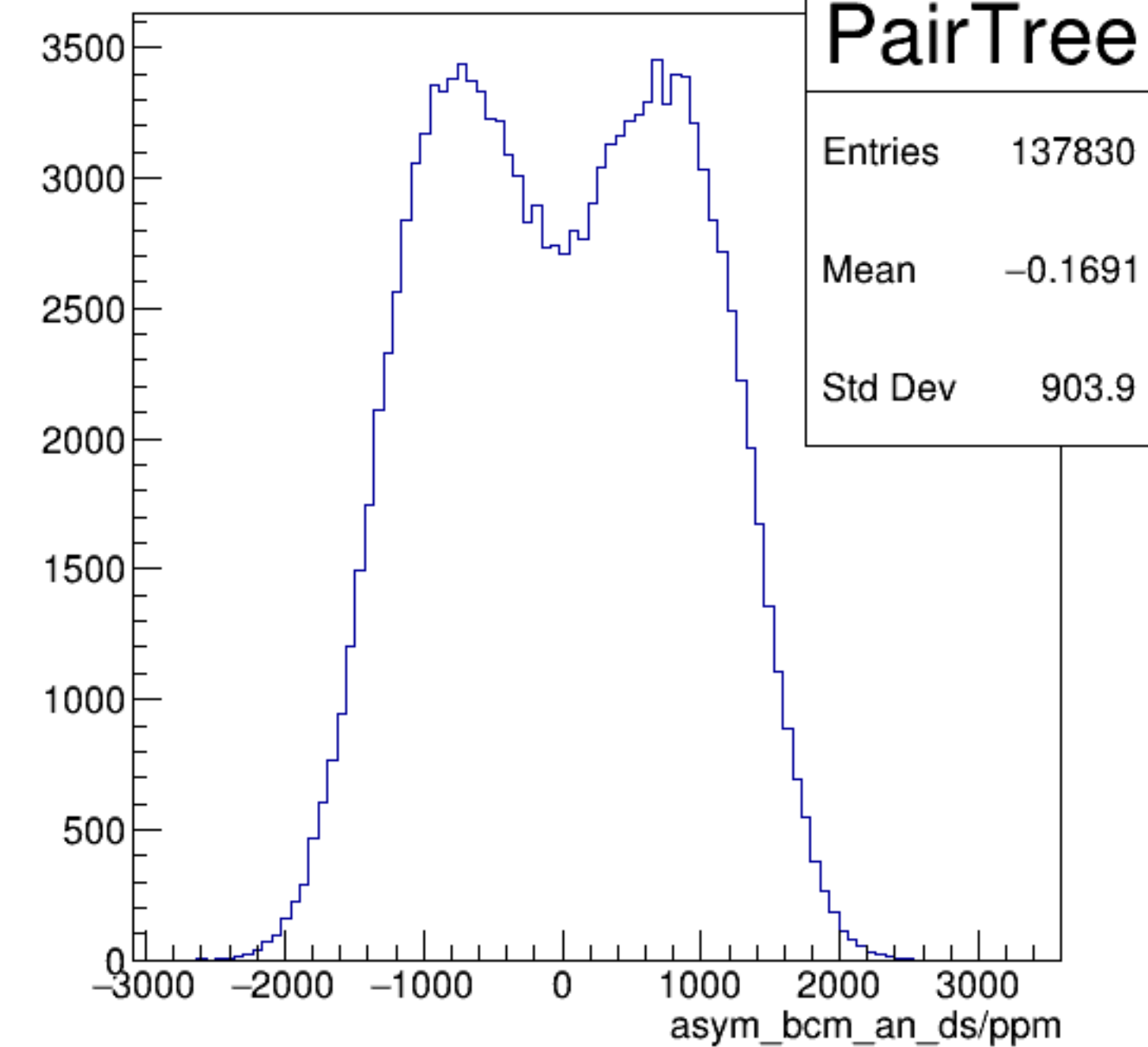
asym_bcm_an_ds/ppm {ErrorFlag==0}
