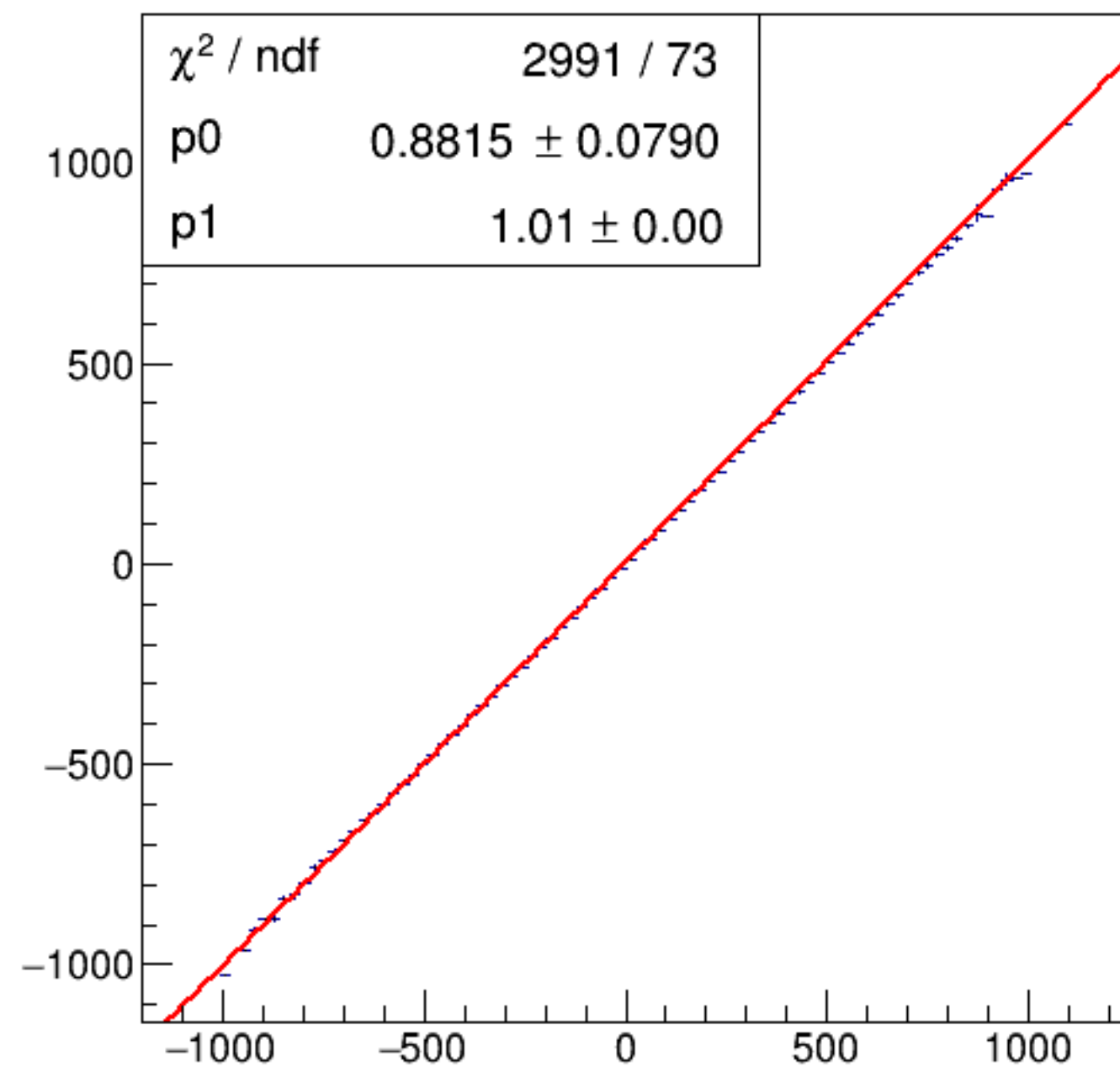
run6098_000_asym_bcm_an_us_vs_asym_bcm_an_ds3_mul.png
