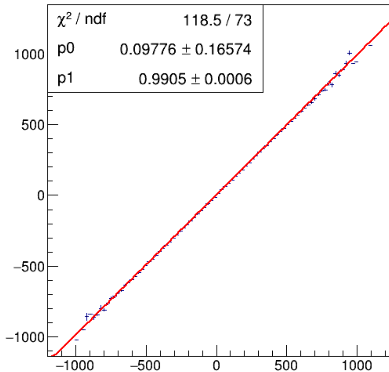
run6098_000_asym_bcm_dg_us_vs_asym_bcm_an_ds3_mul.png
