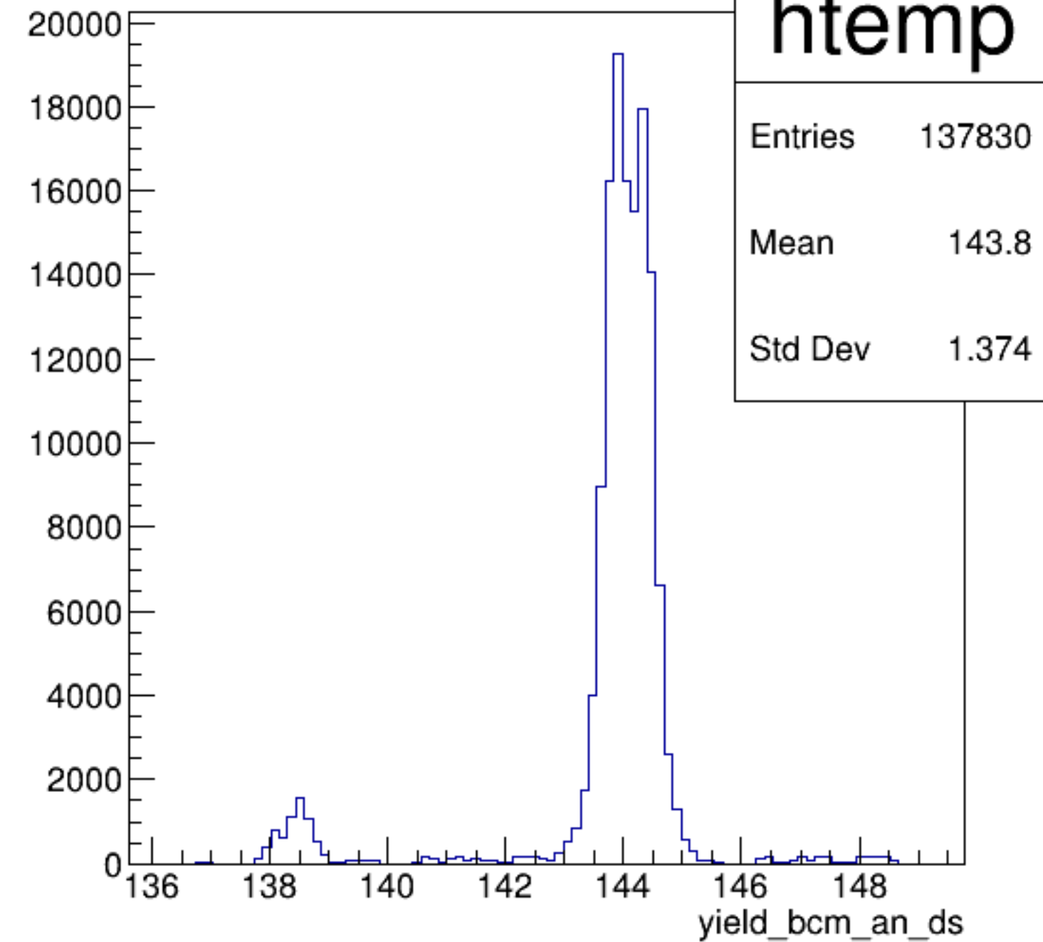
yield_bcm_an_ds {ErrorFlag==0}
