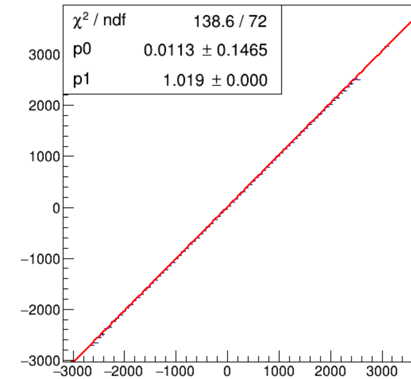
run6098_000_asym_bcm_dg_ds_vs_asym_bcm_an_us_pr.png
