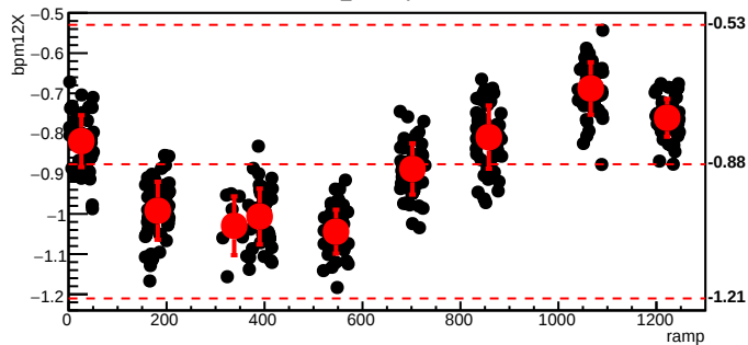
bmod_trim3,cyc=5422
