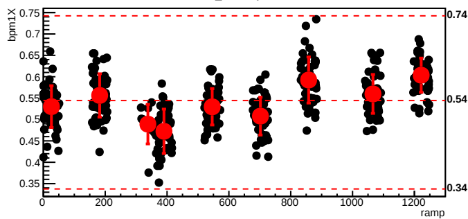
bmod_trim3,cyc=5422
