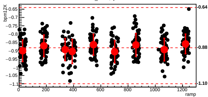
bmod_trim4,cyc=5422
