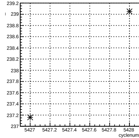
4eX_coil7:cyclenum {run == 6099}
