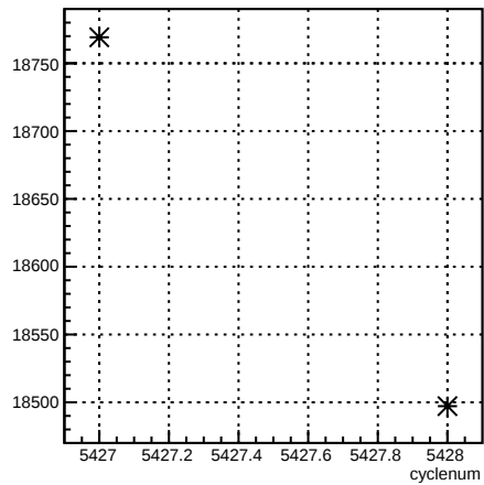
usl_coil6:cyclenum {run == 6099}
