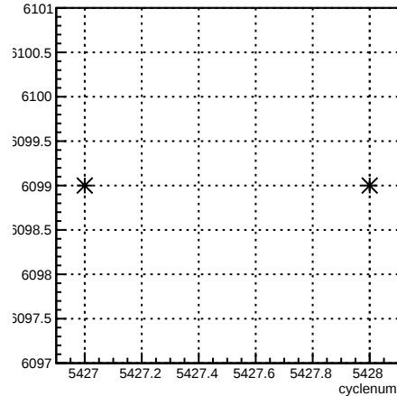
run:cyclenum {run == 6099}
