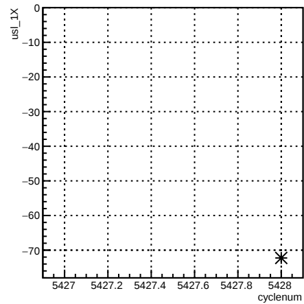
usl_1X:cyclenum {run == 6099}
