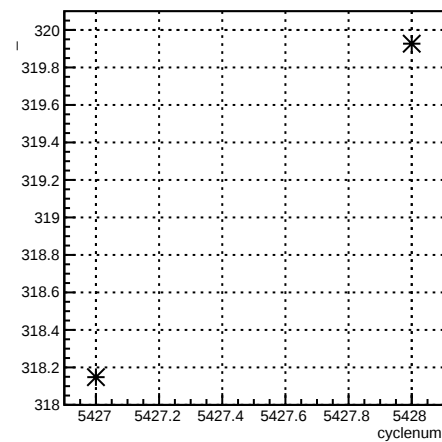
1X_coil7:cyclenum {run == 6099}
