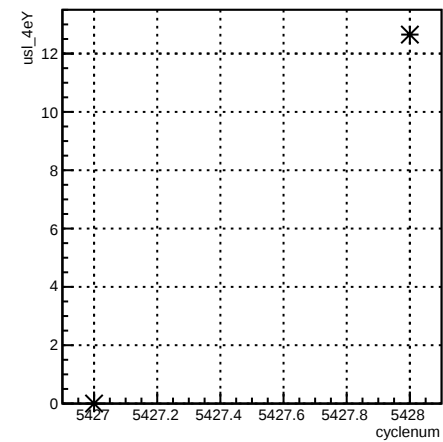
usl_4eY:cyclenum {run == 6099}
