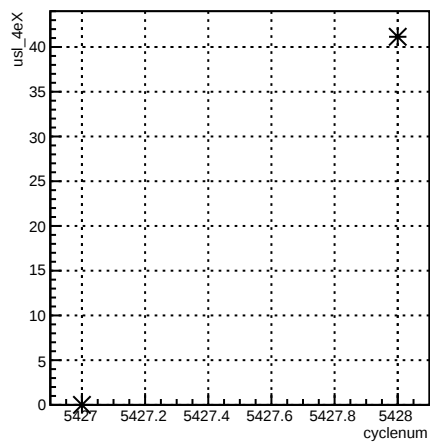
usl_4eX:cyclenum {run == 6099}
