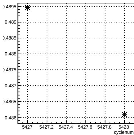
alpha13_4eX1X:cyclenum {run == 6099}
