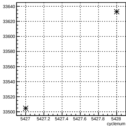
usr_coil7:cyclenum {run == 6099}
