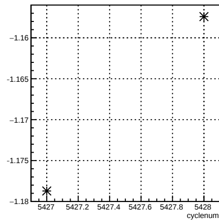
delta13_12X4eX:cyclenum {run == 6099}
