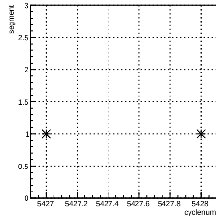
segment:cyclenum {run == 6099}
