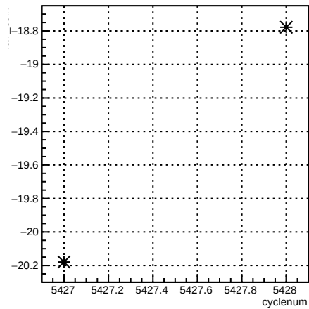
4eY_coil7:cyclenum {run == 6099}
