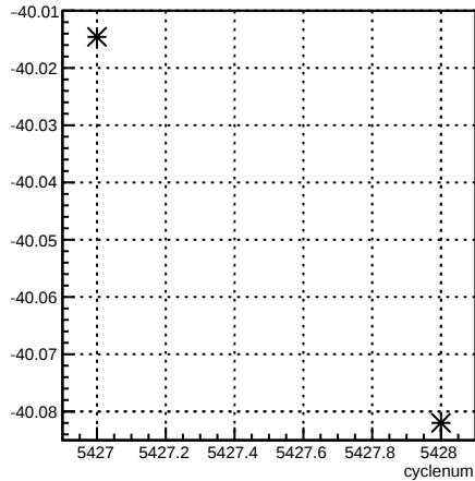
4eX_coil3:cyclenum {run == 6099}
