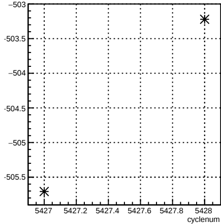
12X_coil7:cyclenum {run == 6099}
