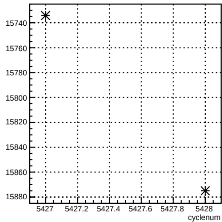
usr_coil6:cyclenum {run == 6099}
