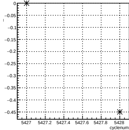
delta46_12X4eY:cyclenum {run == 6099}
