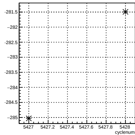
4eX_coil1:cyclenum {run == 6099}
