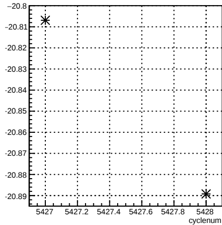
1X_coil3:cyclenum {run == 6099}
