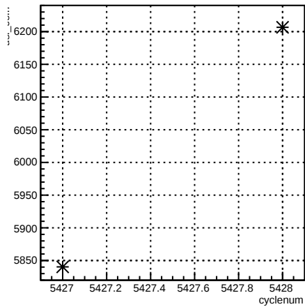
usl_coil7:cyclenum {run == 6099}
