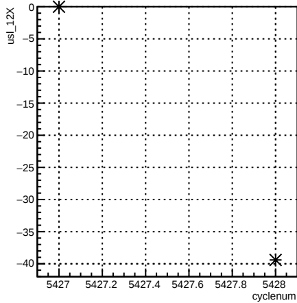
usl_12X:cyclenum {run == 6099}
