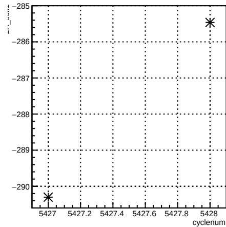
1X_coil1:cyclenum {run == 6099}
