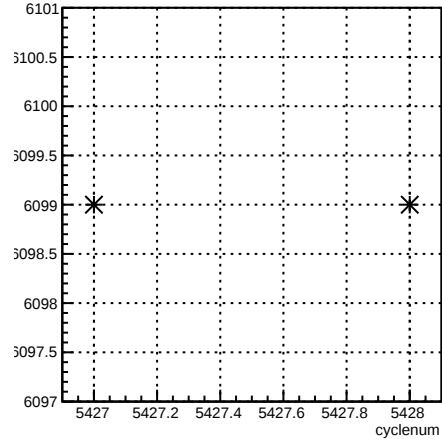
run:cyclenum {run == 6099}
