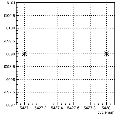
run:cyclenum {run == 6099}
