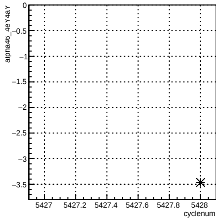
alpha46_4eY4aY:cyclenum {run == 6099}
