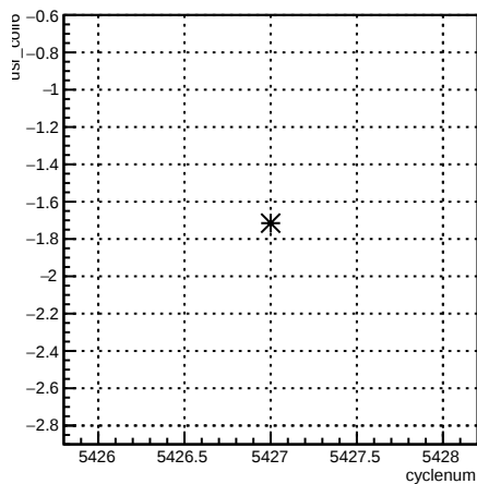
usr_coil6:cyclenum {run == 6099}
