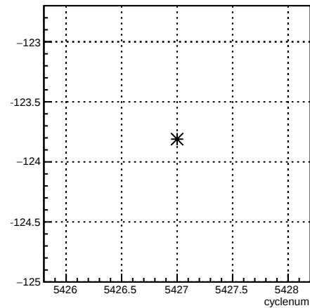
usr_4eY:cyclenum {run == 6099}
