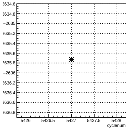
usr_coil3:cyclenum {run == 6099}
