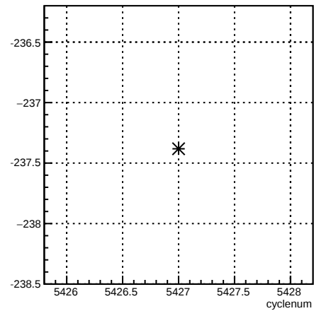
12X_coil6:cyclenum {run == 6099}
