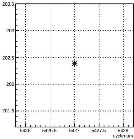
4aY_coil4:cyclenum {run == 6099}
