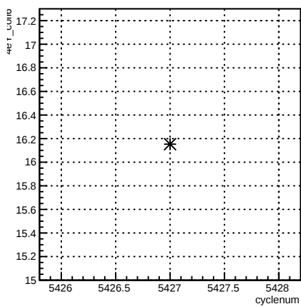
4eY_coil6:cyclenum {run == 6099}
