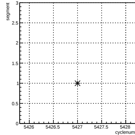
segment:cyclenum {run == 6099}
