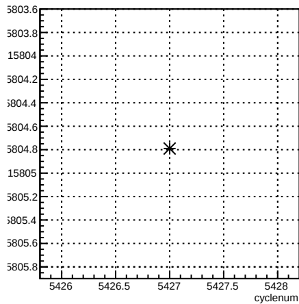
usr_coil1:cyclenum {run == 6099}
