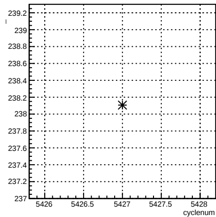
4eX_coil7:cyclenum {run == 6099}
