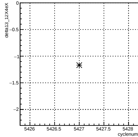
delta13_12X4eX:cyclenum {run == 6099}
