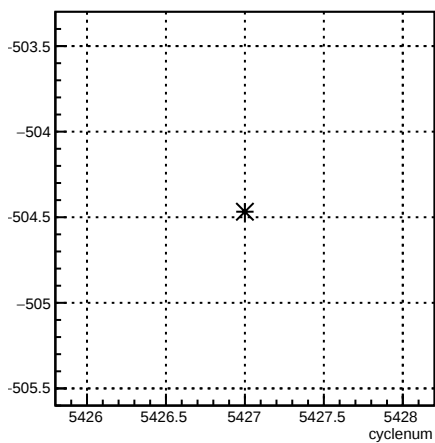
12X_coil7:cyclenum {run == 6099}
