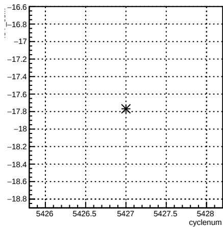
4eY_coil7:cyclenum {run == 6099}
