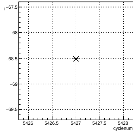
usl_4eY:cyclenum {run == 6099}
