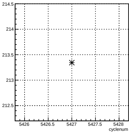
4eY_coil4:cyclenum {run == 6099}
