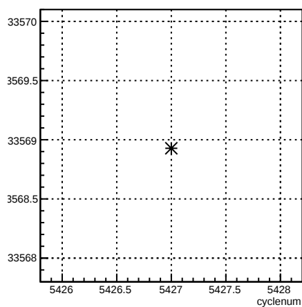
usr_coil7:cyclenum {run == 6099}
