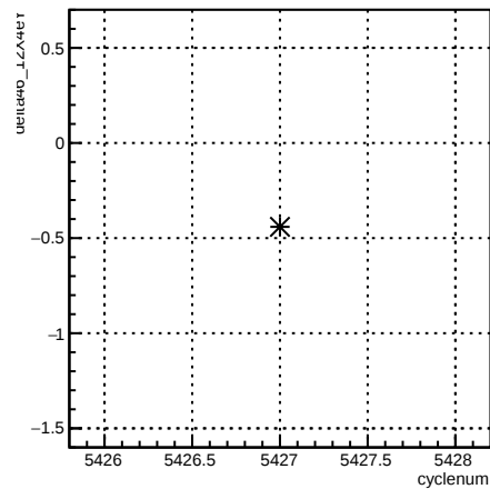
delta46_12X4eY:cyclenum {run == 6099}
