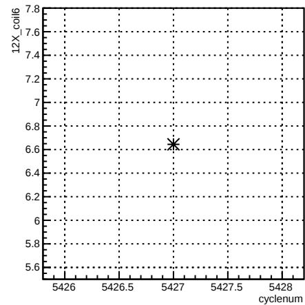
12X_coil6:cyclenum {run == 6099}
