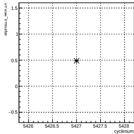
alpha13_4eX1X:cyclenum {run == 6099}
