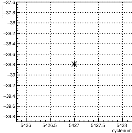
usl_12X:cyclenum {run == 6099}
