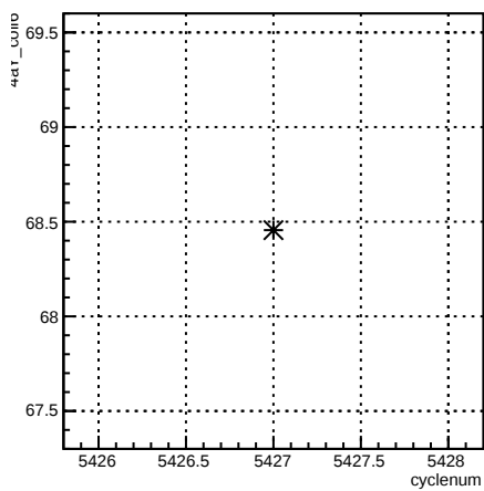
4aY_coil6:cyclenum {run == 6099}
