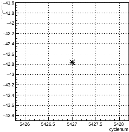
usr_12X:cyclenum {run == 6099}
