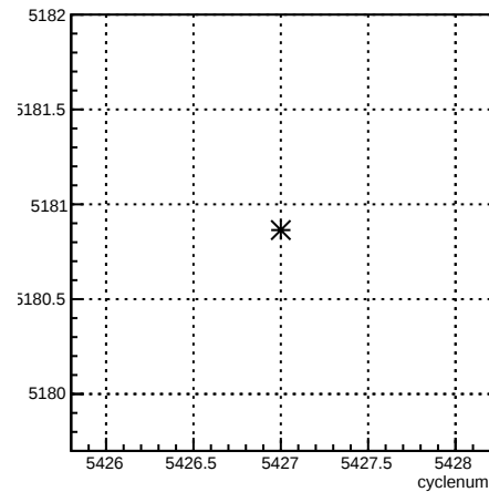
usr_coil4:cyclenum {run == 6099}
