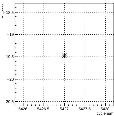
4aY_coil7:cyclenum {run == 6099}
