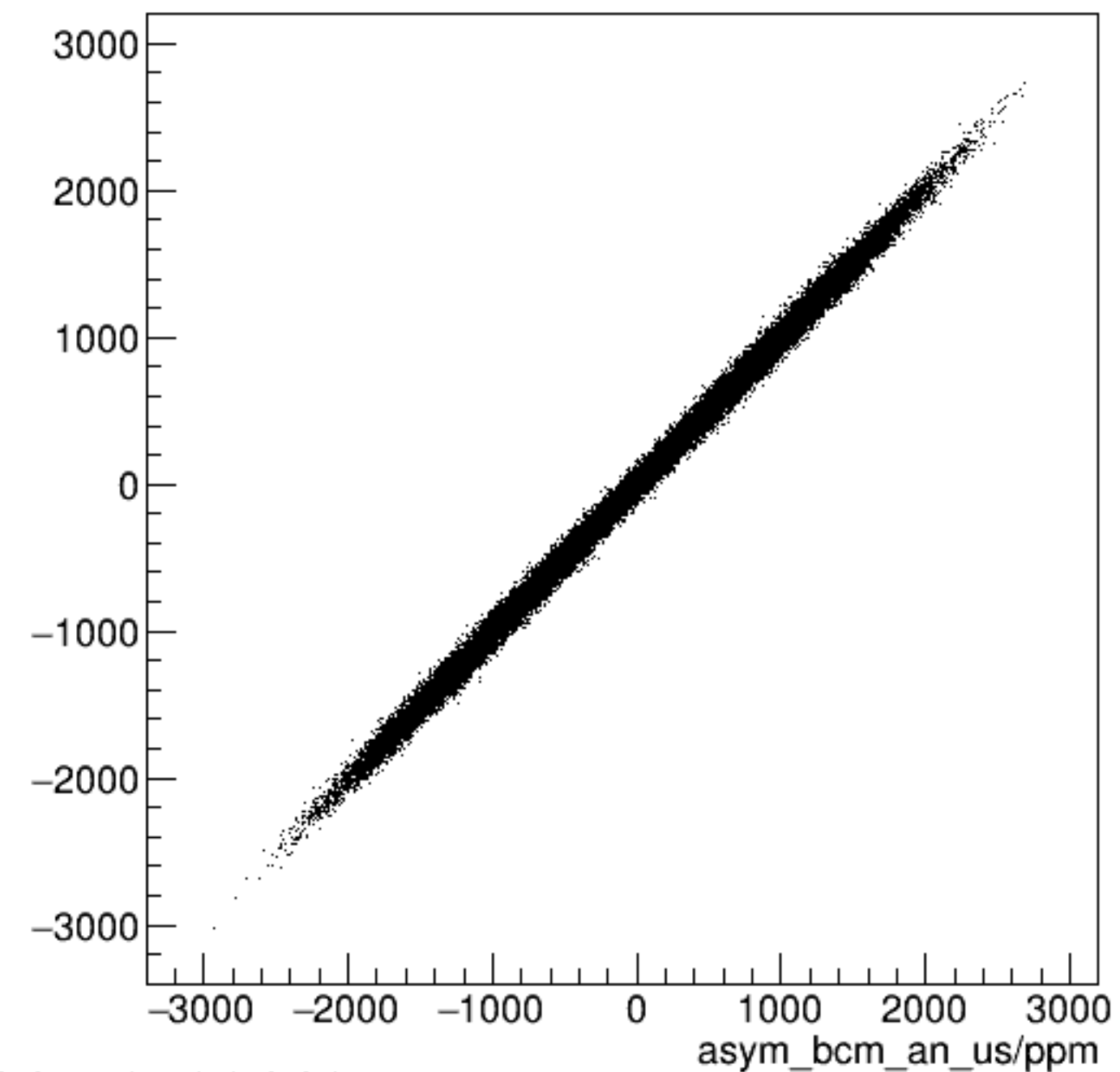
run6099_000_asym_bcm_dg_ds_vs_asym_bcm_an_us_pr.png
