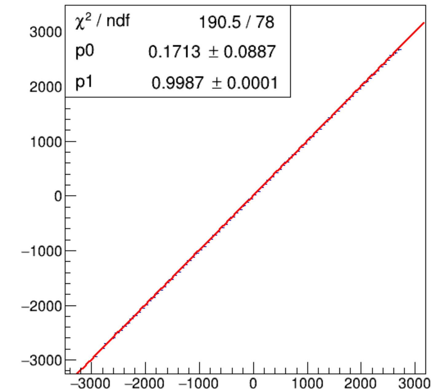
run6099_000_asym_bcm_an_ds_vs_asym_bcm_an_ds3_pr.png
