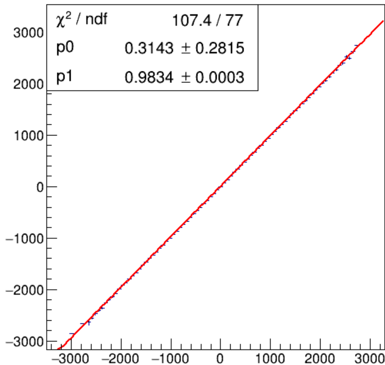
run6099_000_asym_bcm_dg_us_vs_asym_bcm_dg_ds_pr.png
