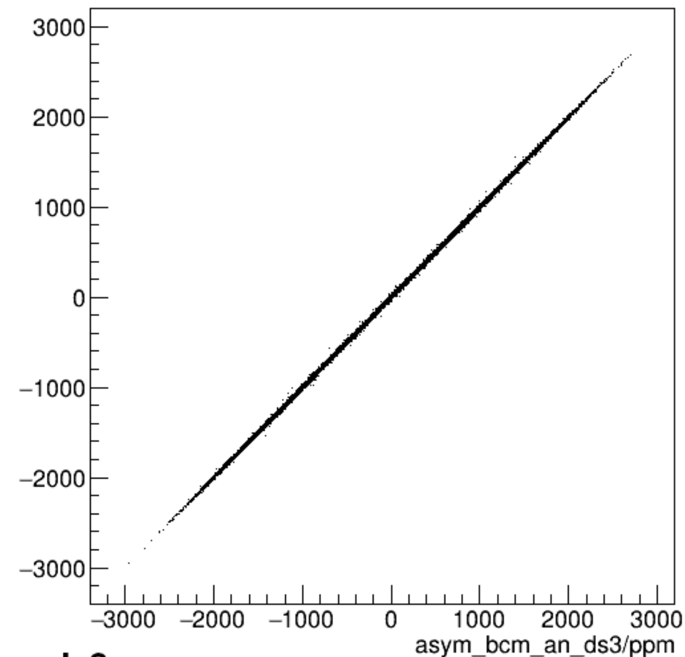
run6099_000_asym_bcm_an_ds_vs_asym_bcm_an_ds3_pr.png
