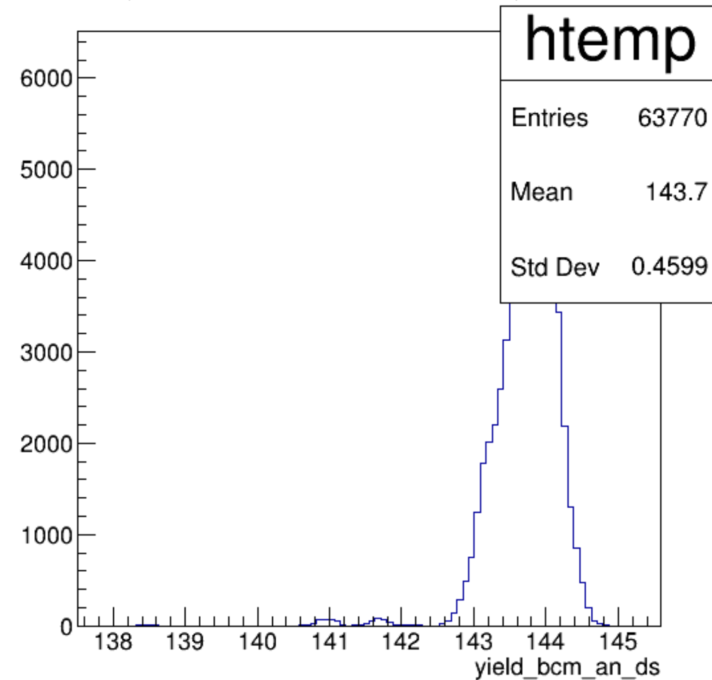
yield_bcm_an_ds {ErrorFlag==0}
