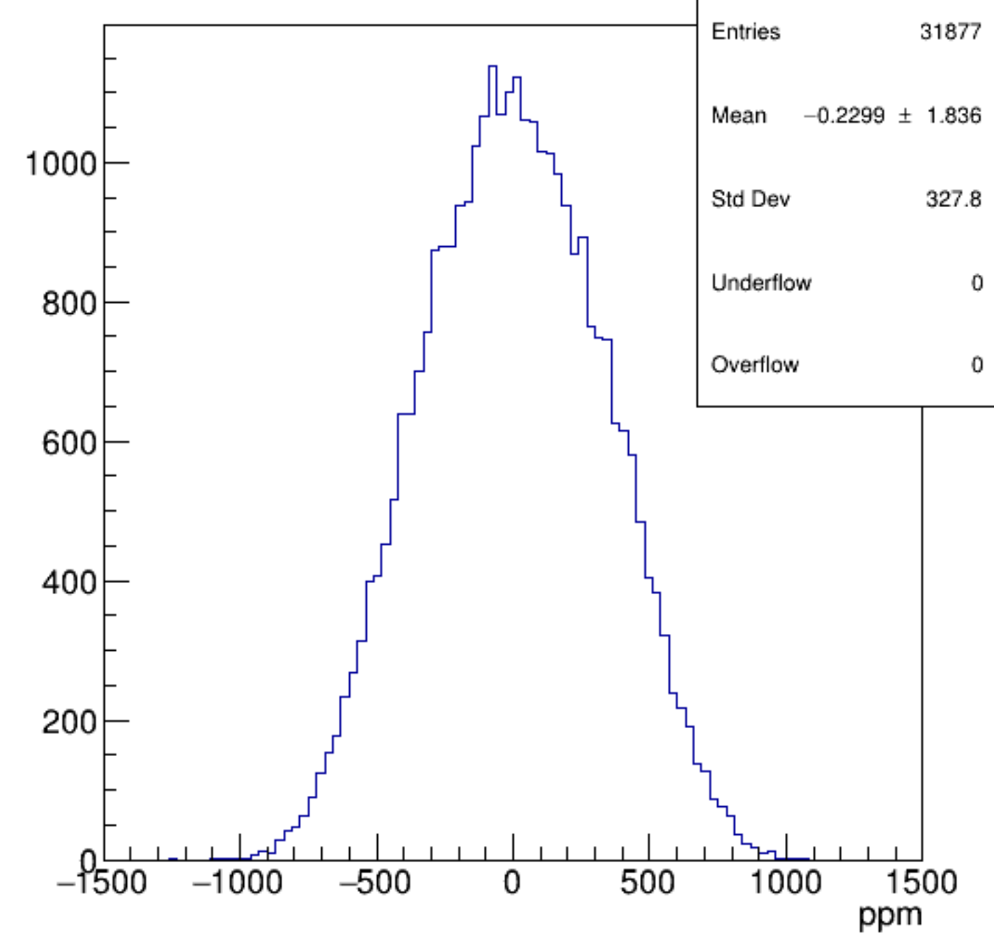
asym_bcm_dg_ds
