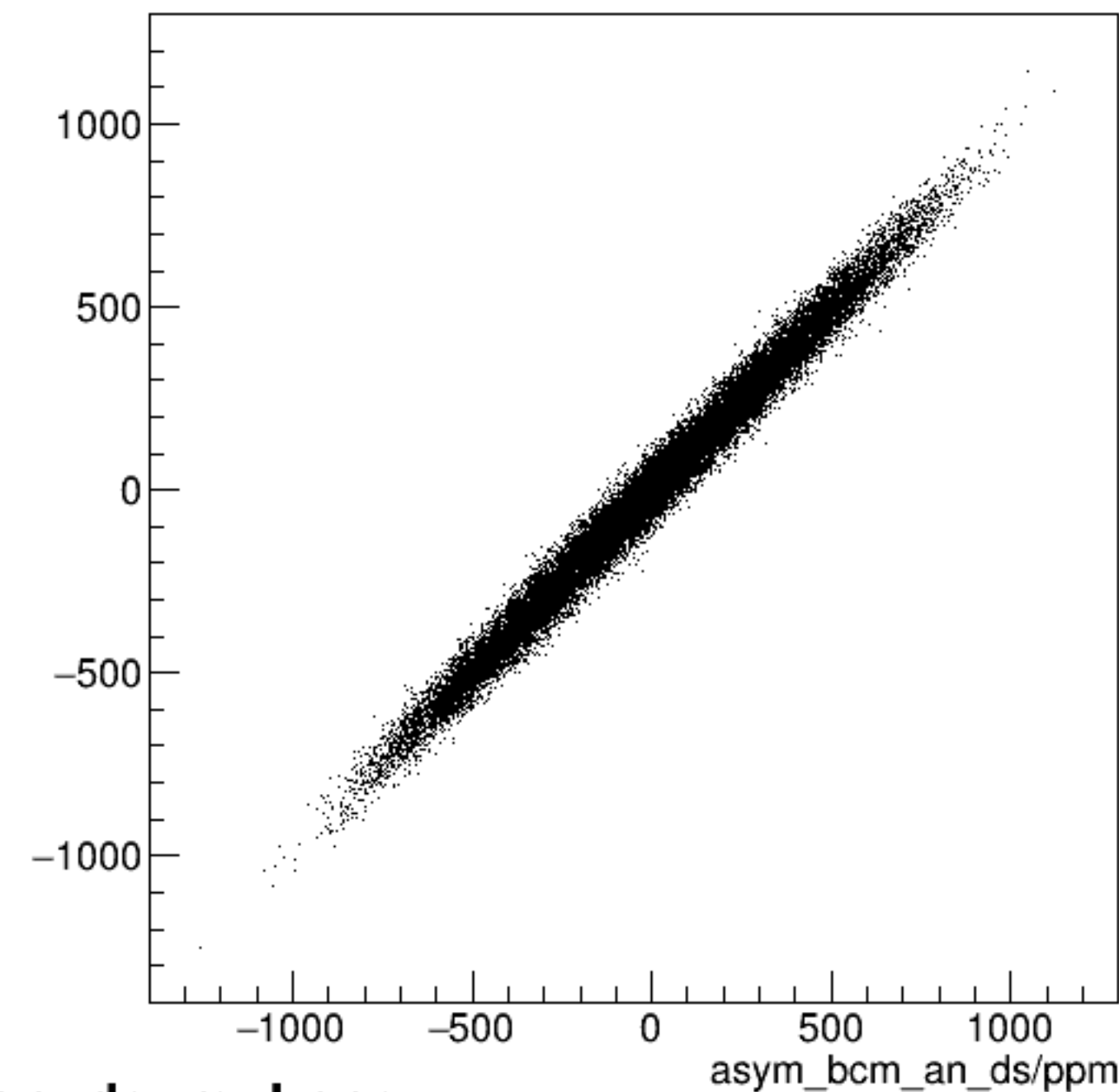
run6099_000_asym_bcm_dg_us_vs_asym_bcm_an_ds_mul.png
