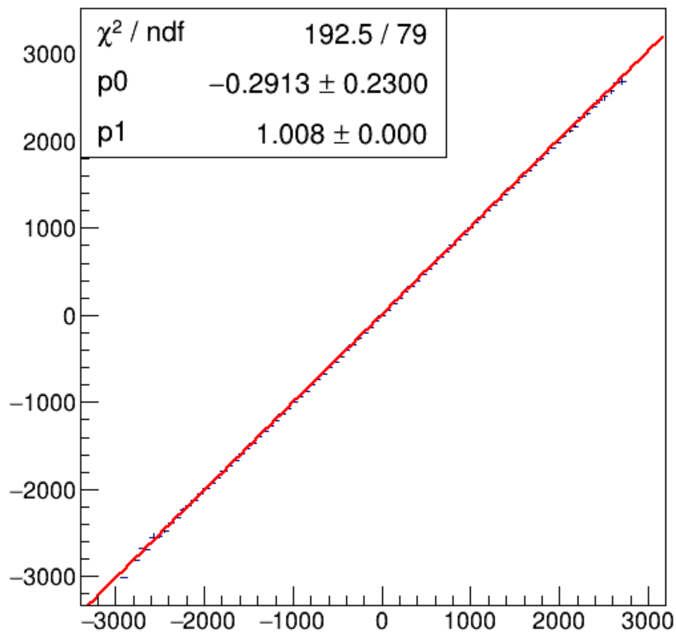
run6099_000_asym_bcm_dg_ds_vs_asym_bcm_an_us_pr.png
