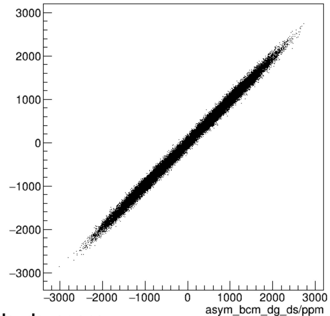
run6099_000_asym_bcm_dg_us_vs_asym_bcm_dg_ds_pr.png
