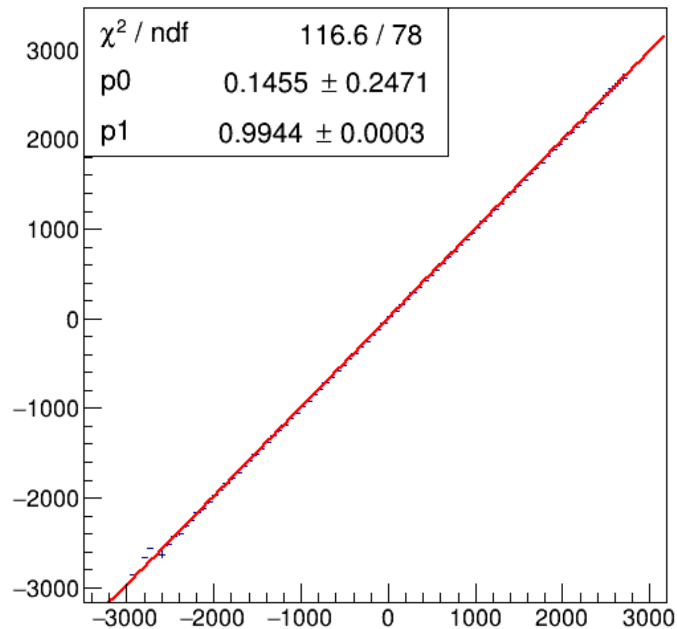
run6099_000_asym_bcm_dg_us_vs_asym_bcm_an_ds3_pr.png
