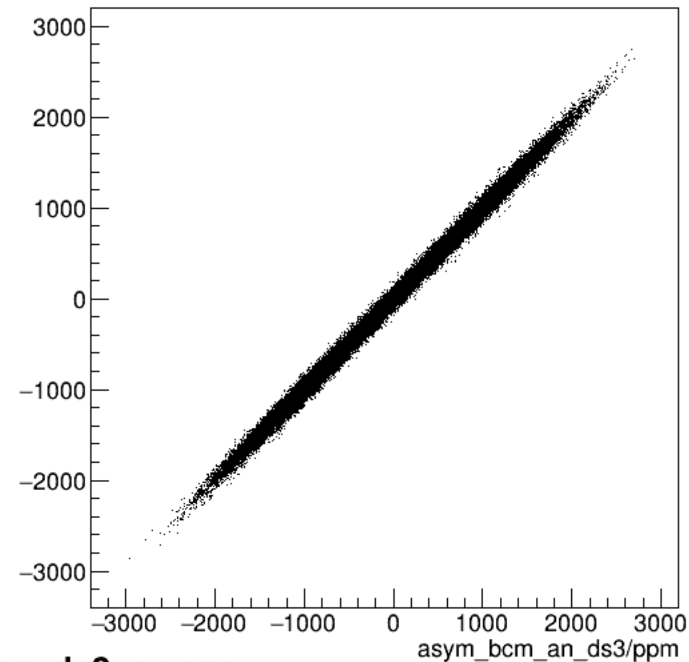
run6099_000_asym_bcm_dg_us_vs_asym_bcm_an_ds3_pr.png
