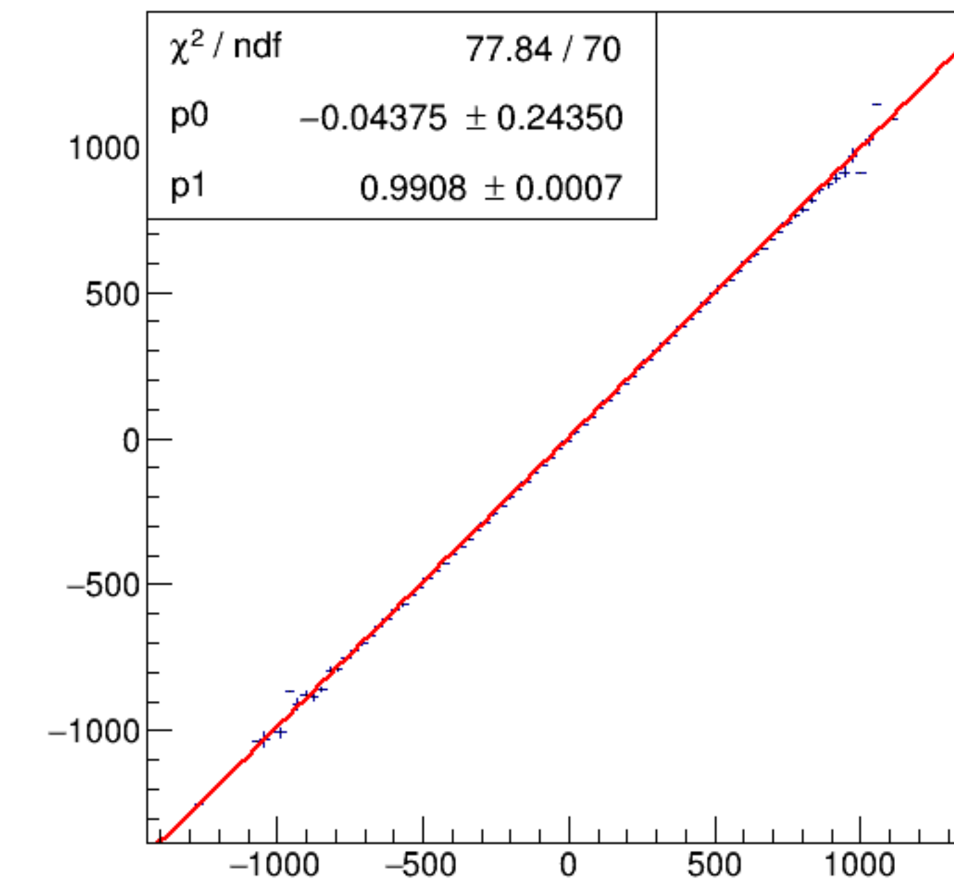
run6099_000_asym_bcm_dg_us_vs_asym_bcm_an_ds_mul.png
