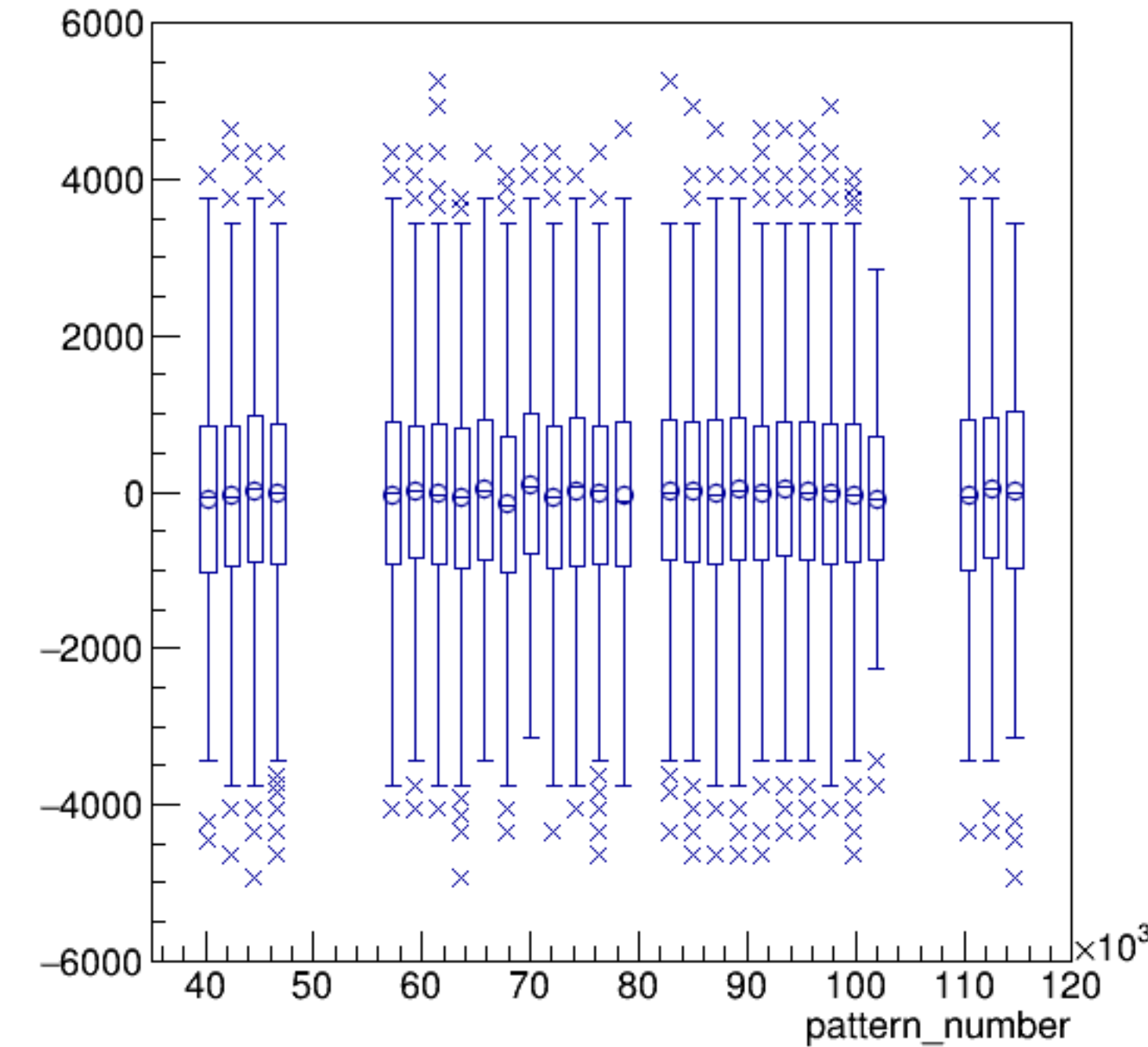
asym_usl/ppm:pattern_number {ErrorFlag==0}
