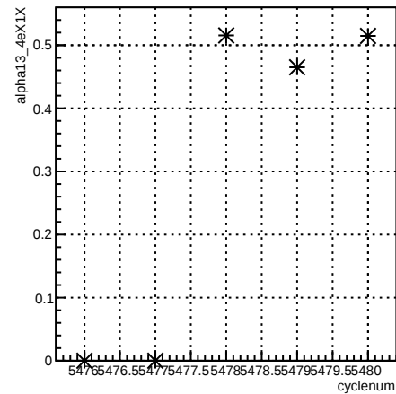
alpha13_4eX1X:cyclenum {run == 6103}
