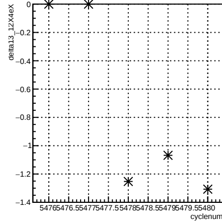
delta13_12X4eX:cyclenum {run == 6103}
