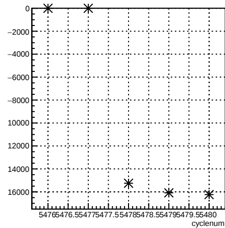
usr_coil1:cyclenum {run == 6103}
