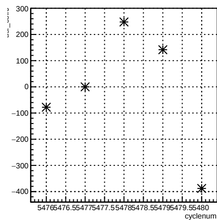
usr_coil6:cyclenum {run == 6103}
