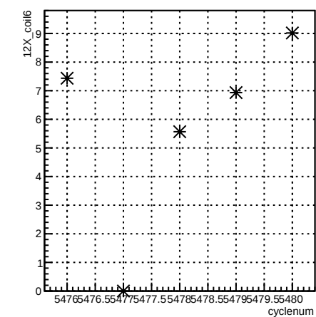
12X_coil6:cyclenum {run == 6103}
