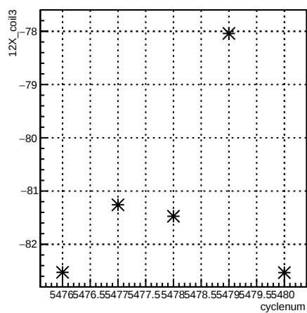
12X_coil3:cyclenum {run == 6103}
