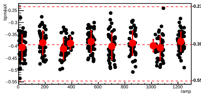
bmod_trim6,cyc=5476
