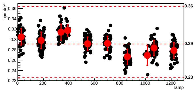
bmod_trim6,cyc=5476
