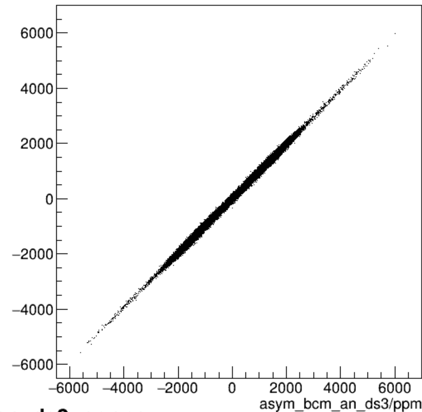
run6104_000_asym_bcm_dg_us_vs_asym_bcm_an_ds3_pr.png
