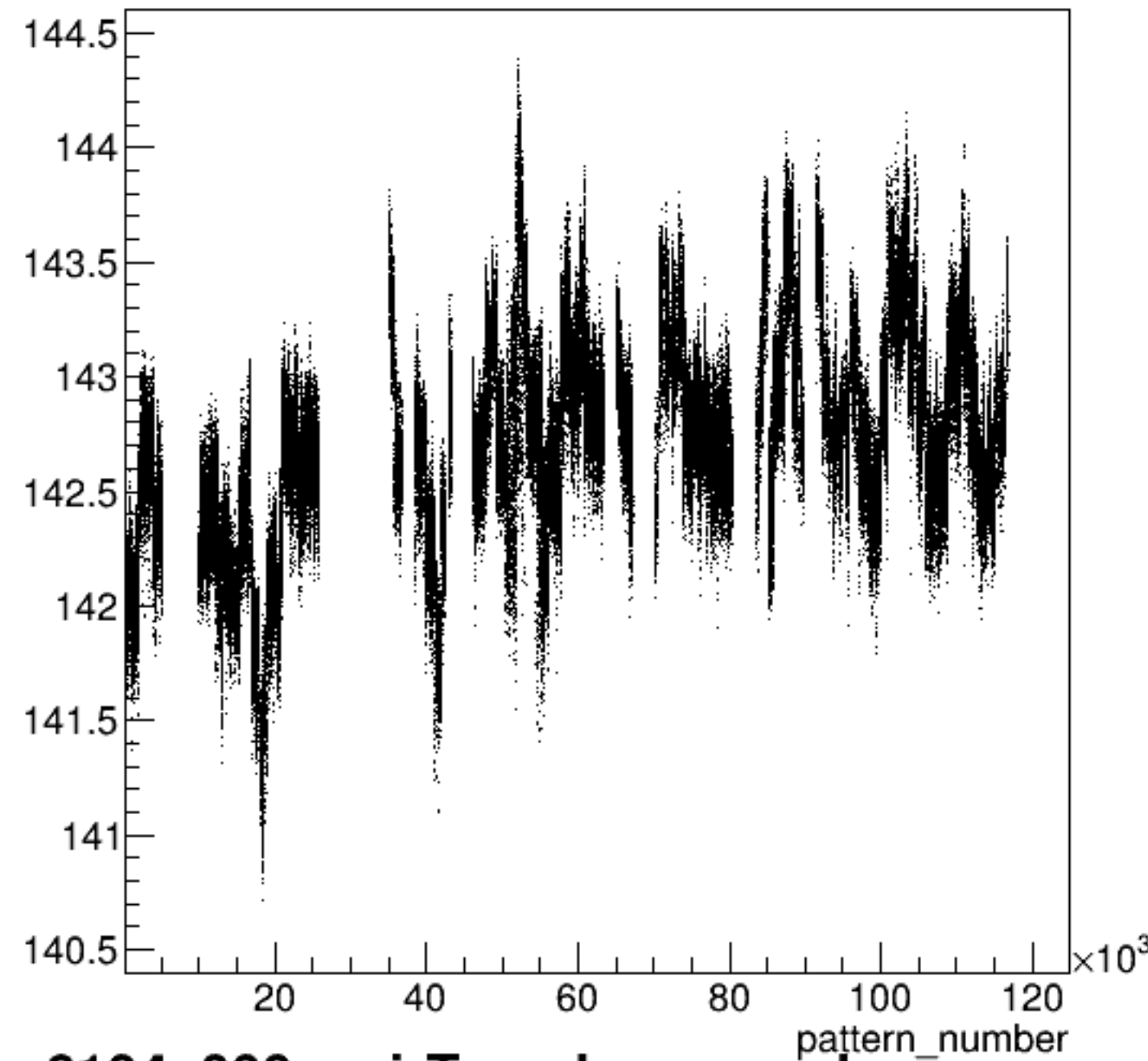
yield_bcm_an_ds:pattern_number {ErrorFlag==0}
