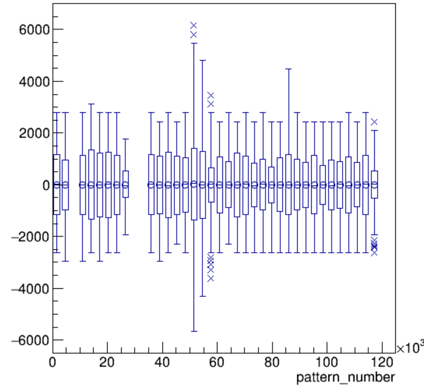
asym_bcm_an_ds/ppm:pattern_number {ErrorFlag==0}
