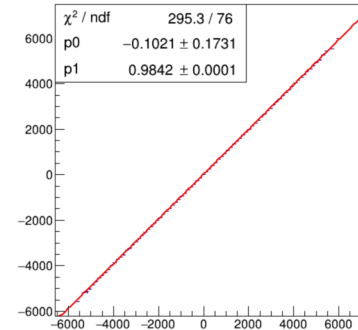
run6104_000_asym_bcm_dg_us_vs_asym_bcm_an_ds3_pr.png
