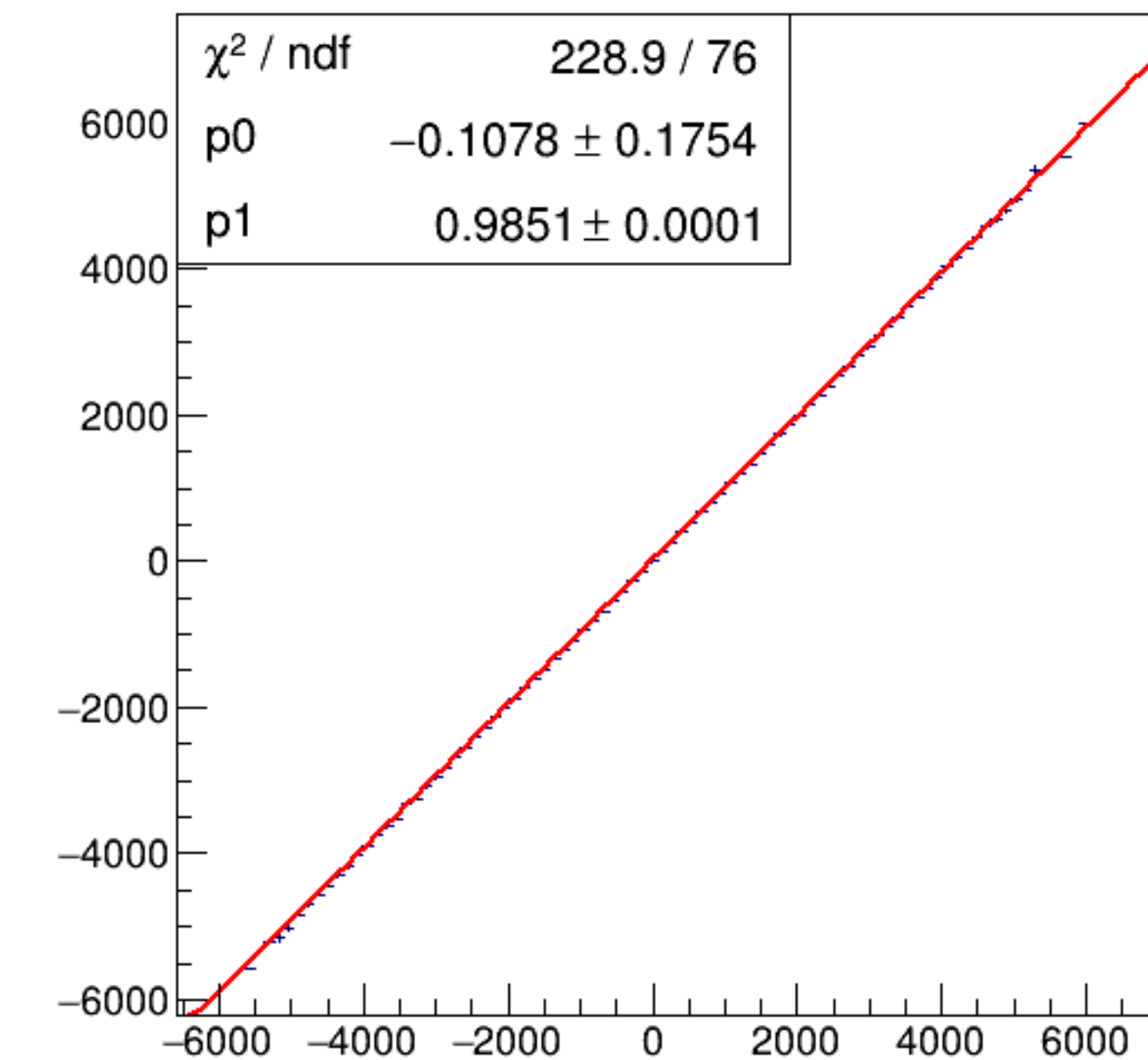
run6104_000_asym_bcm_dg_us_vs_asym_bcm_an_ds_pr.png
