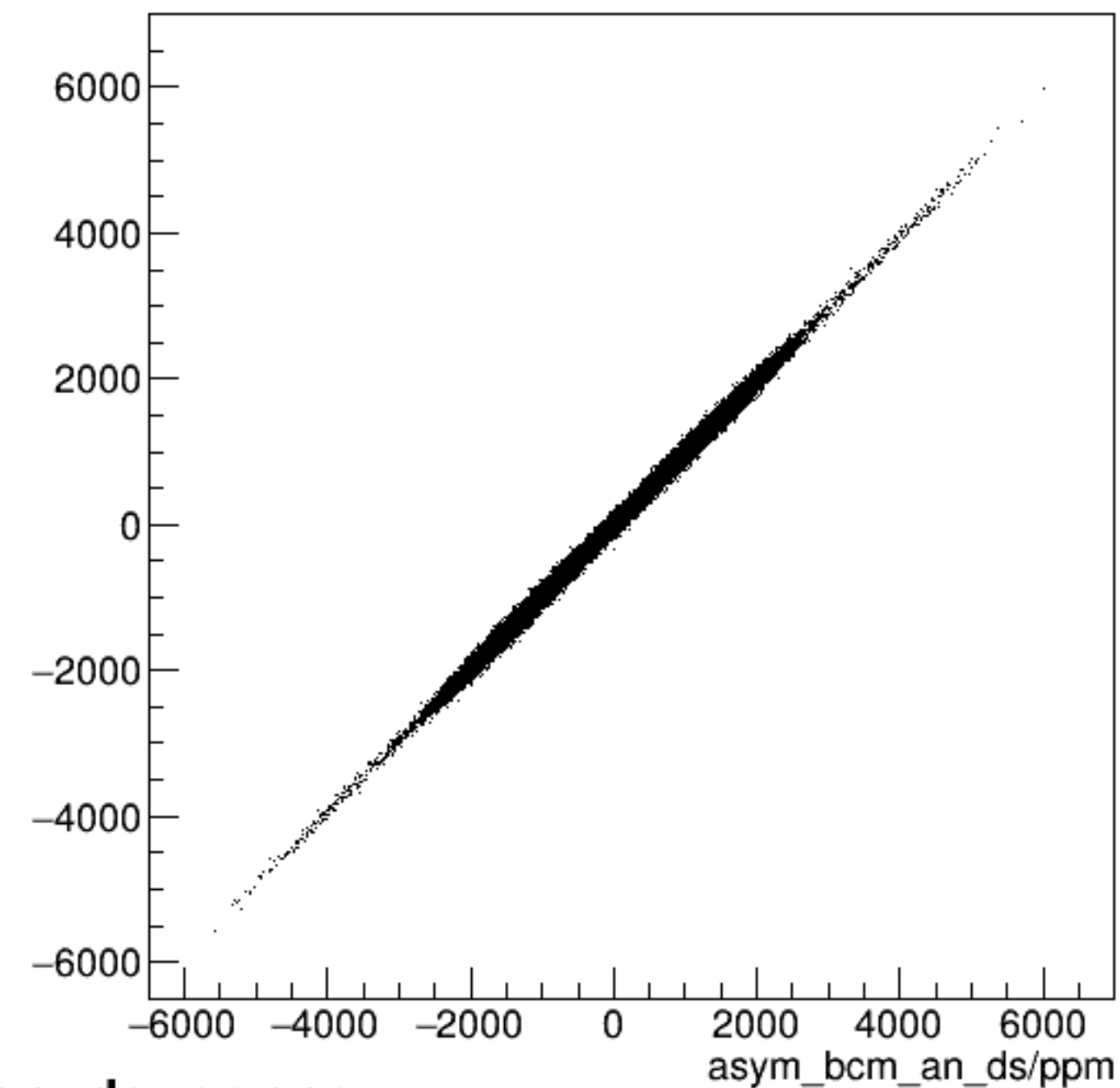
run6104_000_asym_bcm_dg_us_vs_asym_bcm_an_ds_pr.png
