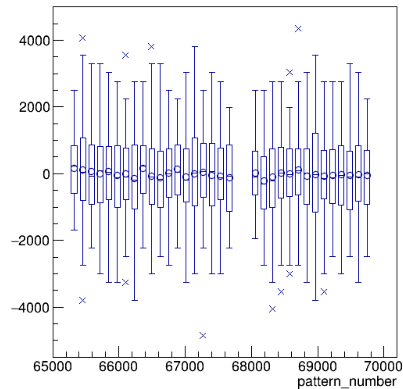
asym_sam5/ppm:pattern_number {ErrorFlag==0}
