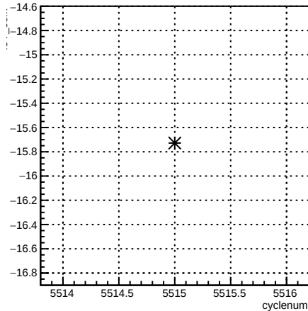
4eY_coil7:cyclenum {run == 6116}
