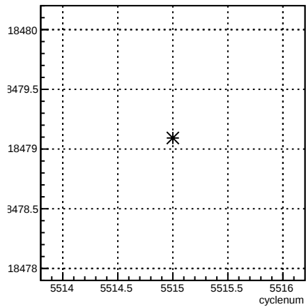
usl_coil6:cyclenum {run == 6116}
