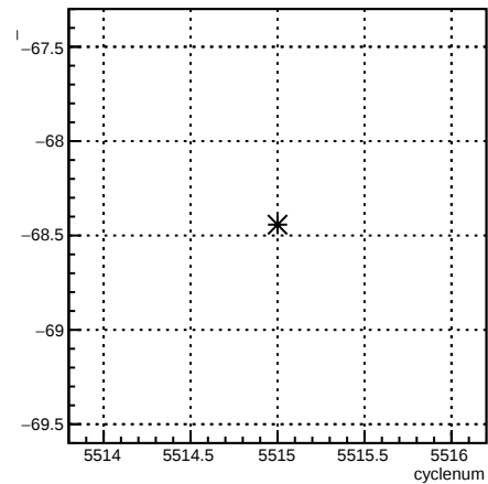
usl_4eY:cyclenum {run == 6116}
