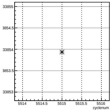
usr_coil7:cyclenum {run == 6116}
