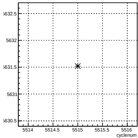
usl_coil7:cyclenum {run == 6116}
