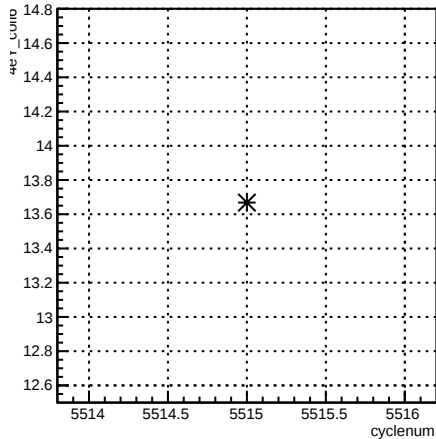
4eY_coil6:cyclenum {run == 6116}
