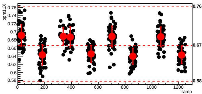
bmod_trim4,cyc=5518
