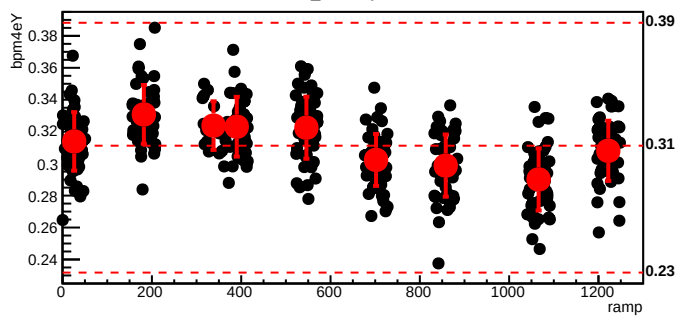
bmod_trim6,cyc=5518
