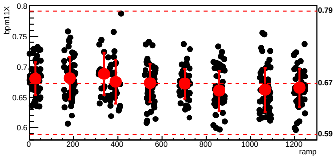
bmod_trim6,cyc=5518
