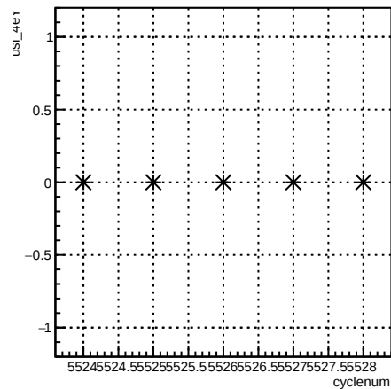
usl_4eY:cyclenum {run == 6118}
