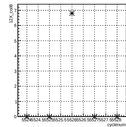
12X_coil6:cyclenum {run == 6118}
