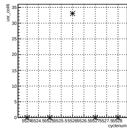
usr_coil6:cyclenum {run == 6118}
