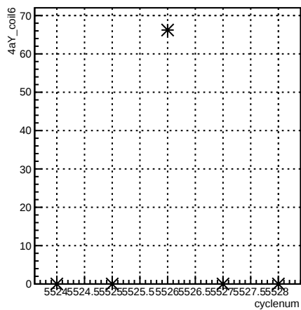
4aY_coil6:cyclenum {run == 6118}
