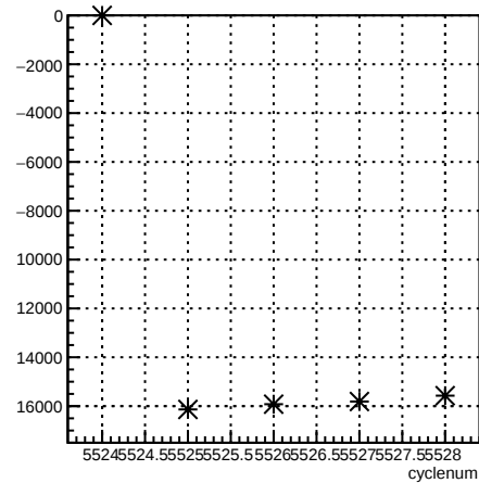
usr_coil1:cyclenum {run == 6118}
