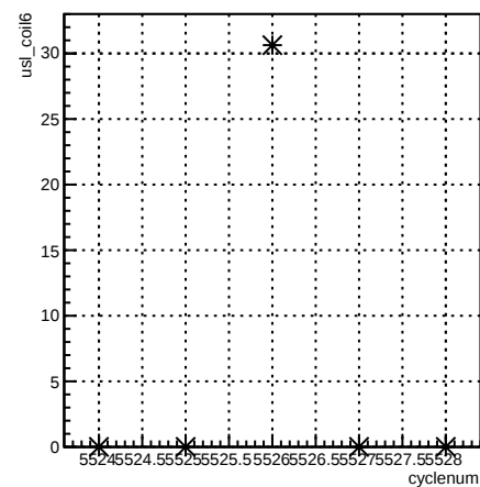
usl_coil6:cyclenum {run == 6118}
