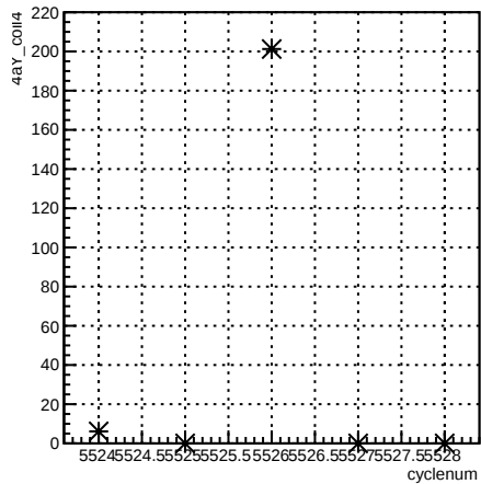
4aY_coil4:cyclenum {run == 6118}
