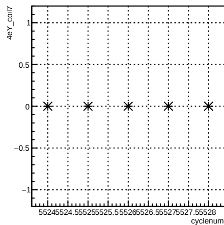
4eY_coil7:cyclenum {run == 6118}
