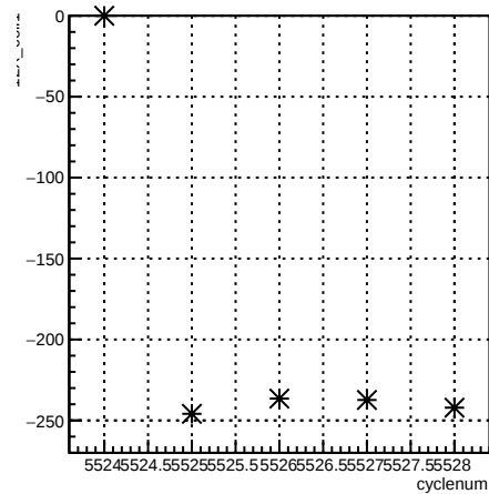
12X_coil1:cyclenum {run == 6118}
