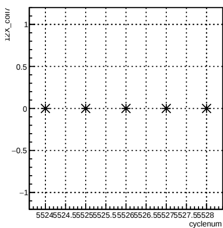
12X_coil7:cyclenum {run == 6118}
