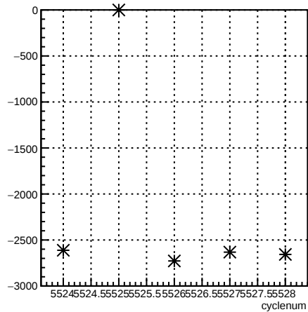
usr_coil3:cyclenum {run == 6118}
