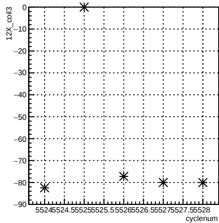
12X_coil3:cyclenum {run == 6118}
