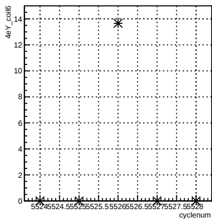
4eY_coil6:cyclenum {run == 6118}
