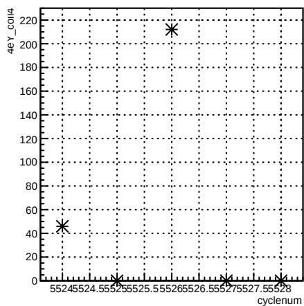
4eY_coil4:cyclenum {run == 6118}
