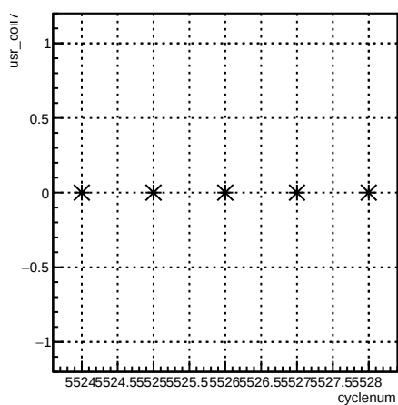
usr_coil7:cyclenum {run == 6118}
