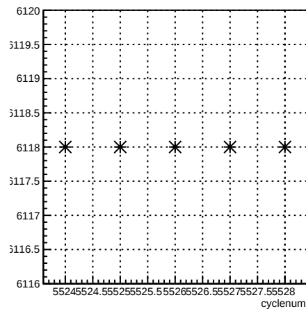
run:cyclenum {run == 6118}
