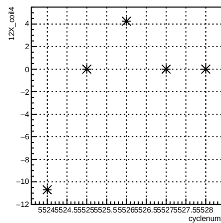
12X_coil4:cyclenum {run == 6118}
