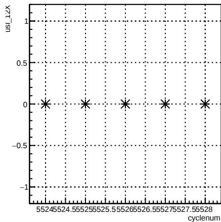
usl_12X:cyclenum {run == 6118}
