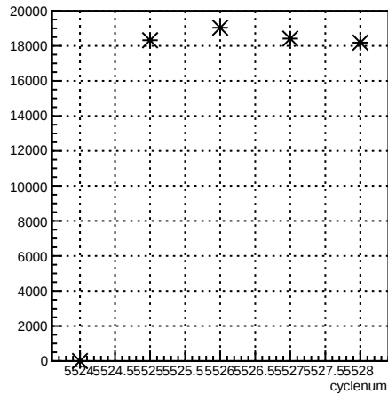
usl_coil1:cyclenum {run == 6118}
