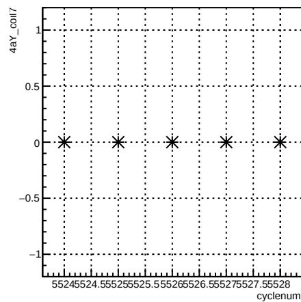
4aY_coil7:cyclenum {run == 6118}
