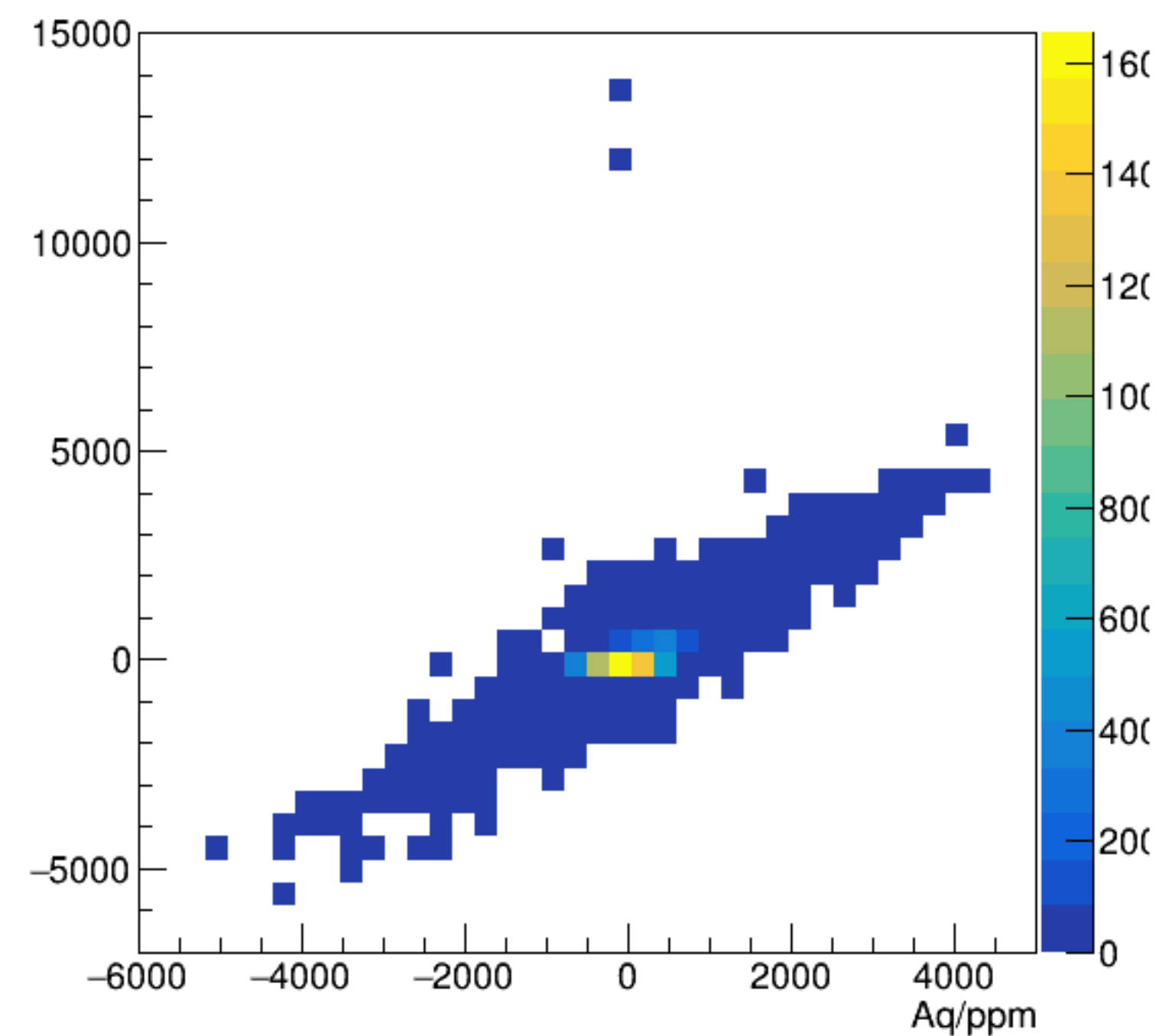
asym_bpm0i02WS/ppm:Aq/ppm {ErrorFlag==0}
