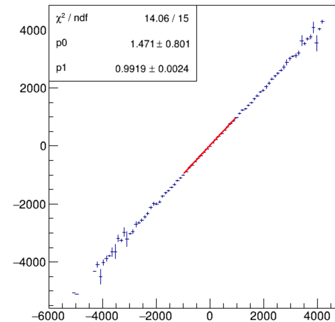
asym_bpm1WS/ppm:Aq/ppm {ErrorFlag==0}
