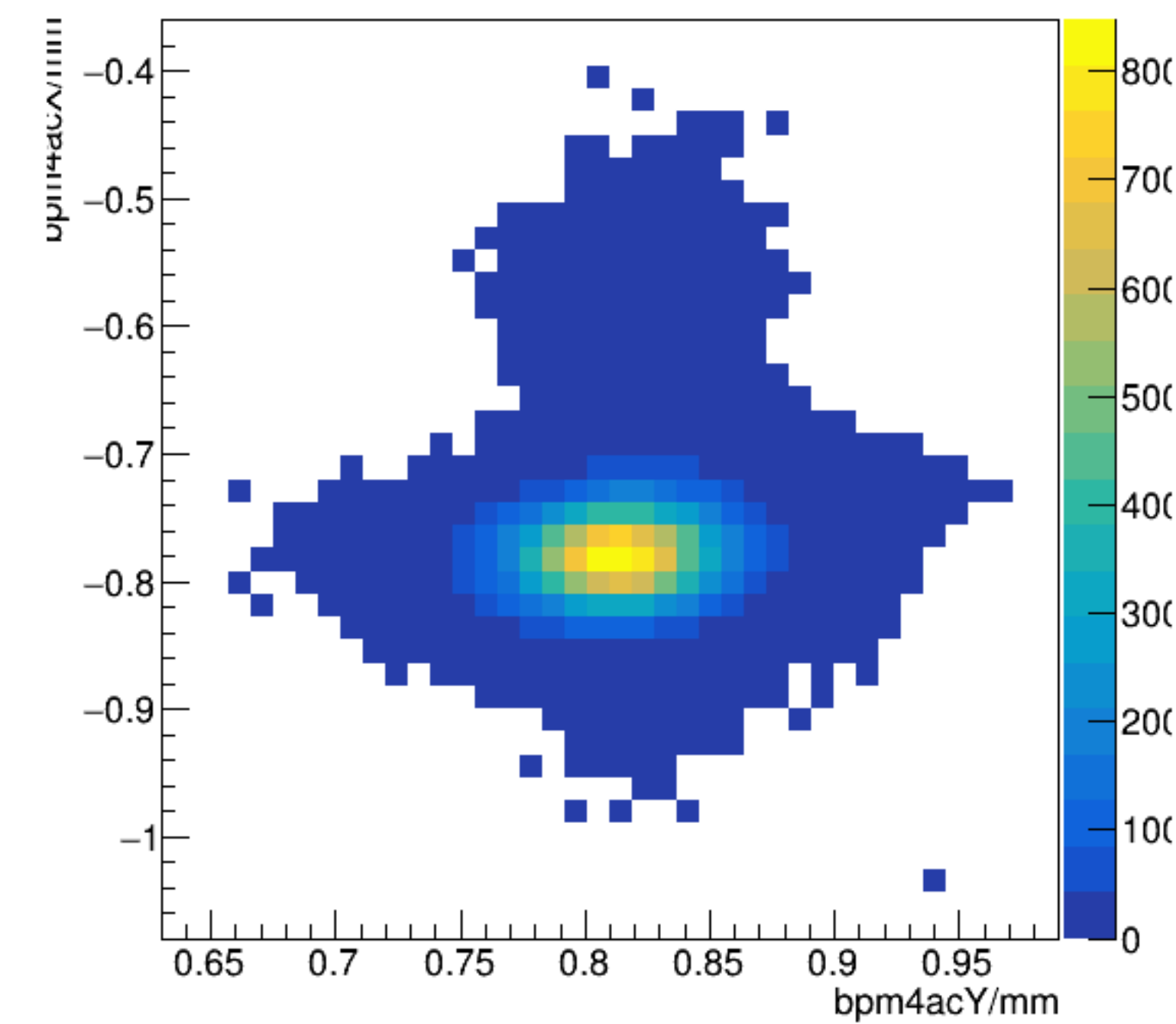
bpm4acX/mm:bpm4acY/mm {ErrorFlag==0}
