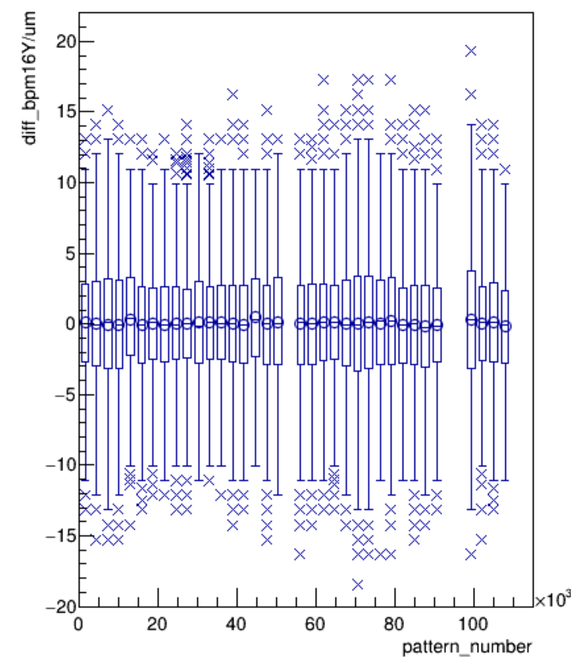
diff_bpm16Y/um:pattern_number {ErrorFlag==0}
