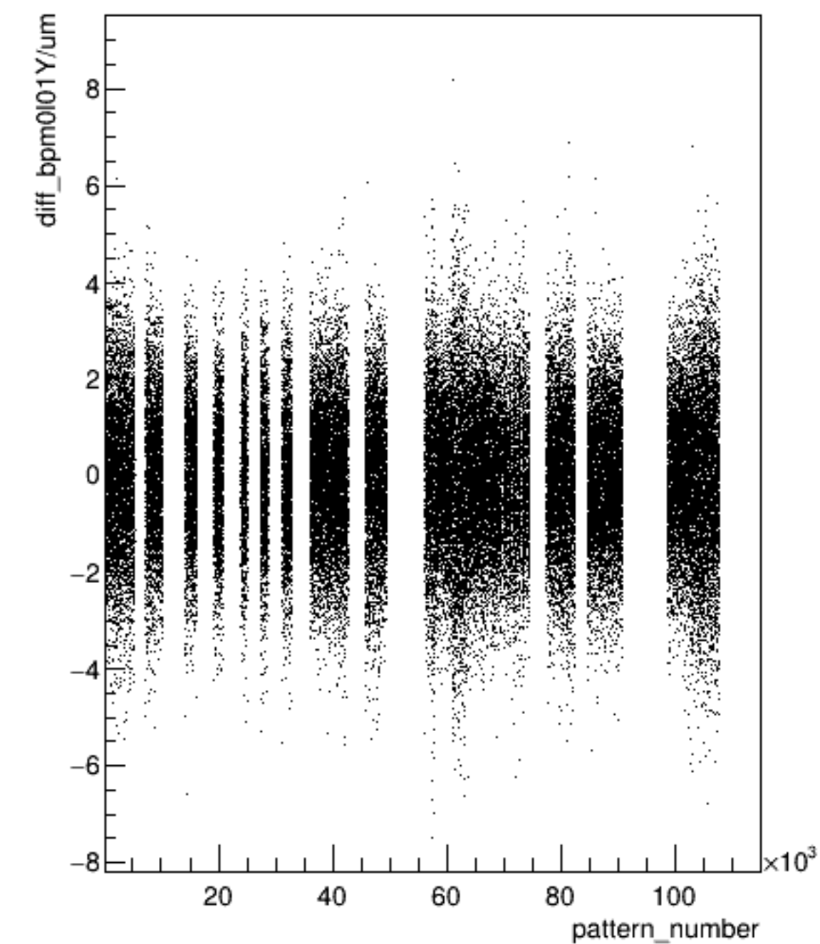
diff_bpm0101Y/um:pattern_number {ErrorFlag==0}
