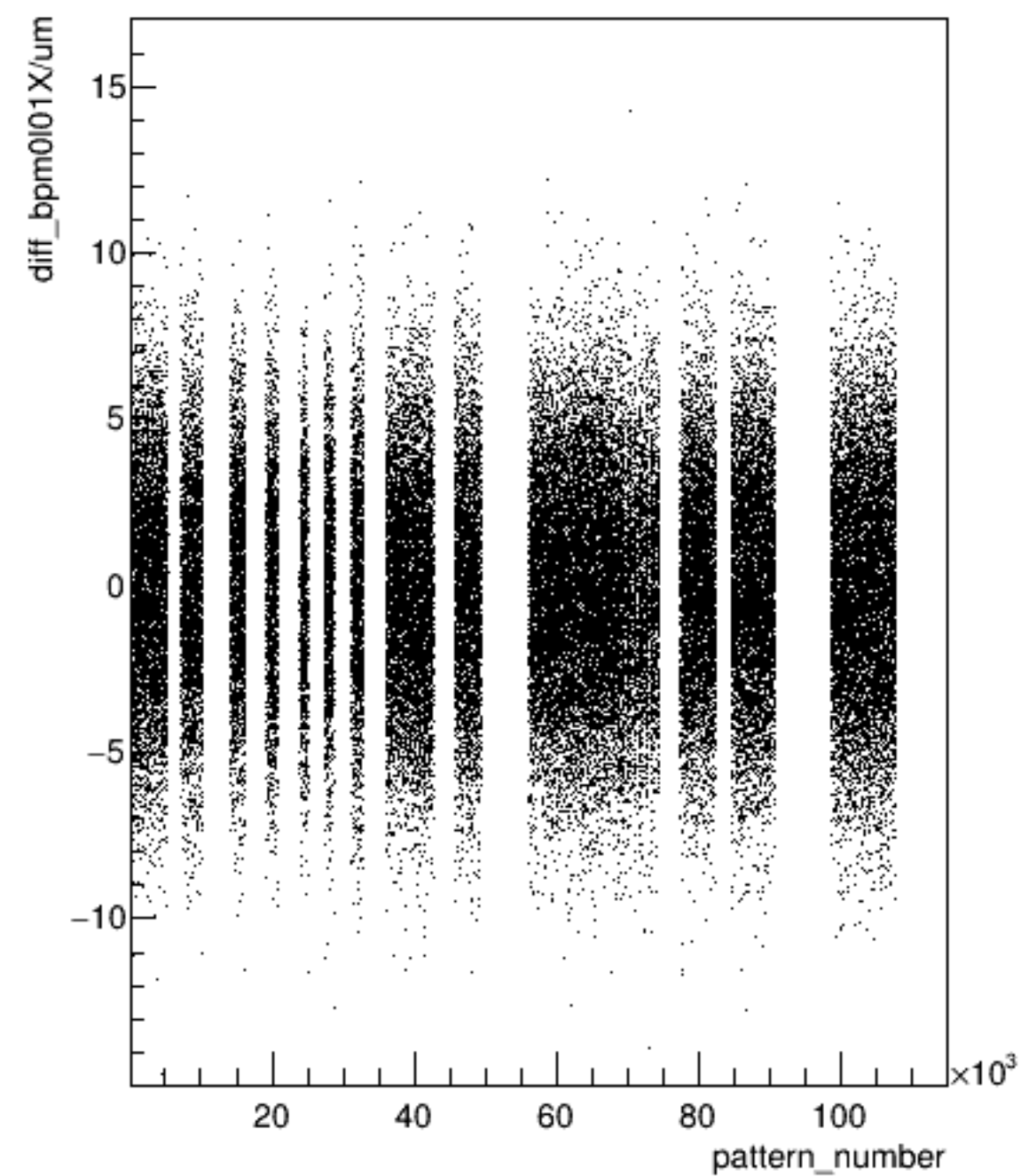
diff_bpm0101X/um:pattern_number {ErrorFlag==0}
