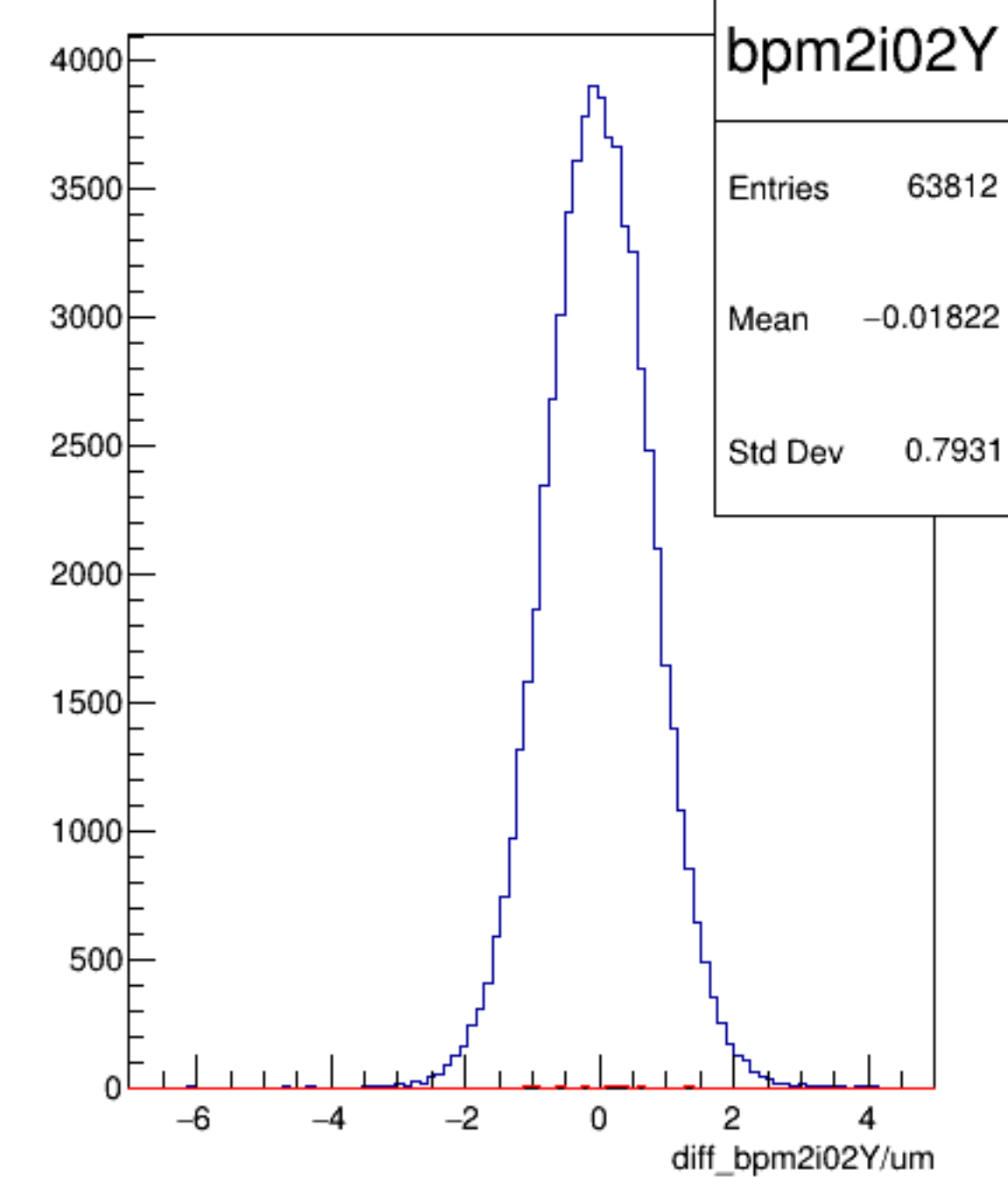
diff_bpm2i02Y/um {ErrorFlag==0}
