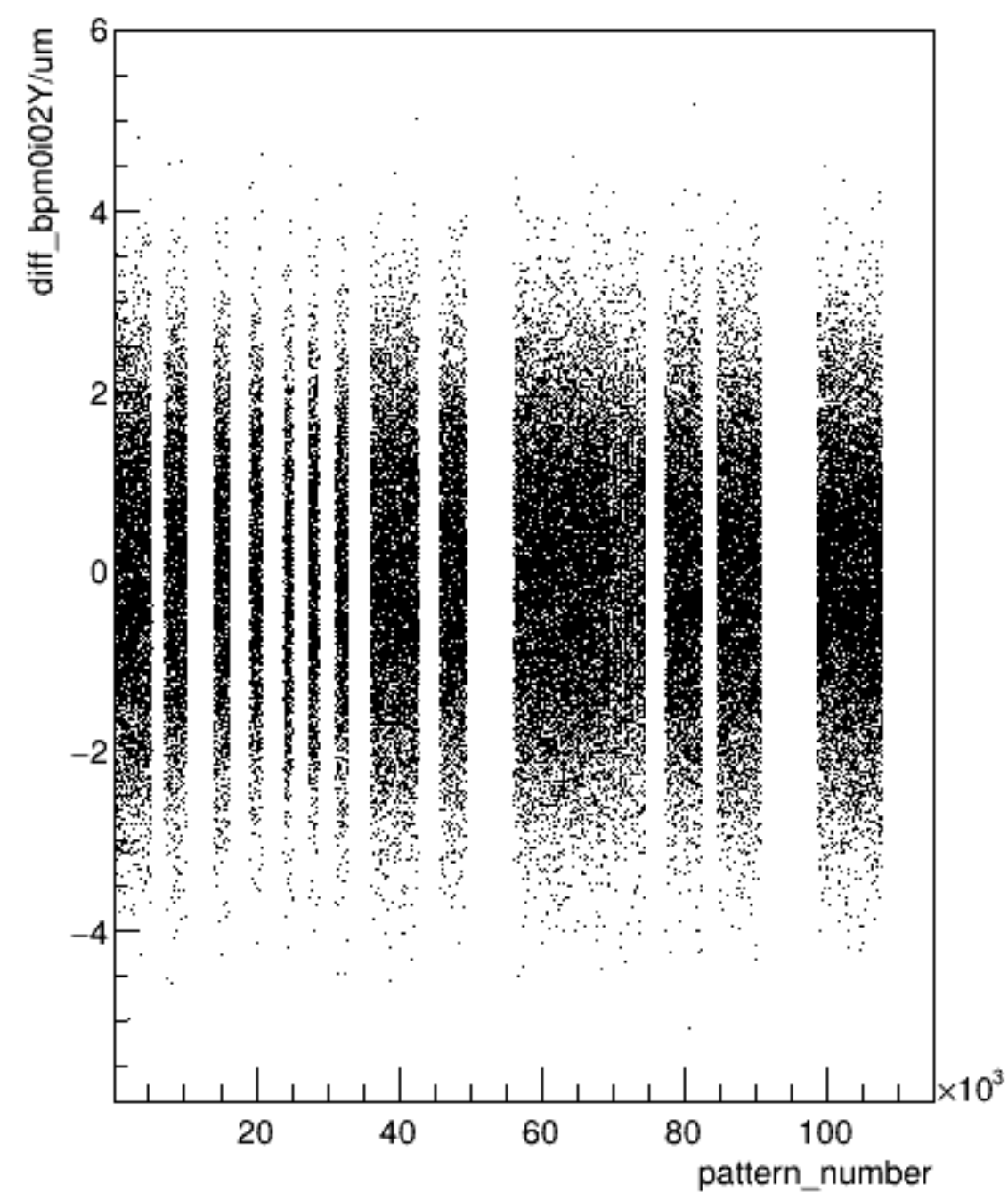
diff_bpm0i02Y/um:pattern_number (ErrorFlag==0)
