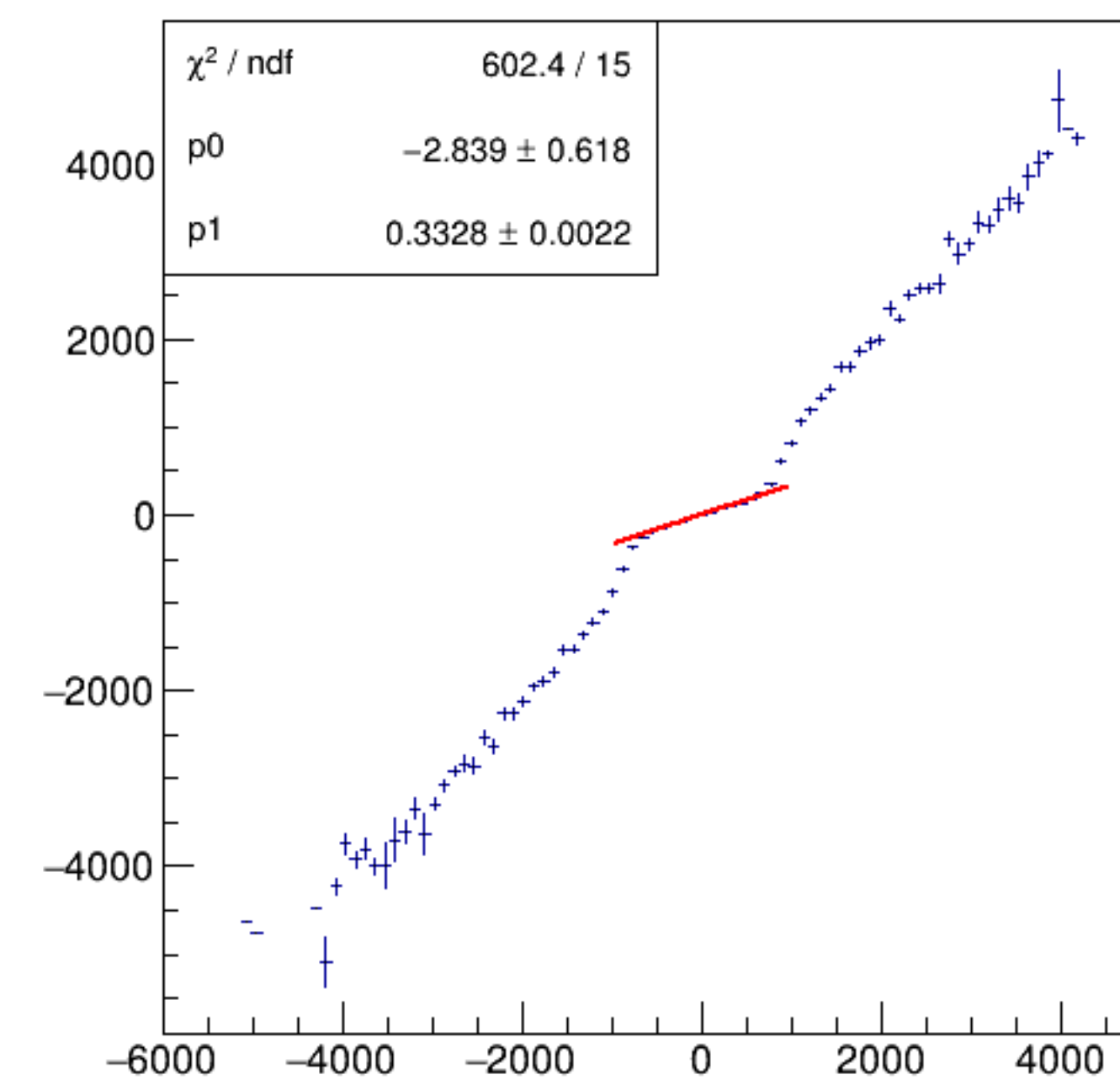
asym_bpm0i02WS/ppm:Aq/ppm {ErrorFlag==0}
