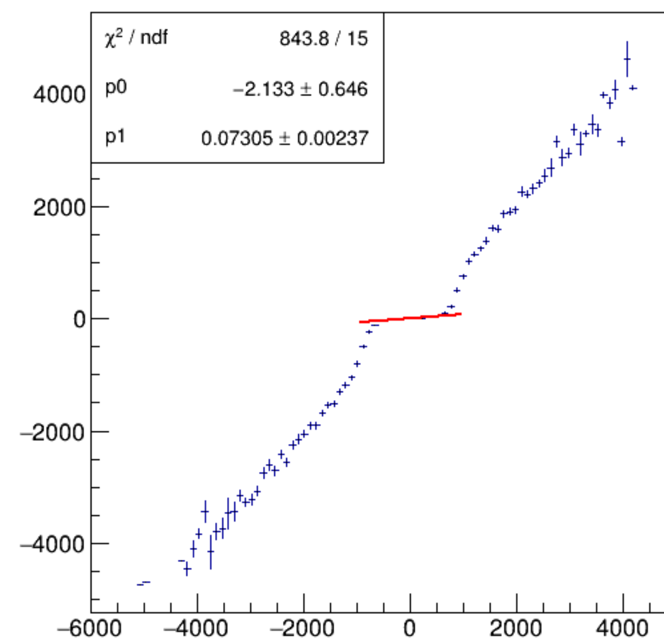
asym_bpm2i02WS/ppm:Aq/ppm {ErrorFlag==0}
