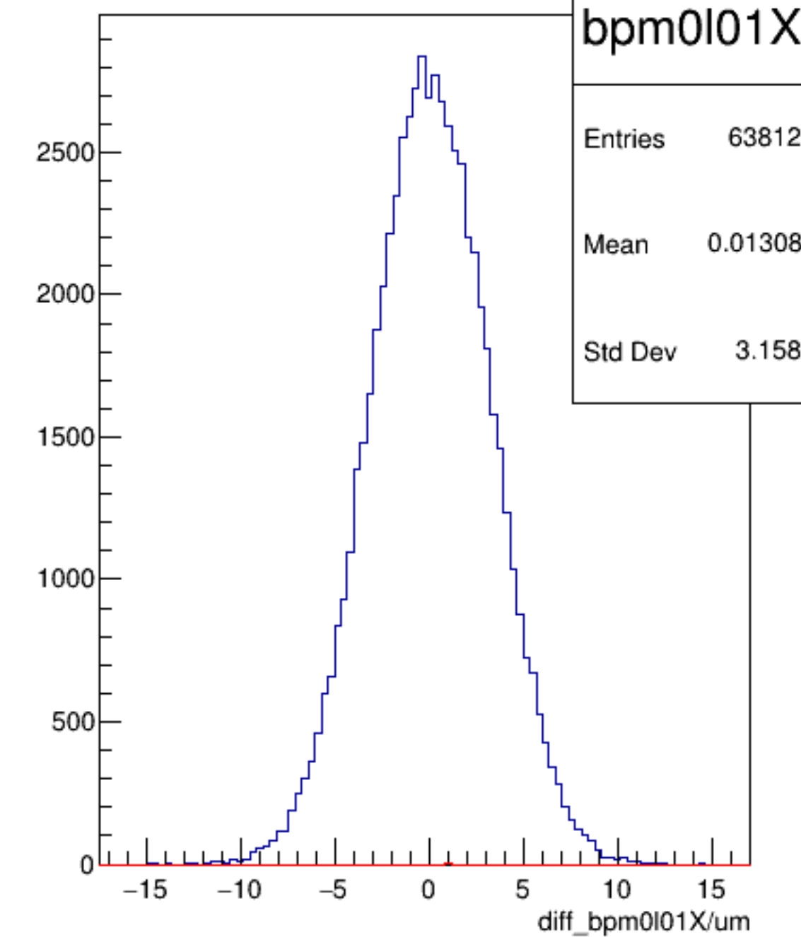
diff_bpm0101X/um {ErrorFlag==0}
