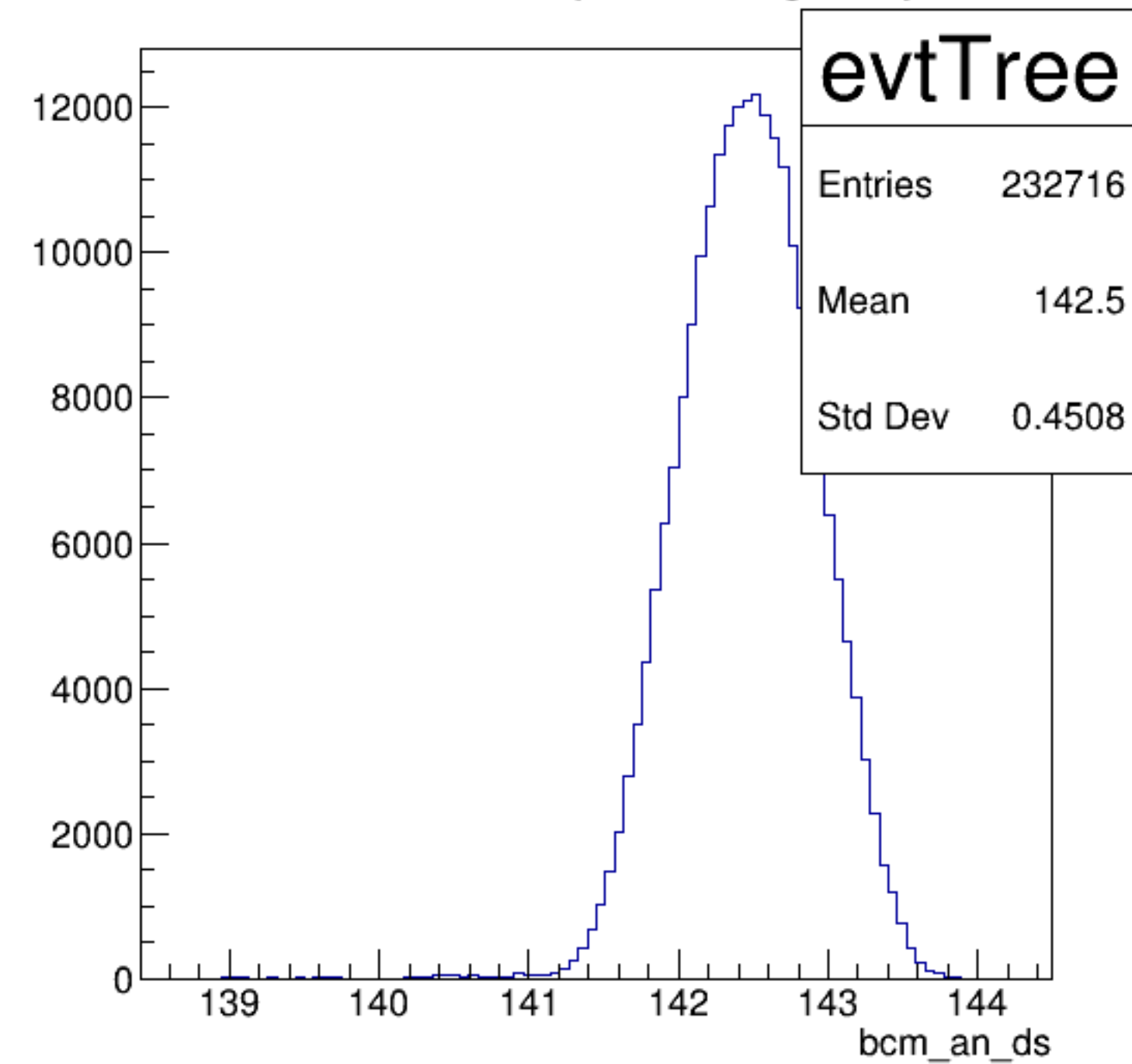
bcm_an_ds {ErrorFlag==0}
