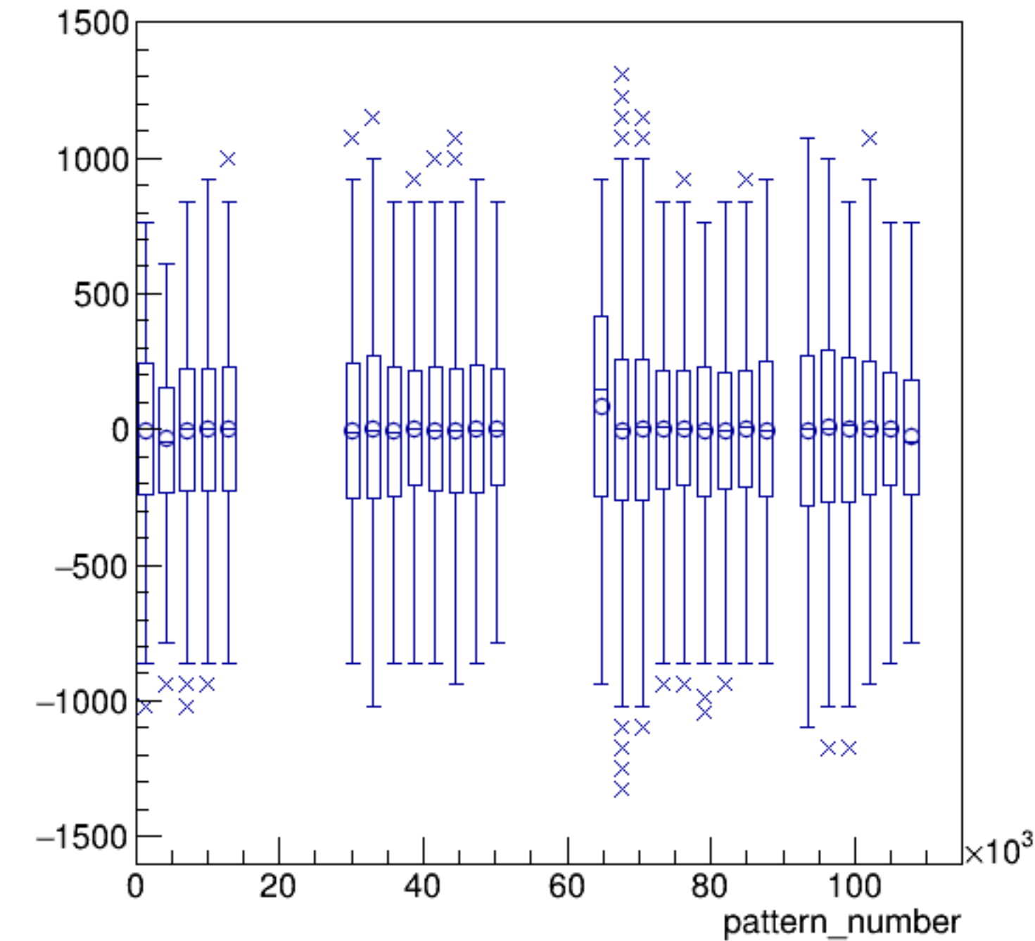
asym_bcm_an_ds/ppm:pattern_number {ErrorFlag==0}
