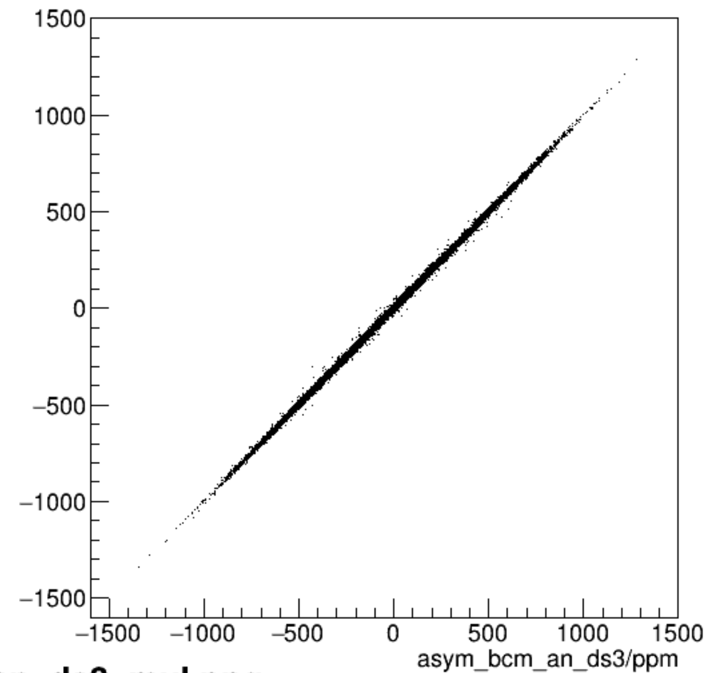
run6131_000_asym_bcm_an_ds_vs_asym_bcm_an_ds3_mul.png
