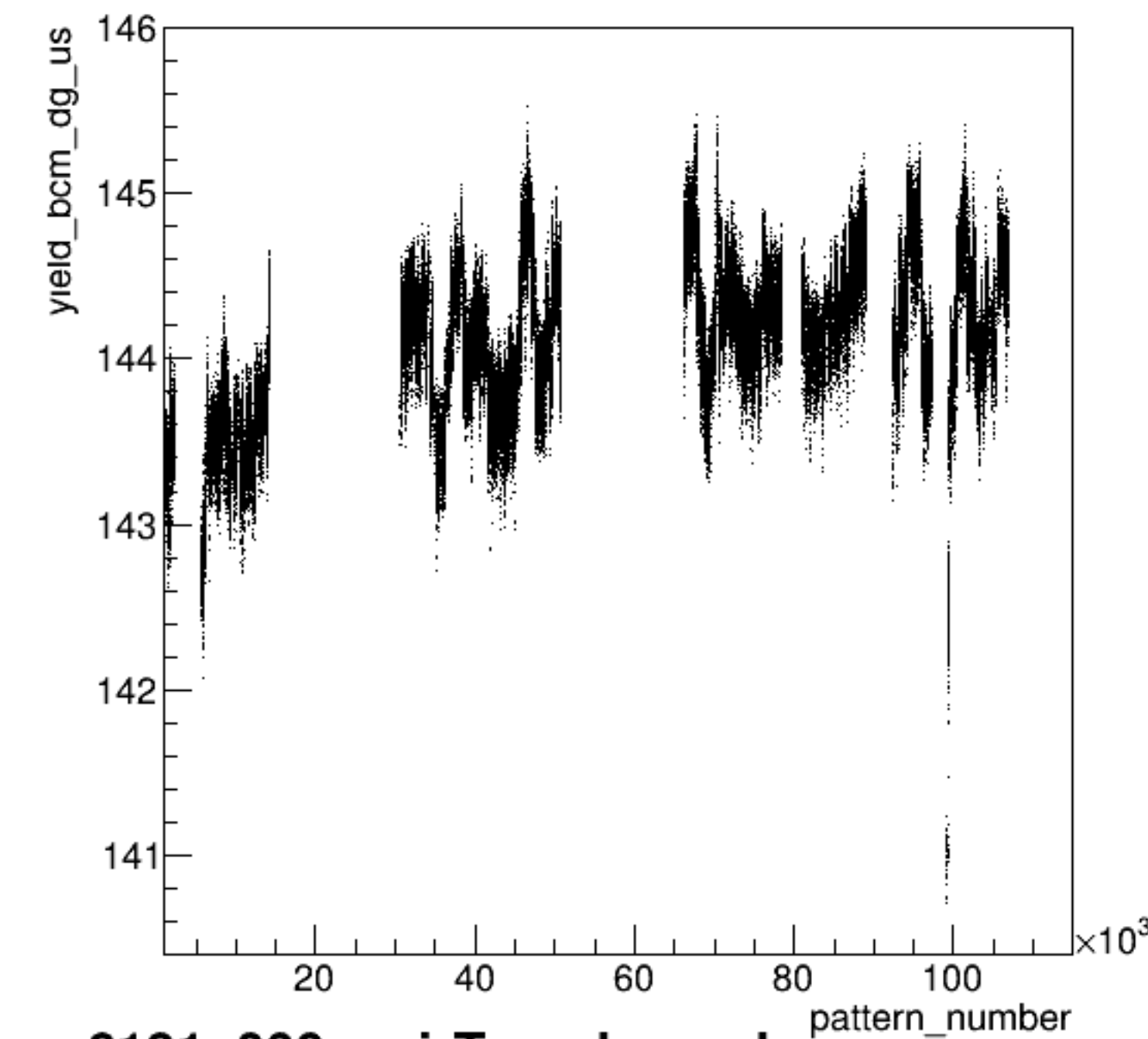
yield_bcm_dg_us:pattern_number {ErrorFlag==0}
