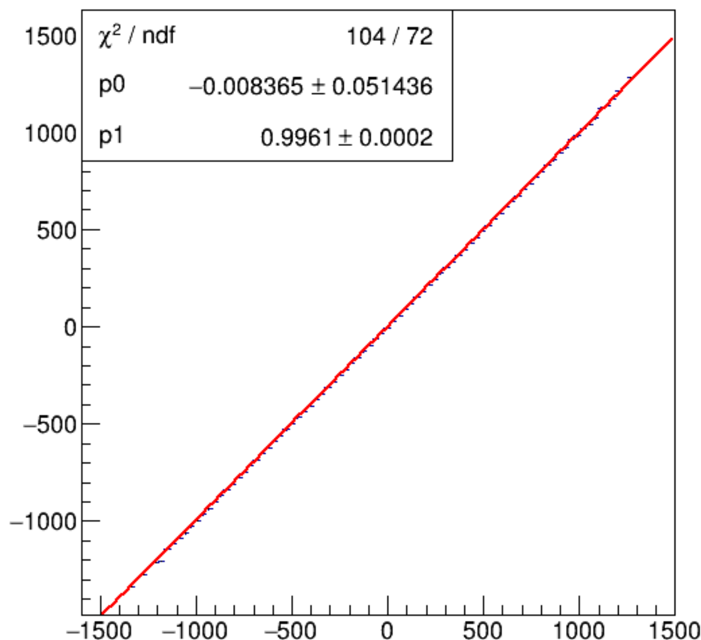
run6131_000_asym_bcm_an_ds_vs_asym_bcm_an_ds3_mul.png
