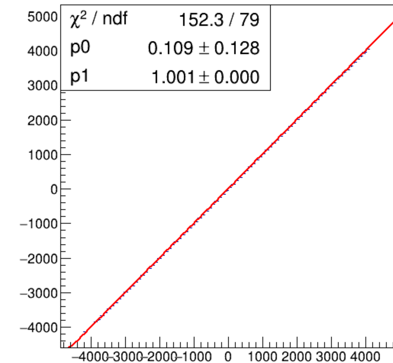
run6131_000_asym_bcm_an_us_vs_asym_bcm_an_ds_pr.png
