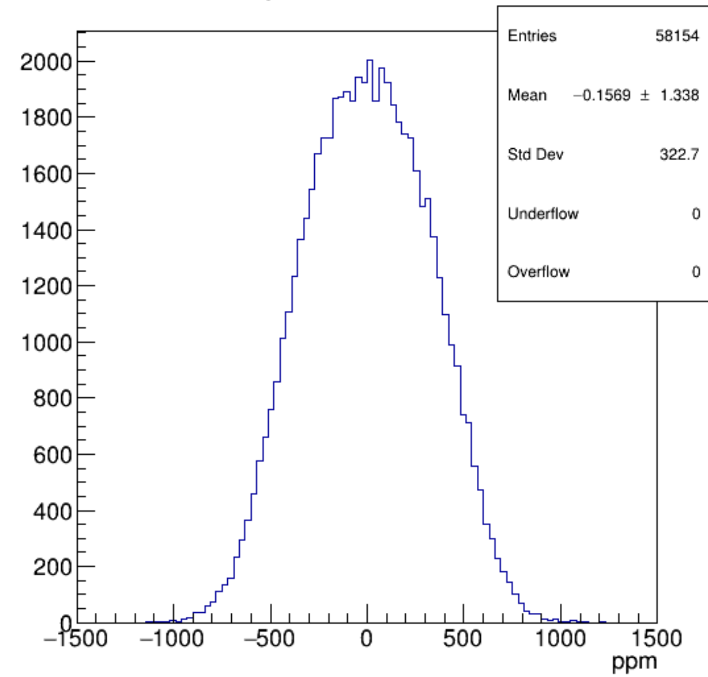
asym_bcm_an_us
