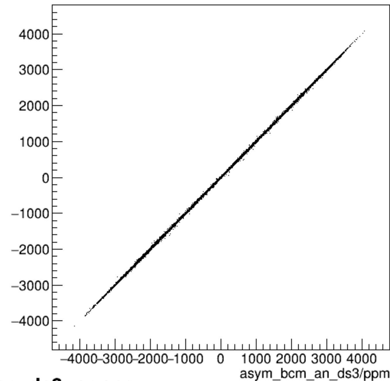
run6131_000_asym_bcm_an_ds_vs_asym_bcm_an_ds3_pr.png
