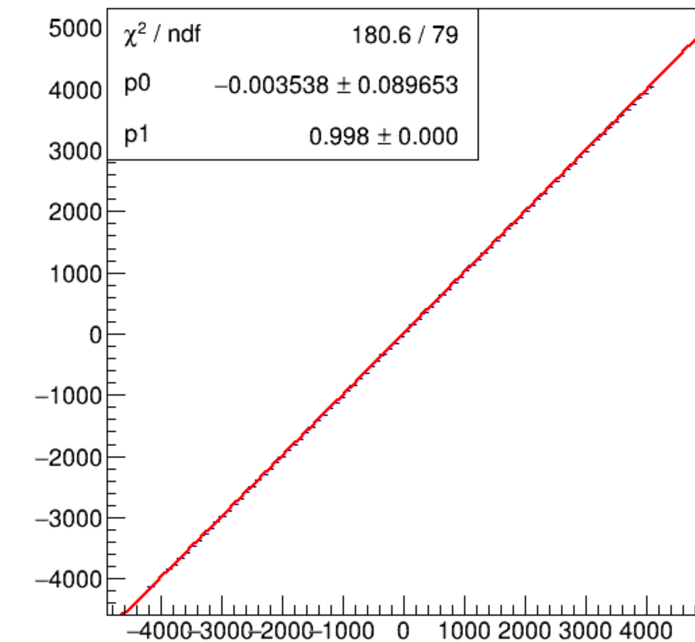
run6131_000_asym_bcm_an_ds_vs_asym_bcm_an_ds3_pr.png
