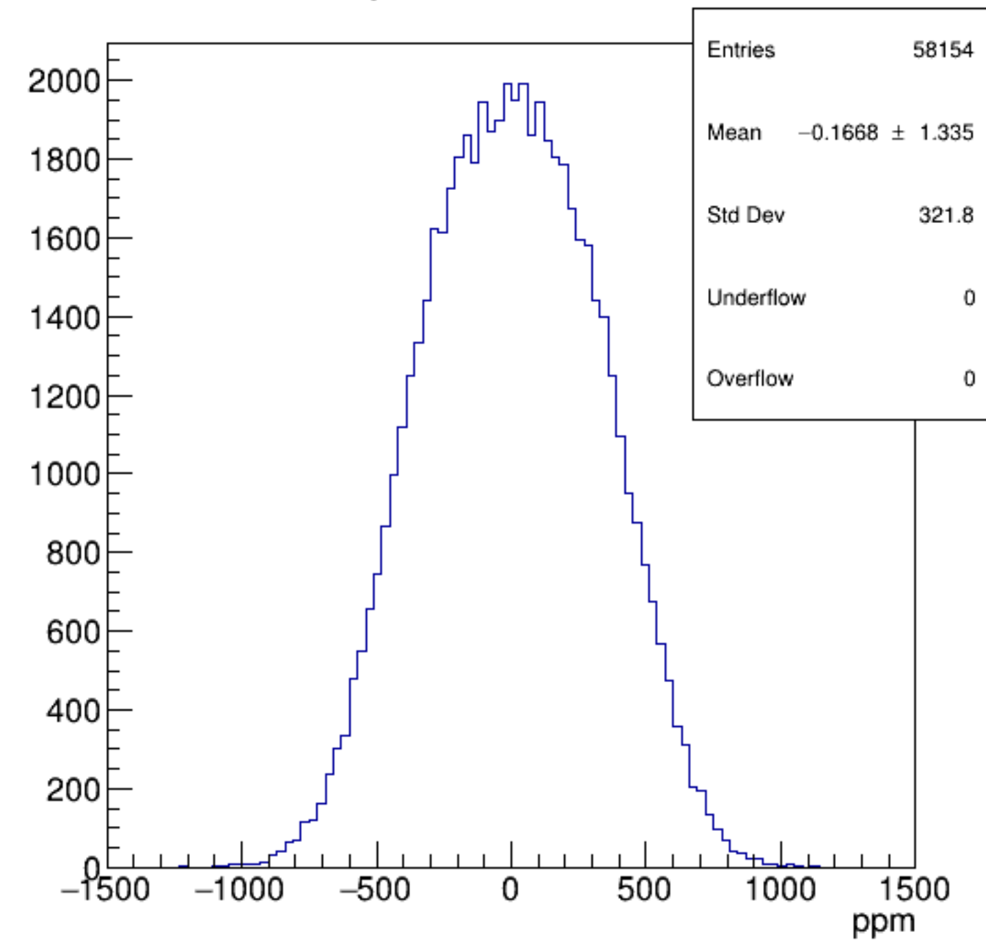
asym_bcm_an_ds
