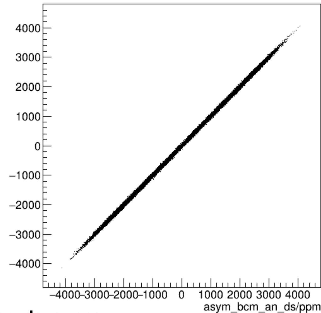
run6131_000_asym_bcm_an_us_vs_asym_bcm_an_ds_pr.png
