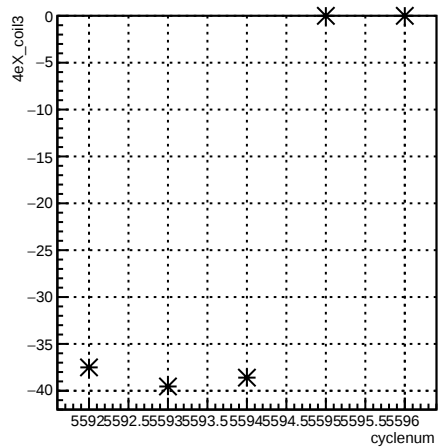
4eX_coil3:cyclenum {run == 6133}
