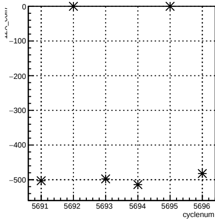
12X_coil7:cyclenum {run == 6186}
