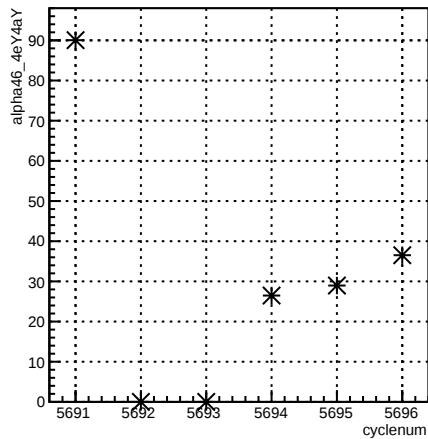
alpha46_4eY4aY:cyclenum {run == 6186}
