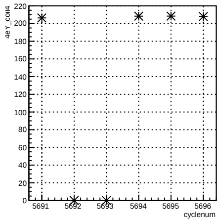
4eY_coil4:cyclenum {run == 6186}
