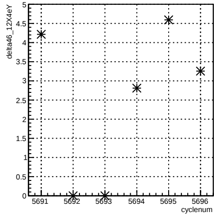
delta46_12X4eY:cyclenum {run == 6186}
