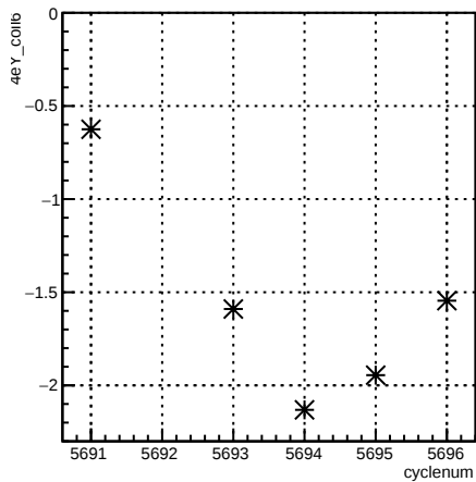
4eY_coil6:cyclenum {run == 6186}
