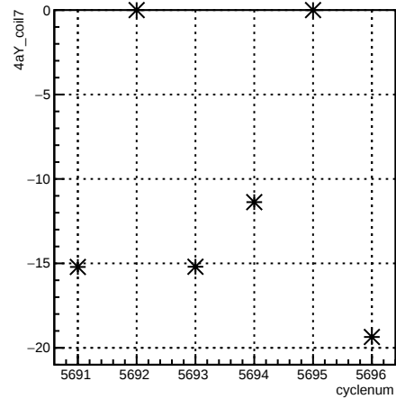
4aY_coil7:cyclenum {run == 6186}
