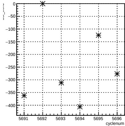
usl_coil6:cyclenum {run == 6186}
