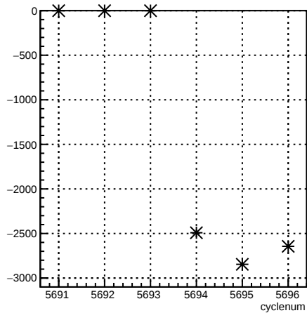
usr_coil3:cyclenum {run == 6186}
