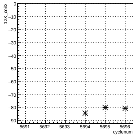
12X_coil3:cyclenum {run == 6186}
