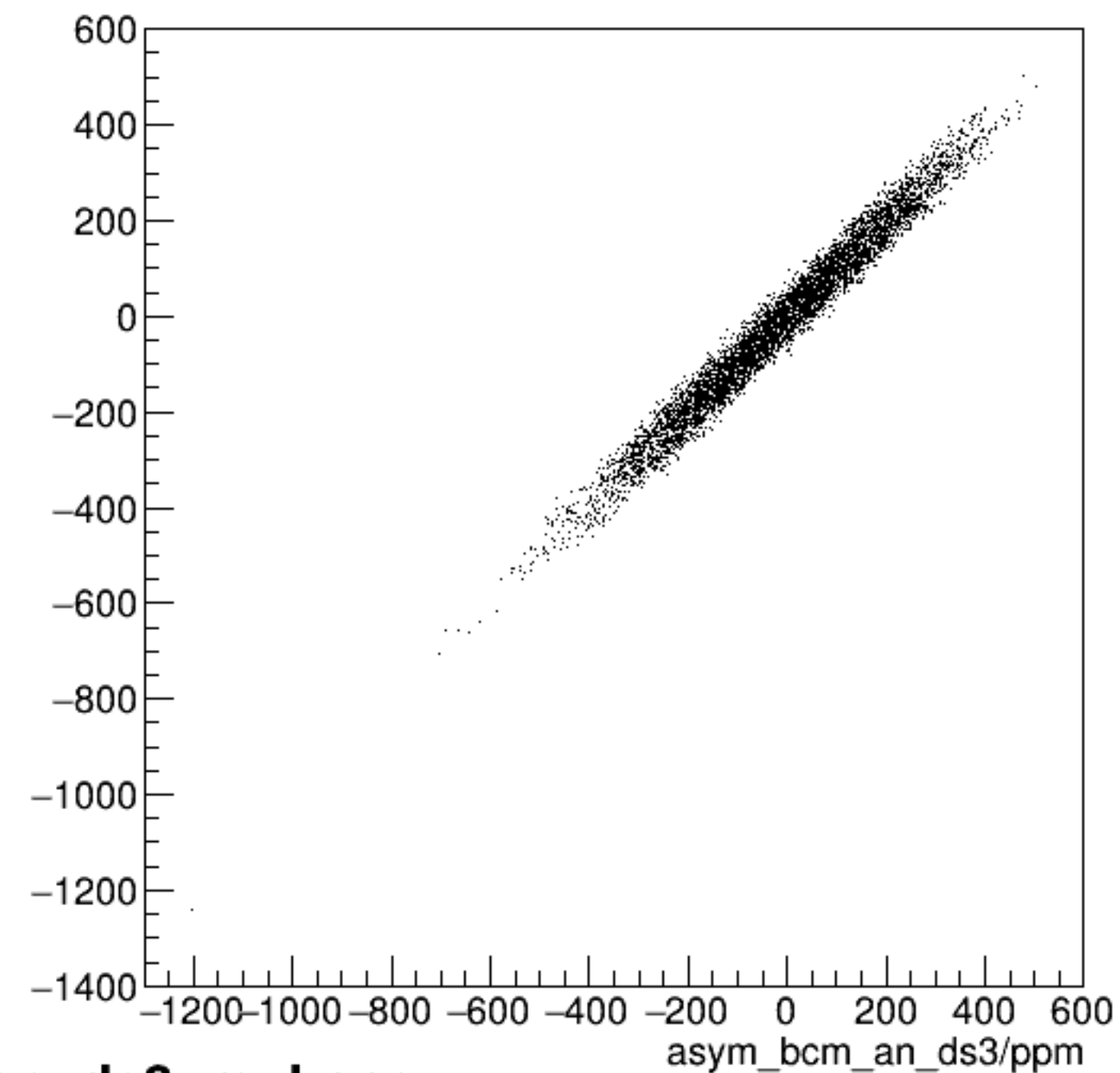
run6201_000_asym_bcm_an_us_vs_asym_bcm_an_ds3_mul.png
