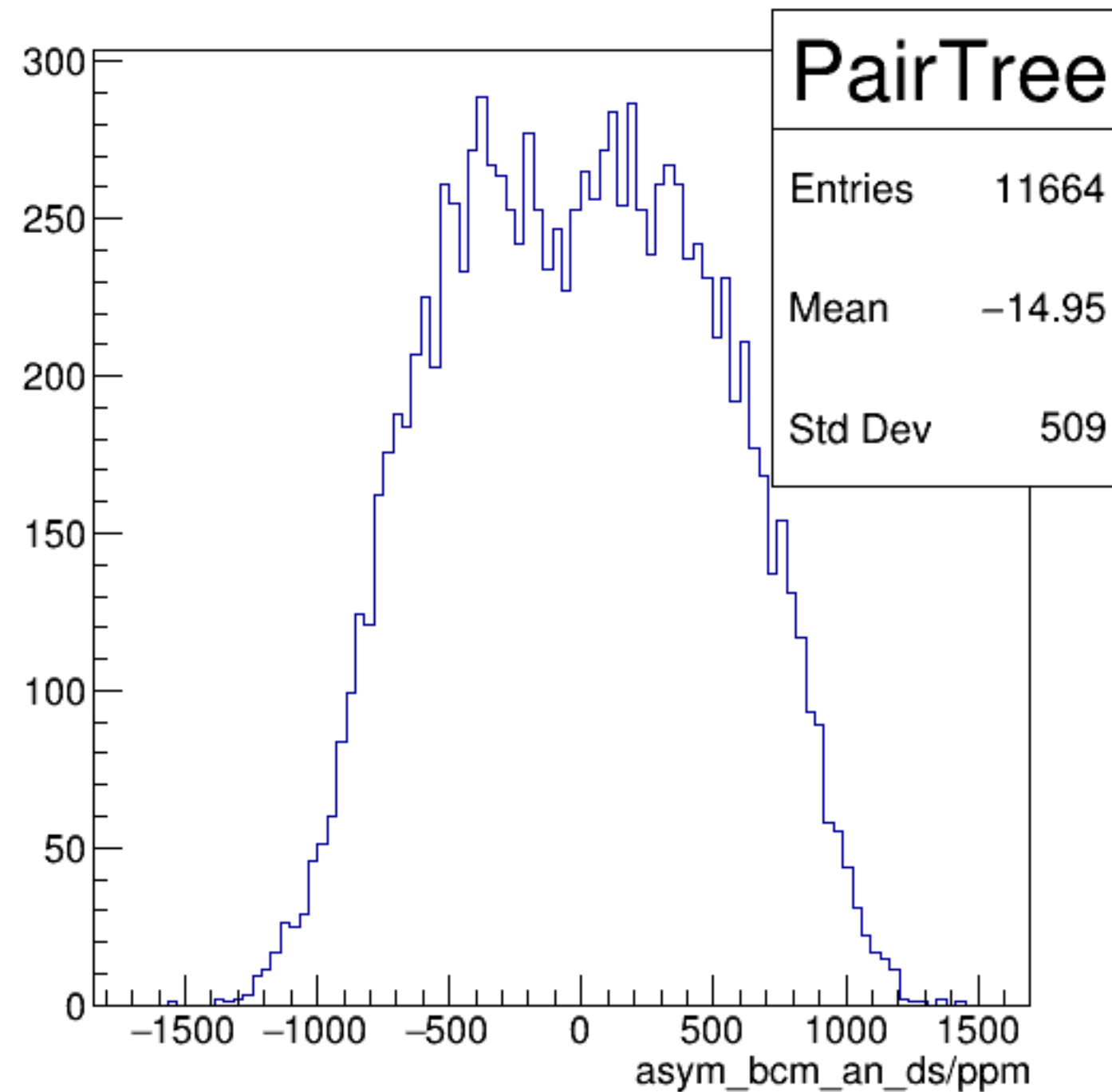
asym_bcm_an_ds/ppm {ErrorFlag==0}
