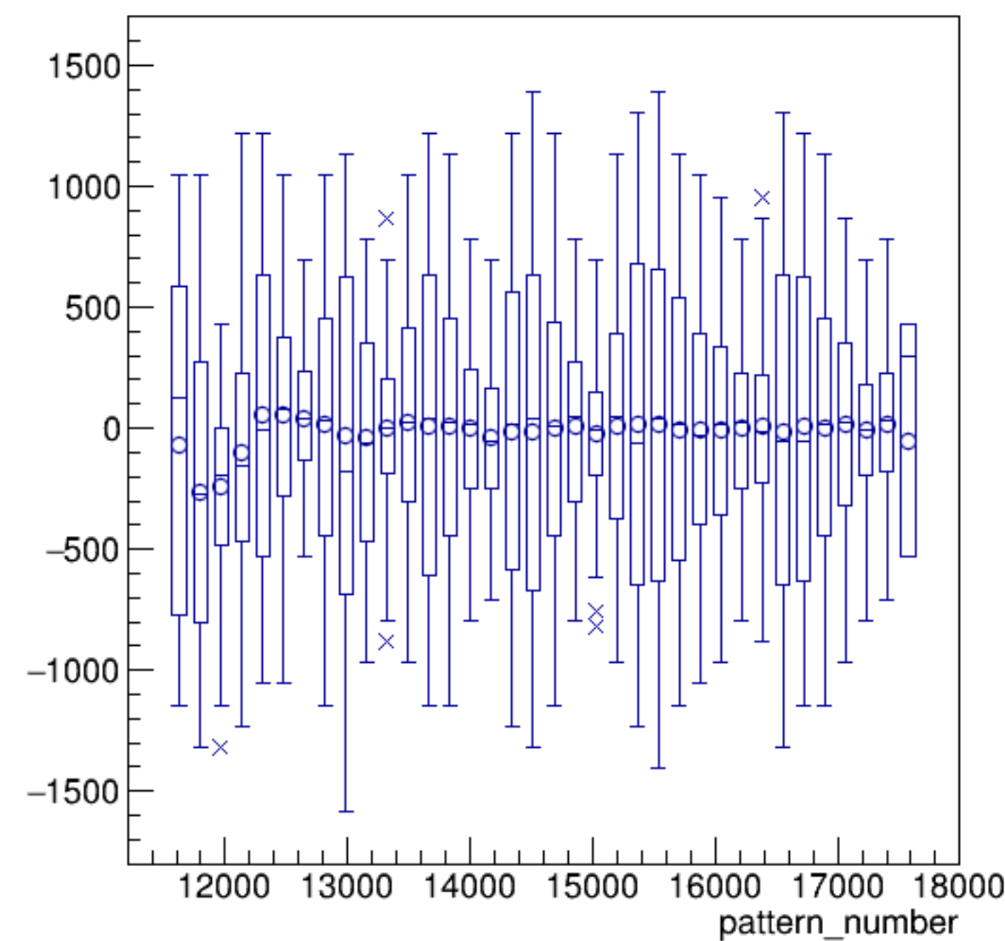
asym_bcm_an_ds/ppm:pattern_number {ErrorFlag==0}
