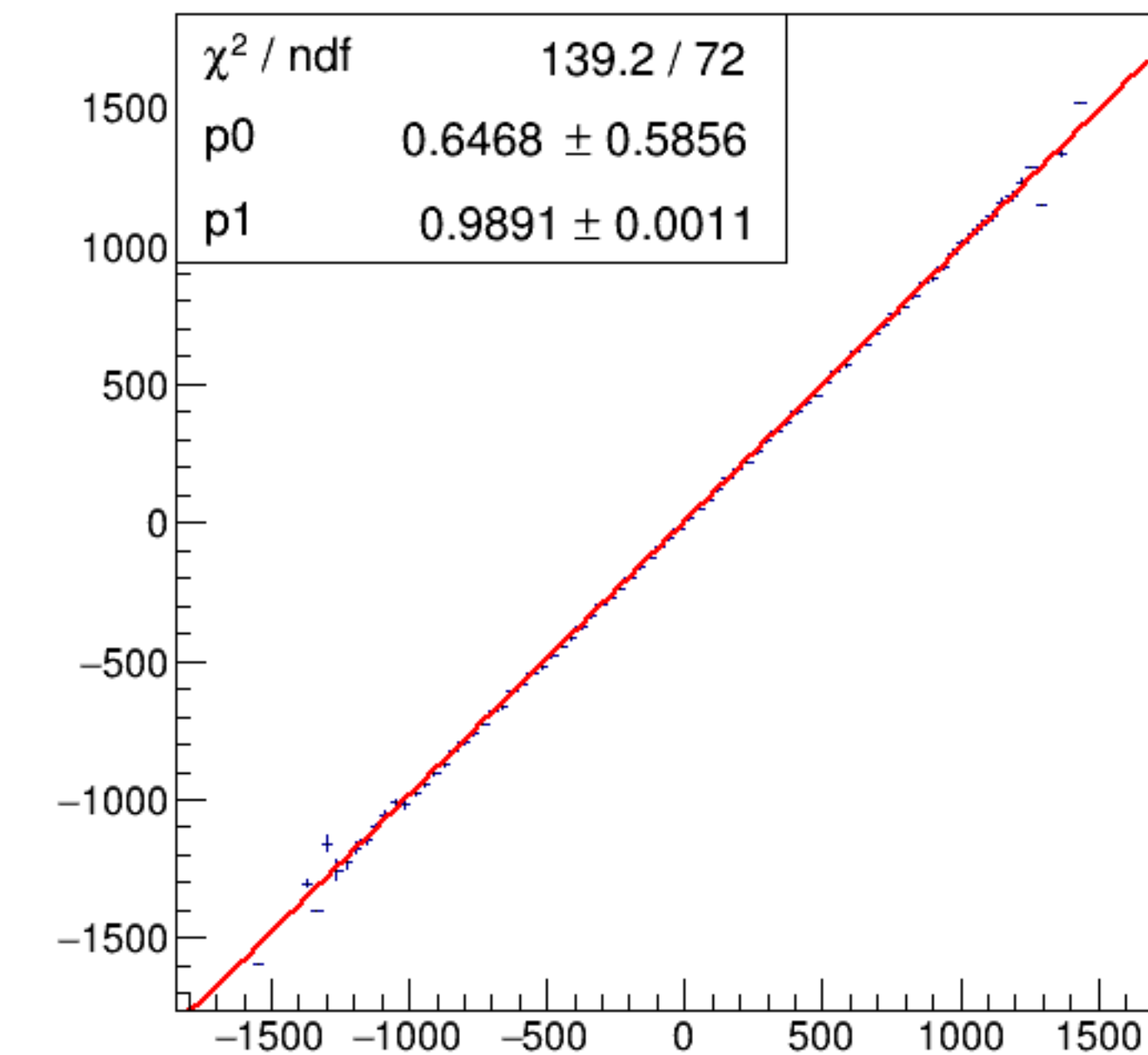
run6201_000_asym_bcm_dg_us_vs_asym_bcm_an_ds_pr.png
