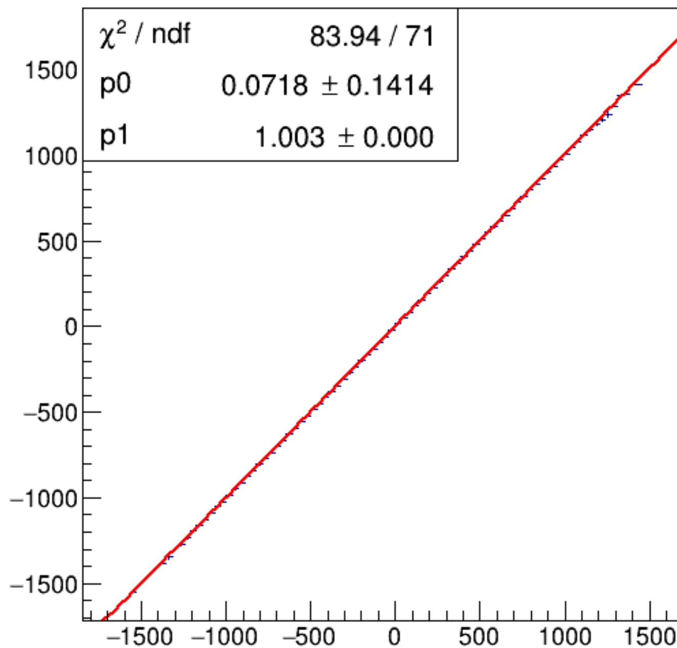
run6201_000_asym_bcm_an_ds_vs_asym_bcm_an_ds3_pr.png
