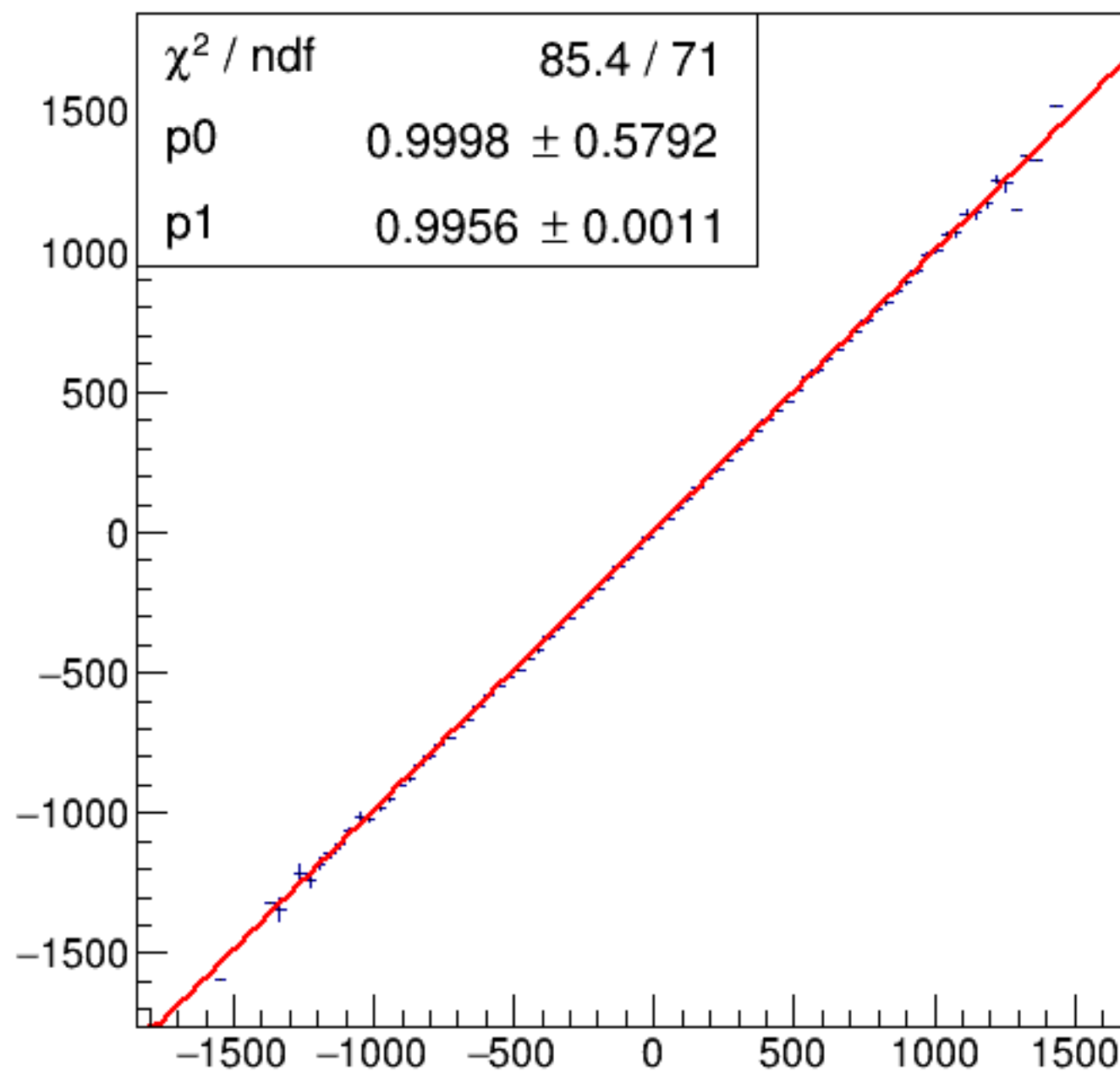
run6201_000_asym_bcm_dg_us_vs_asym_bcm_an_ds3_pr.png
