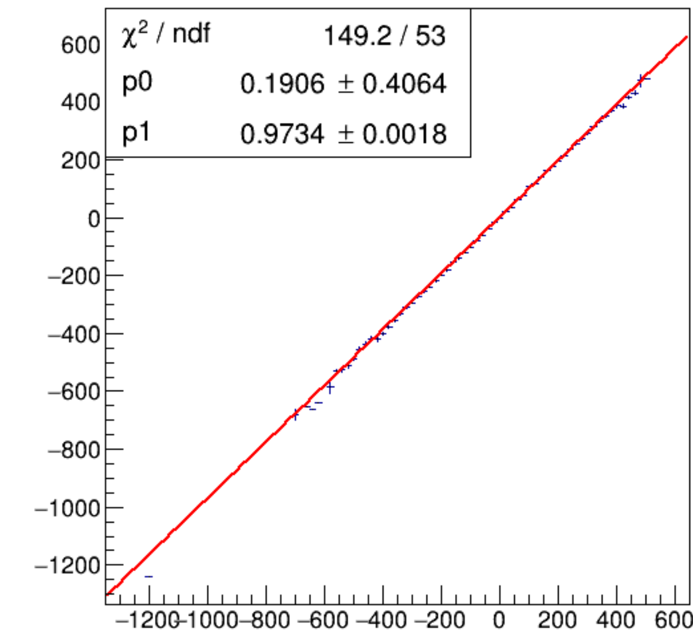
run6201_000_asym_bcm_an_us_vs_asym_bcm_an_ds3_mul.png
