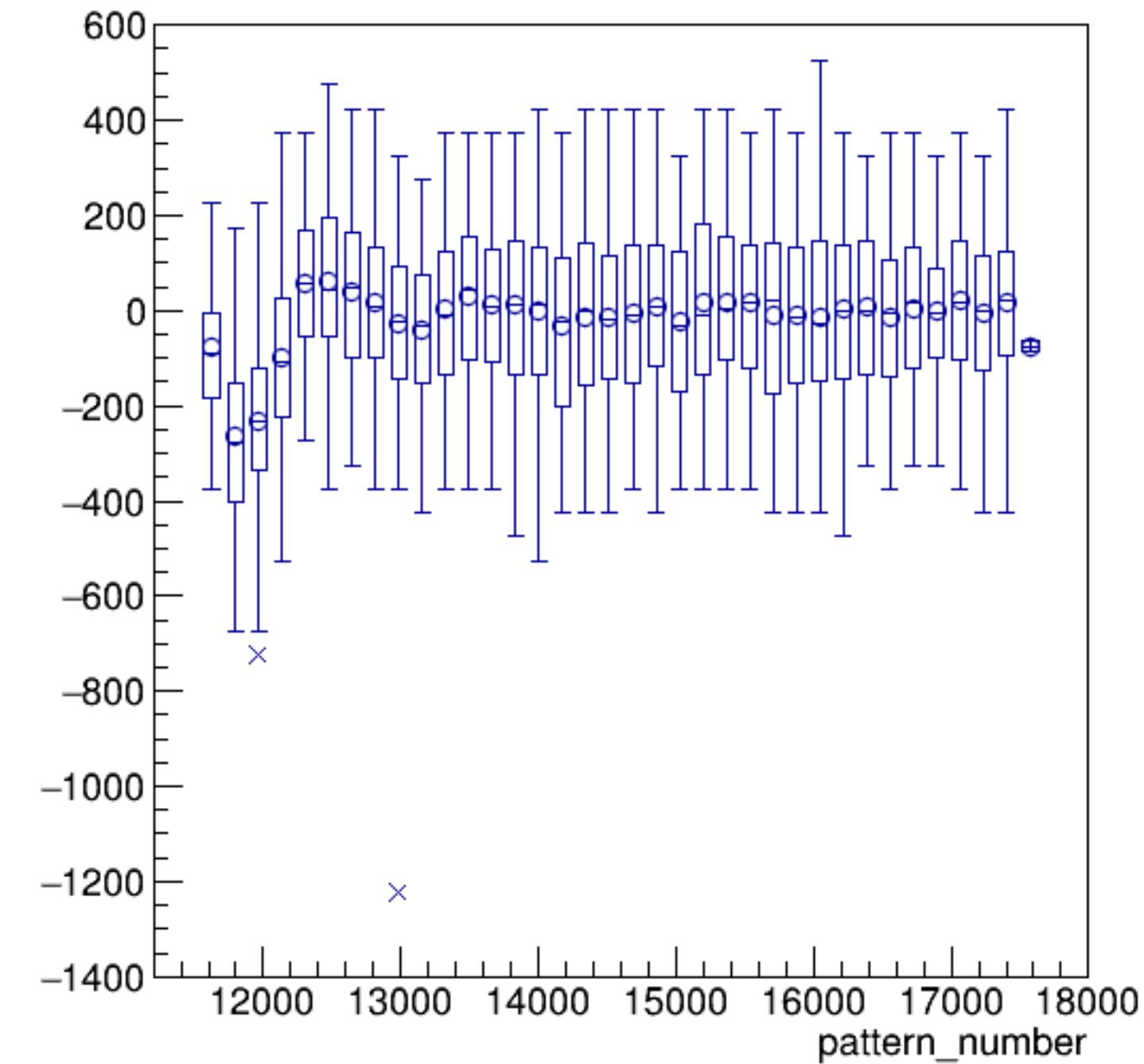
asym_bcm_an_us/ppm:pattern_number {ErrorFlag==0}
