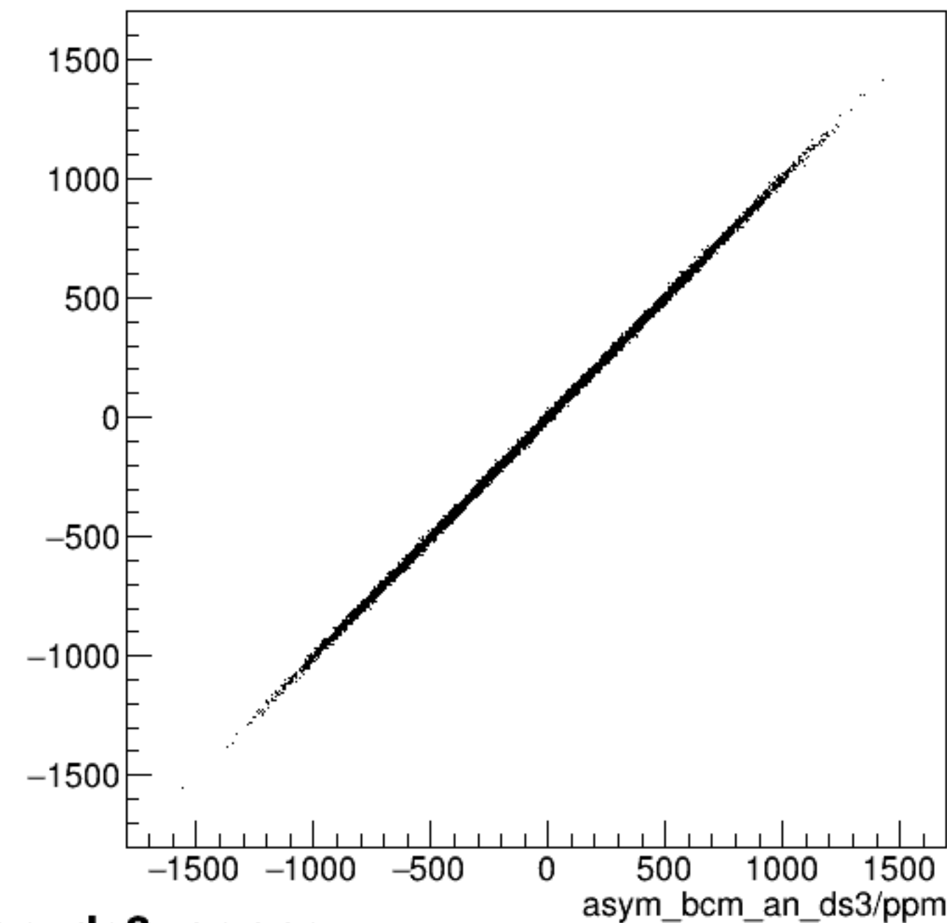
run6201_000_asym_bcm_an_ds_vs_asym_bcm_an_ds3_pr.png
