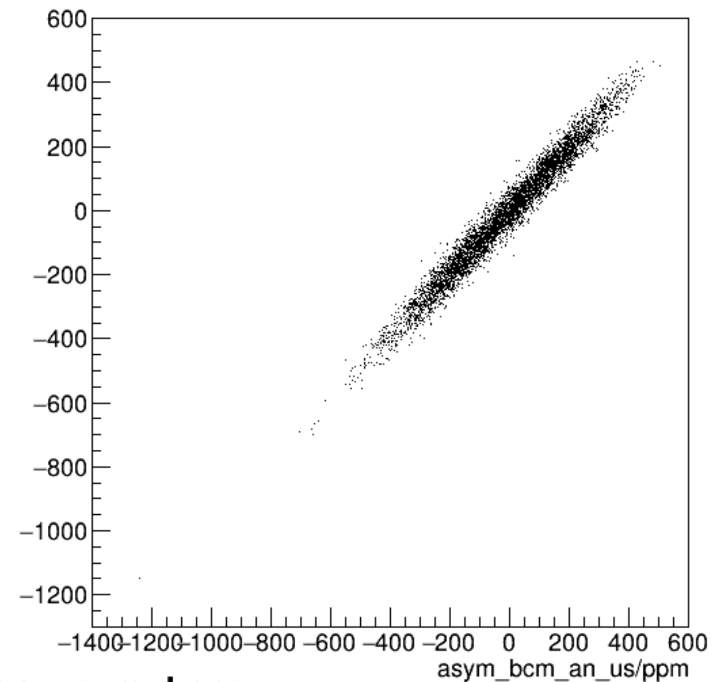
run6201_000_asym_bcm_dg_ds_vs_asym_bcm_an_us_mul.png
