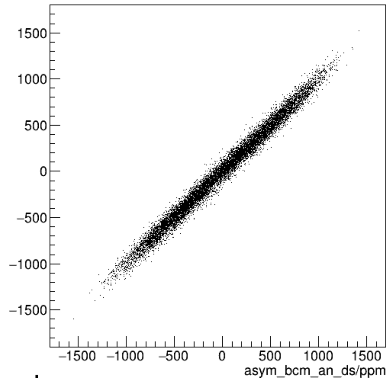
run6201_000_asym_bcm_dg_us_vs_asym_bcm_an_ds_pr.png
