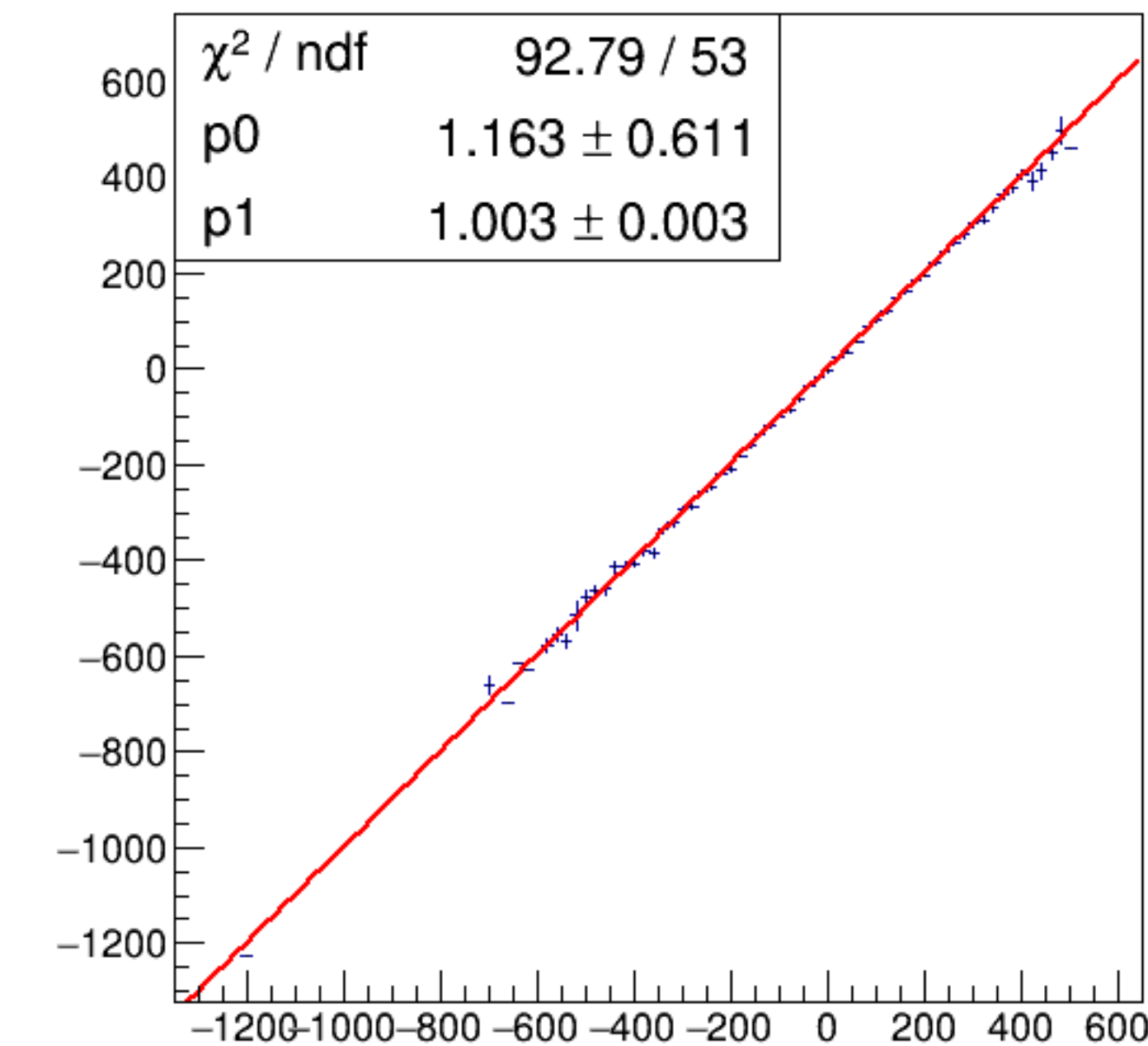
run6201_000_asym_bcm_dg_us_vs_asym_bcm_an_ds3_mul.png
