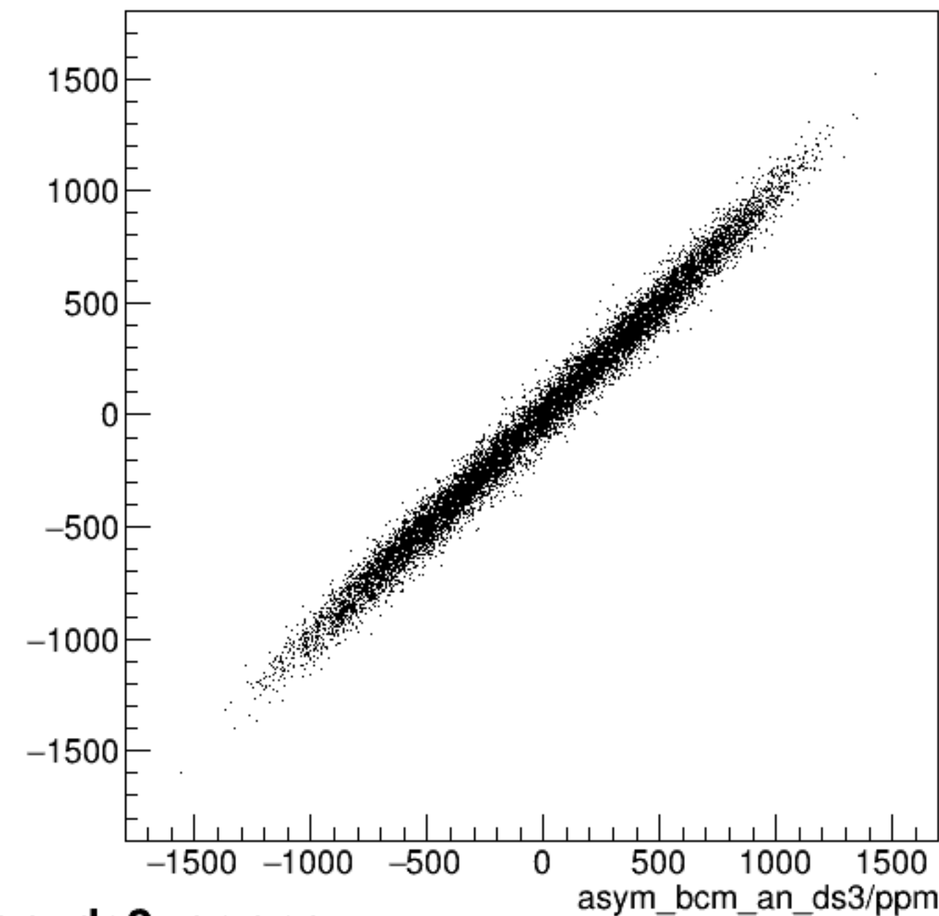
run6201_000_asym_bcm_dg_us_vs_asym_bcm_an_ds3_pr.png
