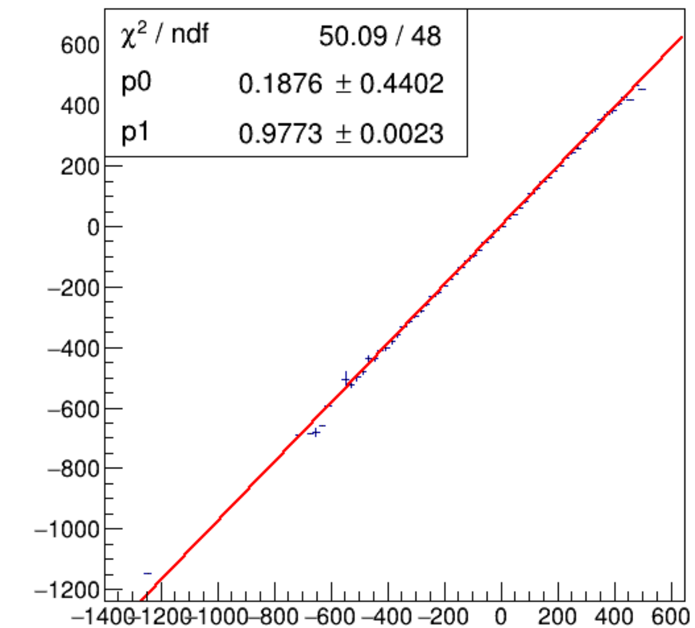
run6201_000_asym_bcm_dg_ds_vs_asym_bcm_an_us_mul.png
