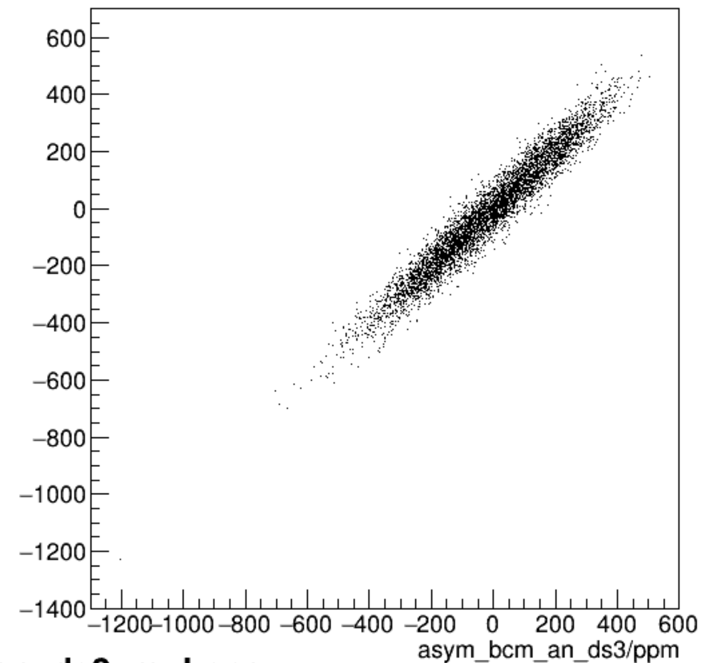
run6201_000_asym_bcm_dg_us_vs_asym_bcm_an_ds3_mul.png
