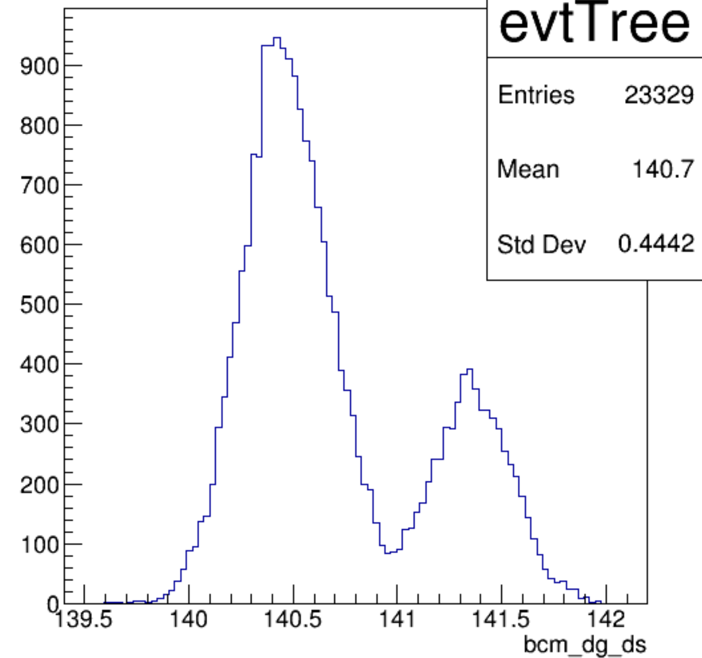
bcm_dg_ds {ErrorFlag==0}
