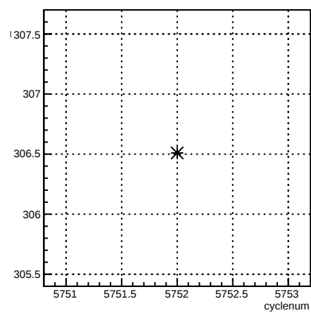
1X_coil7:cyclenum {run == 6208}
