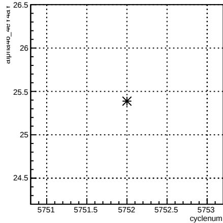
alpha46_4eY4aY:cyclenum {run == 6208}
