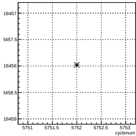
usr_coil6:cyclenum {run == 6208}
