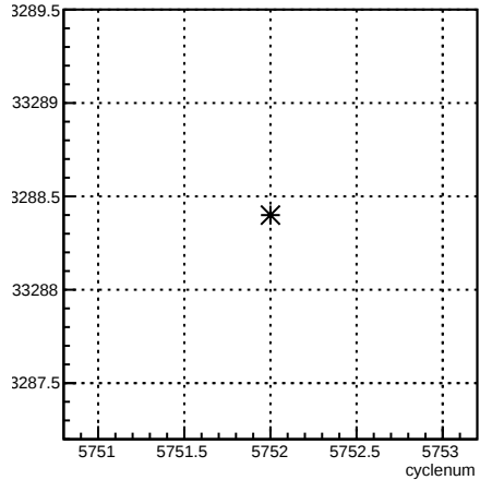
usr_coil7:cyclenum {run == 6208}
