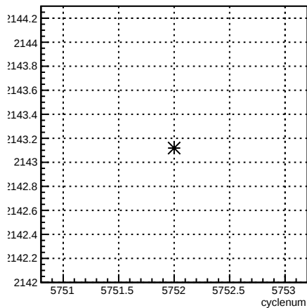
usl_coil7:cyclenum {run == 6208}
