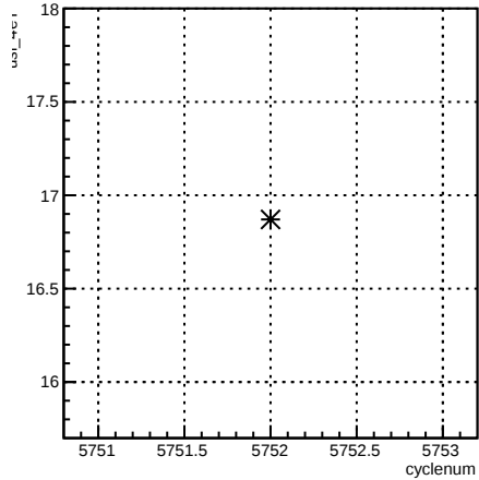
usl_4eY:cyclenum {run == 6208}
