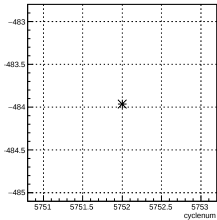
12X_coil7:cyclenum {run == 6208}
