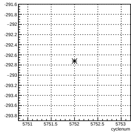
1X_coil1:cyclenum {run == 6208}
