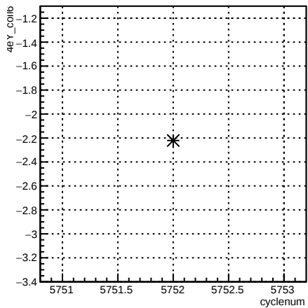
4eY_coil6:cyclenum {run == 6208}
