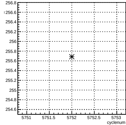
4eX_coil7:cyclenum {run == 6208}
