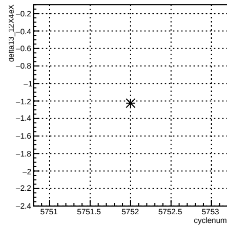
delta13_12X4eX:cyclenum {run == 6208}
