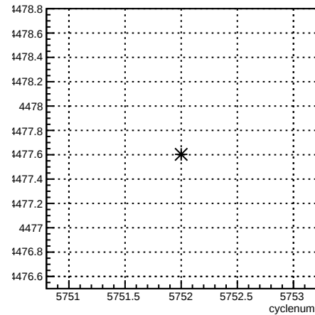
usl_coil4:cyclenum {run == 6208}
