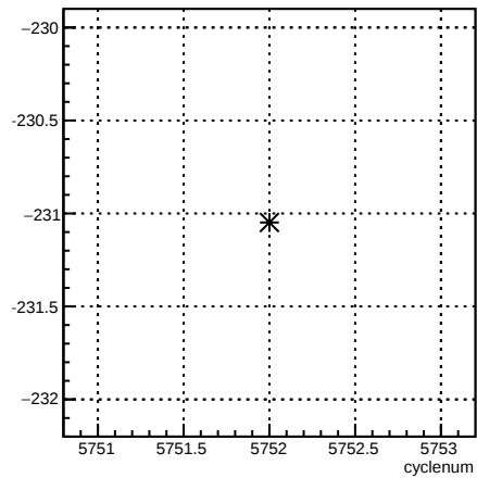
12X_coil6:cyclenum {run == 6208}
