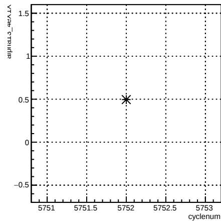
alpha13_4eX1X:cyclenum {run == 6208}
