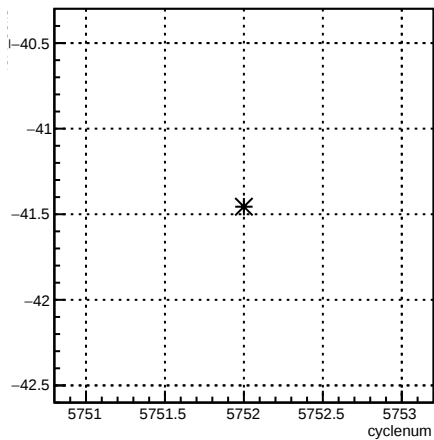
4eX_coil3:cyclenum {run == 6208}
