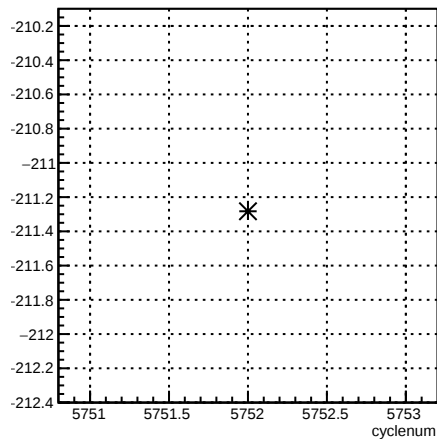
usl_coil6:cyclenum {run == 6208}
