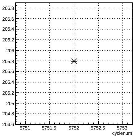
4eY_coil4:cyclenum {run == 6208}
