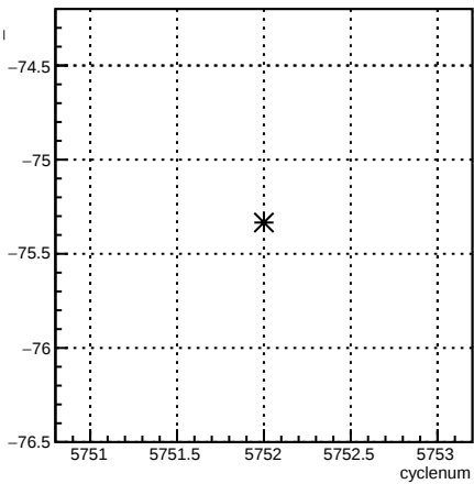
usl_4eY:cyclenum {run == 6208}
