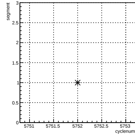
segment:cyclenum {run == 6208}
