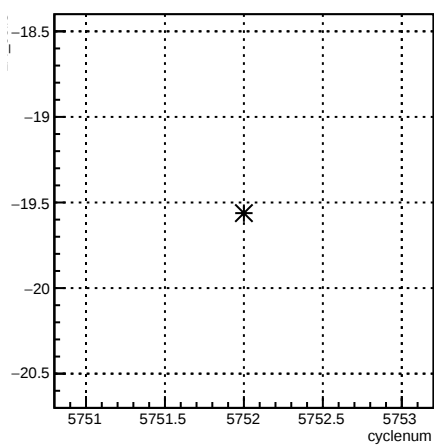
1X_coil3:cyclenum {run == 6208}
