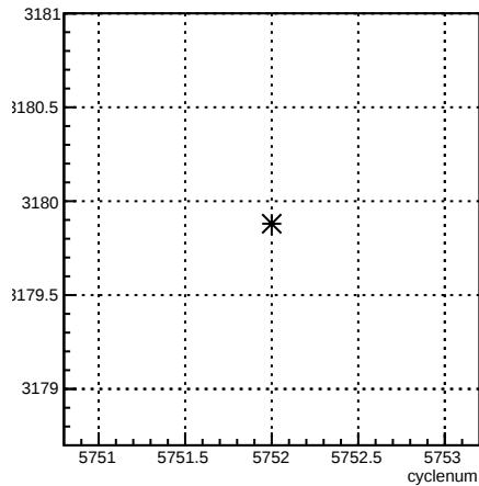
usl_coil3:cyclenum {run == 6208}
