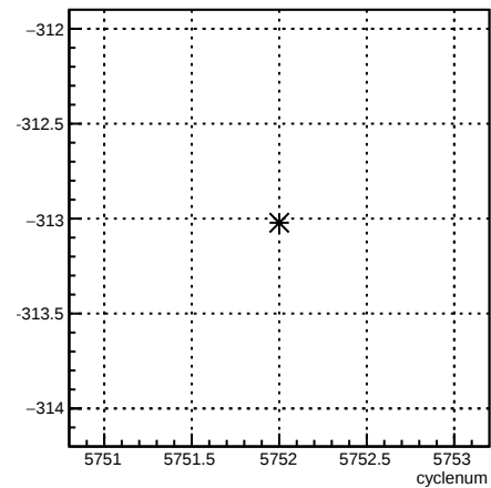
4eX_coil1:cyclenum {run == 6208}
