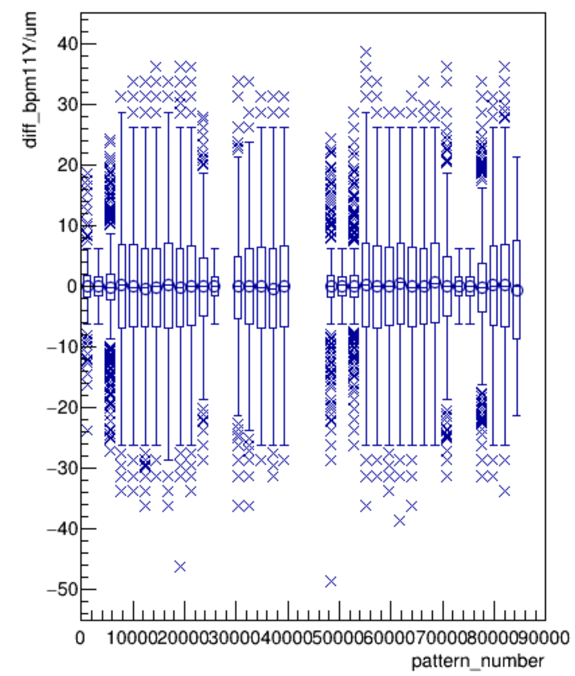
diff_bpm11Y/um:pattern_number {ErrorFlag==0}
