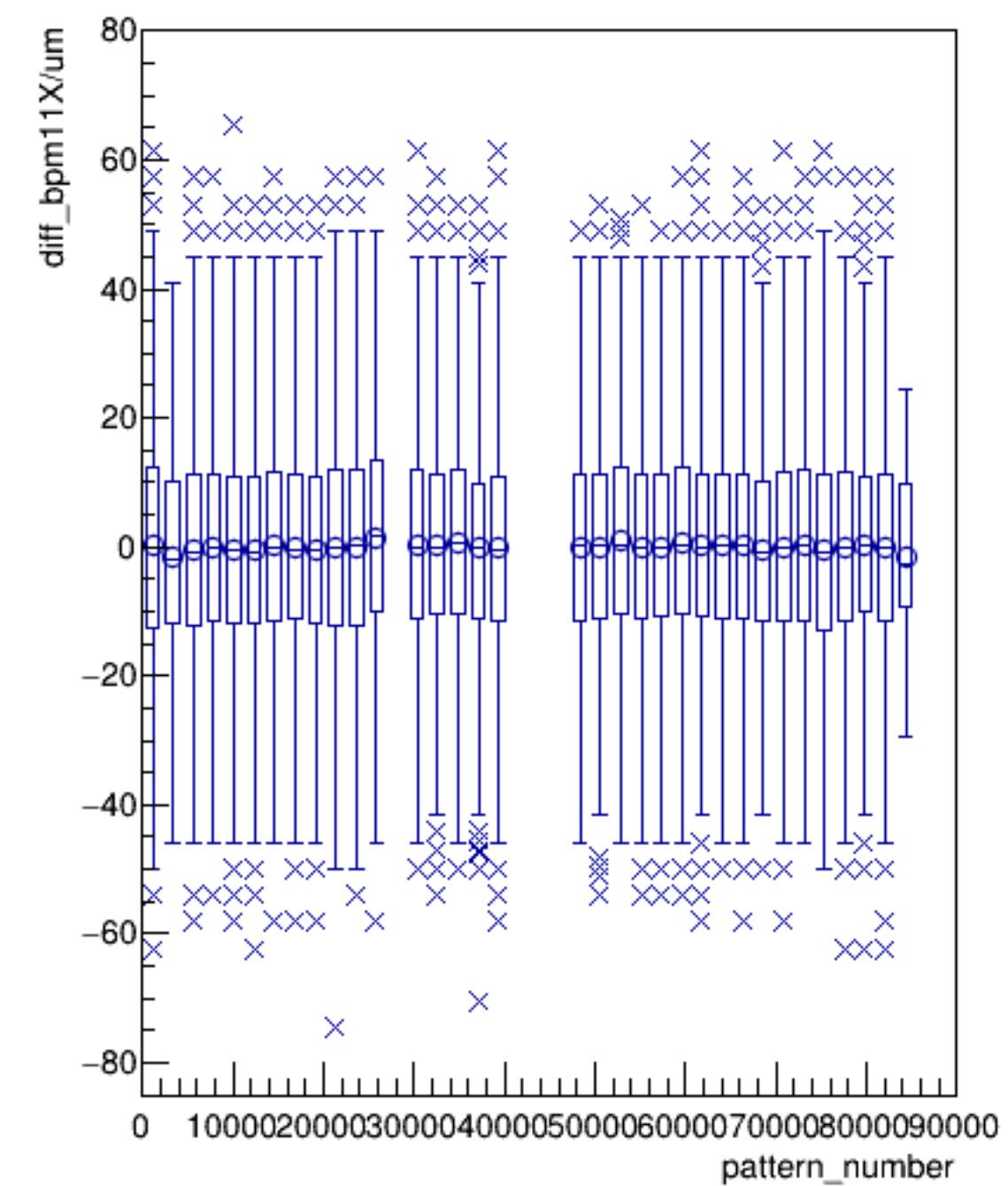
diff_bpm11X/um:pattern_number {ErrorFlag==0}
