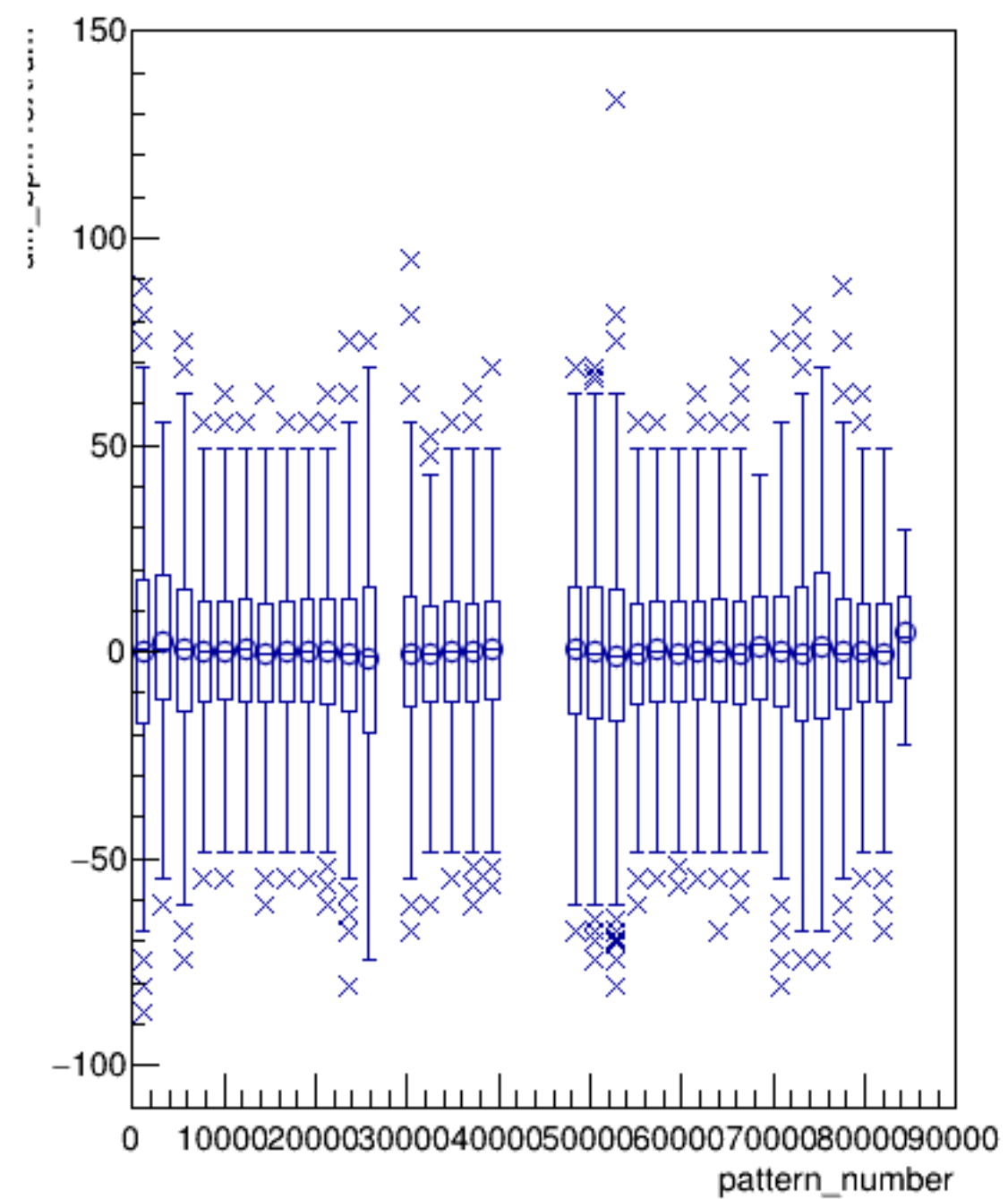
diff_bpm4eX/um:pattern_number {ErrorFlag==0}
