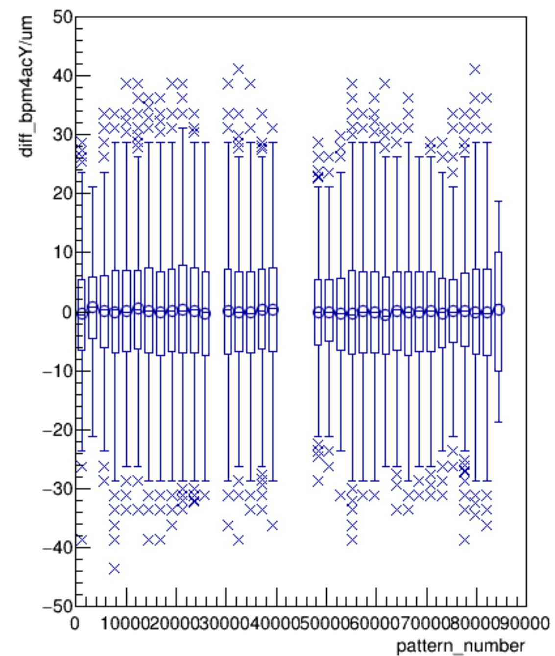
diff_bpm4acY/um:pattern_number {ErrorFlag==0}
