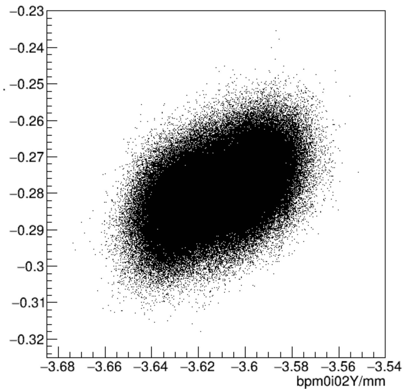
bpm0i02X/mm:bpm0i02Y/mm {ErrorFlag==0}
