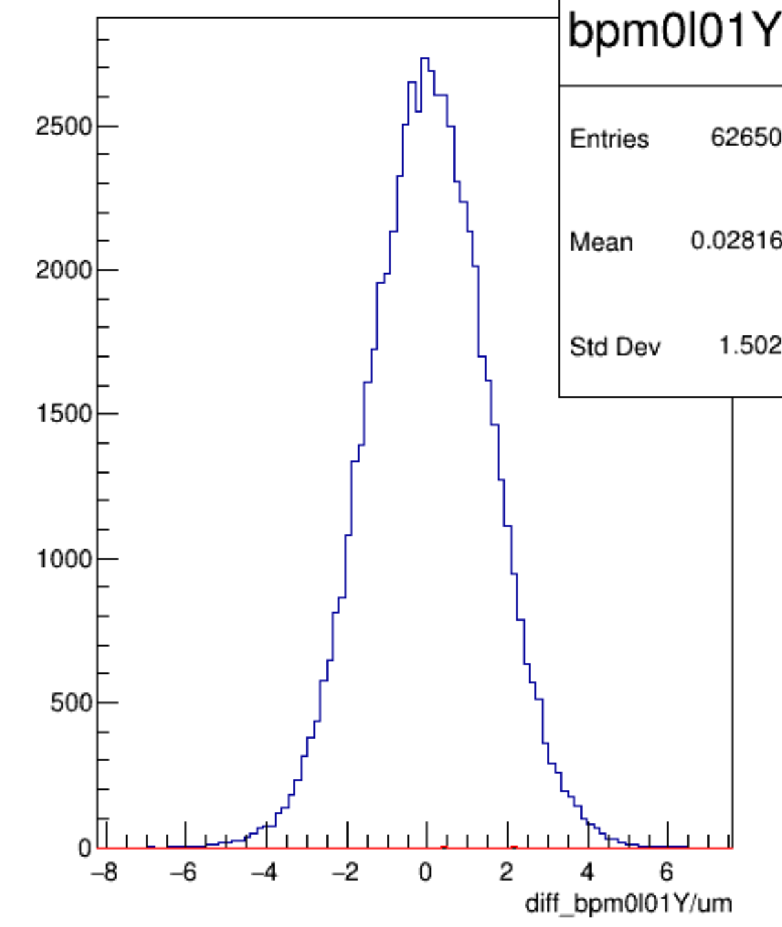
diff_bpm0l01Y/um {ErrorFlag==0}
