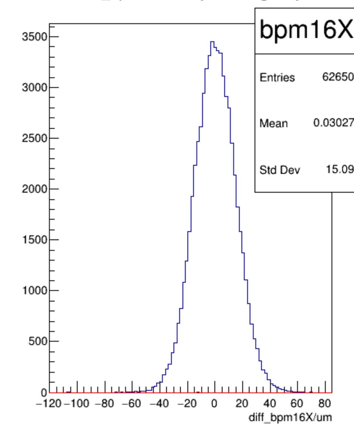
diff_bpm16X/um {ErrorFlag==0}
