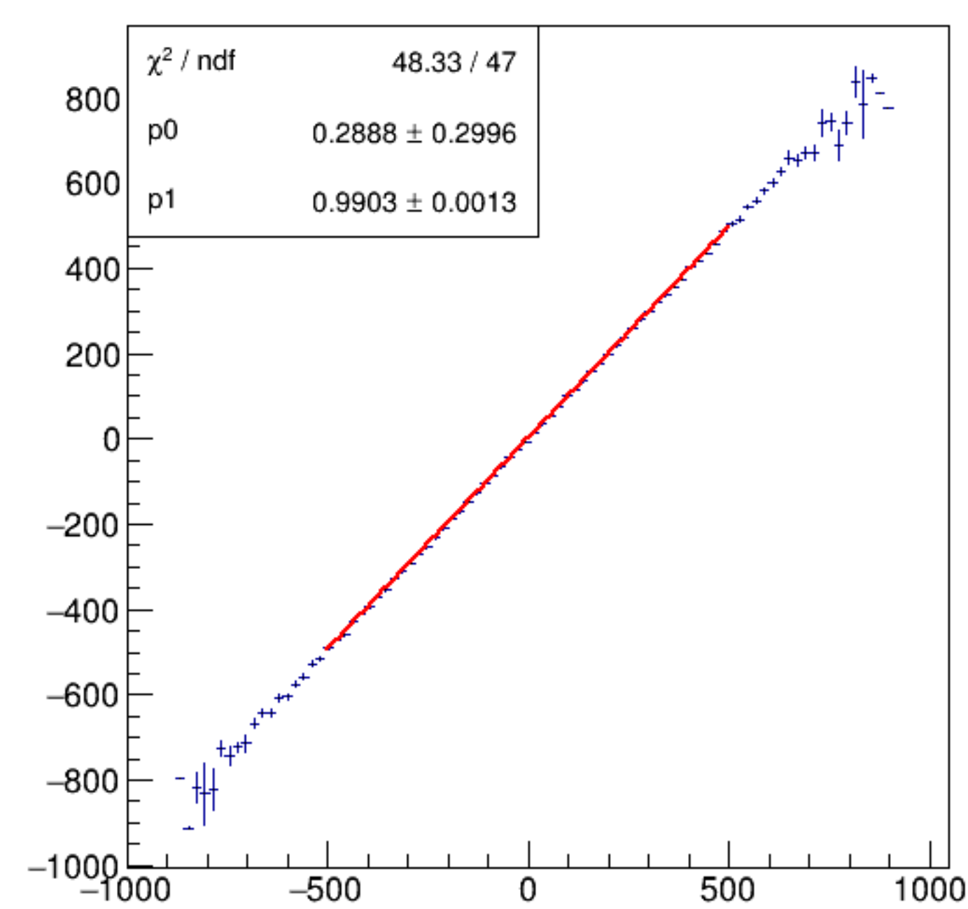
asym_bpm11WS/ppm:Aq/ppm {ErrorFlag==0}
