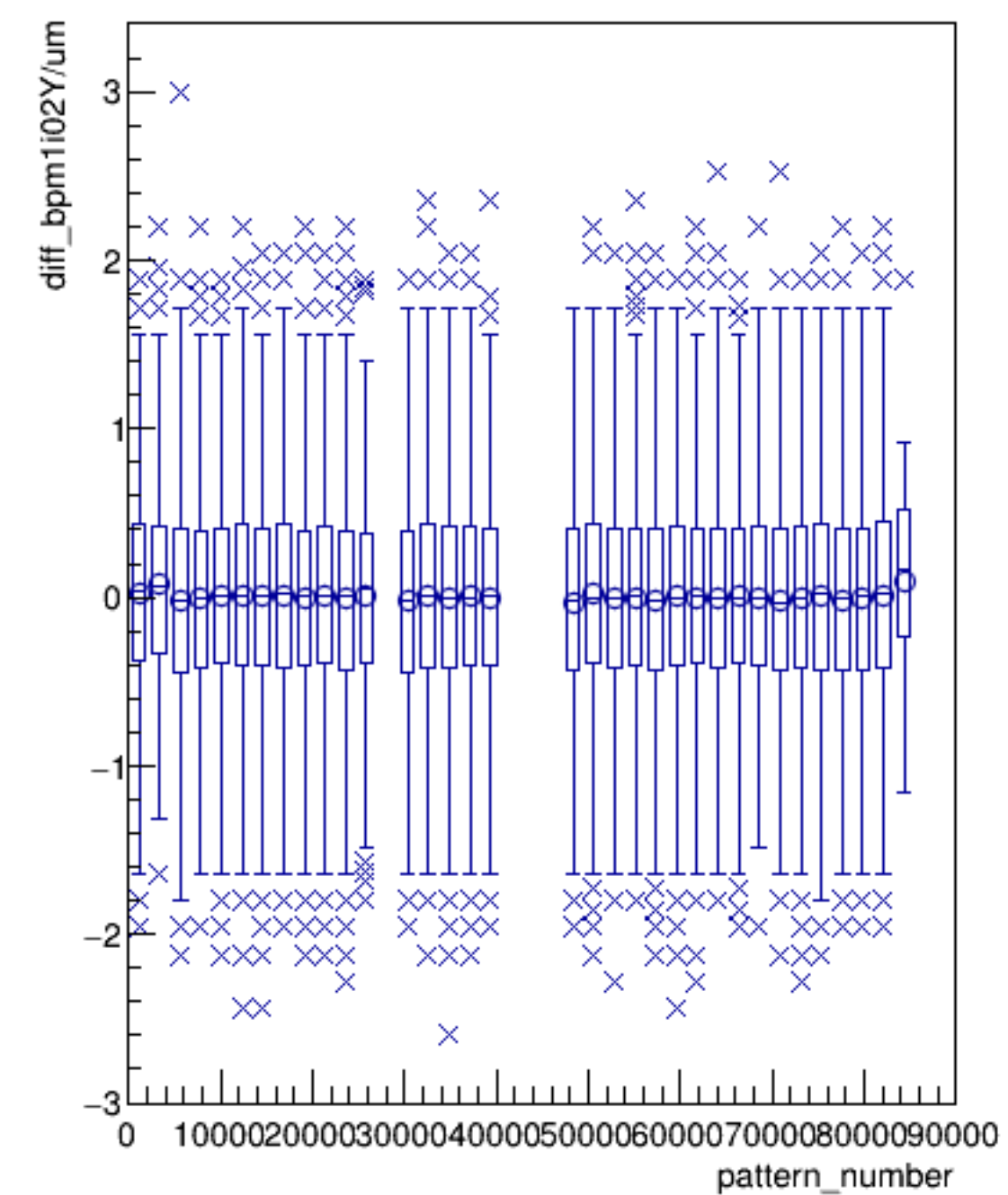
diff_bpm1i02Y/um:pattern_number (ErrorFlag==0)
