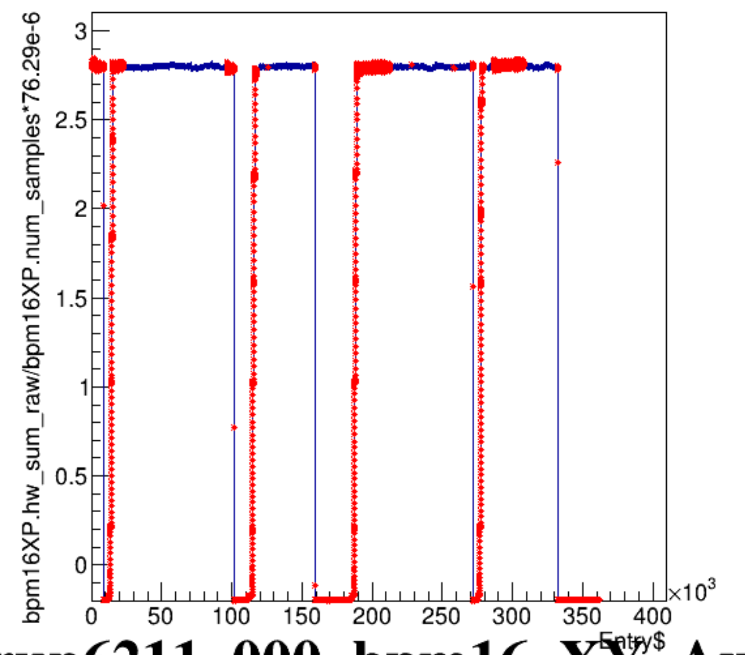
bpm16XP.hw_sum_raw/bpm16XP.num_samples*76.29e-6:Entry$
