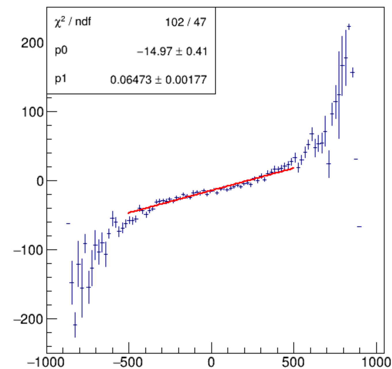
asym_bpm2i01WS/ppm:Aq/ppm {ErrorFlag==0}
