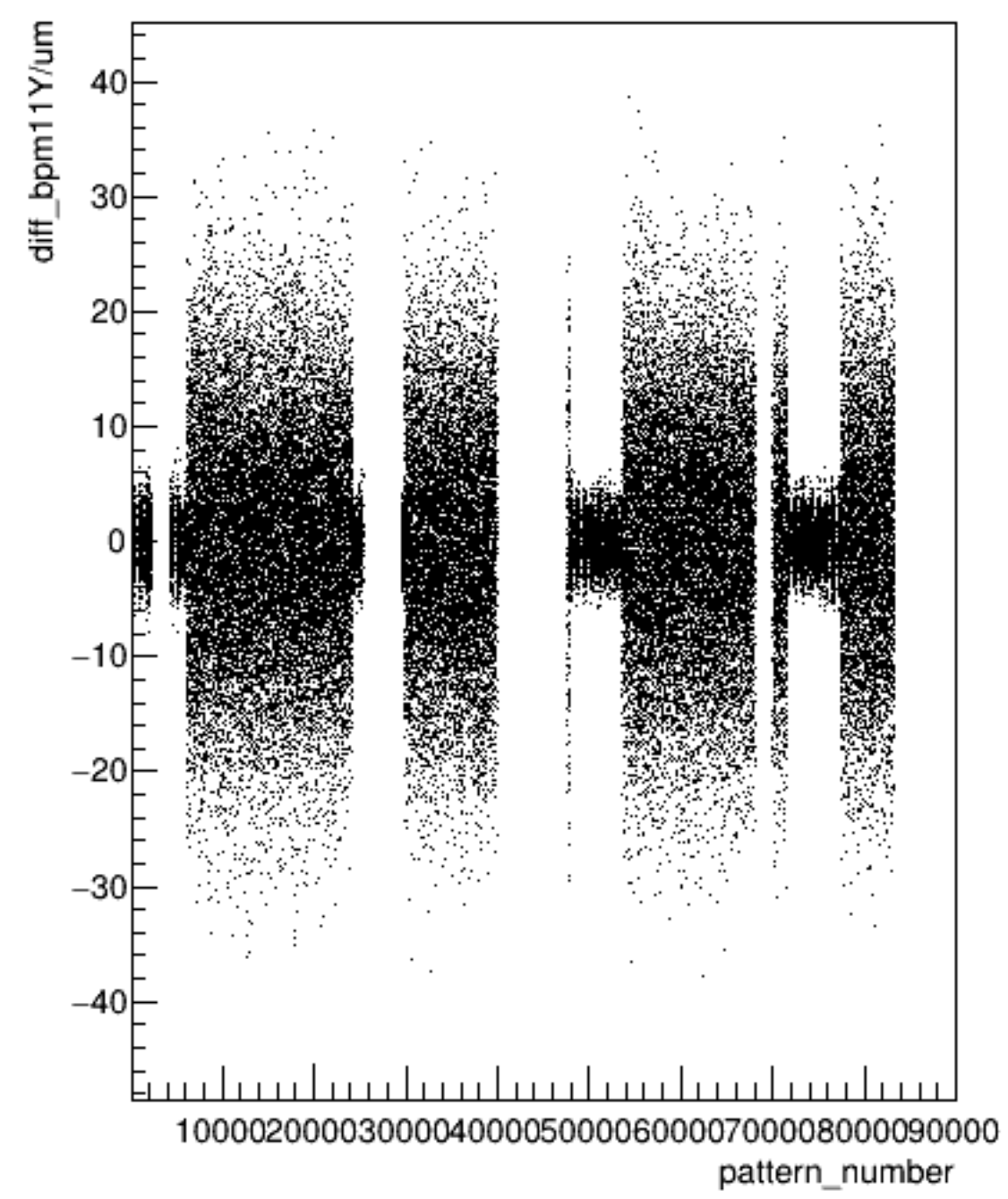
diff_bpm11Y/um:pattern_number {ErrorFlag==0}
