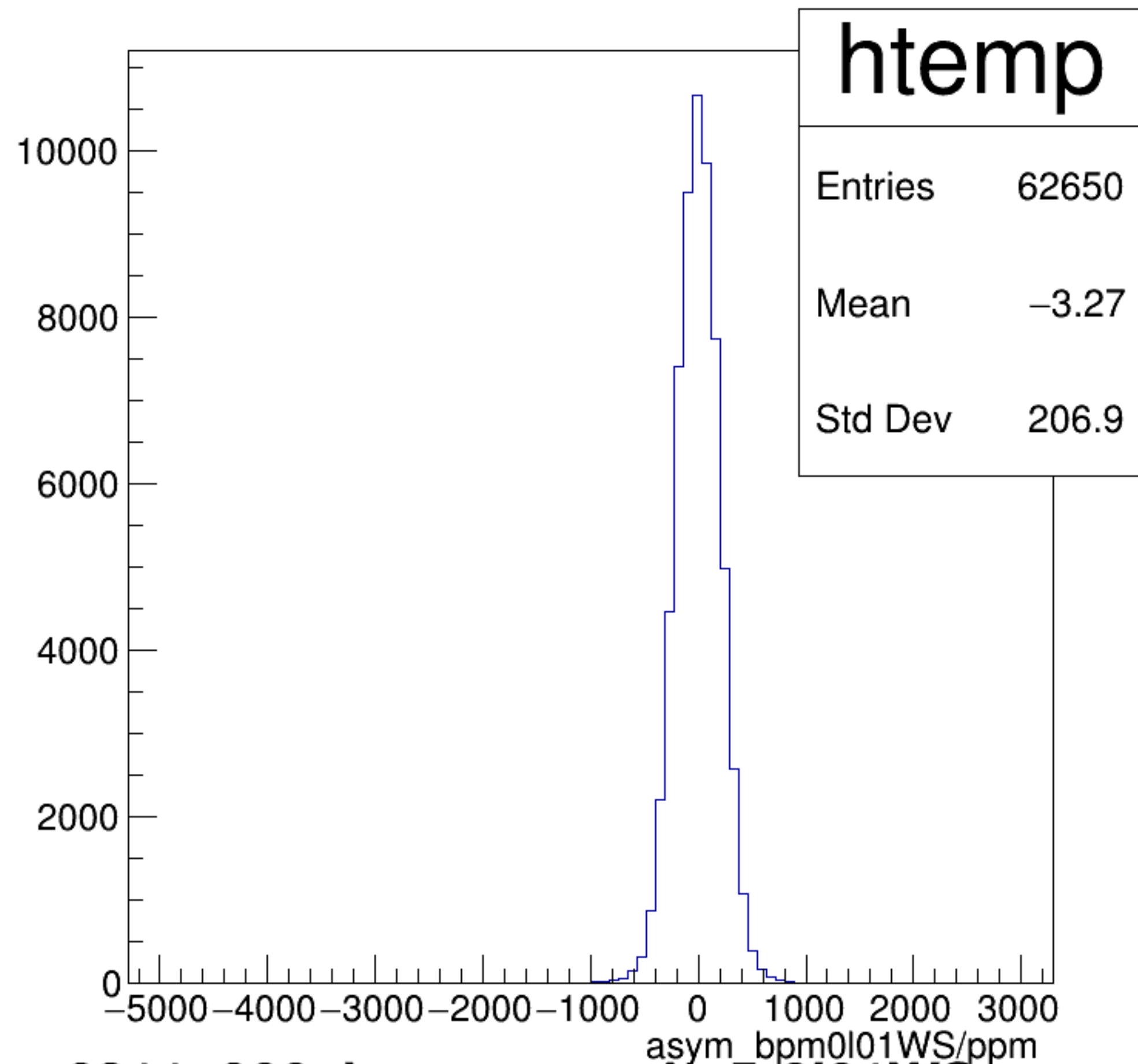
asym_bpm0l01WS/ppm {ErrorFlag==0}
