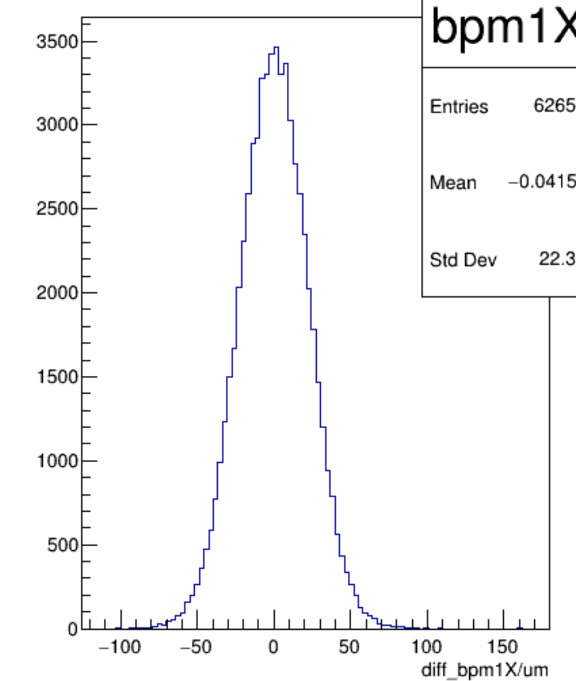
diff_bpm1X/um {ErrorFlag==0}
