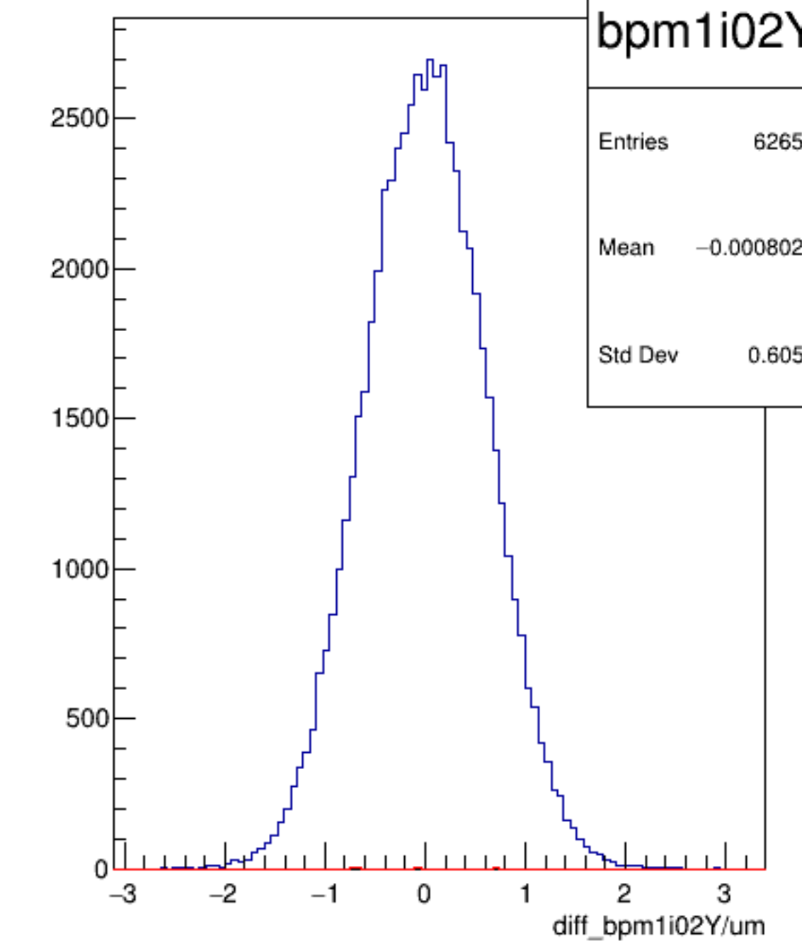
diff_bpm1i02Y/um {ErrorFlag==0}
