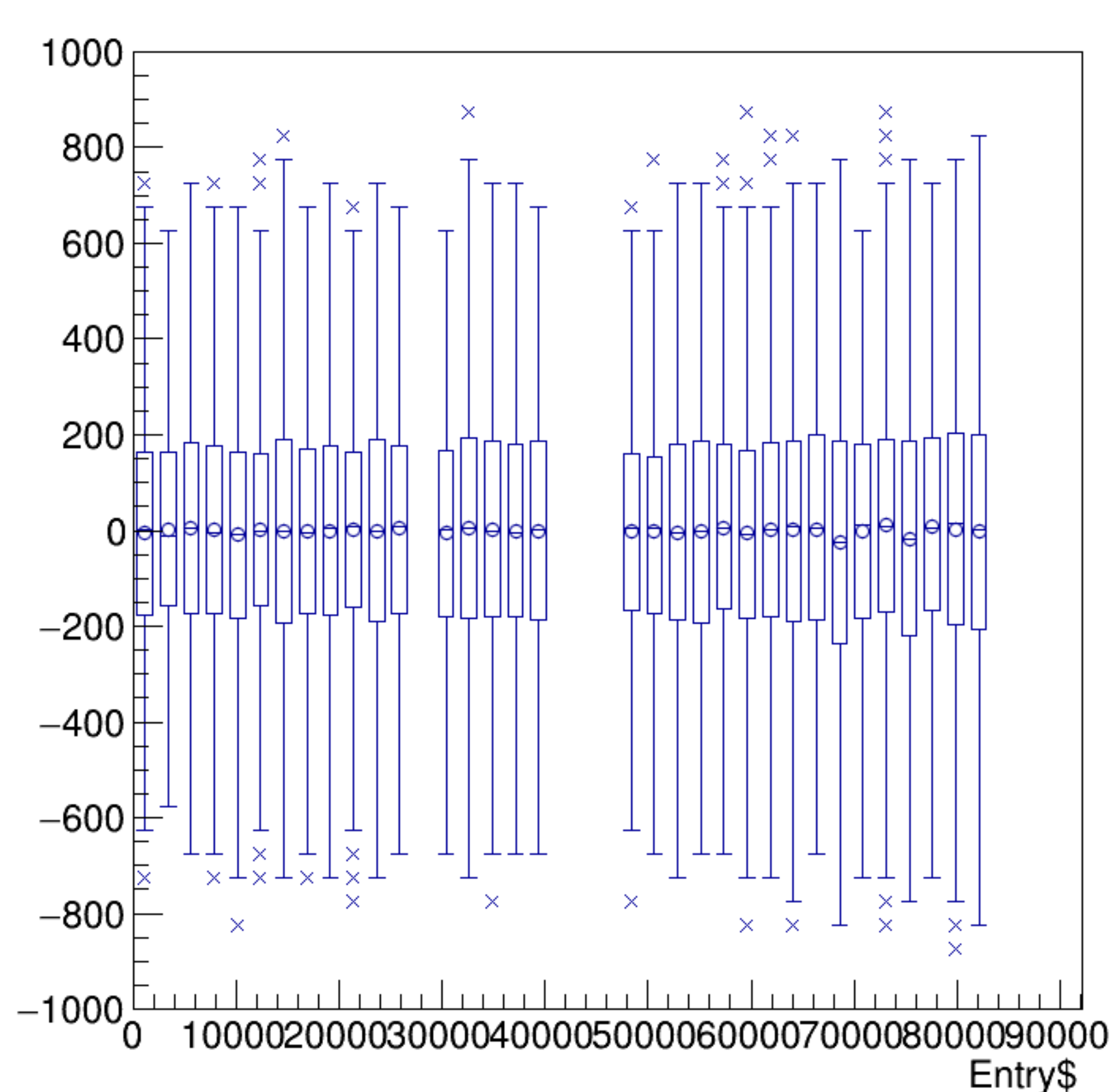
asym_bcm_an_us/ppm:Entry$ {ErrorFlag==0}
