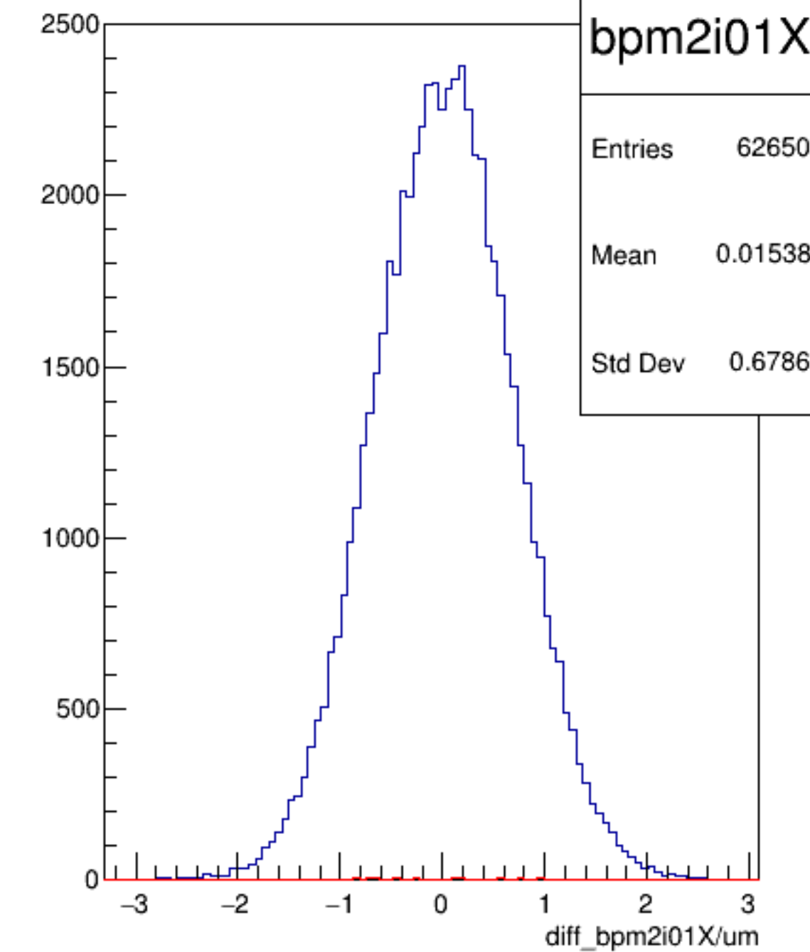
diff_bpm2i01X/um {ErrorFlag==0}
