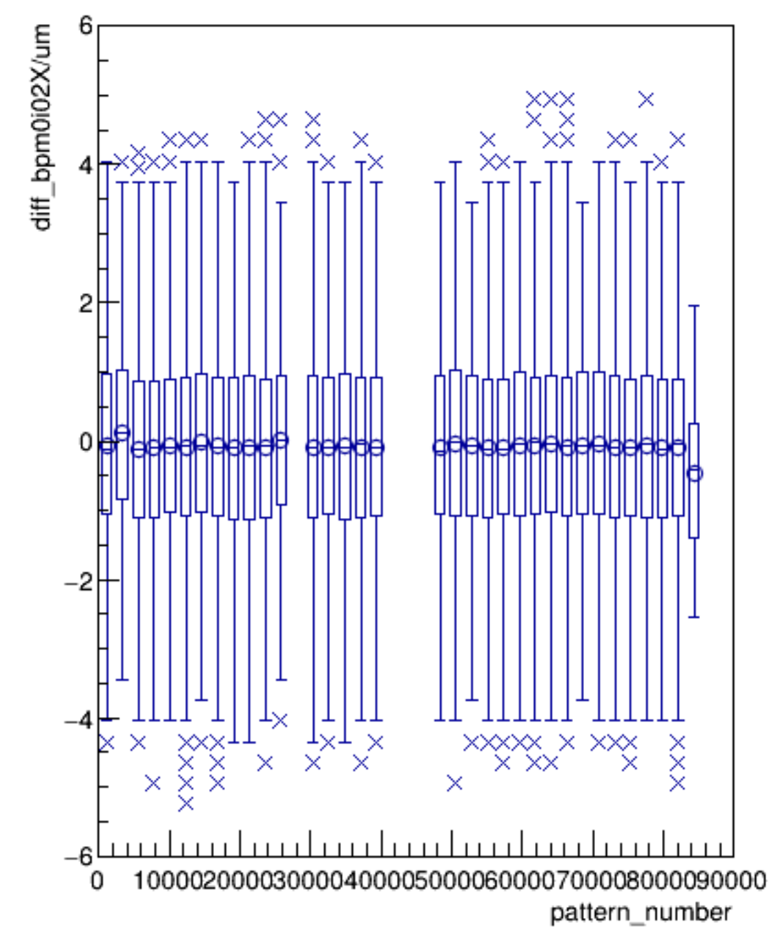
diff_bpm0i02X/um:pattern_number (ErrorFlag==0)
