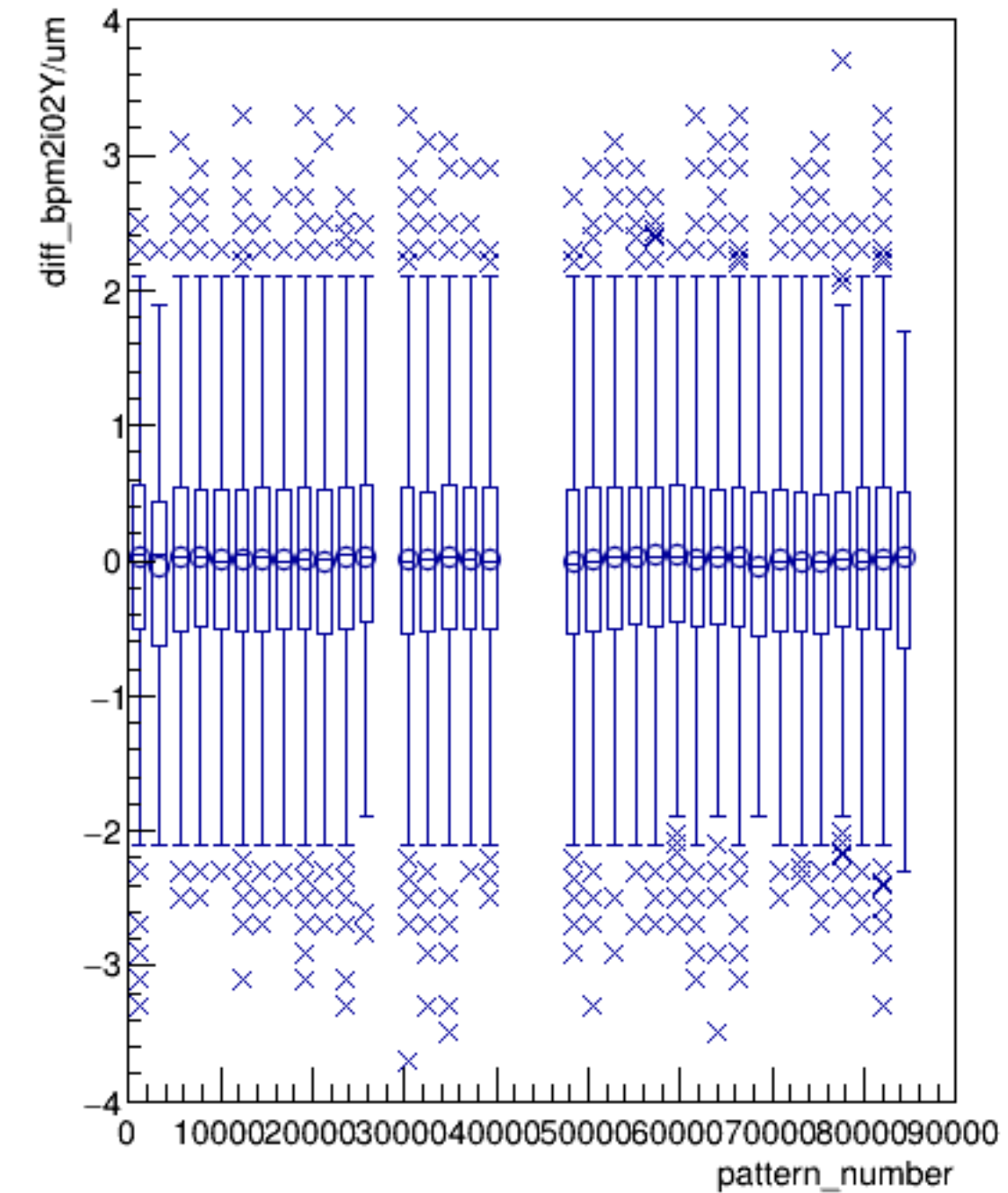
diff_bpm2i02Y/um:pattern_number (ErrorFlag==0)
