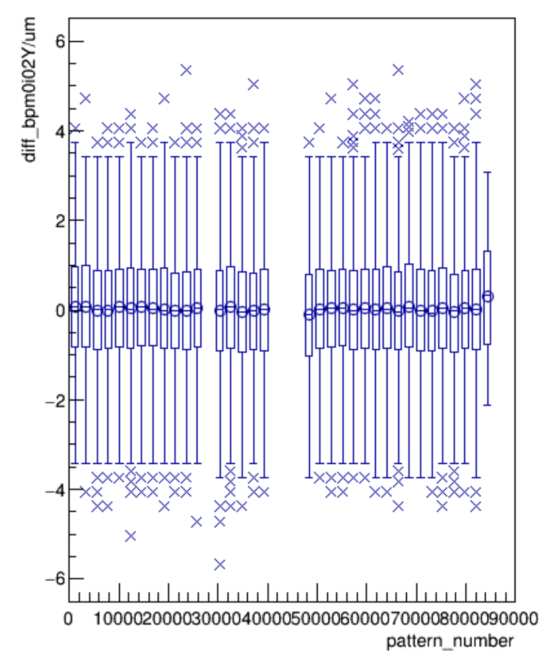
diff_bpm0i02Y/um:pattern_number (ErrorFlag==0)
