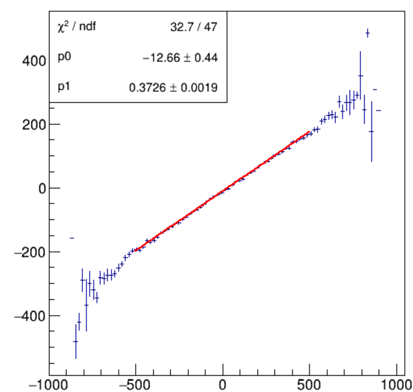
asym_bpm0i02WS/ppm:Aq/ppm {ErrorFlag==0}
