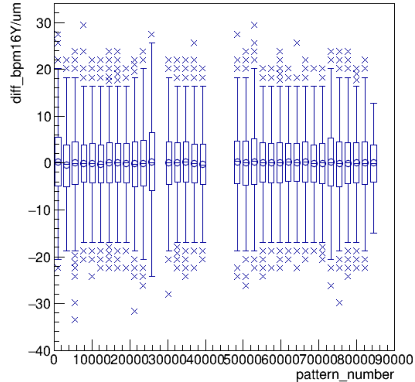
diff_bpm16Y/um:pattern_number {ErrorFlag==0}
