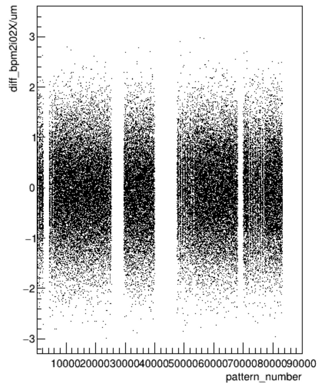
diff_bpm2i02X/um:pattern_number (ErrorFlag==0)
