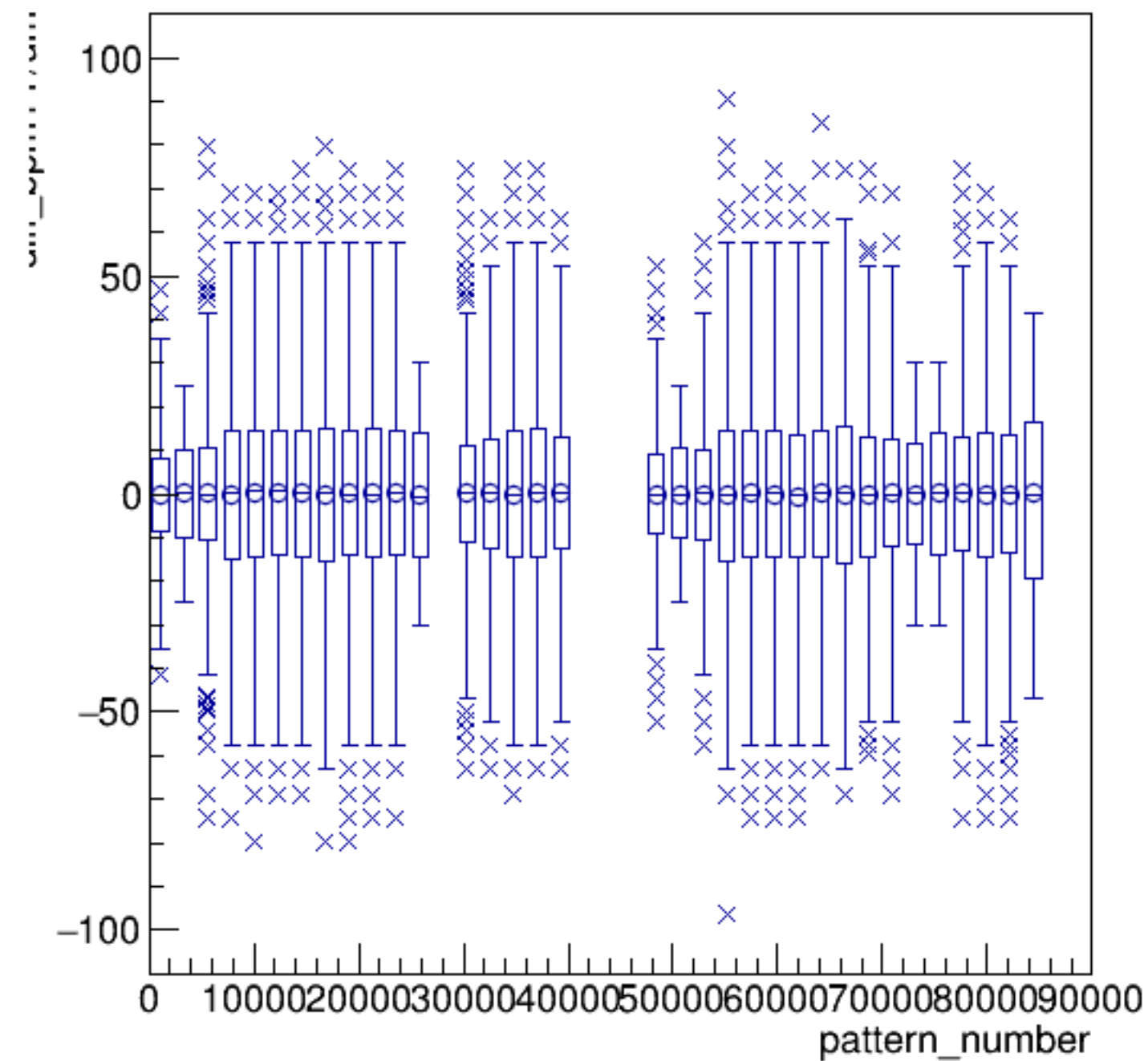
diff_bpm1Y/um:pattern_number {ErrorFlag==0}
