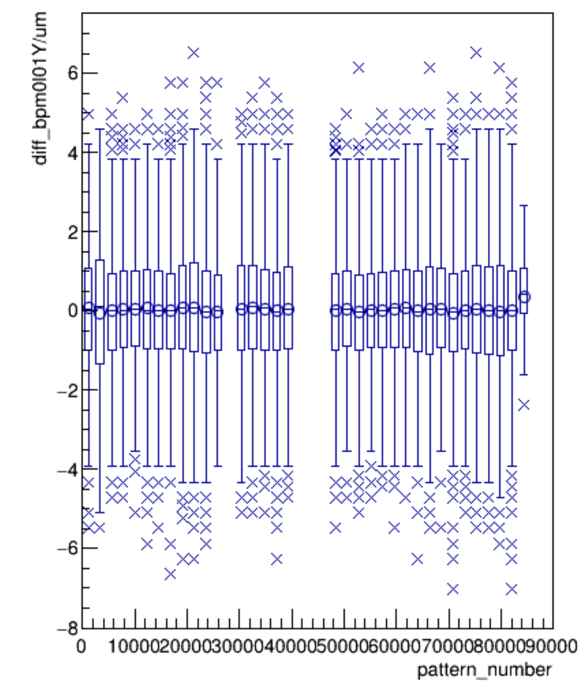
diff_bpm0l01Y/um:pattern_number {ErrorFlag==0}
