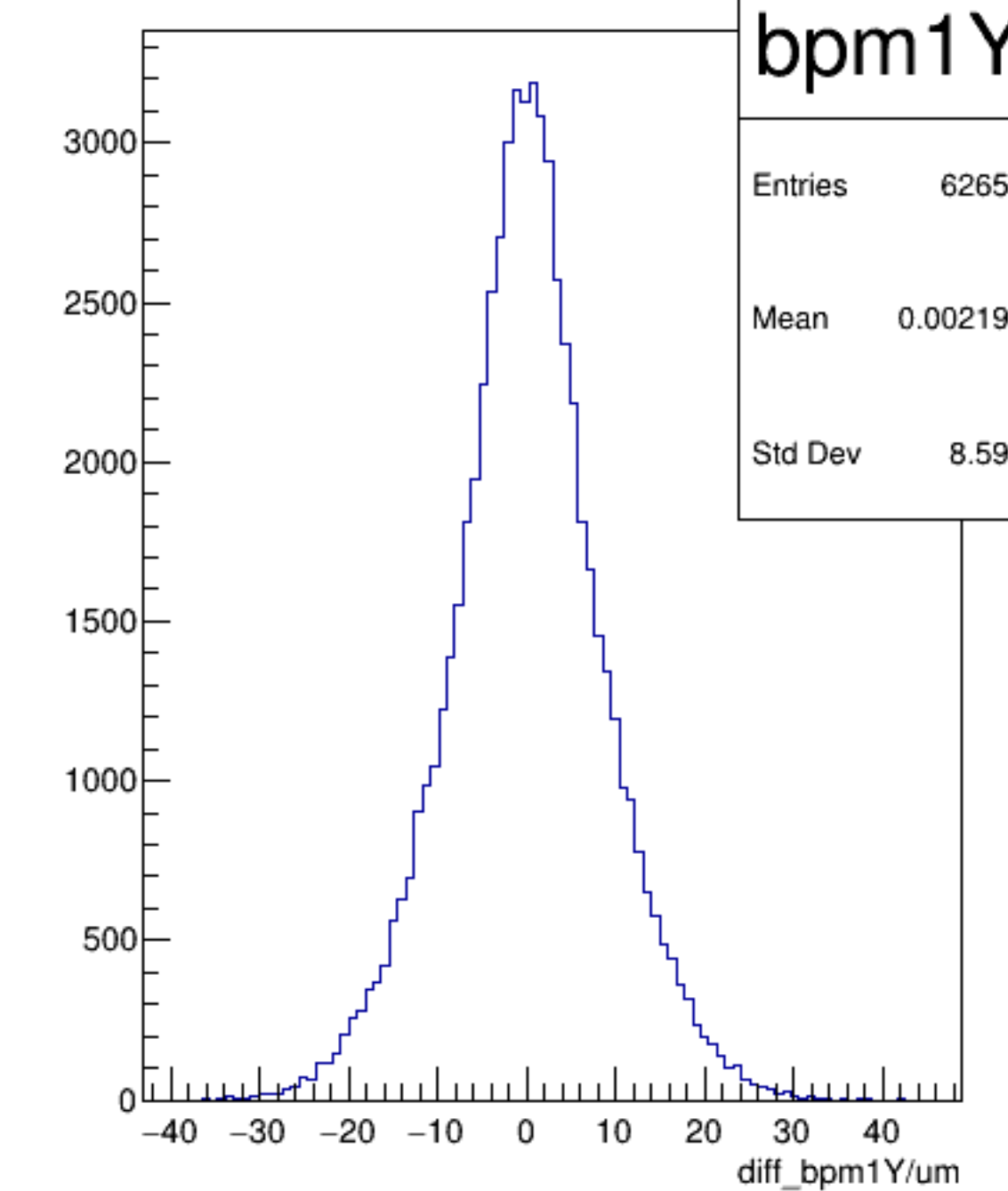
diff_bpm1Y/um {ErrorFlag==0}
