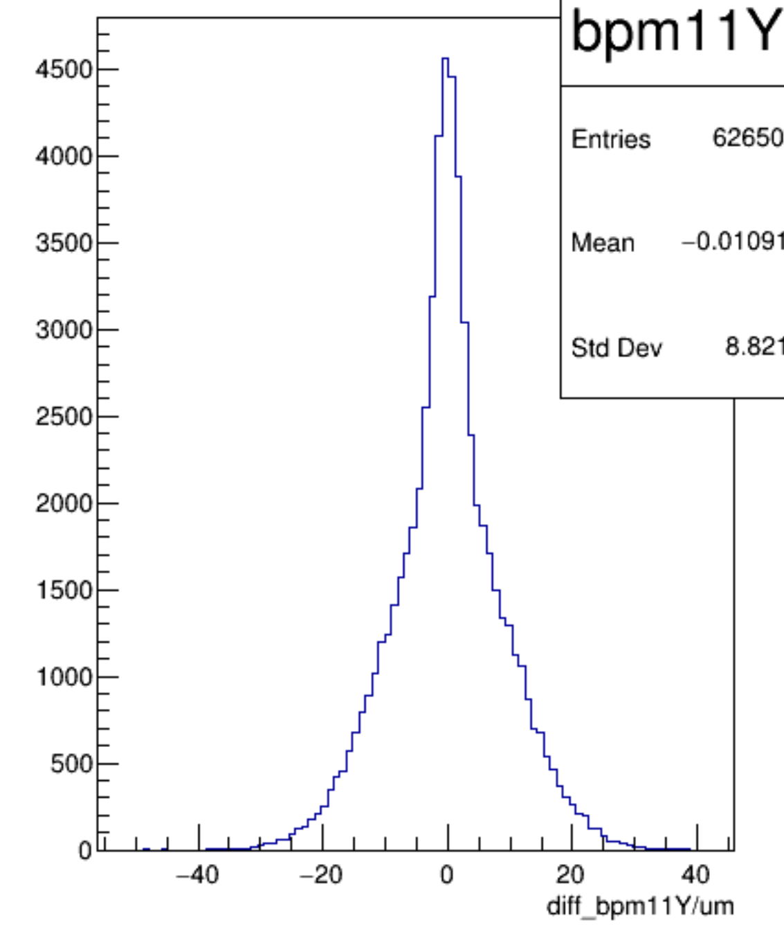
diff_bpm11Y/um {ErrorFlag==0}
