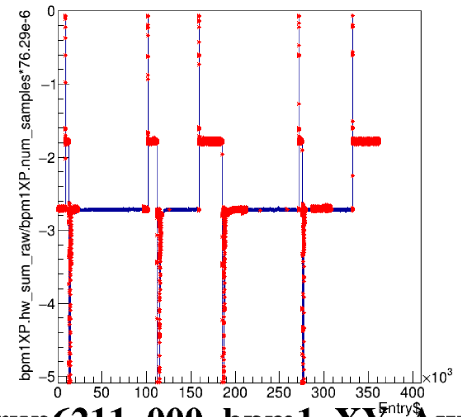
bpm1XP.hw_sum_raw/bpm1XP.num_samples*76.29e-6:Entry$
