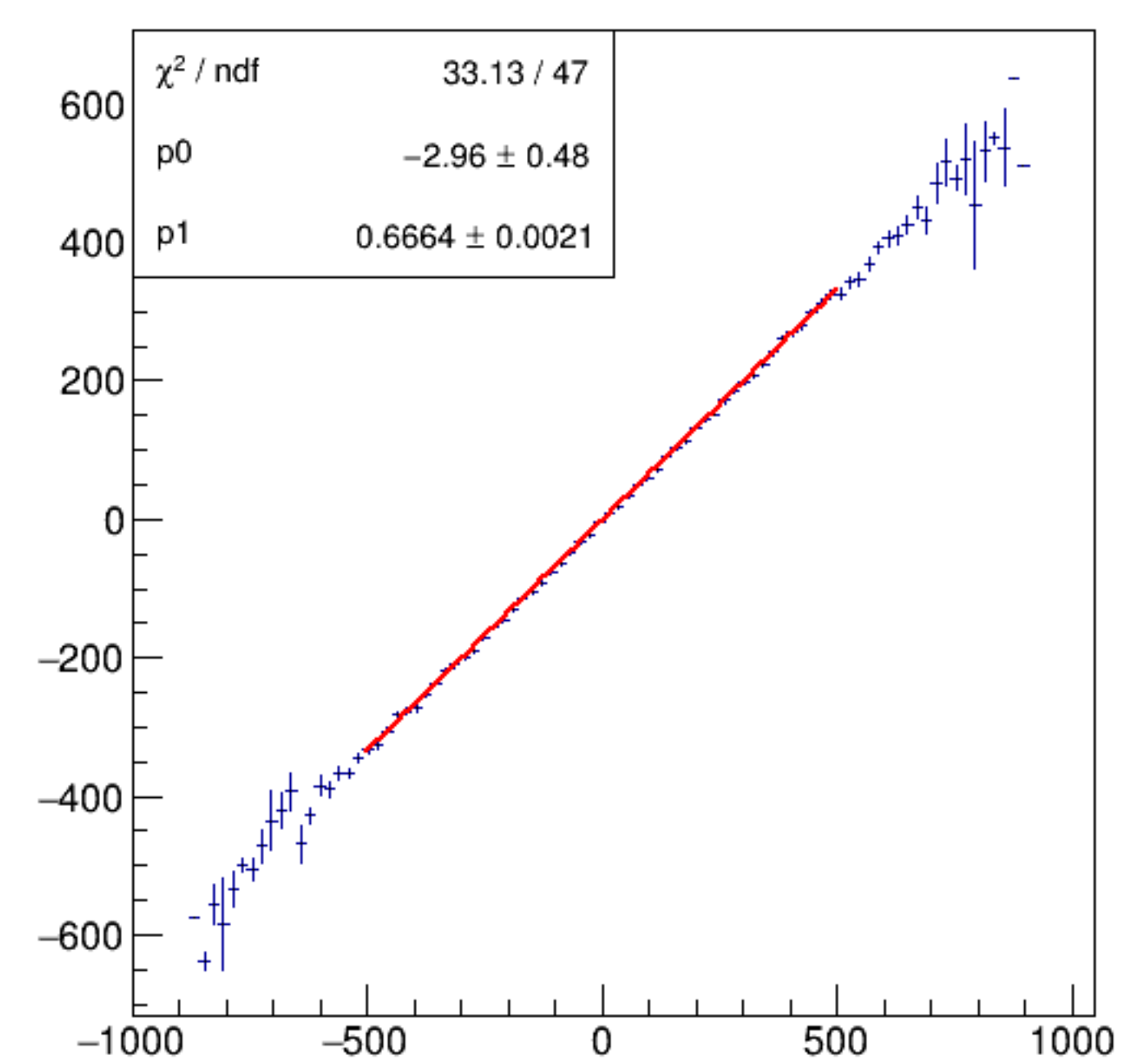
asym_bpm0l01WS/ppm:Aq/ppm {ErrorFlag==0}
