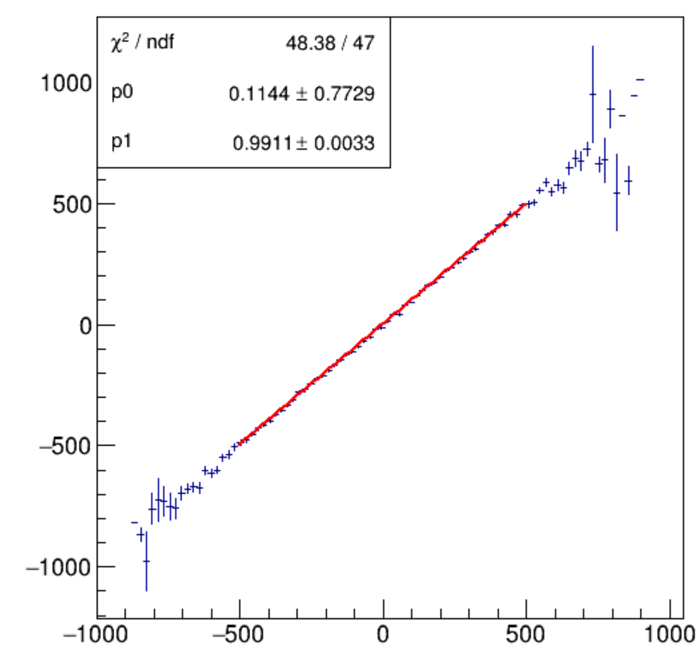
asym_bpm1WS/ppm:Aq/ppm {ErrorFlag==0}
