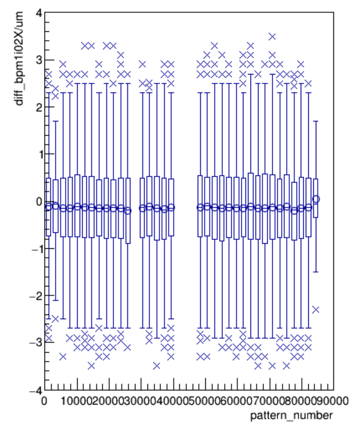
diff_bpm1i02X/um:pattern_number (ErrorFlag==0)
