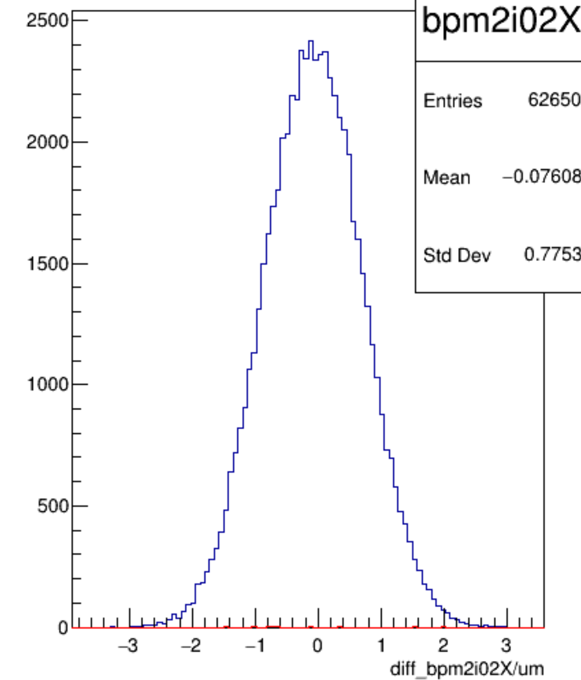
diff_bpm2i02X/um {ErrorFlag==0}
