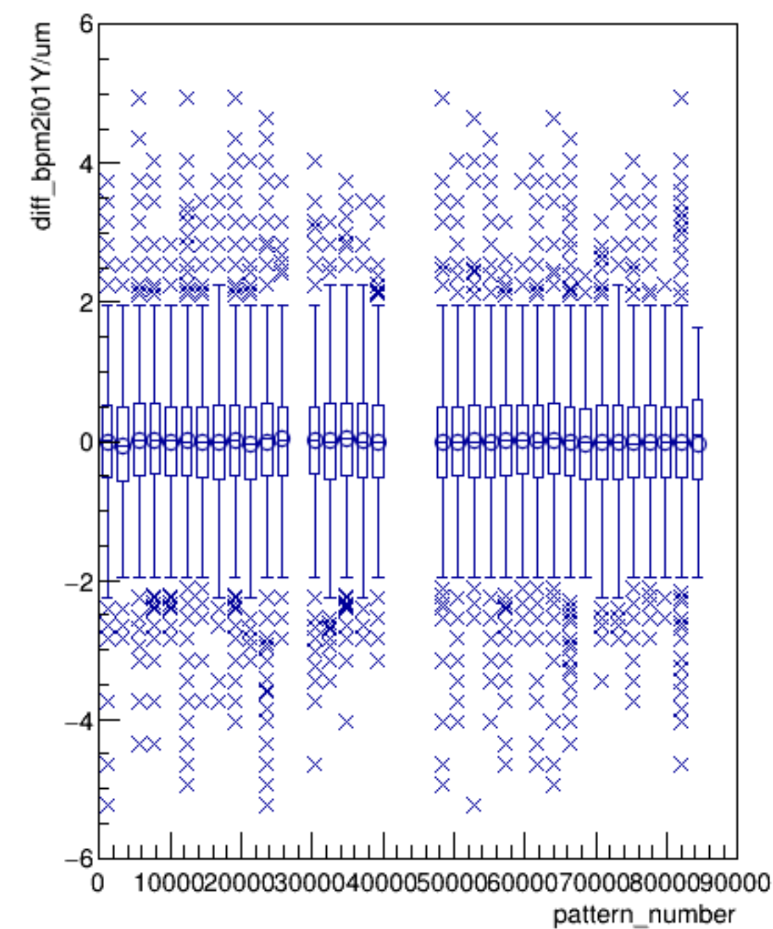
diff_bpm2i01Y/um:pattern_number (ErrorFlag==0)
