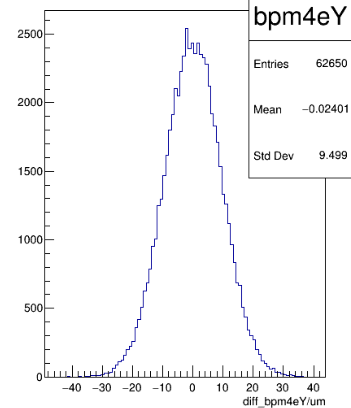
diff_bpm4eY/um {ErrorFlag==0}
