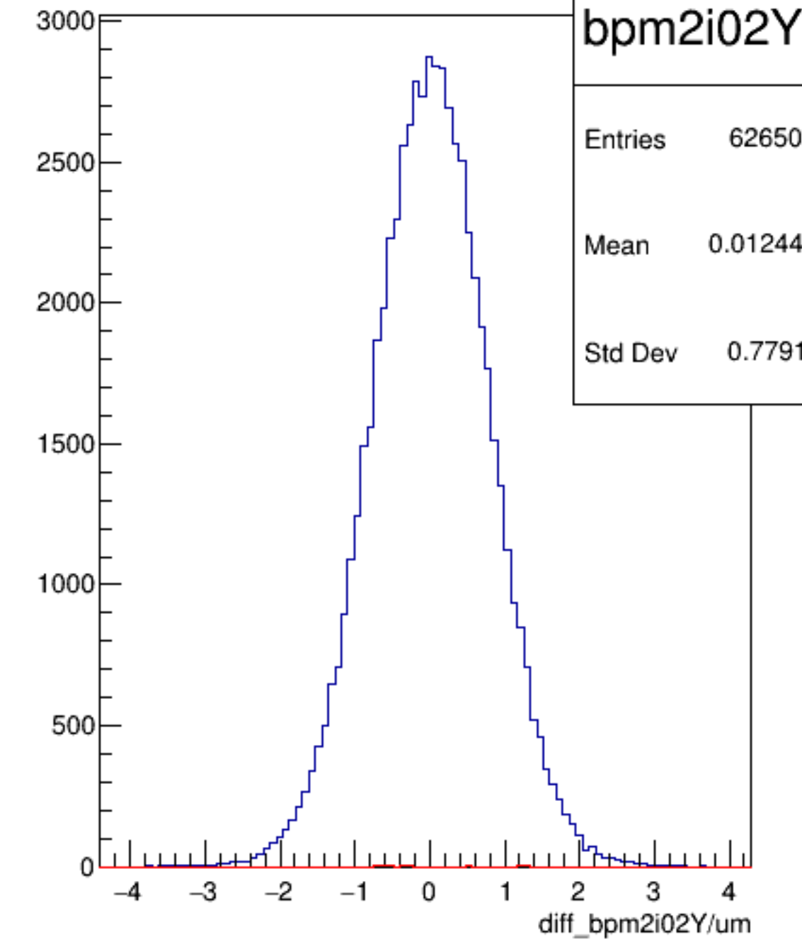
diff_bpm2i02Y/um {ErrorFlag==0}
