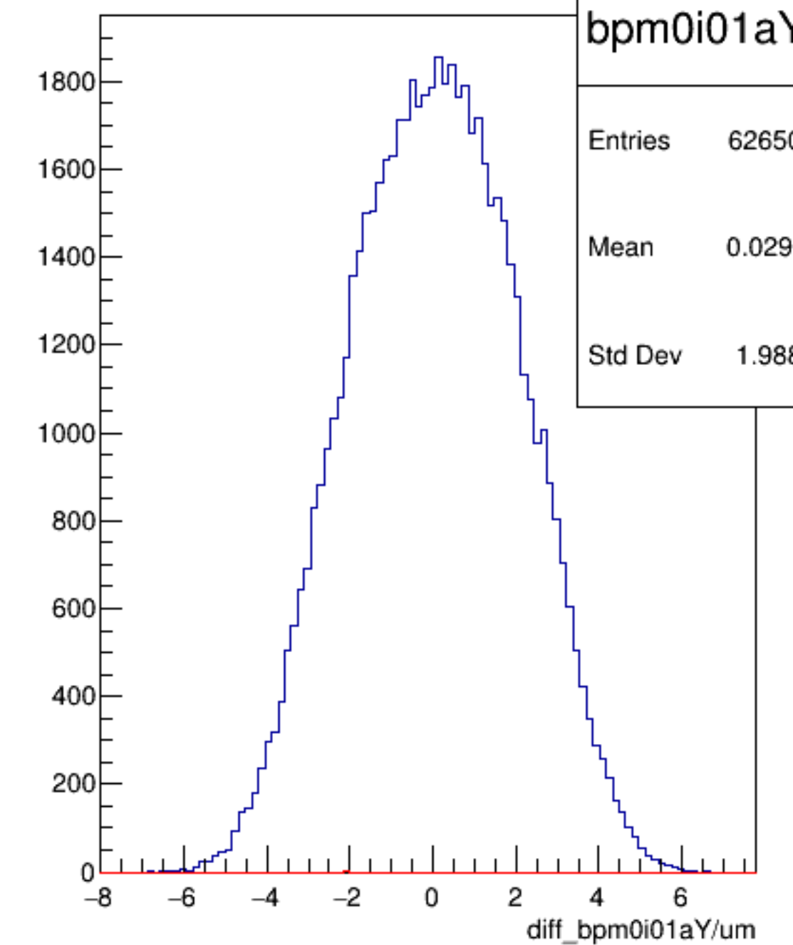
diff_bpm0i01aY/um {ErrorFlag==0}
