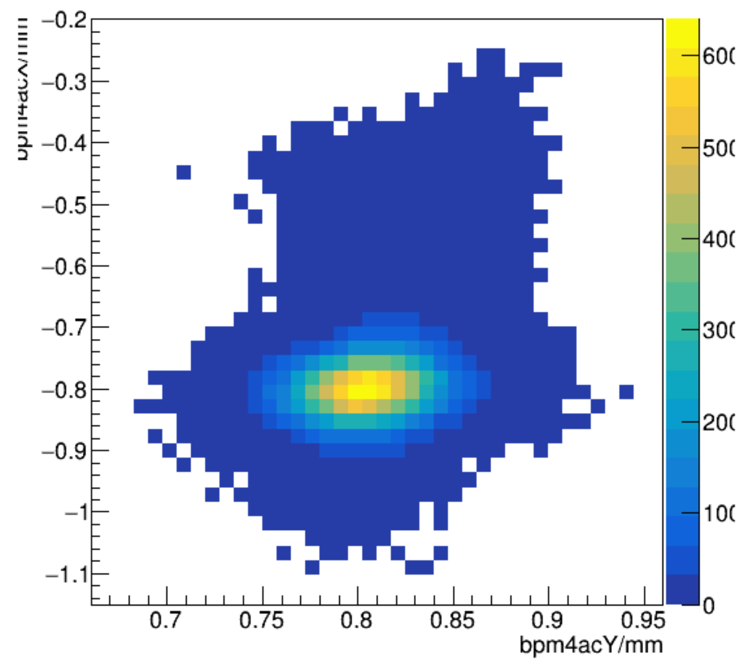
bpm4acX/mm:bpm4acY/mm {ErrorFlag==0}
