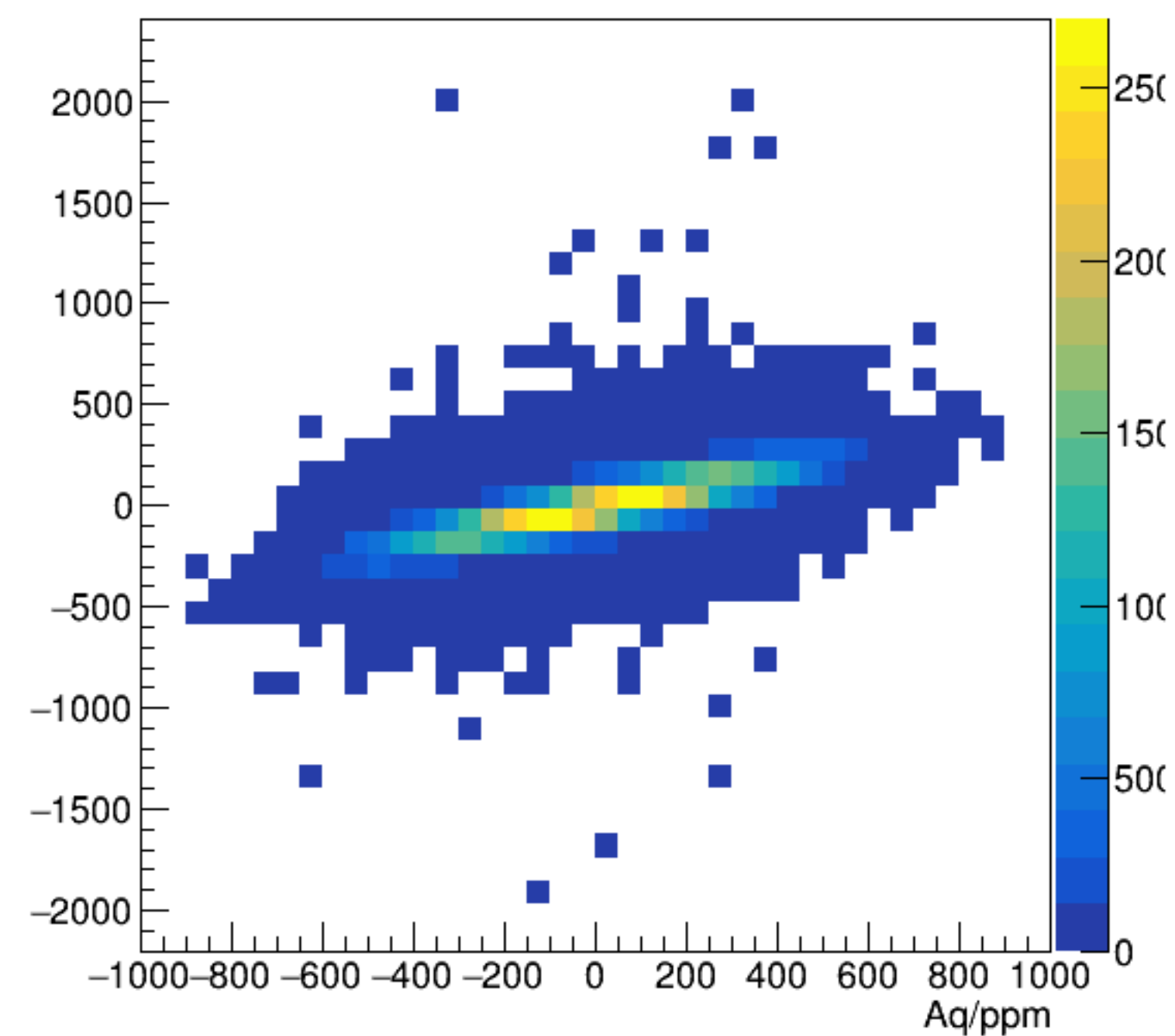
asym_bpm0i01aWS/ppm:Aq/ppm {ErrorFlag==0}
