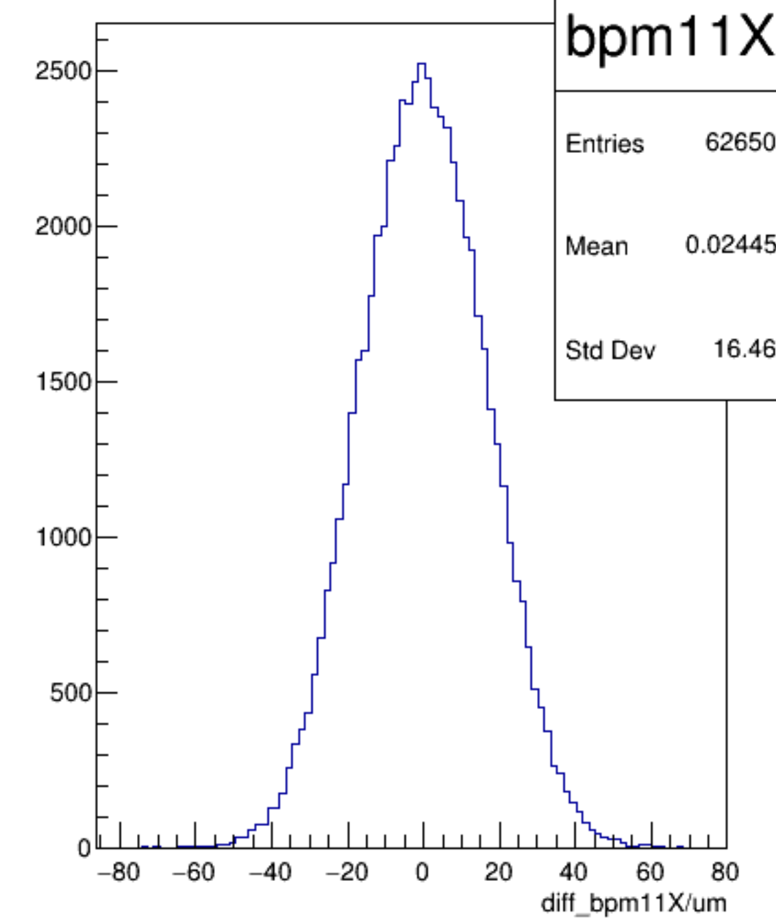
diff_bpm11X/um {ErrorFlag==0}
