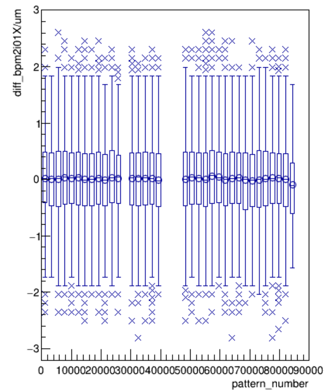
diff_bpm2i01X/um:pattern_number (ErrorFlag==0)
