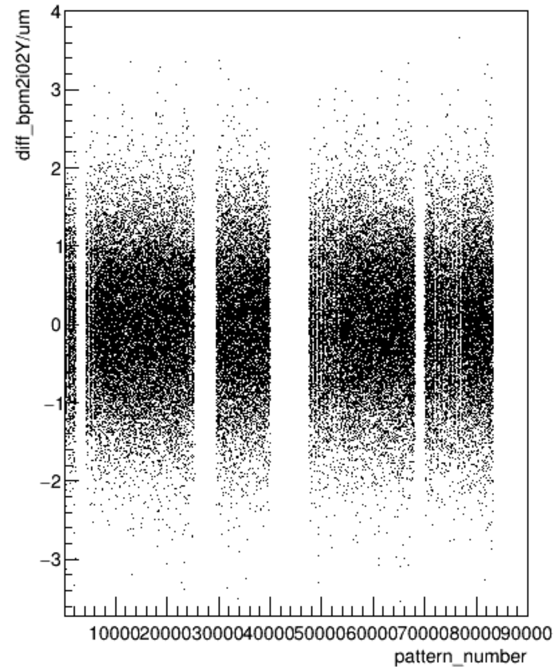
diff_bpm2i02Y/um:pattern_number (ErrorFlag==0)
