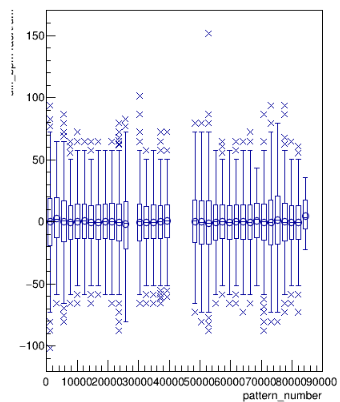
diff_bpm4acX/um:pattern_number {ErrorFlag==0}
