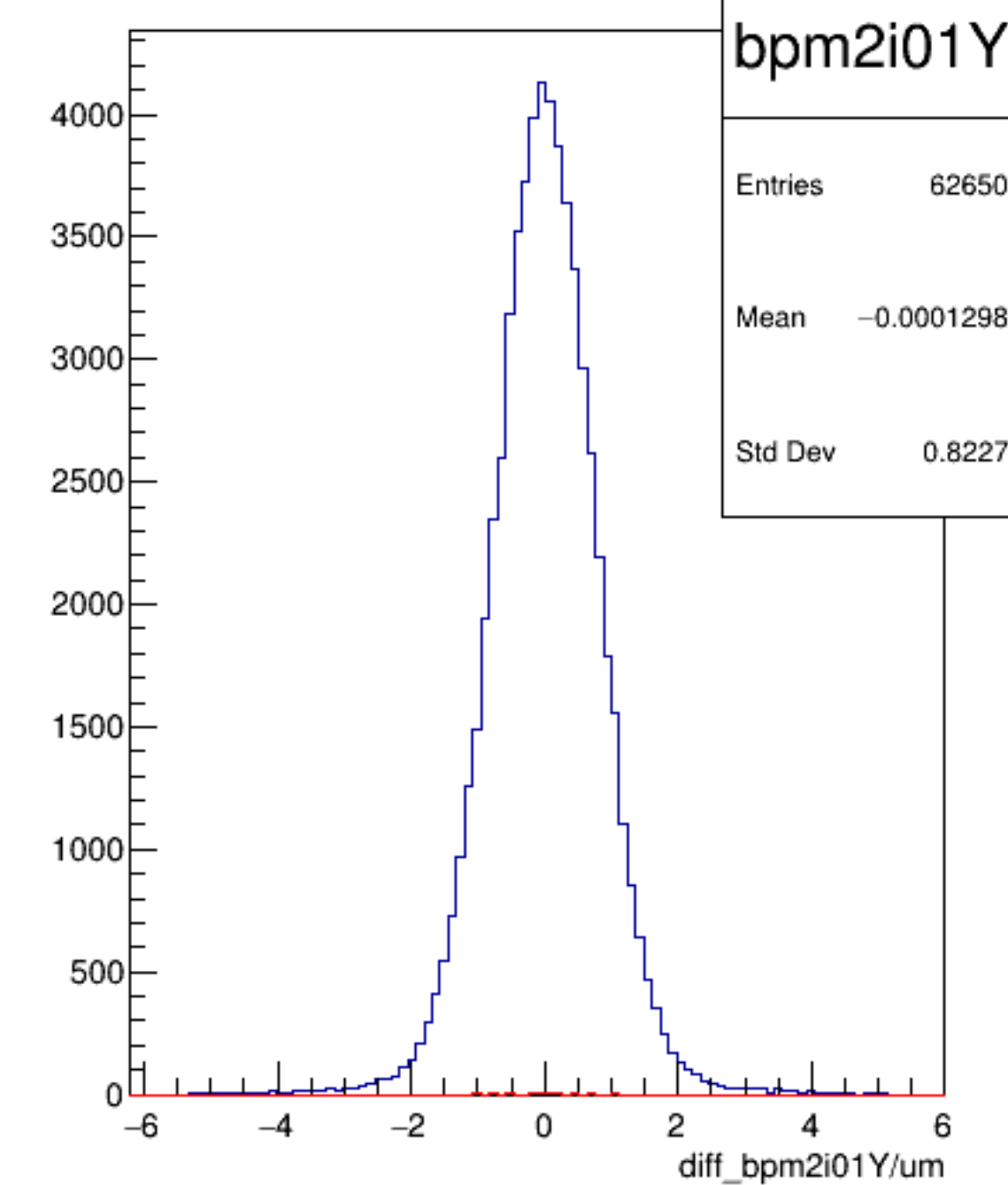
diff_bpm2i01Y/um {ErrorFlag==0}
