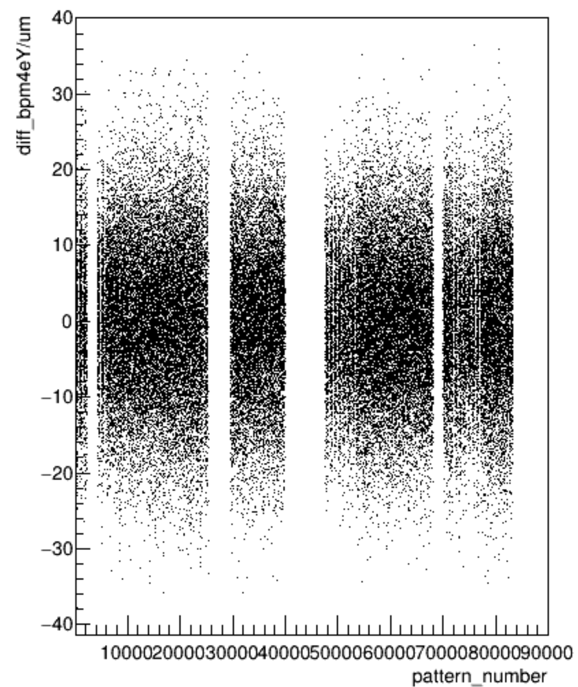
diff_bpm4eY/um:pattern_number {ErrorFlag==0}
