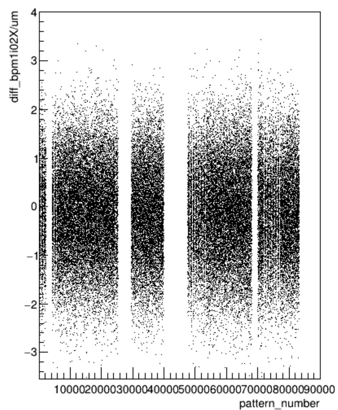
diff_bpm1i02X/um:pattern_number (ErrorFlag==0)
