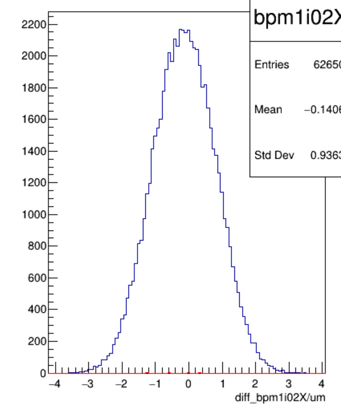
diff_bpm1i02X/um {ErrorFlag==0}
