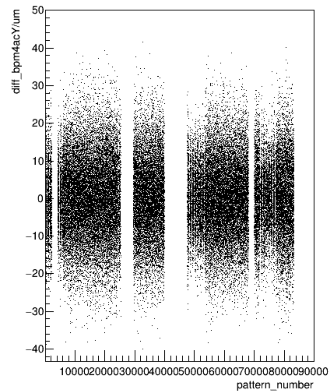
diff_bpm4acY/um:pattern_number {ErrorFlag==0}
