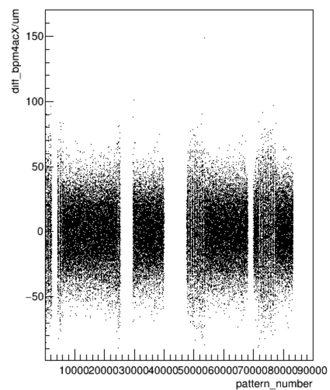
diff_bpm4acX/um:pattern_number {ErrorFlag==0}
