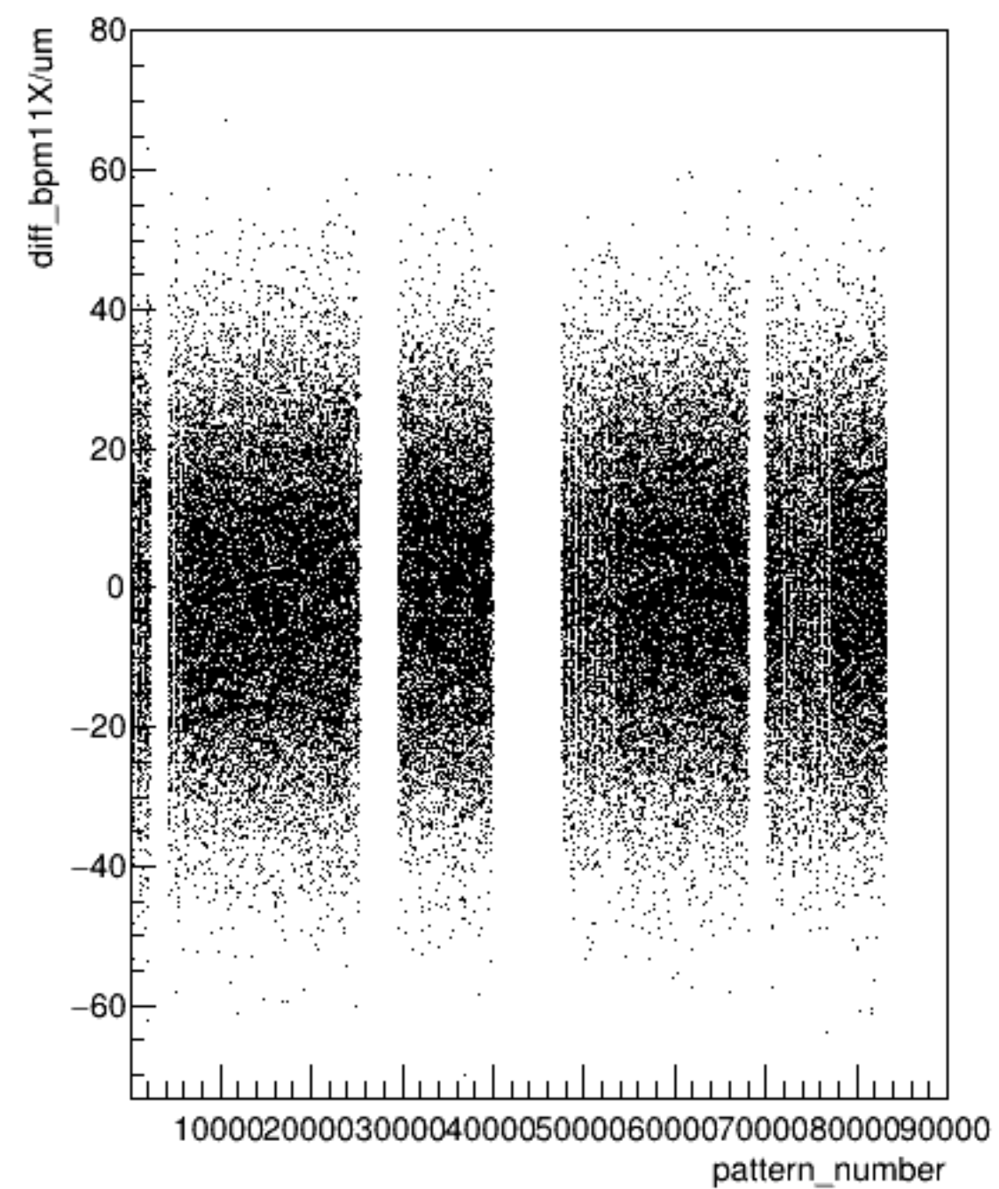
diff_bpm11X/um:pattern_number {ErrorFlag==0}
