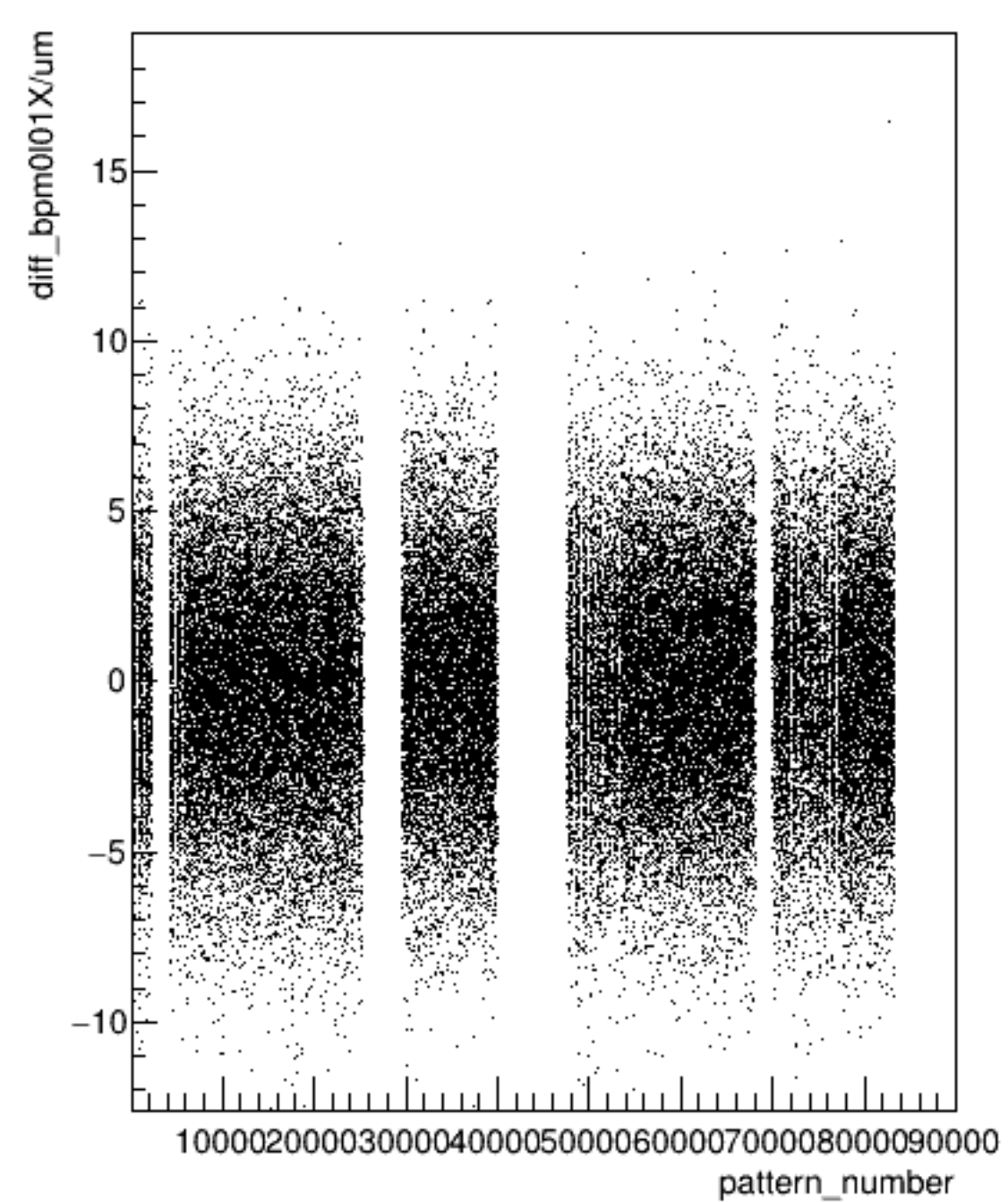
diff_bpm0l01X/um:pattern_number {ErrorFlag==0}
