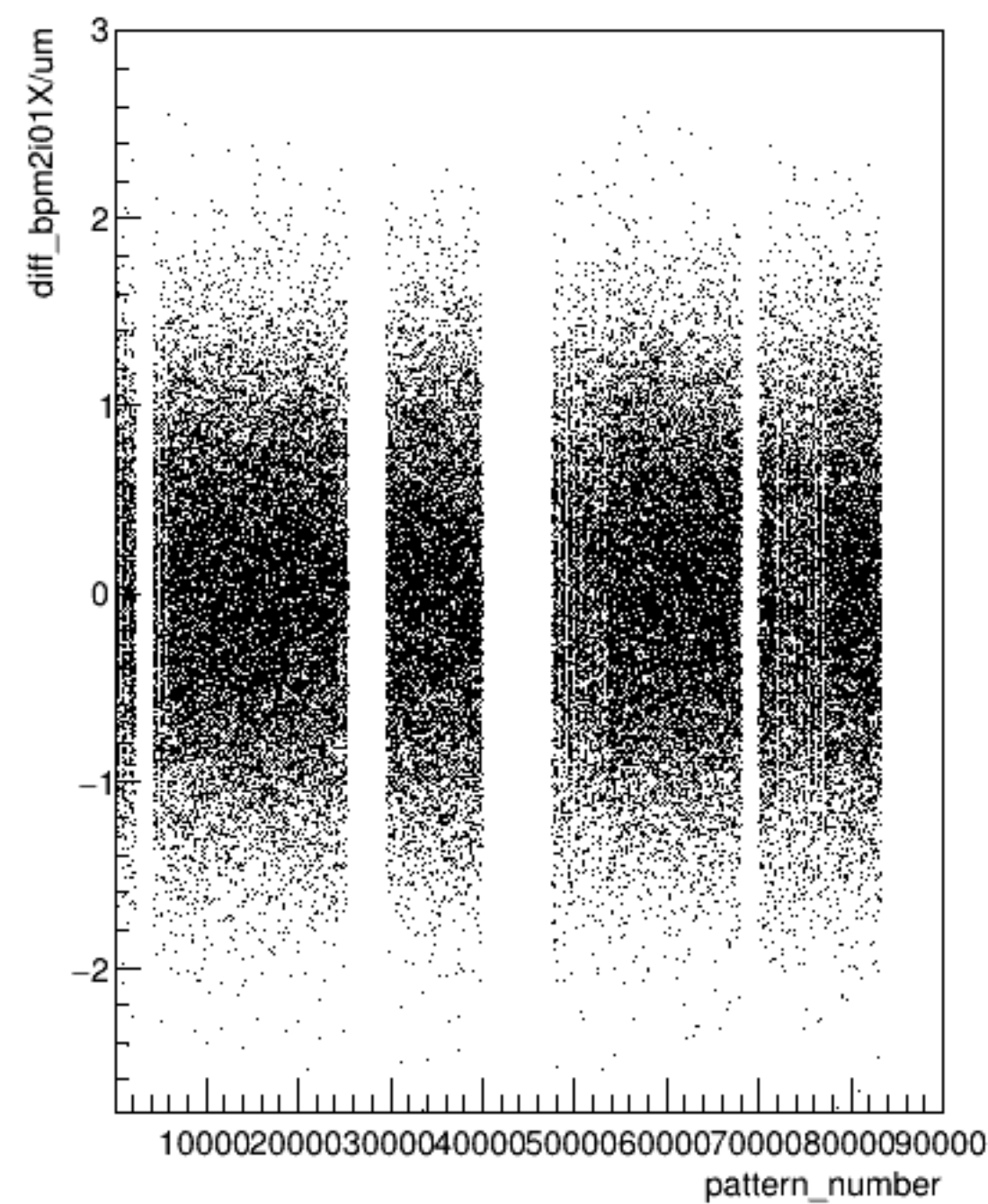
diff_bpm2i01X/um:pattern_number (ErrorFlag==0)
