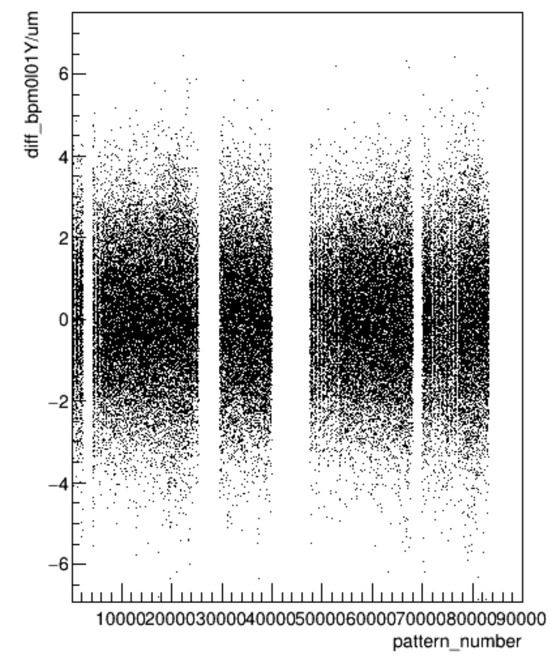
diff_bpm0l01Y/um:pattern_number {ErrorFlag==0}
