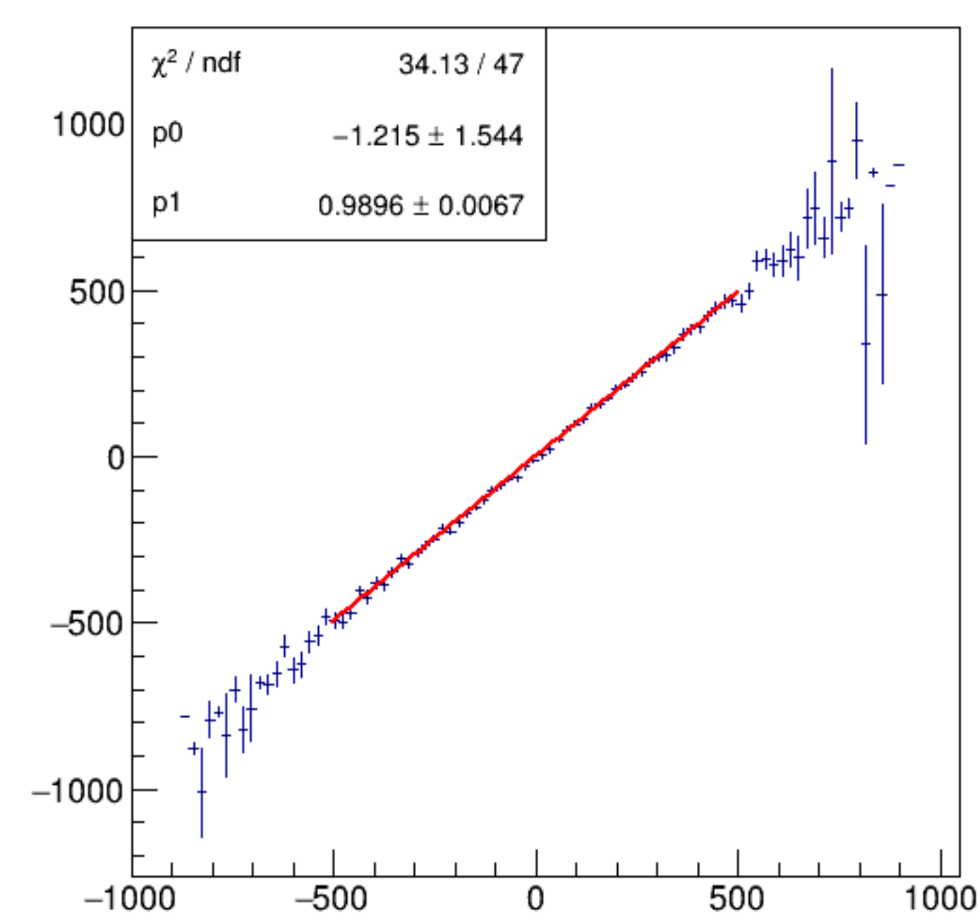
asym_bpm4acWS/ppm:Aq/ppm {ErrorFlag==0}
