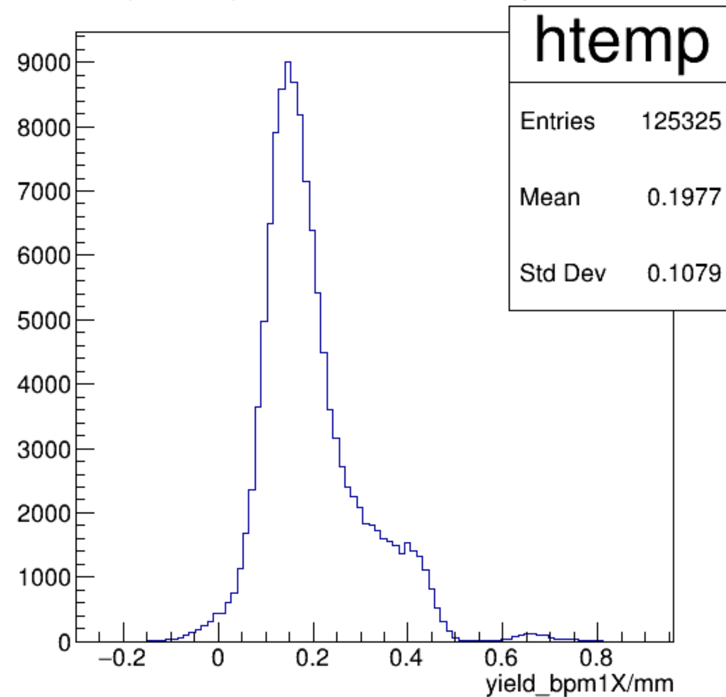
yield_bpm1X/mm {ErrorFlag==0}
