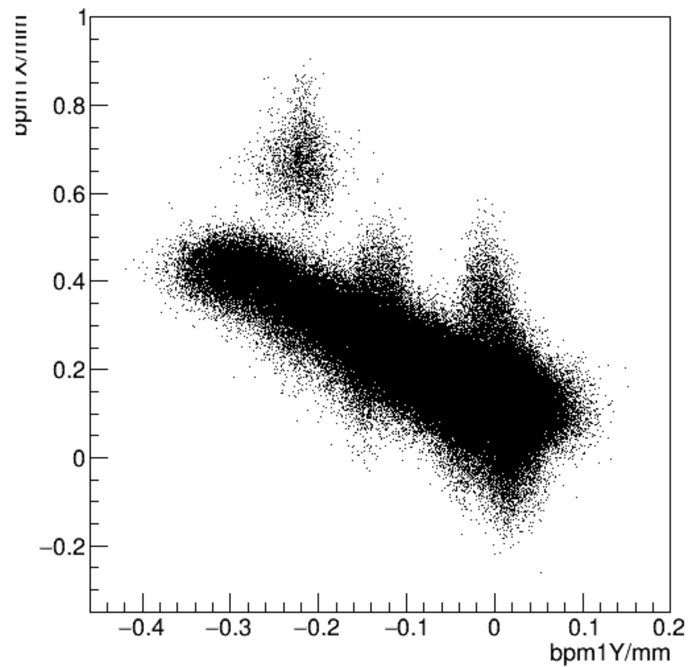
bpm1X/mm:bpm1Y/mm {ErrorFlag==0}
