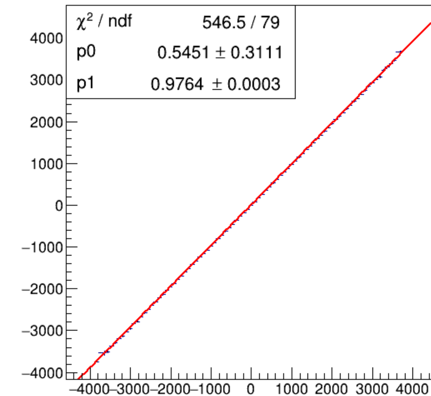
run6213_000_asym_bcm_dg_us_vs_asym_bcm_an_ds_pr.png
