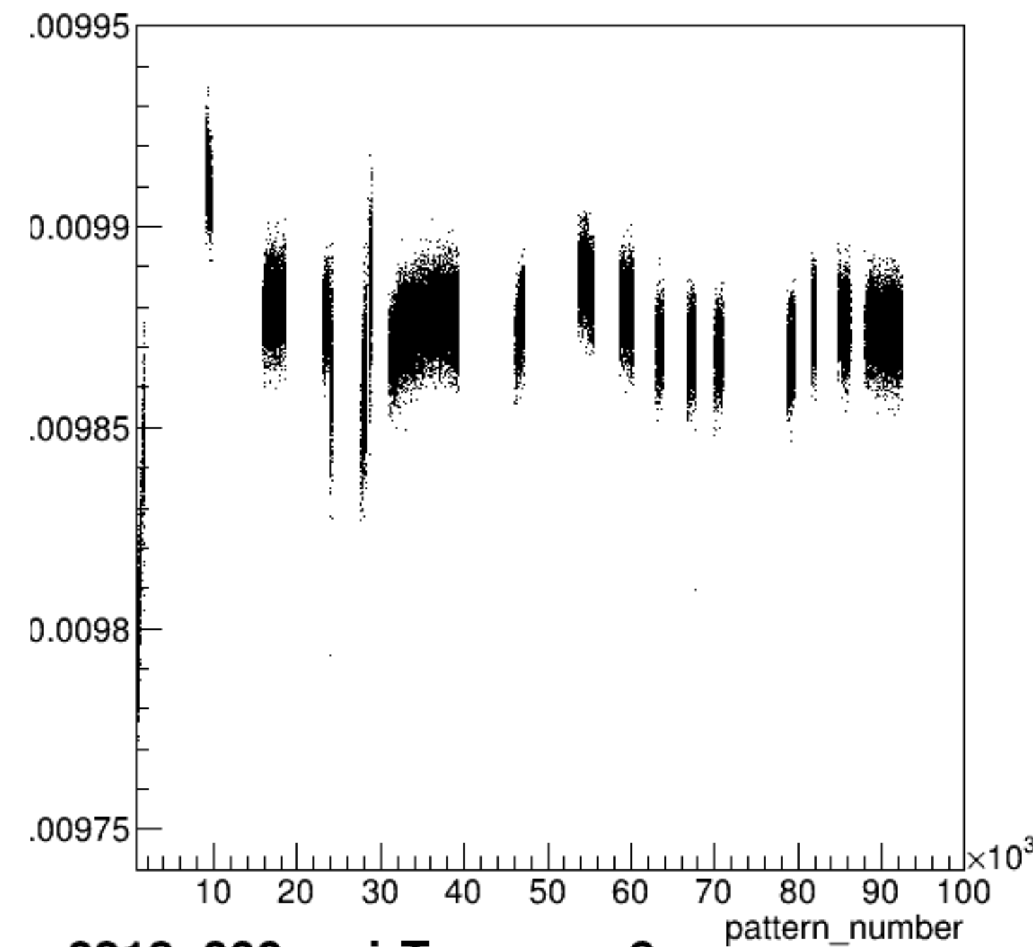
yield_sam8:pattern_number {ErrorFlag==0}
