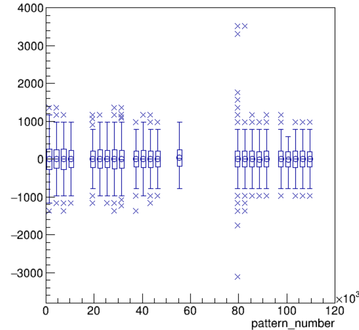
asym_bcm_dg_ds/ppm:pattern_number {ErrorFlag==0}
