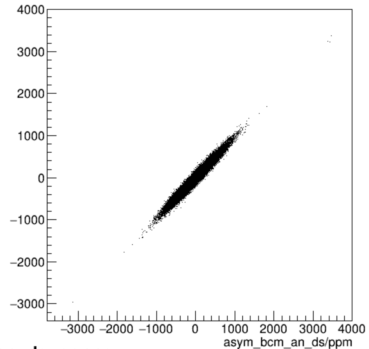
run6236_000_asym_bcm_dg_us_vs_asym_bcm_an_ds_pr.png
