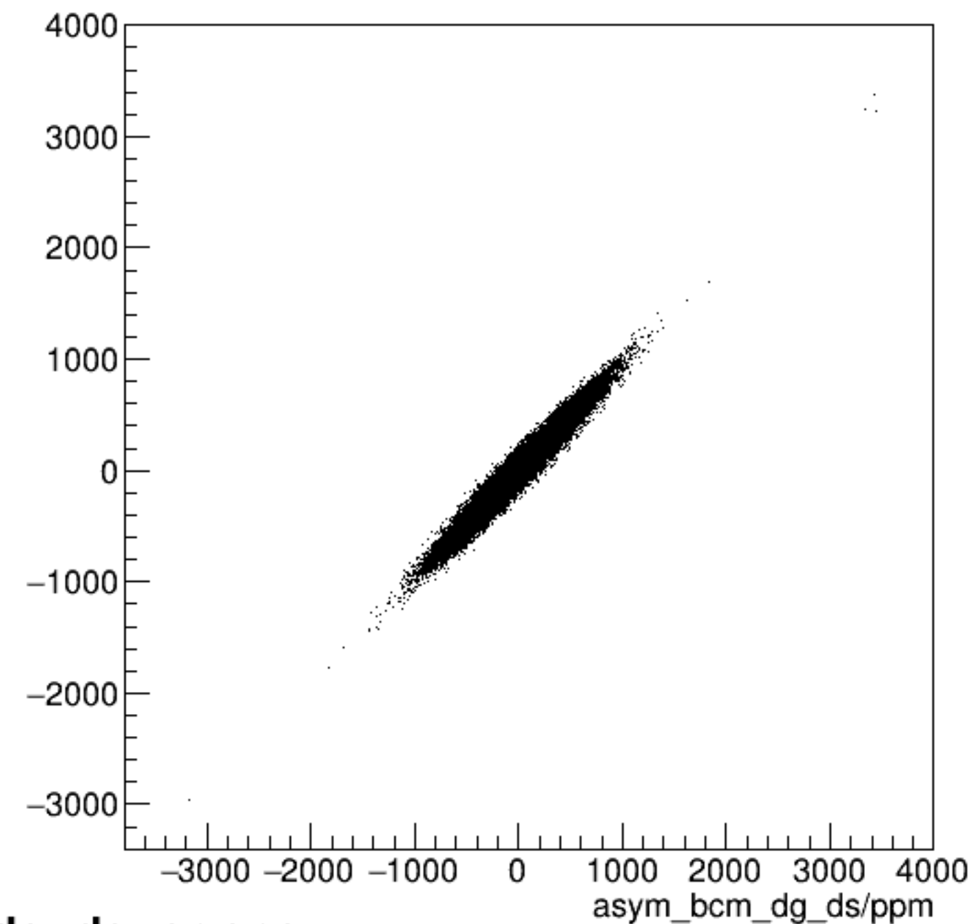
run6236_000_asym_bcm_dg_us_vs_asym_bcm_dg_ds_pr.png
