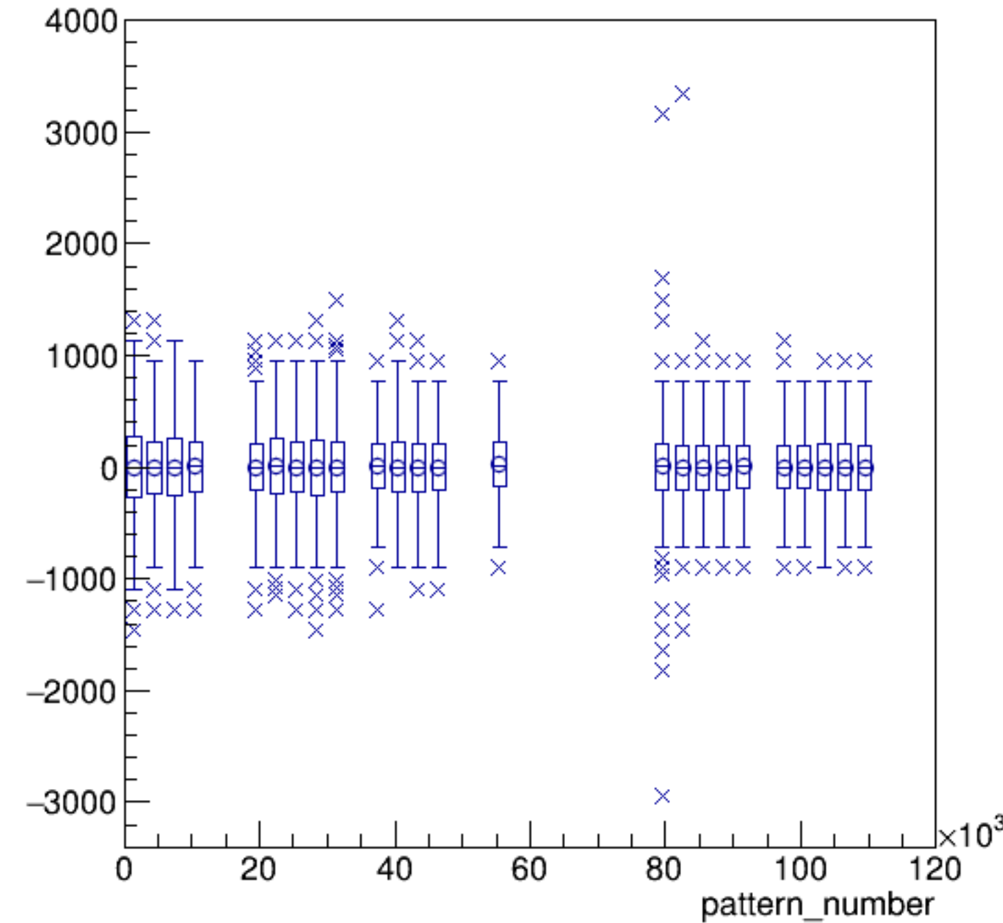
asym_bcm_dg_us/ppm:pattern_number {ErrorFlag==0}
