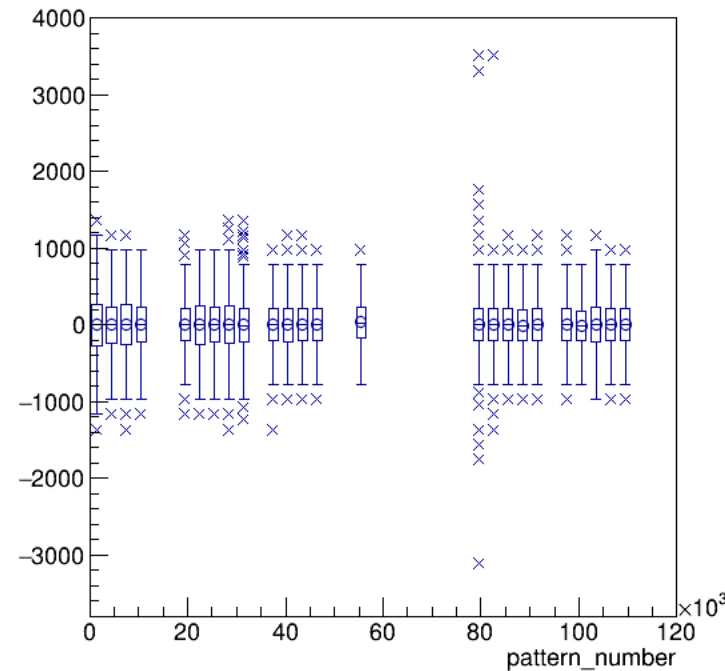
asym_bcm_an_us/ppm:pattern_number {ErrorFlag==0}
