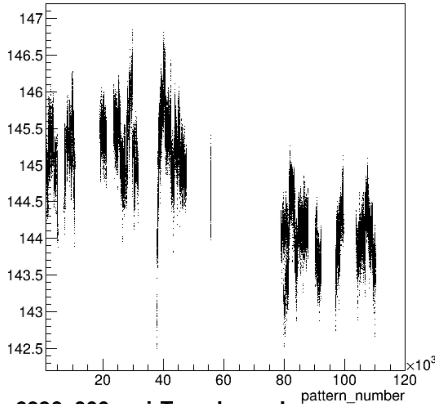
yield_bcm_dg_us:pattern_number {ErrorFlag==0}
