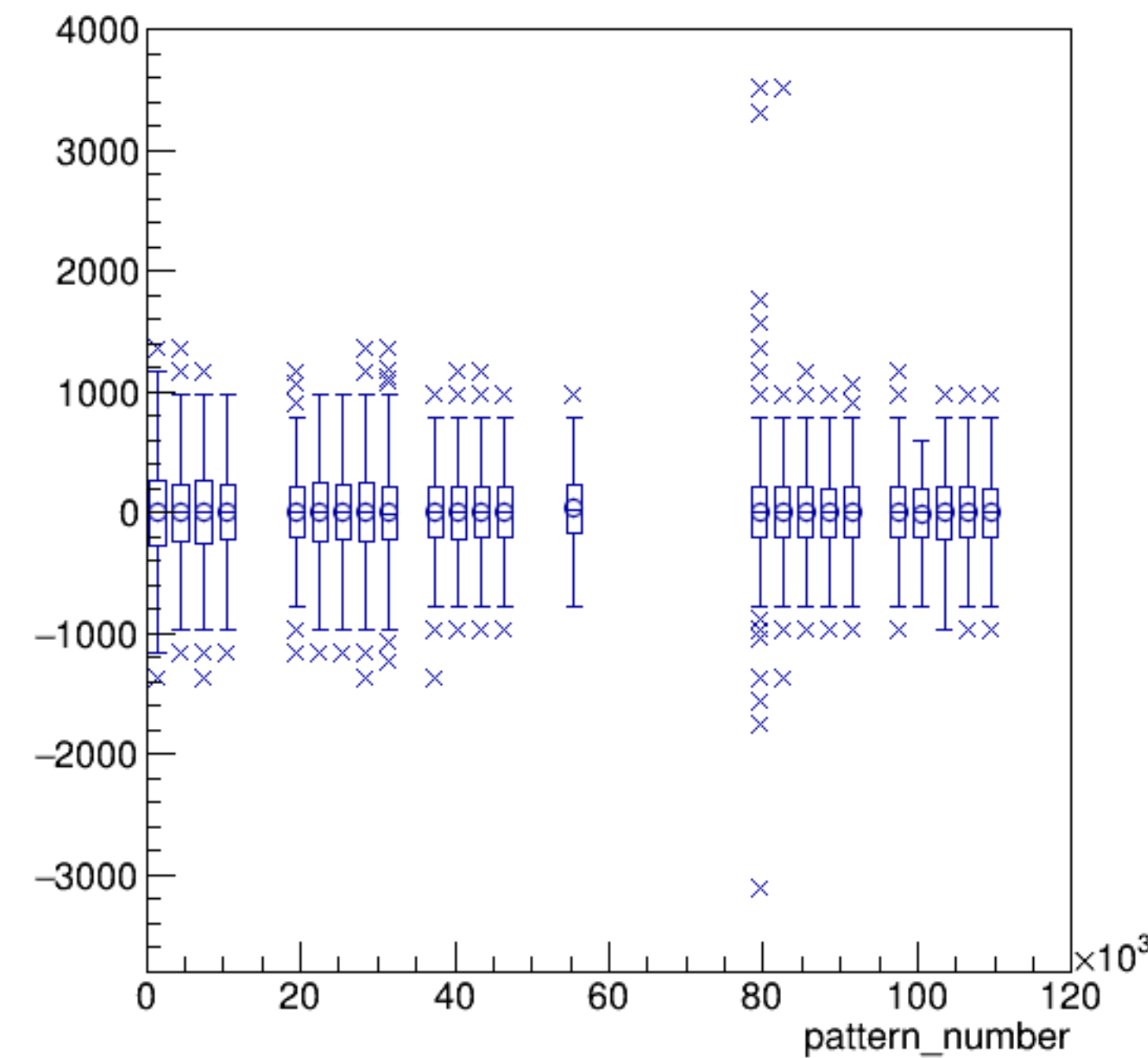
asym_bcm_an_ds3/ppm:pattern_number {ErrorFlag==0}
