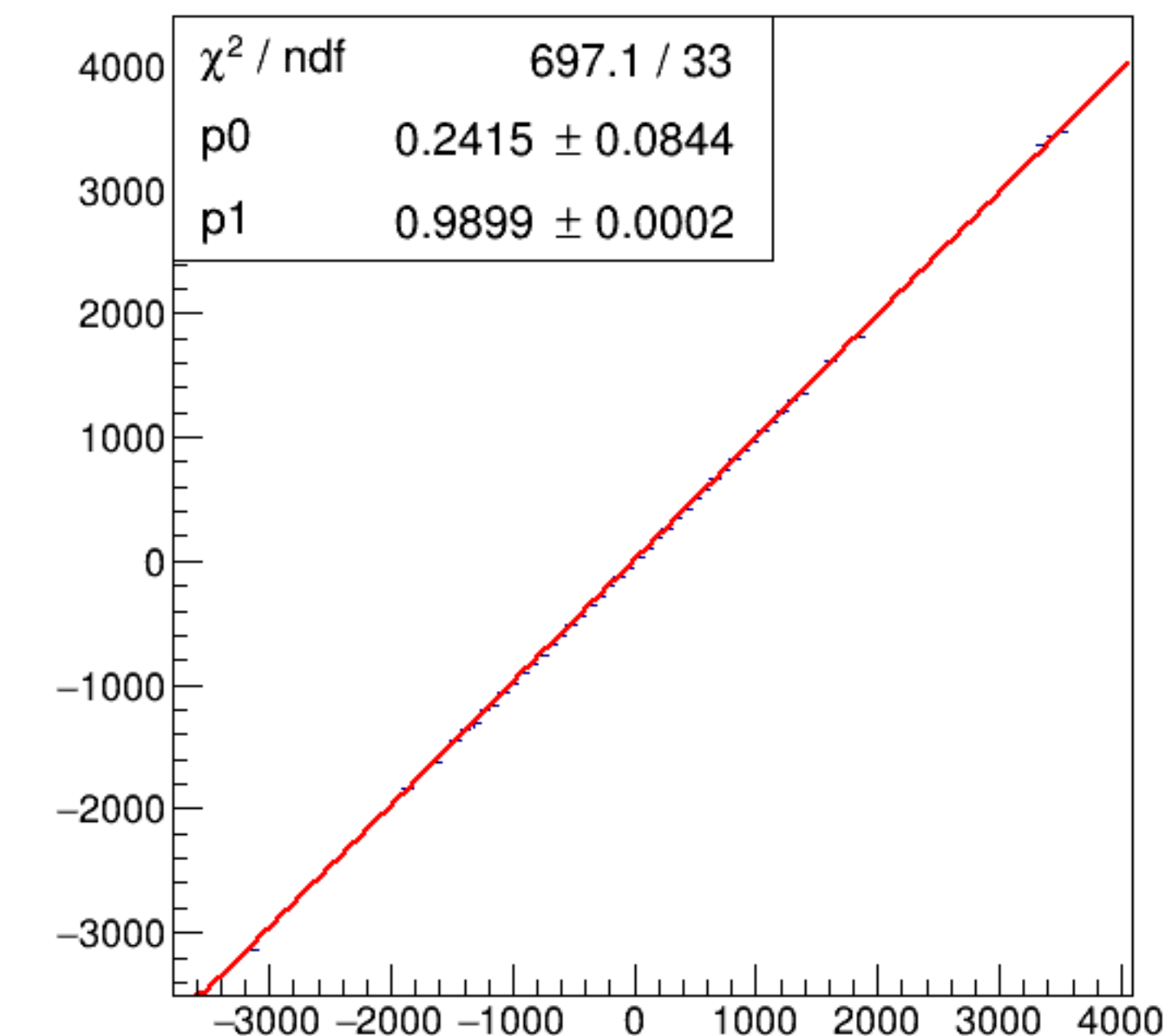
run6236_000_asym_bcm_an_ds_vs_asym_bcm_an_ds3_pr.png
