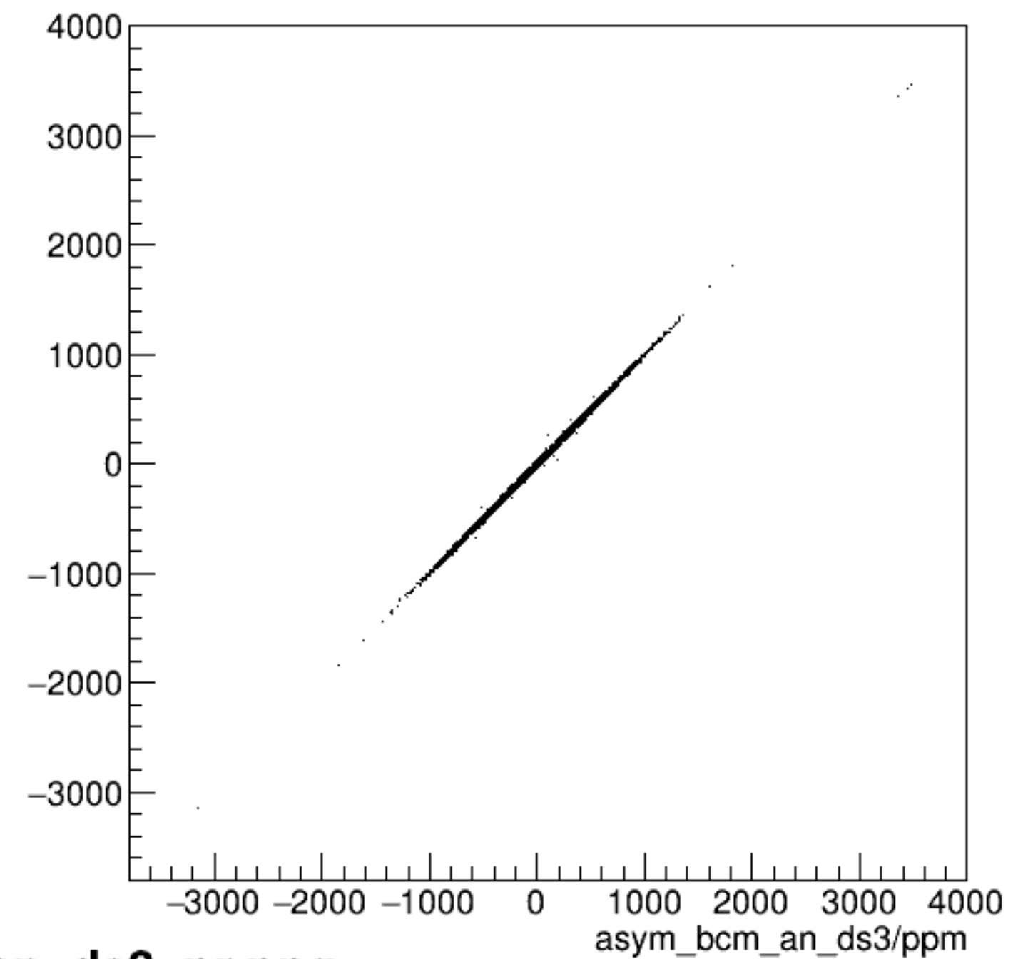
run6236_000_asym_bcm_an_ds_vs_asym_bcm_an_ds3_pr.png
