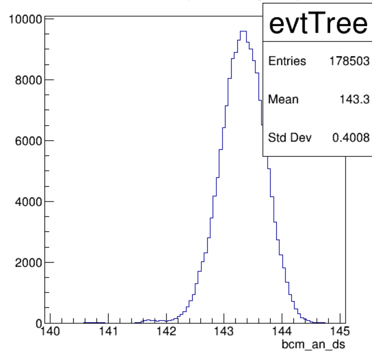
bcm_an_ds {ErrorFlag==0}
