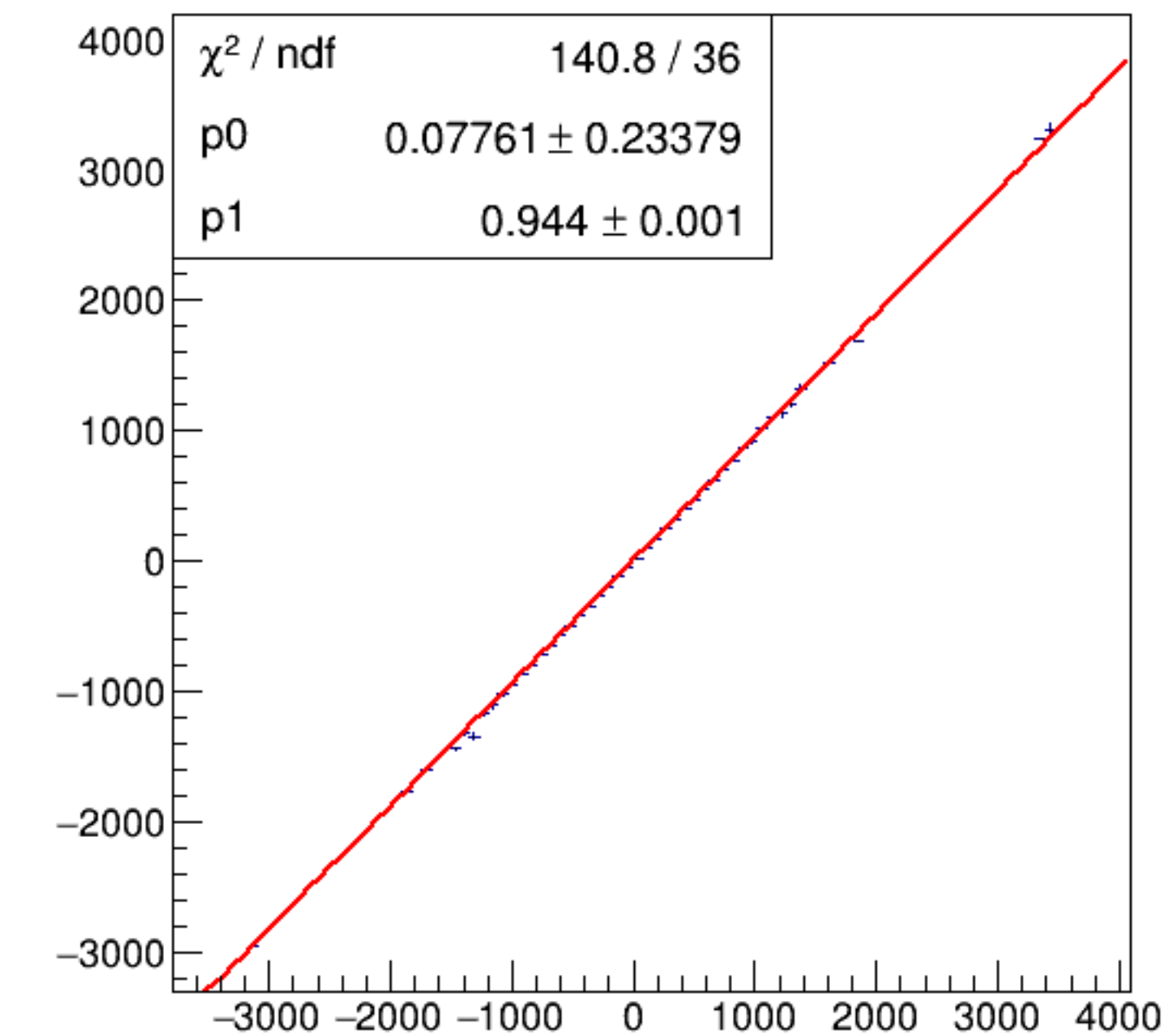
run6236_000_asym_bcm_dg_us_vs_asym_bcm_dg_ds_pr.png
