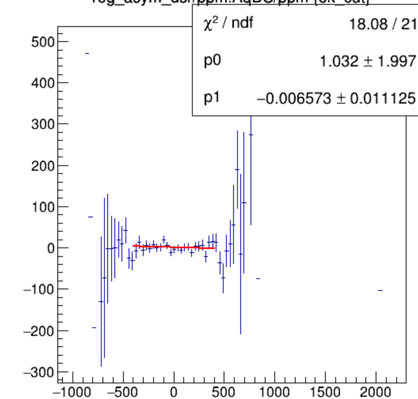
reg_asym_dsr/ppm:AqDS/ppm {ok_cut}
