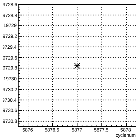
usr_coil1:cyclenum {run == 6285}
