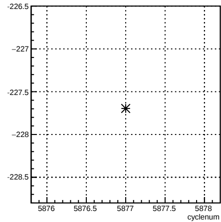
12X_coil1:cyclenum {run == 6285}
