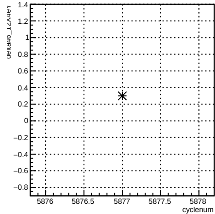
delta46_12X4eY:cyclenum {run == 6285}
