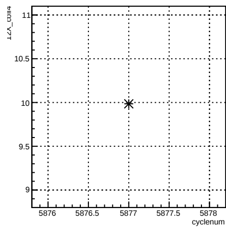
12X_coil4:cyclenum {run == 6285}
