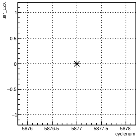
usr_12X:cyclenum {run == 6285}
