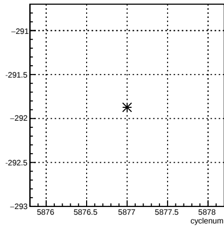
4eX_coil1:cyclenum {run == 6285}
