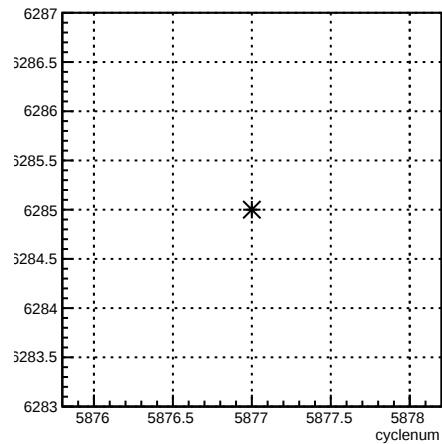
run:cyclenum {run == 6285}
