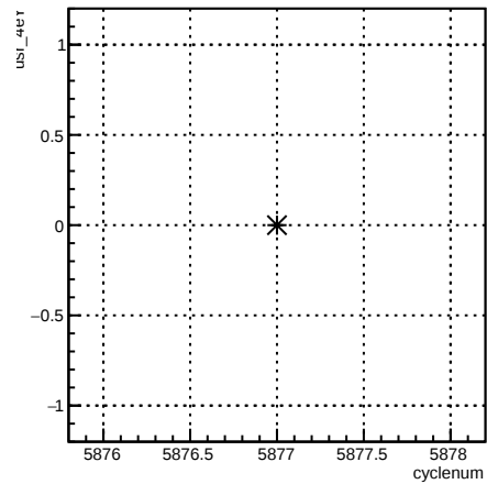
usr_4eY:cyclenum {run == 6285}
