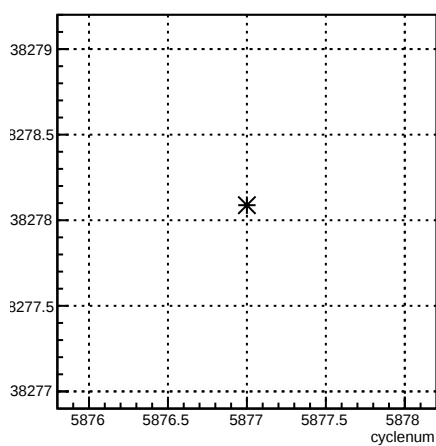
usr_coil7:cyclenum {run == 6285}
