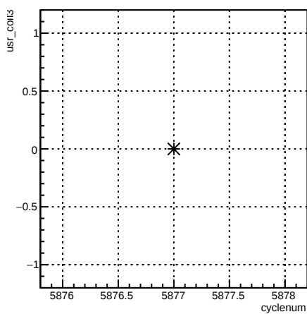
usr_coil3:cyclenum {run == 6285}
