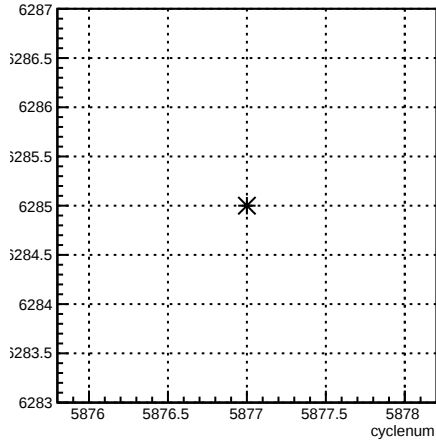
run:cyclenum {run == 6285}
