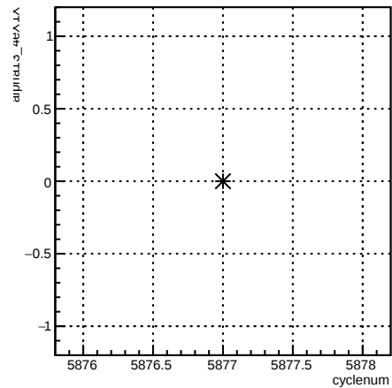
alpha13_4eX1X:cyclenum {run == 6285}
