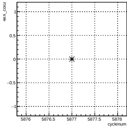
4eX_coil3:cyclenum {run == 6285}
