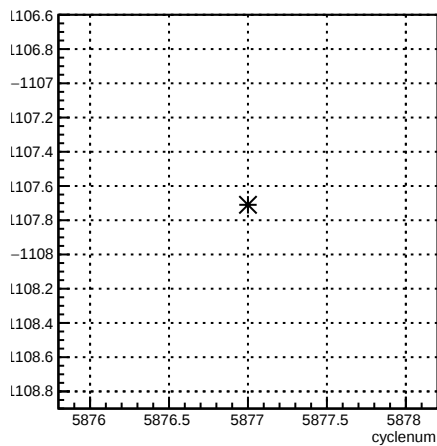
usr_coil6:cyclenum {run == 6285}
