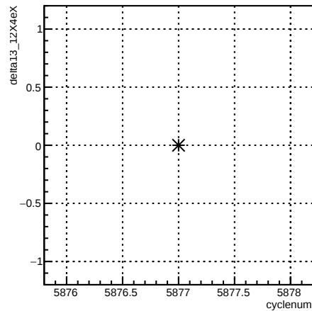
delta13_12X4eX:cyclenum {run == 6285}
