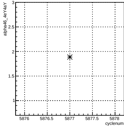
alpha46_4eY4aY:cyclenum {run == 6285}
