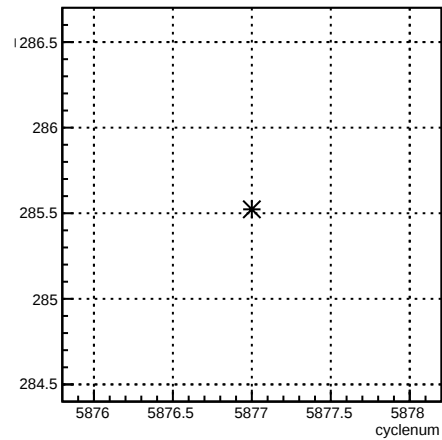
4eX_coil7:cyclenum {run == 6285}
