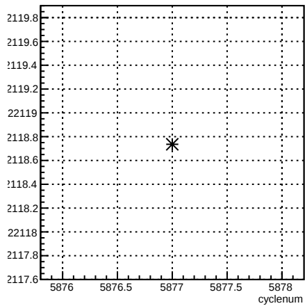
usl_coil6:cyclenum {run == 6285}
