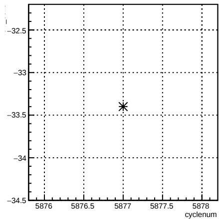
4eY_coil6:cyclenum {run == 6285}
