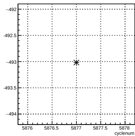
12X_coil7:cyclenum {run == 6285}
