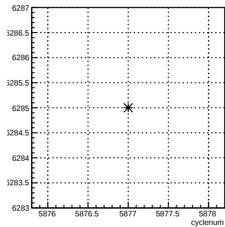
run:cyclenum {run == 6285}
