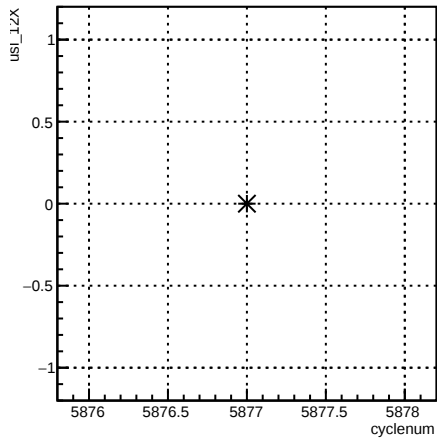
usl_12X:cyclenum {run == 6285}
