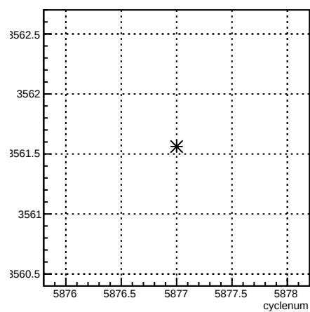
usr_coil4:cyclenum {run == 6285}
