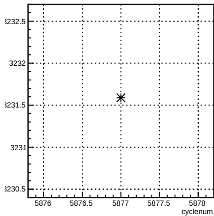
usl_coil7:cyclenum {run == 6285}
