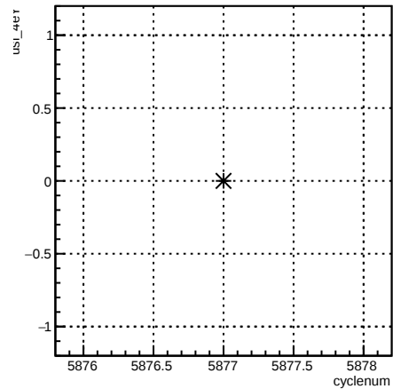
usl_4eY:cyclenum {run == 6285}
