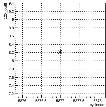
12X_coil6:cyclenum {run == 6285}
