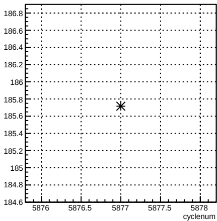
4eY_coil4:cyclenum {run == 6285}
