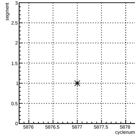
segment:cyclenum {run == 6285}
