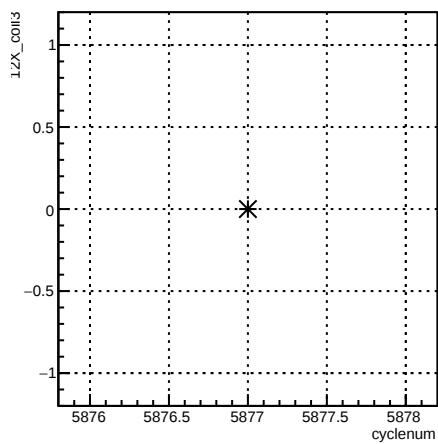
12X_coil3:cyclenum {run == 6285}
