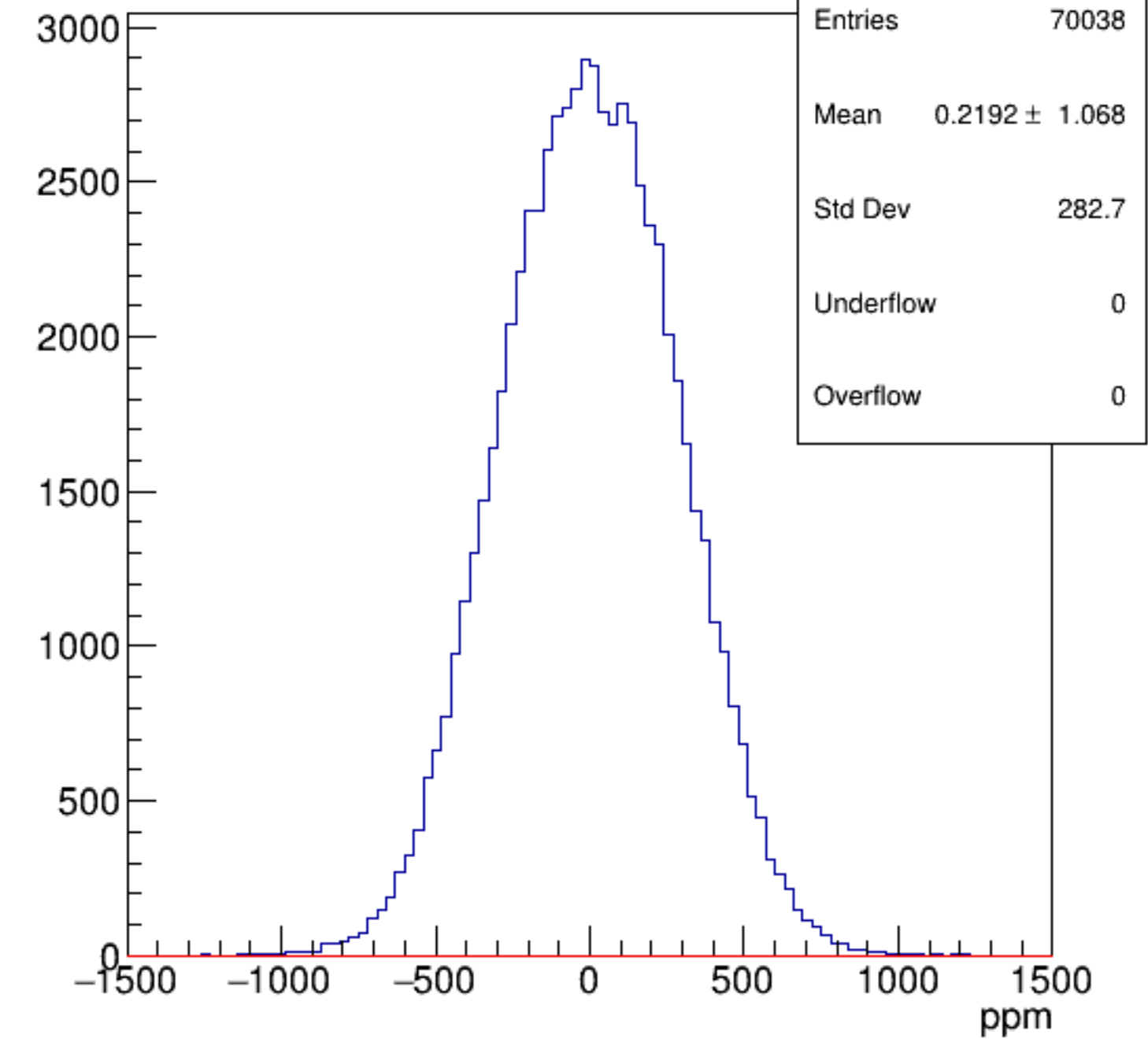
asym_bcm_dg_us
