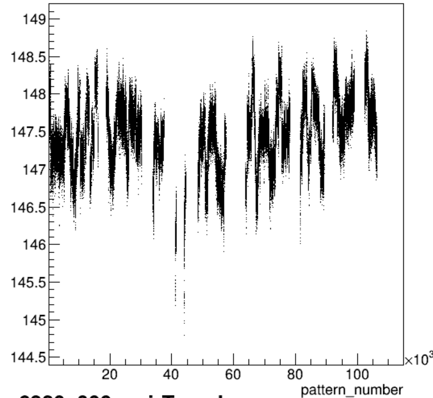
yield_bcm_an_us:pattern_number {ErrorFlag==0}
