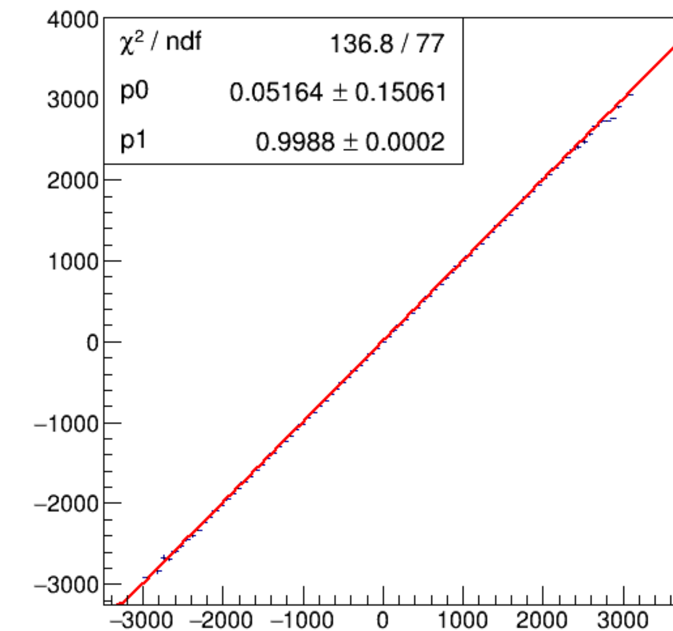
run6320_000_asym_bcm_dg_ds_vs_asym_bcm_an_us_pr.png
