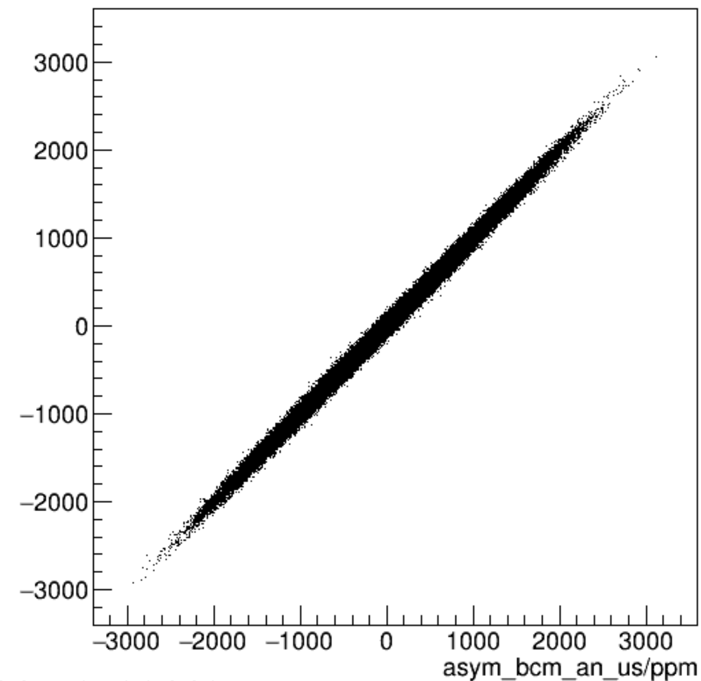
run6320_000_asym_bcm_dg_ds_vs_asym_bcm_an_us_pr.png
