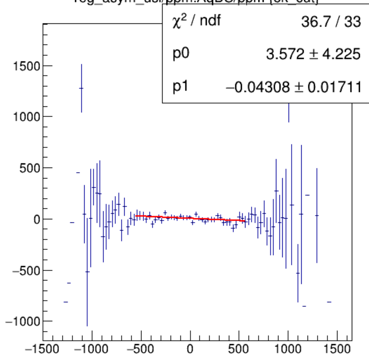
reg_asym_usl/ppm:AqDS/ppm {ok_cut}
