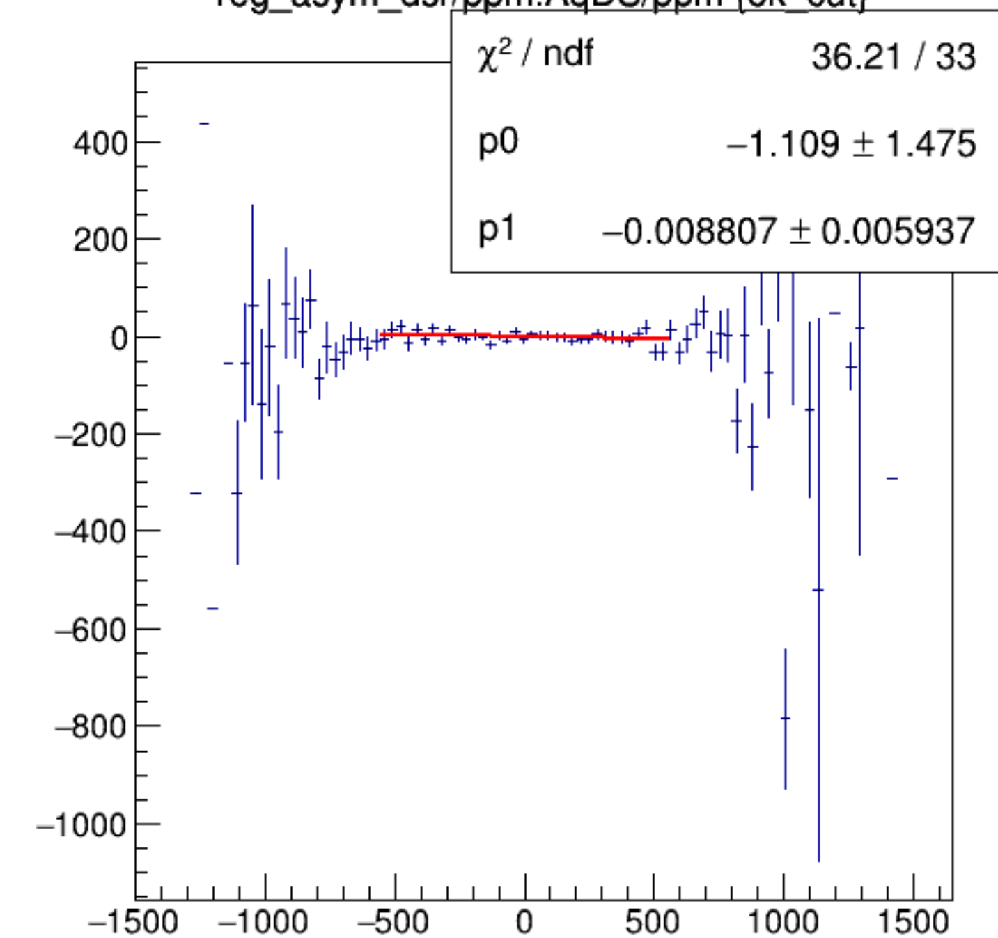
reg_asym_dsr/ppm:AqDS/ppm {ok_cut}
