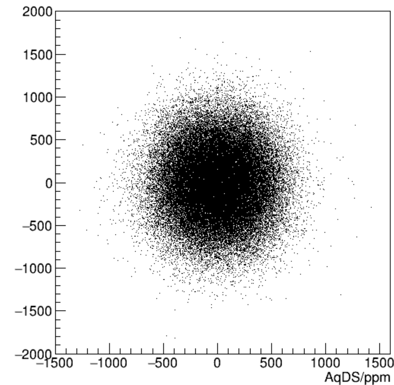
reg_asym_dsr/ppm:AqDS/ppm {ok_cut}
