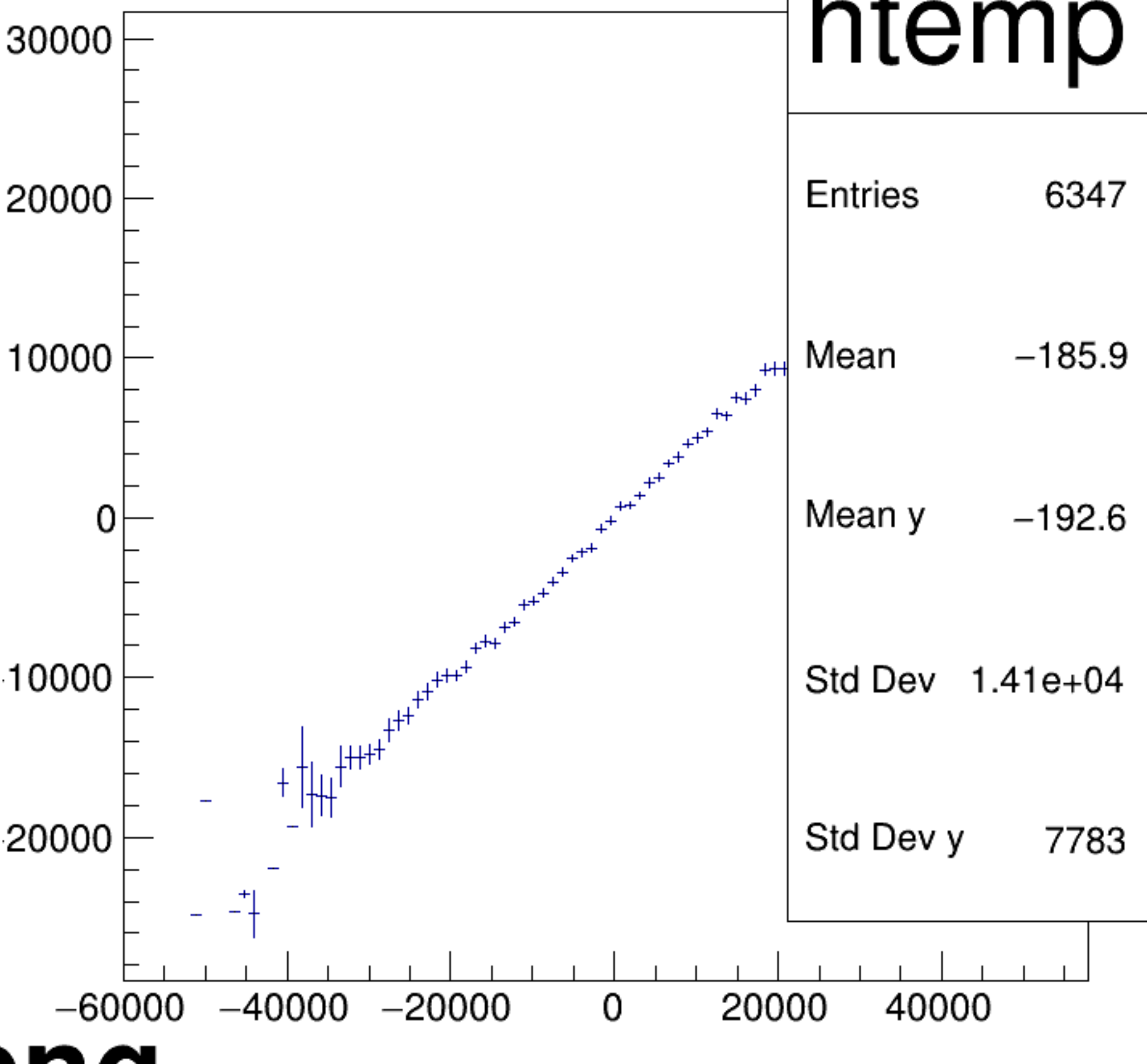
asym_atl2/ppm:asym_atr2/ppm {ok_cut}
