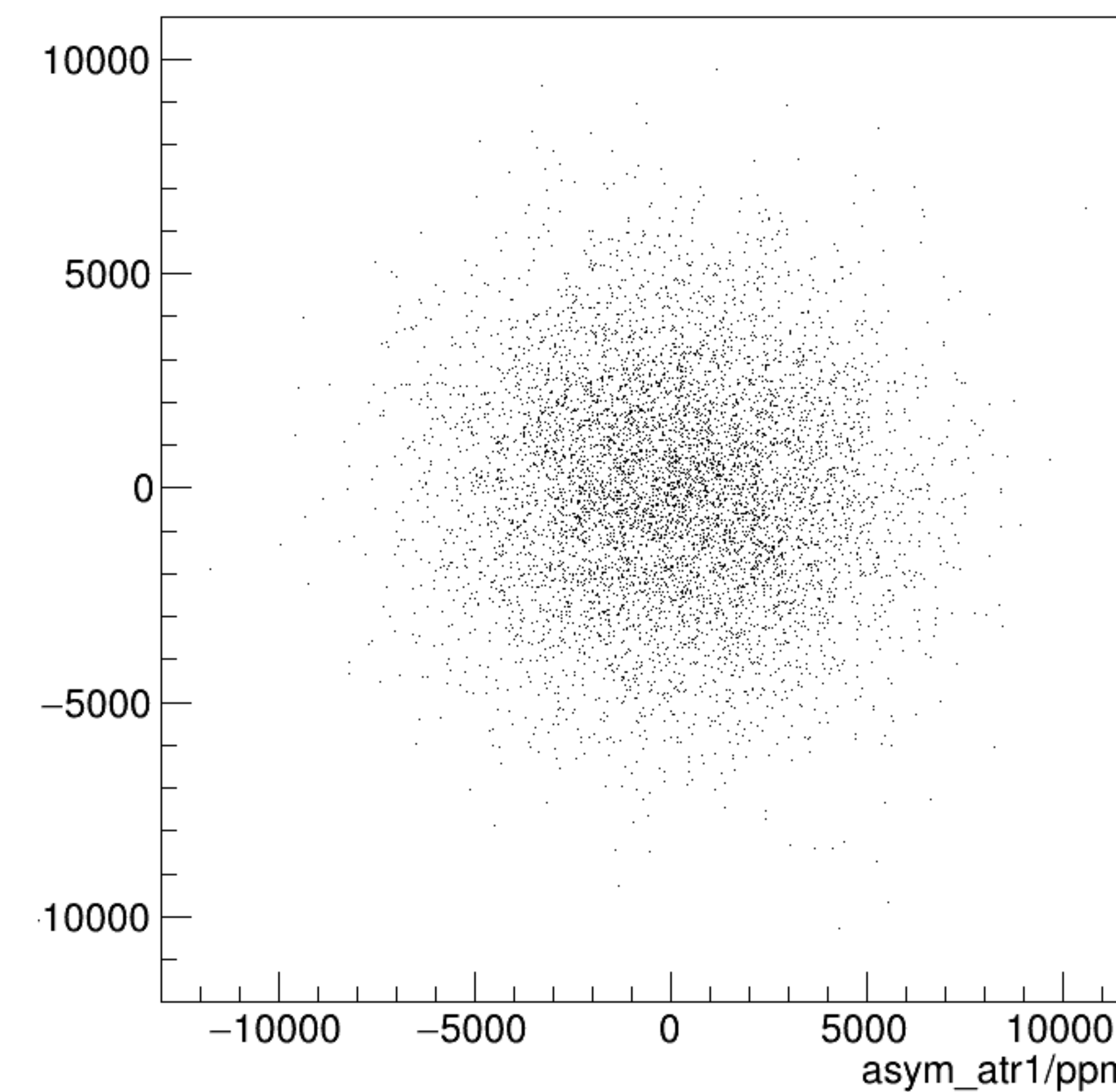
asym_atl1/ppm:asym_atr1/ppm {ok_cut}
