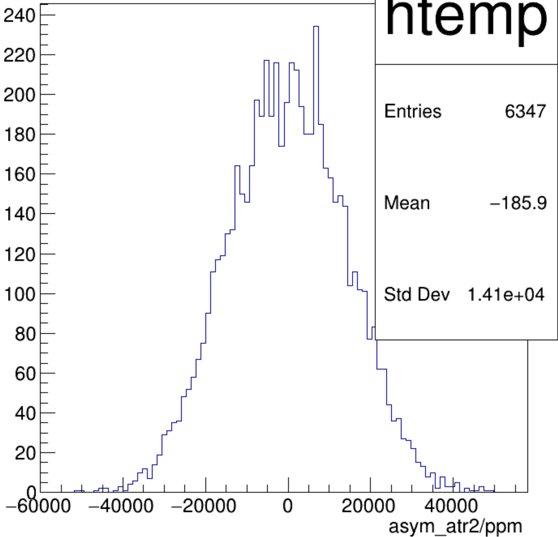
asym_atr2/ppm {ok_cut}
