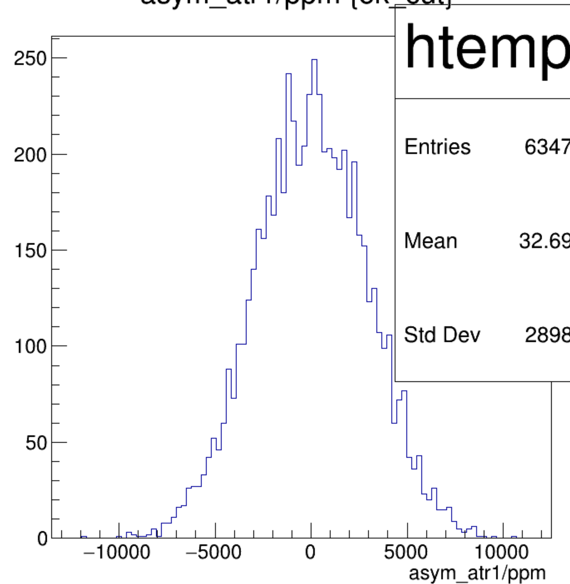
asym_atr1/ppm {ok_cut}
