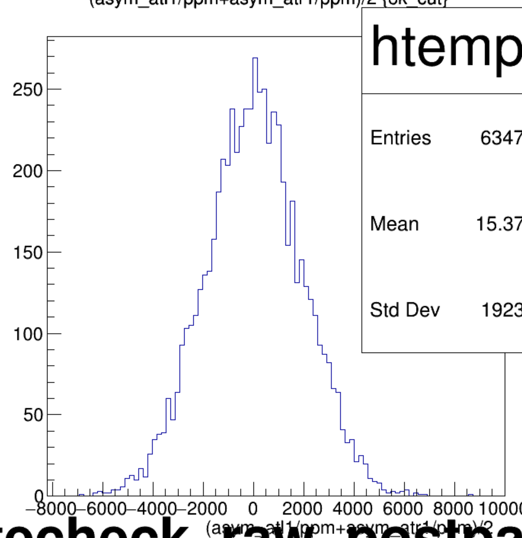
(asym_atl1/ppm+asym_atr1/ppm)/2 {ok_cut}
