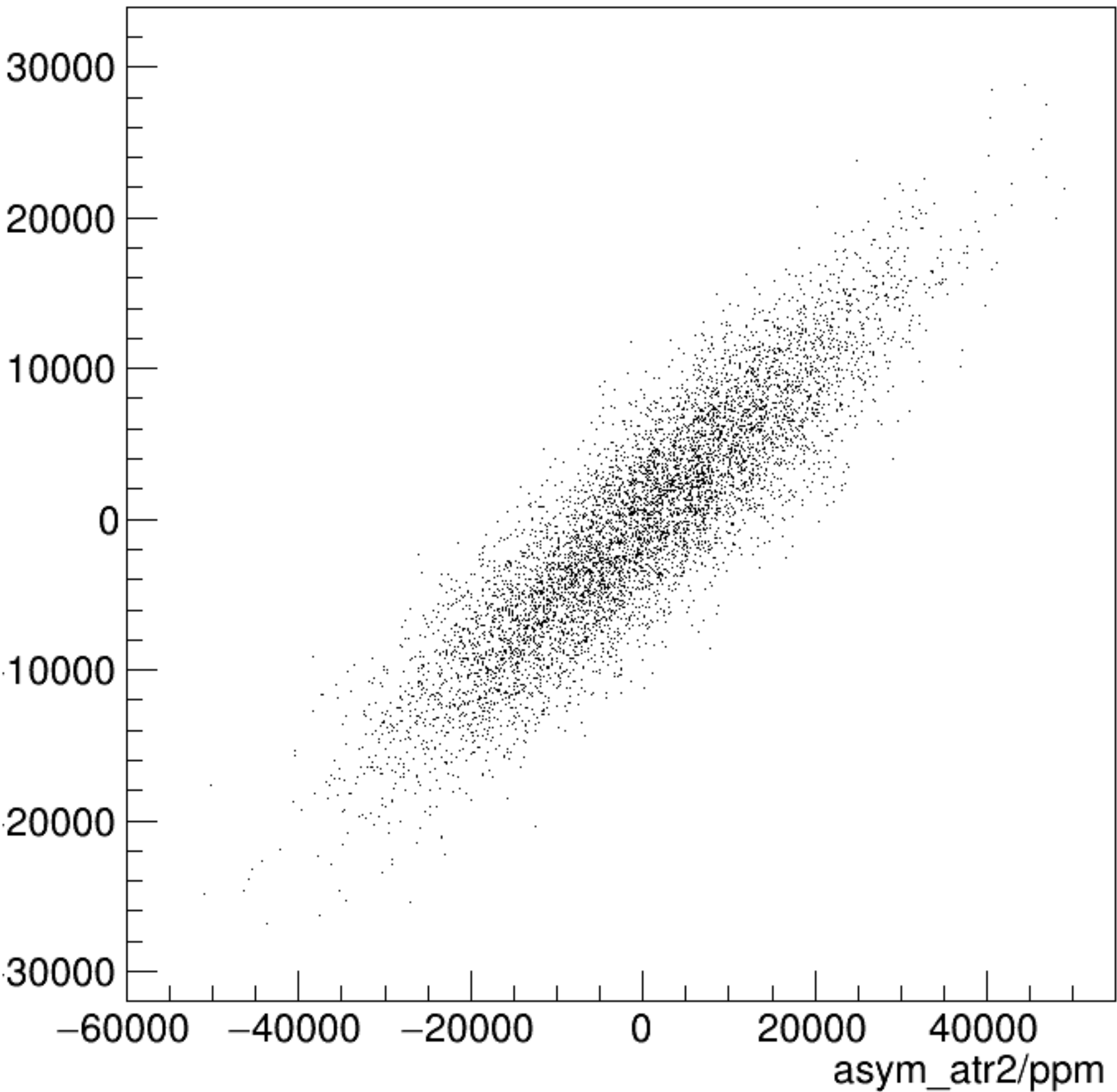
asym_atl2/ppm:asym_atr2/ppm {ok_cut}
