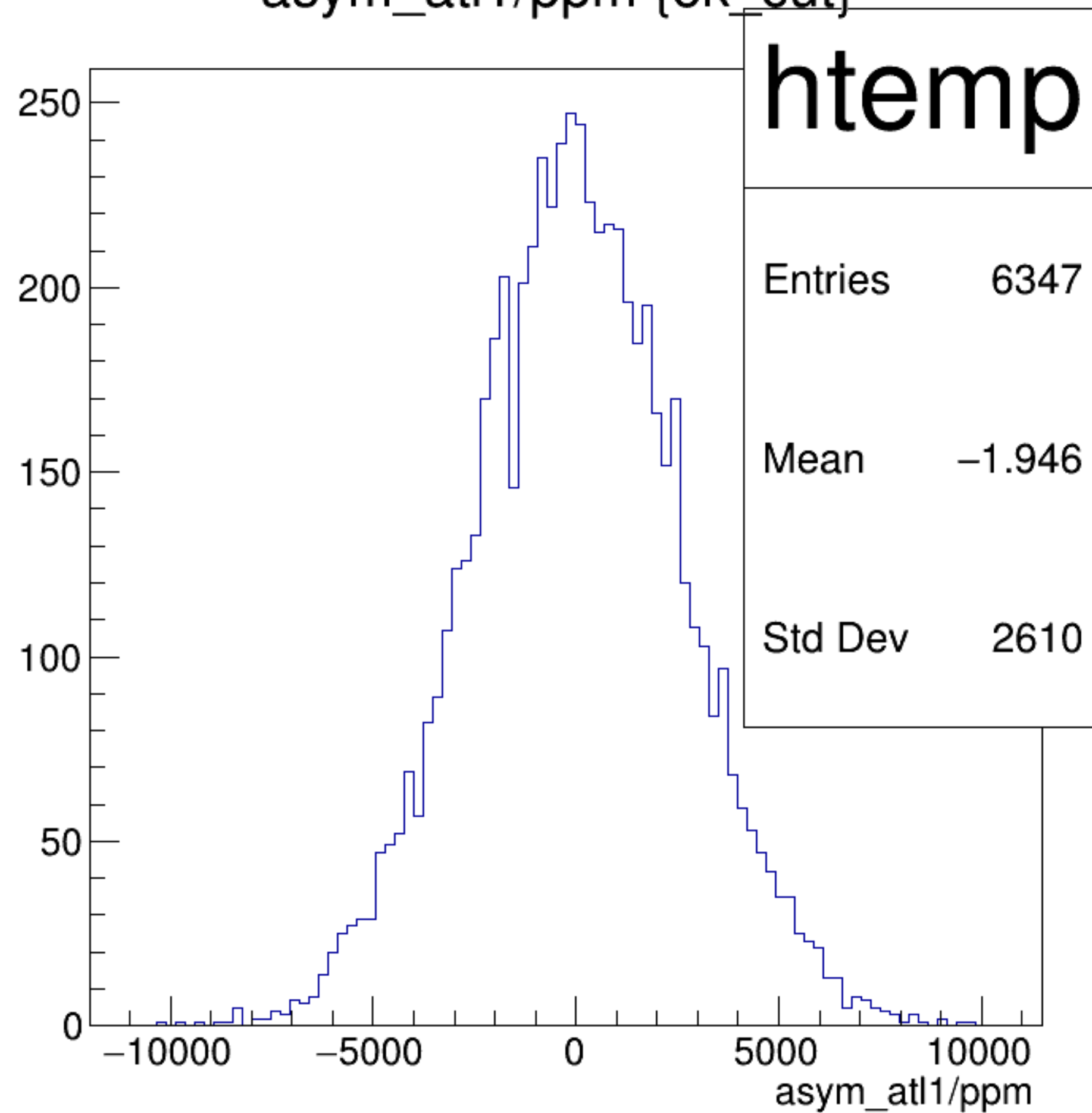
asym_atl1/ppm {ok_cut}
