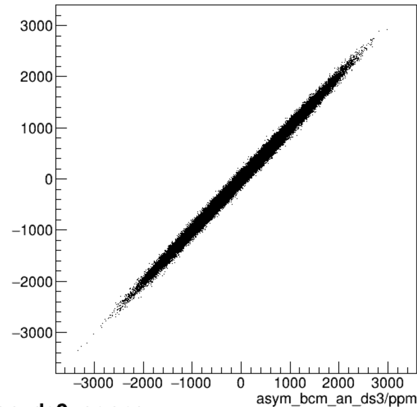
run6328_000_asym_bcm_dg_us_vs_asym_bcm_an_ds3_pr.png
