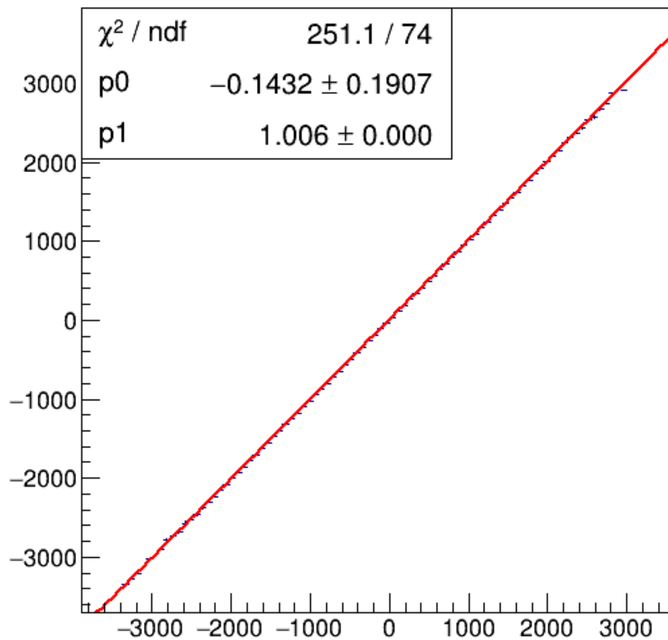
run6328_000_asym_bcm_dg_us_vs_asym_bcm_an_ds3_pr.png
