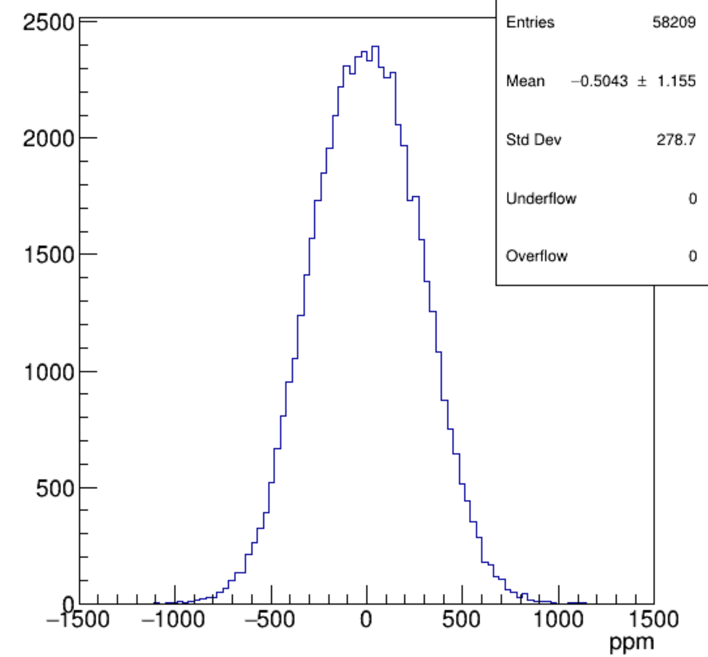
asym_bcm_an_us
