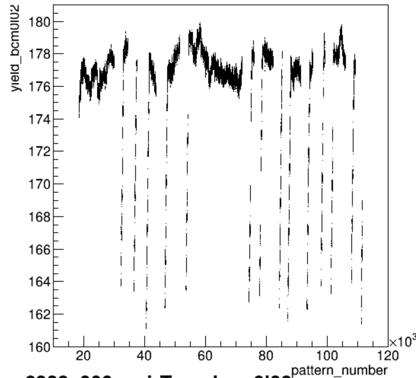
yield_bcm0l02:pattern_number {ErrorFlag==0}
