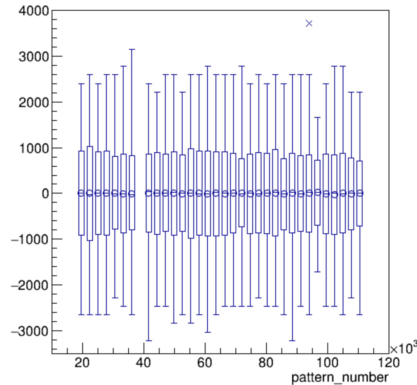
asym_bcm0l02/ppm:pattern_number {ErrorFlag==0}
