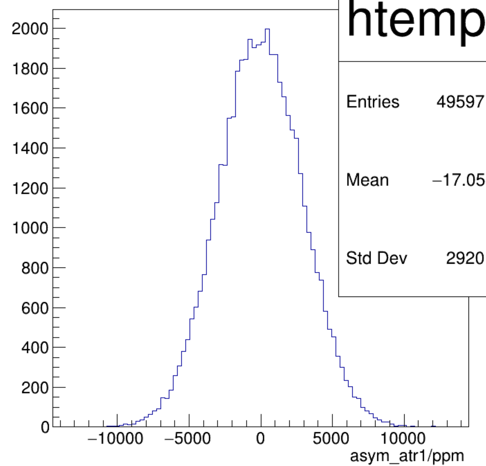
asym_atr1/ppm {ok_cut}
