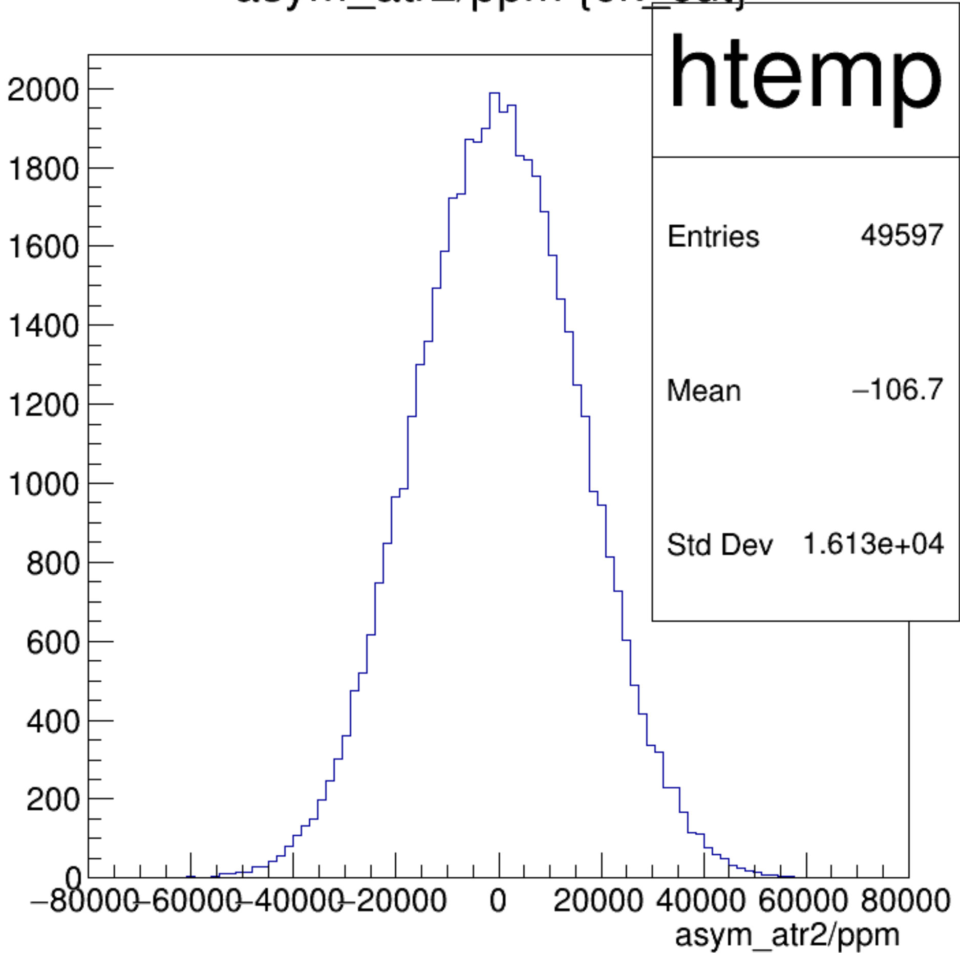
asym_atr2/ppm {ok_cut}
