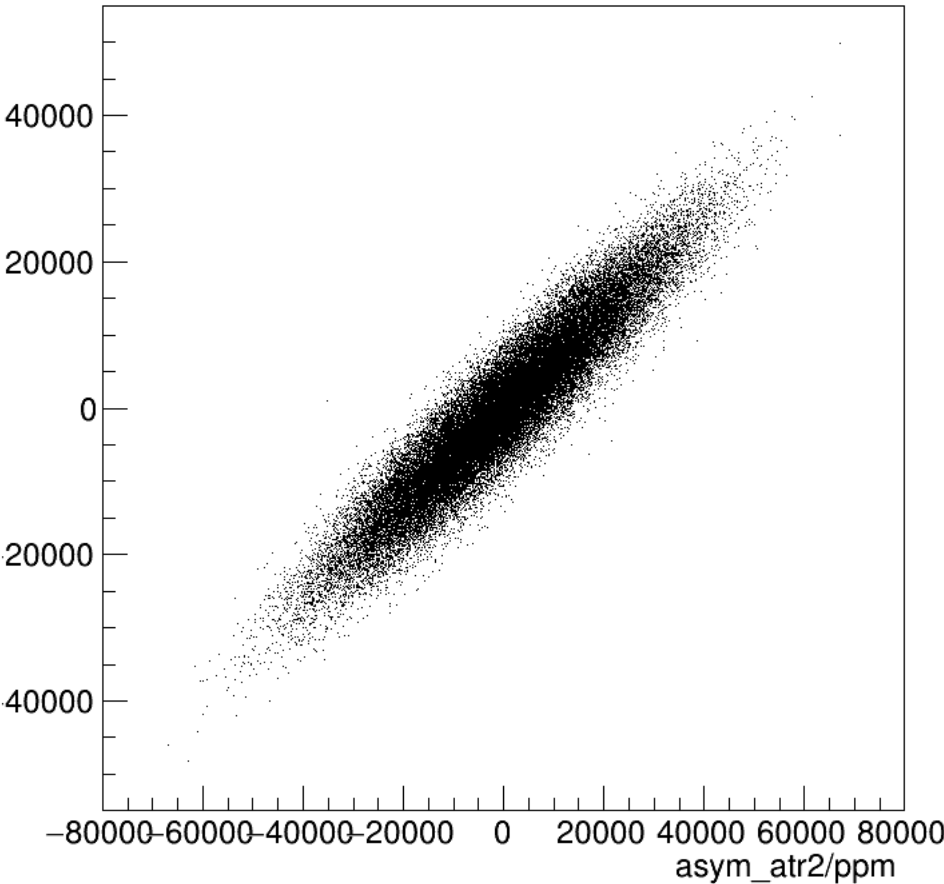
asym_atl2/ppm:asym_atr2/ppm {ok_cut}
