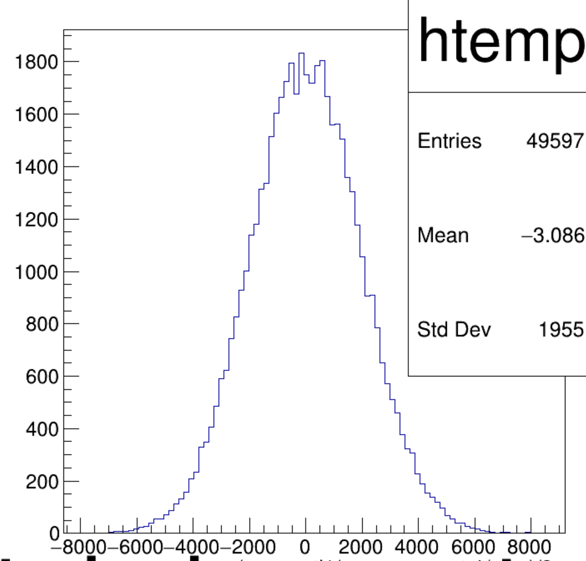
(asym_atl1/ppm+asym_atr1/ppm)/2 {ok_cut}
