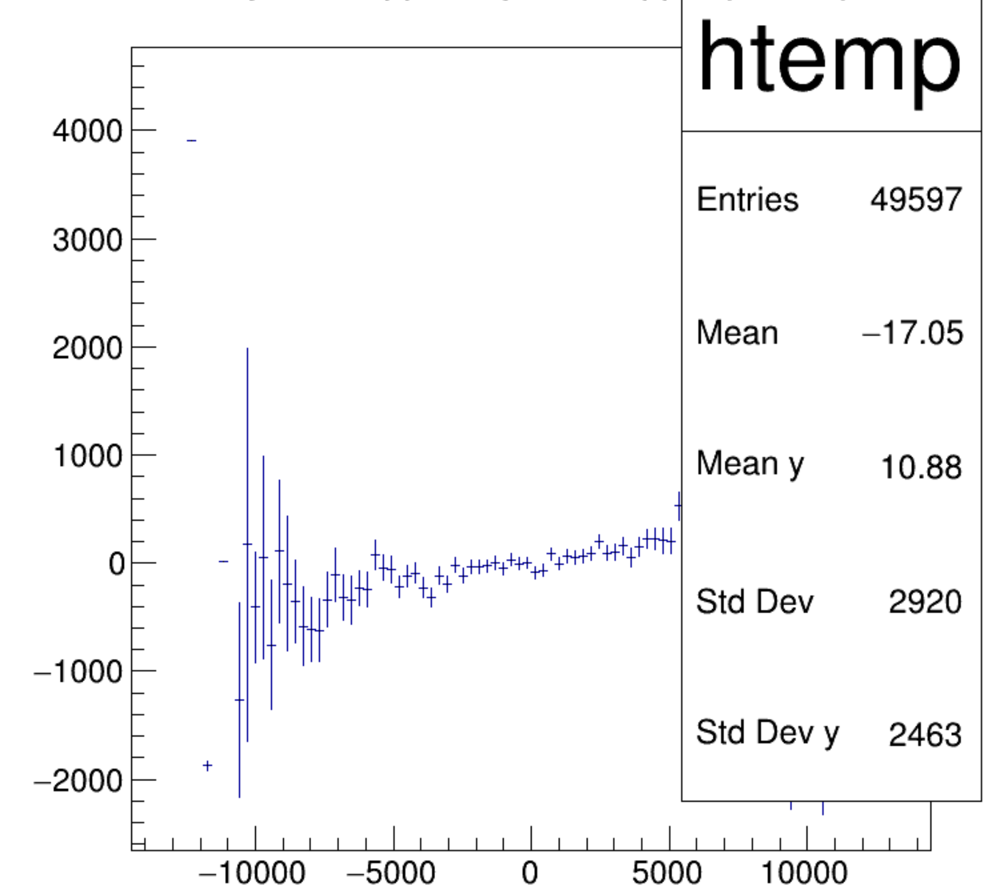
asym_atl1/ppm:asym_atr1/ppm {ok_cut}
