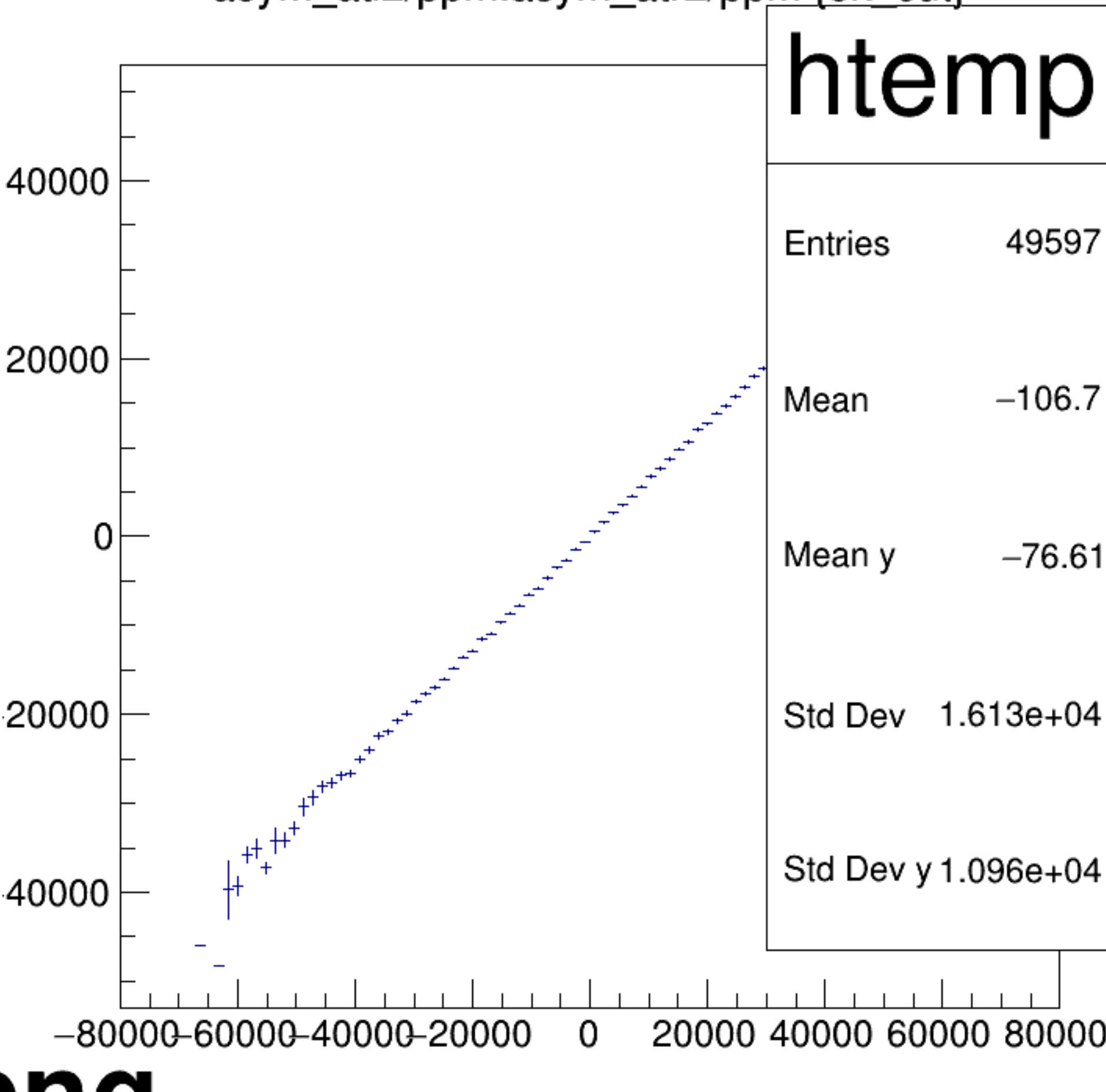
asym_atl2/ppm:asym_atr2/ppm {ok_cut}
