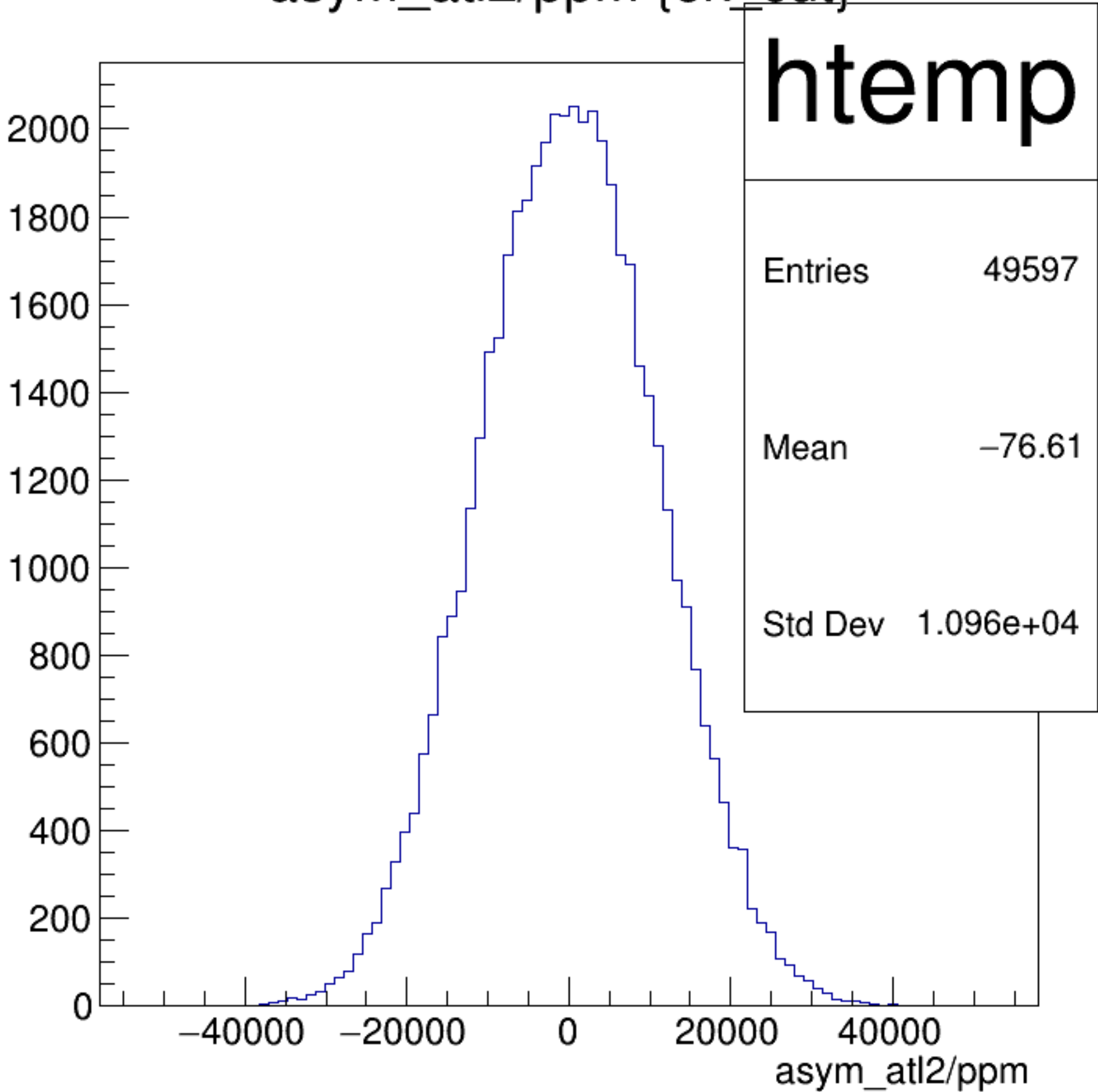
asym_atl2/ppm {ok_cut}
