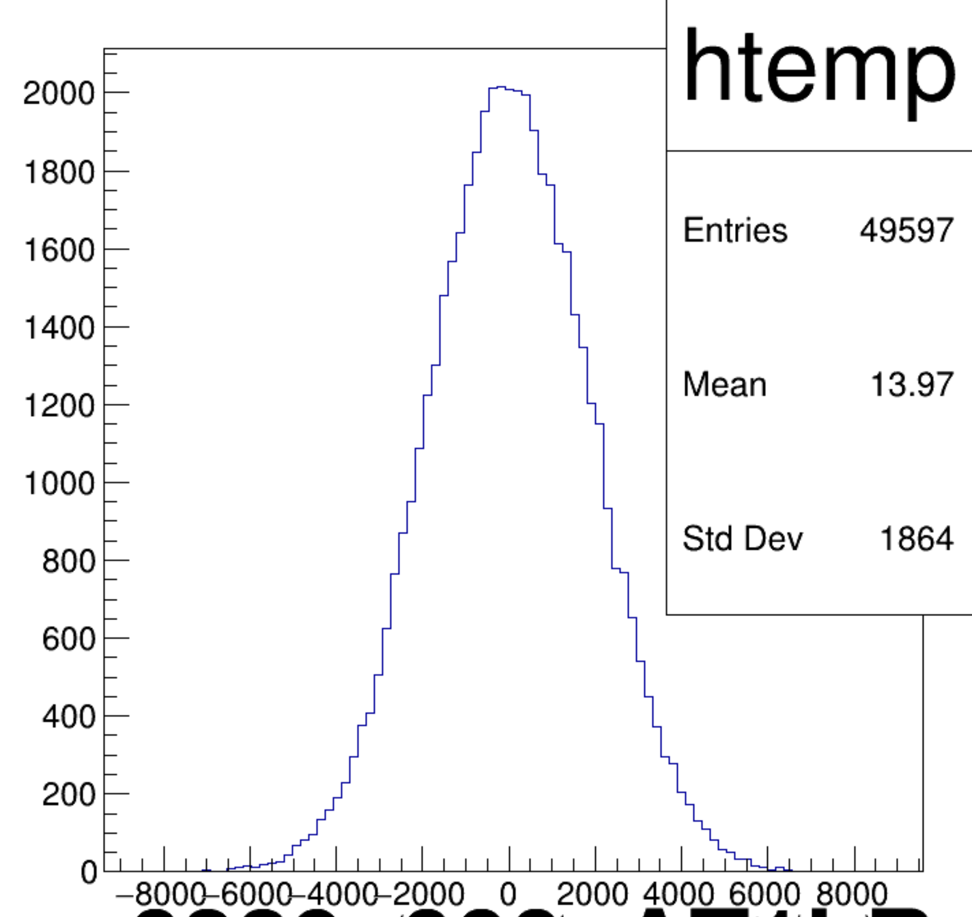
(asym_atl1/ppm-asym_atr1/ppm)/2 {ok_cut}
