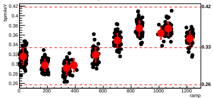
bmod_trim6,cyc=5977
