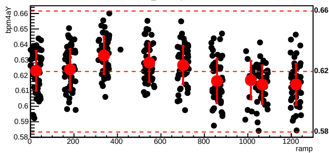
bmod_trim3,cyc=5985
