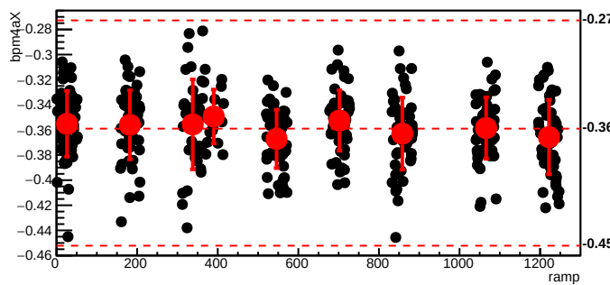
bmod_trim4,cyc=5985
