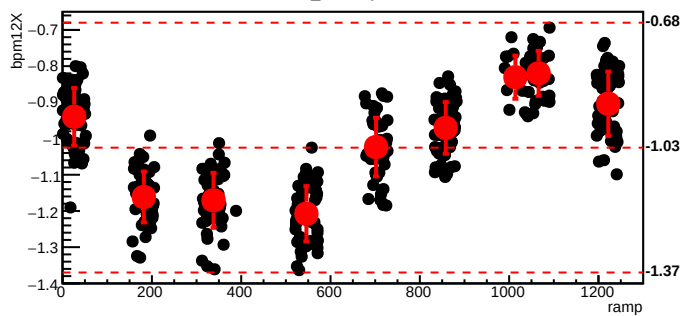
bmod_trim3,cyc=5985
