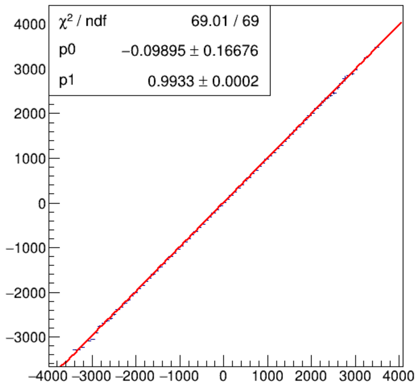
run6331_000_asym_bcm_dg_ds_vs_asym_bcm_an_us_pr.png
