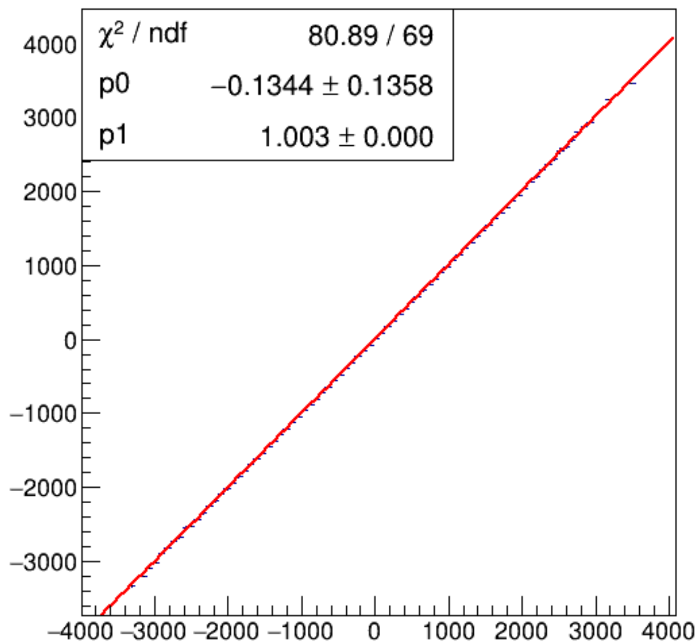
run6331_000_asym_bcm_an_us_vs_asym_bcm_an_ds_pr.png
