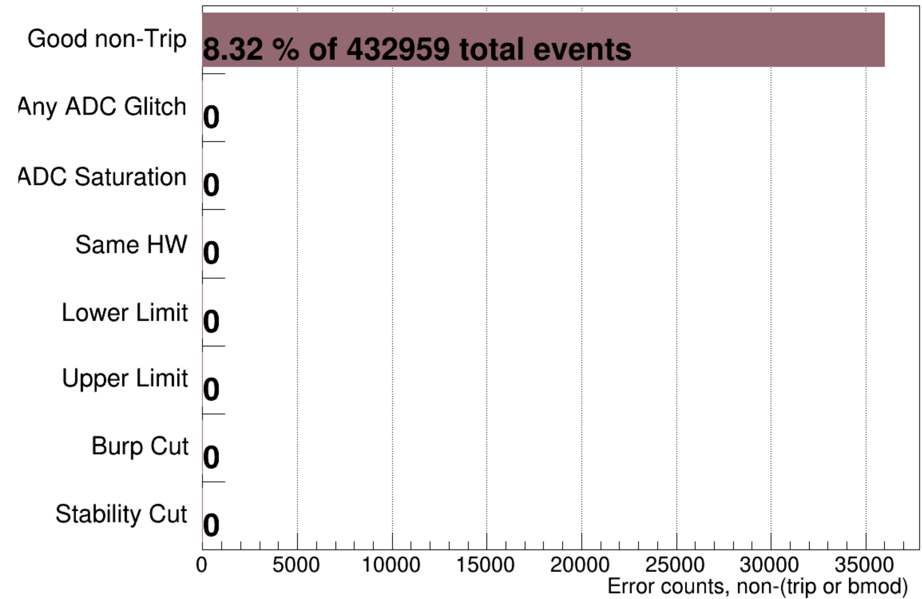
atr2's Device Error Counter &amp;&amp; Not (Trip || BMOD)
