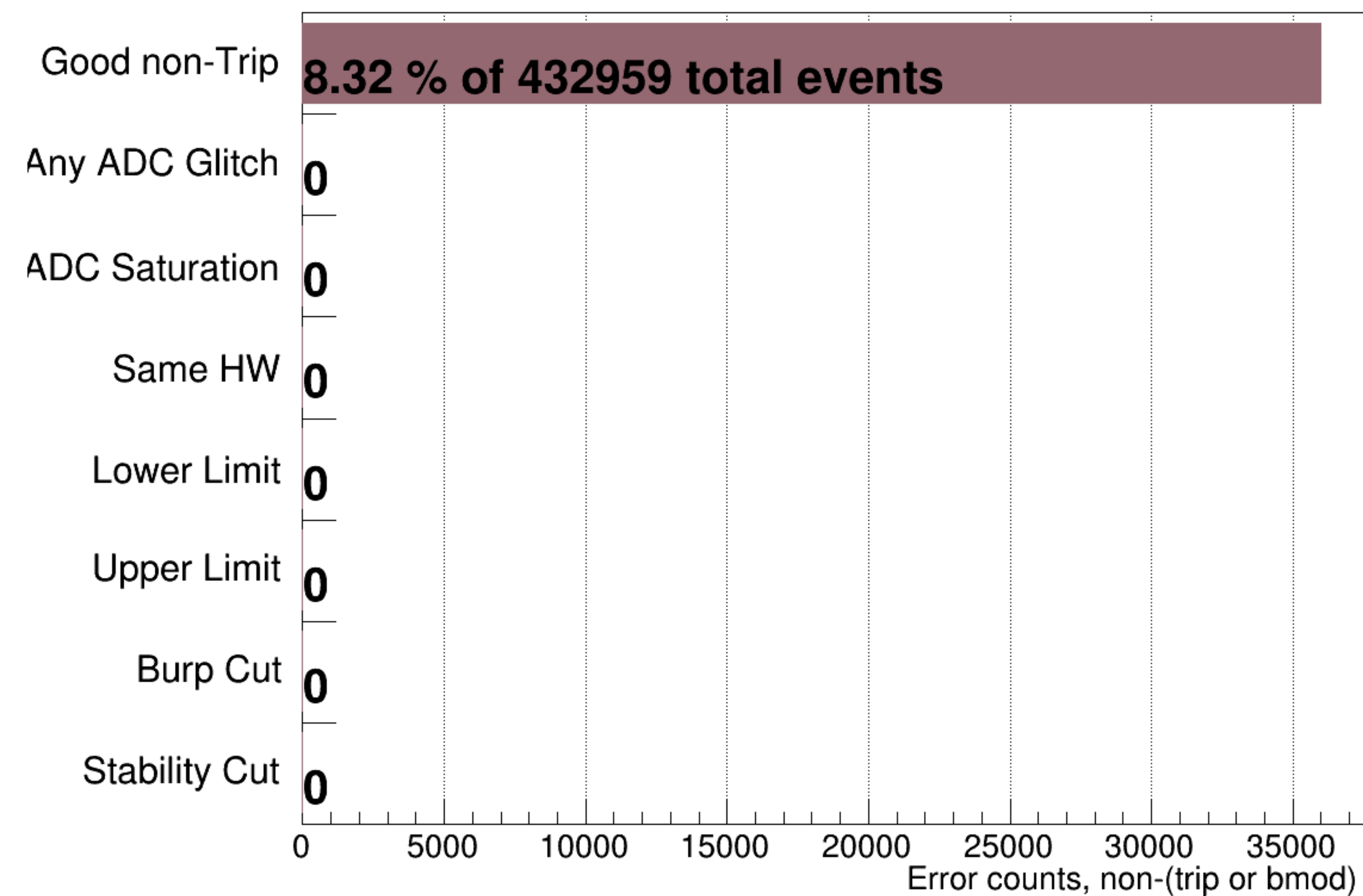
bpm4aX's Device Error Counter &amp;&amp; Not (Trip || BMOD)
