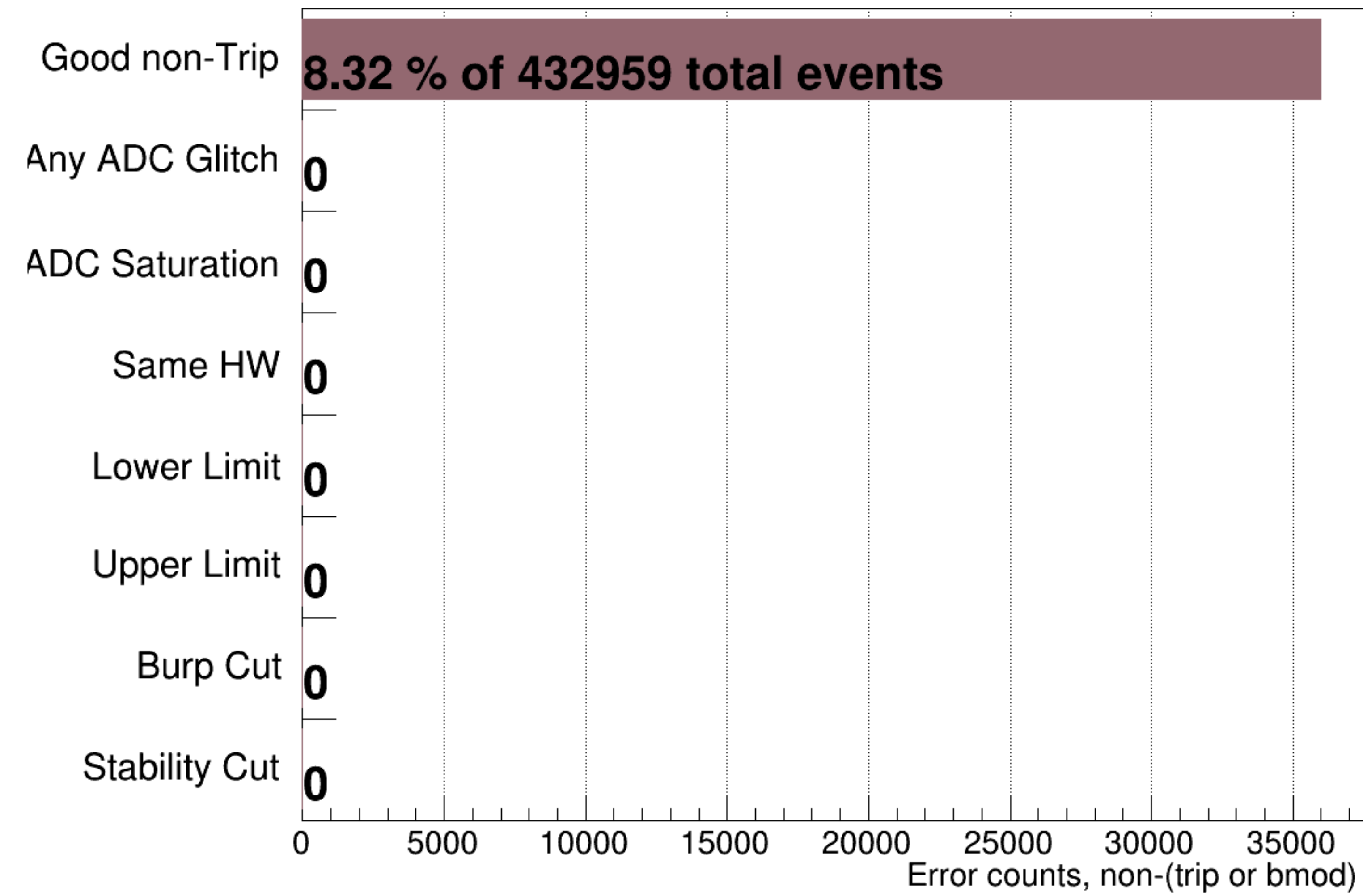
atl1's Device Error Counter &amp;&amp; Not (Trip || BMOD)
