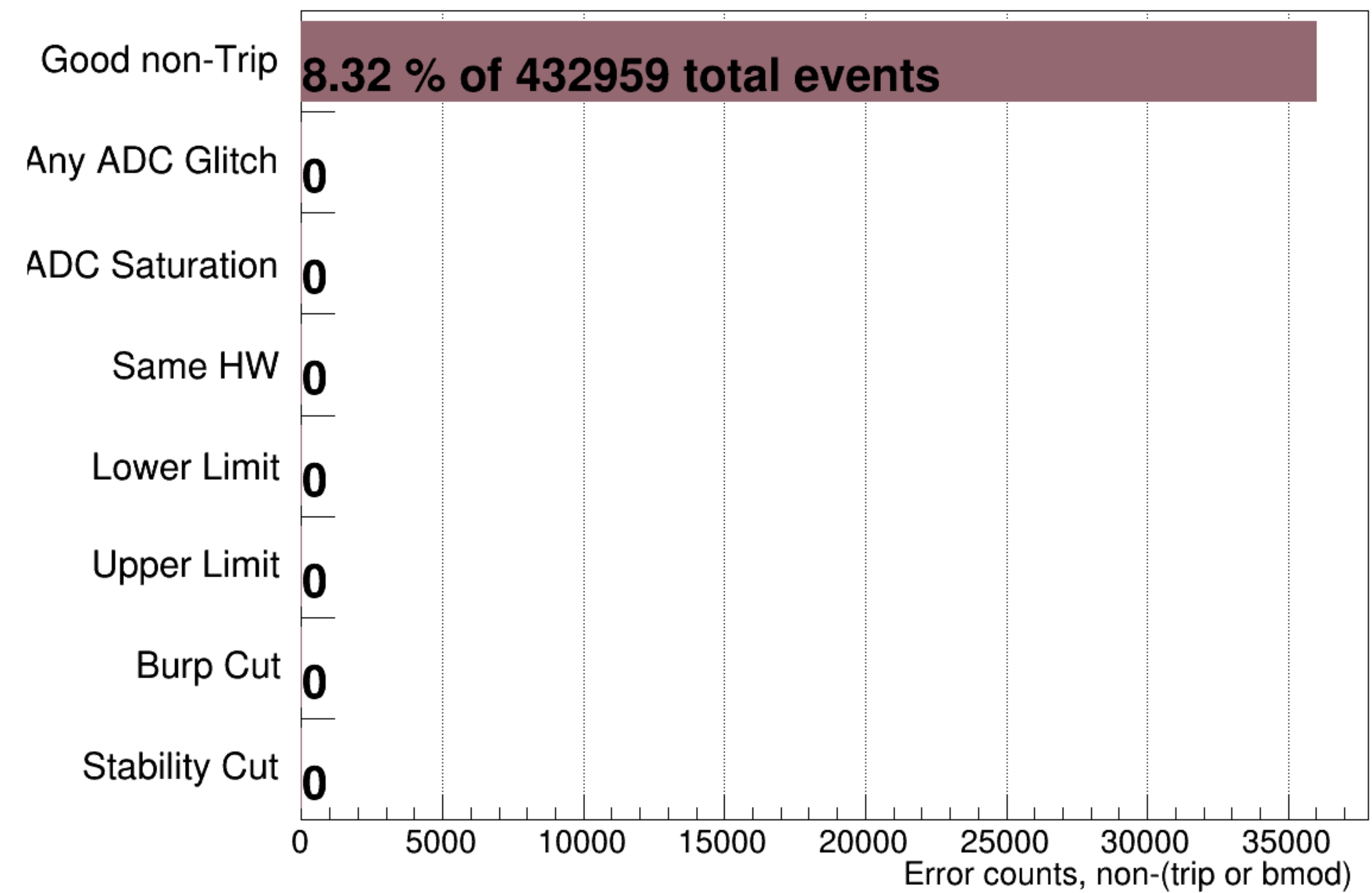
usr's Device Error Counter && Not (Trip || BMOD)
