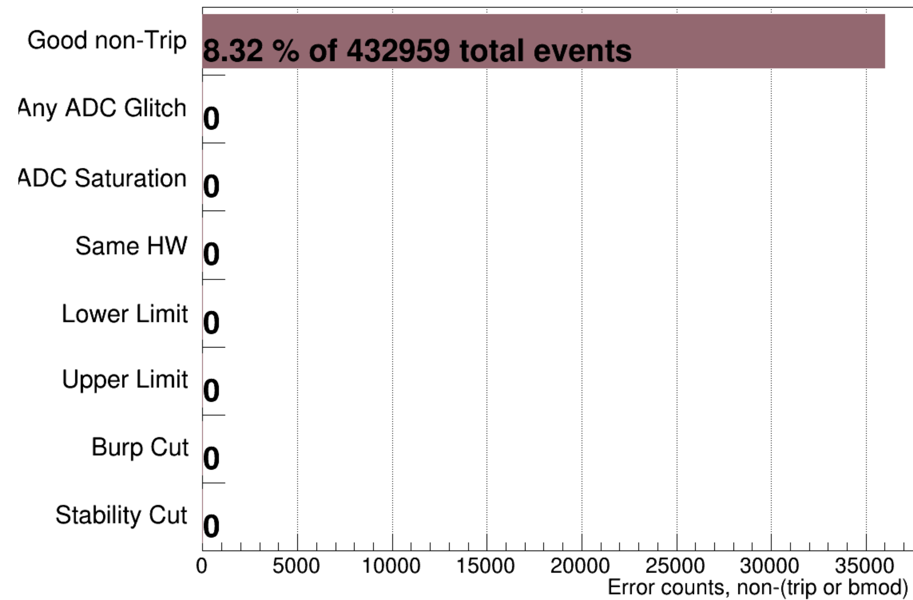
bpm1XM's Device Error Counter &amp; Not (Trip || BMOD)
