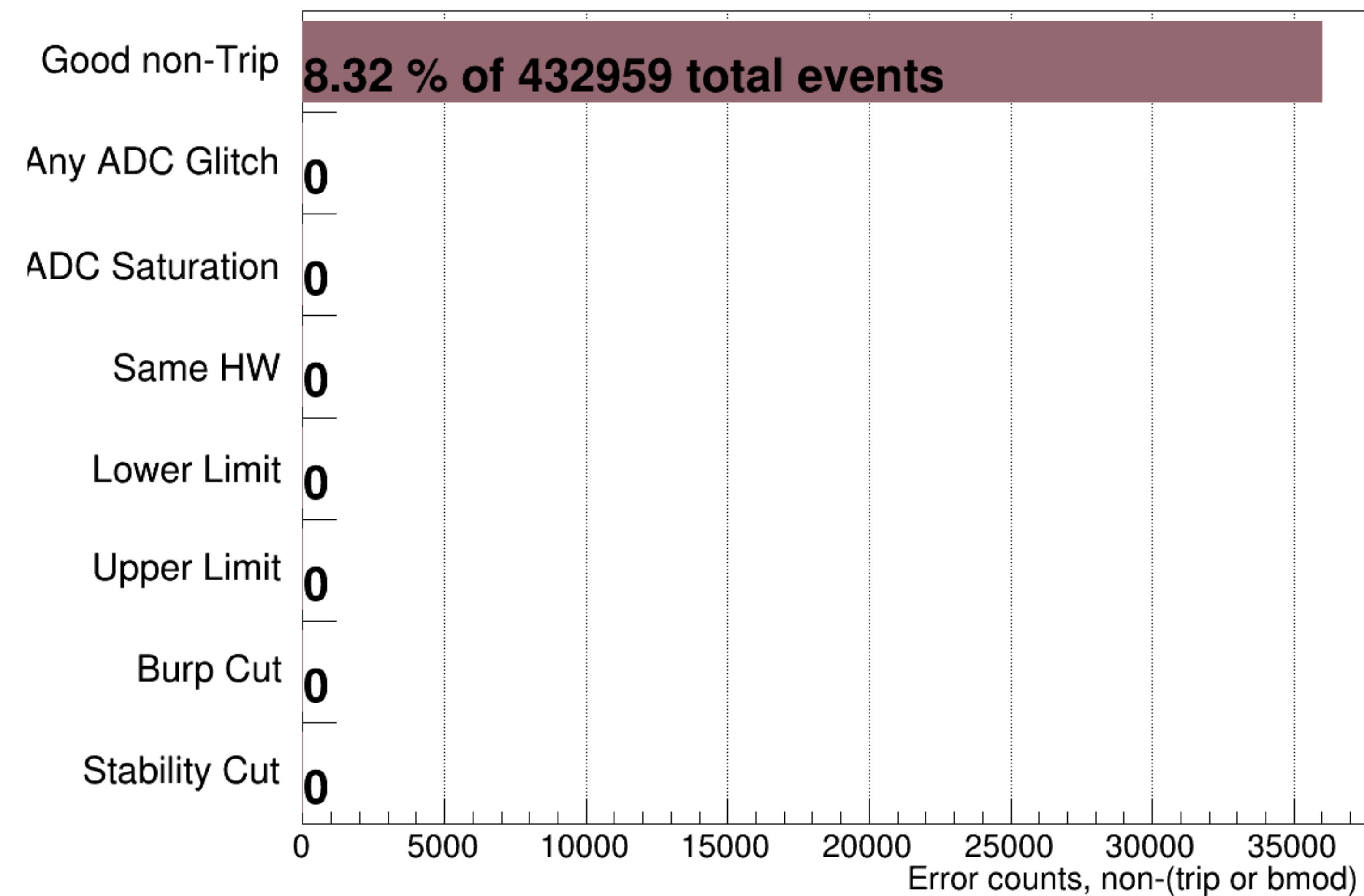
bpm1YP's Device Error Counter &amp; Not (Trip || BMOD)
