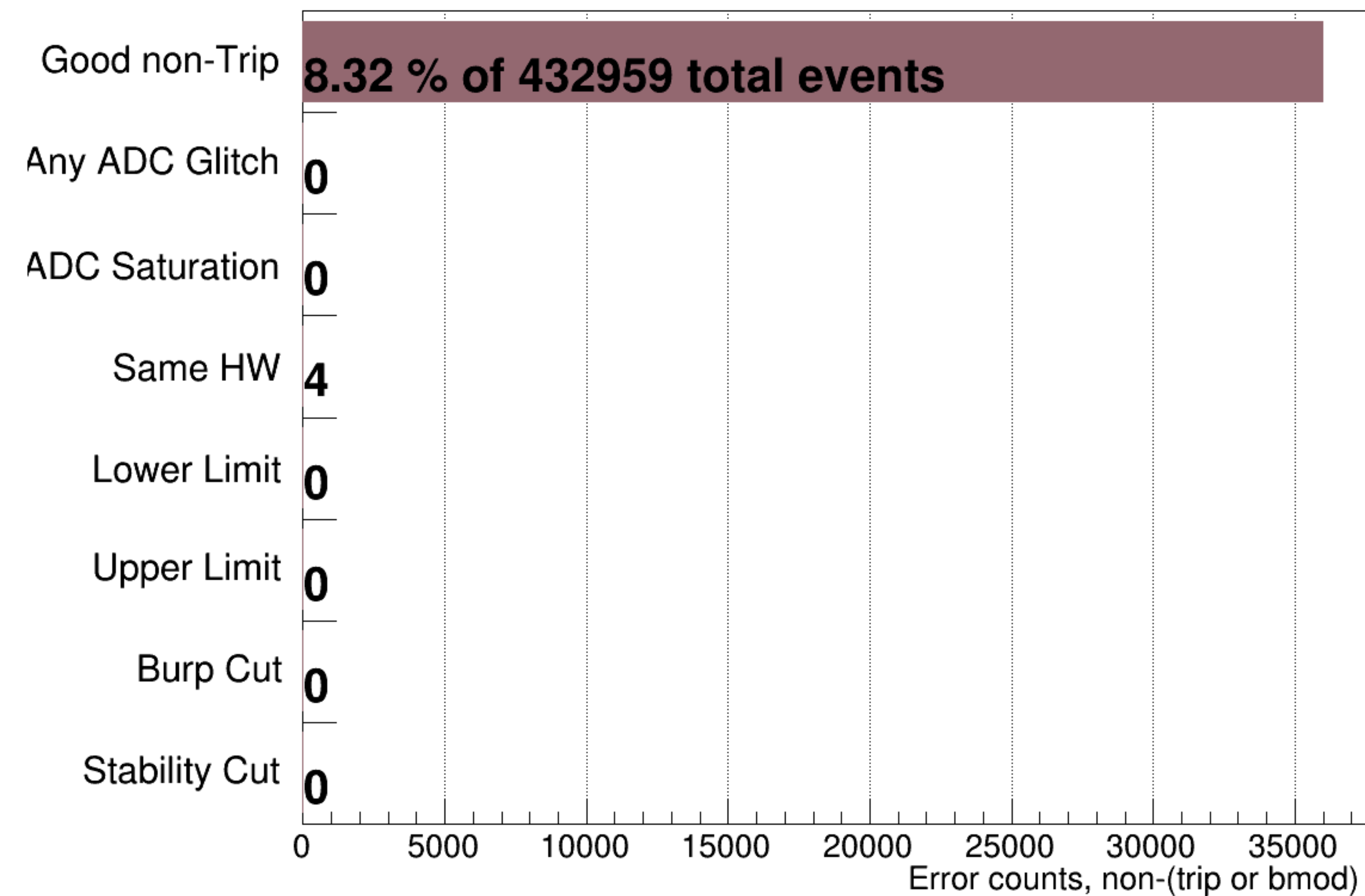
dsl's Device Error Counter && Not (Trip || BMOD)
