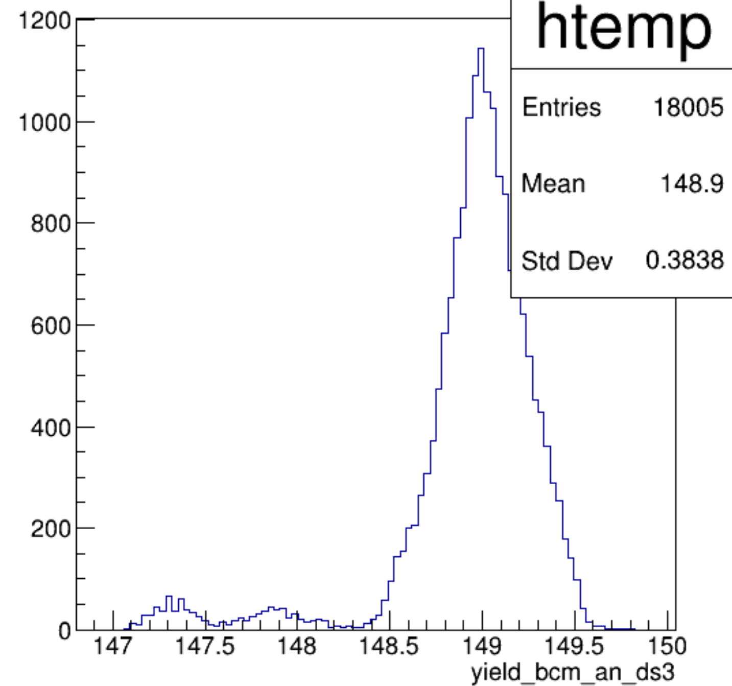
yield_bcm_an_ds3 {ErrorFlag==0}
