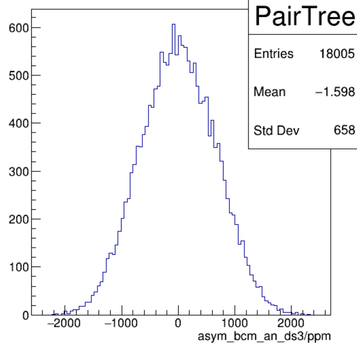
asym_bcm_an_ds3/ppm {ErrorFlag==0}
