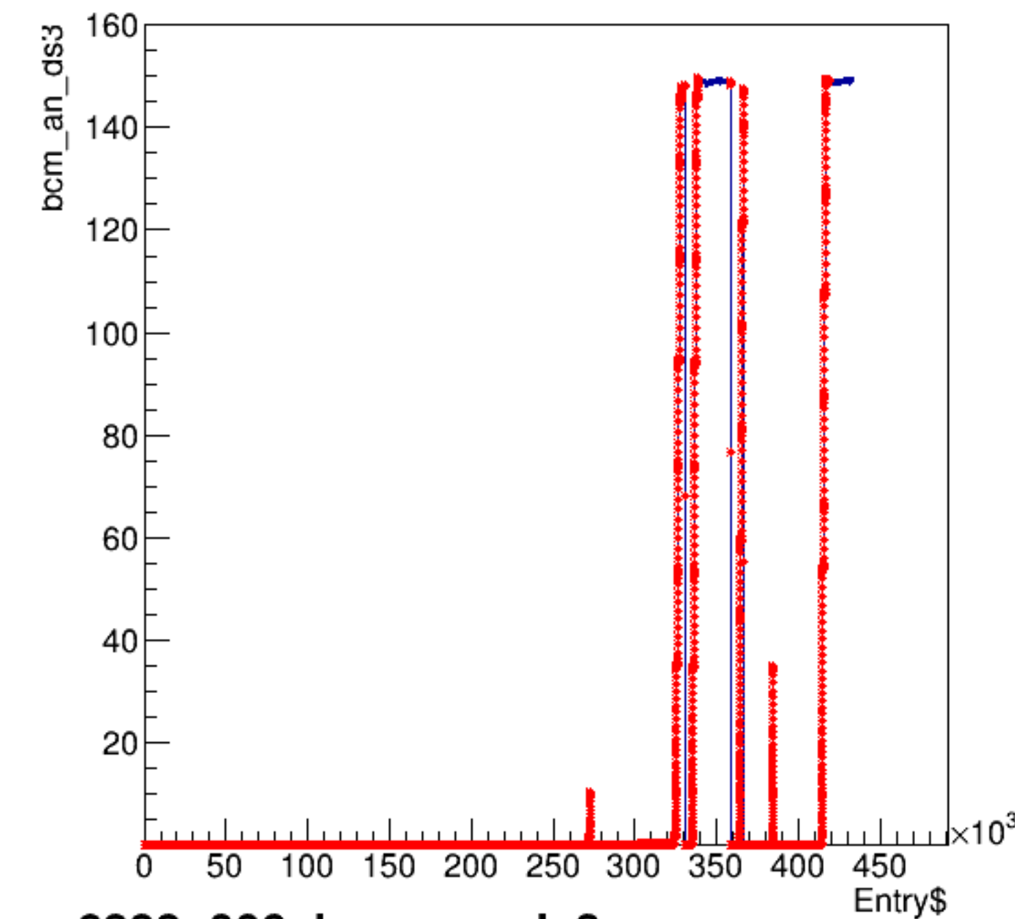
bcm_an_ds3:Entry$
