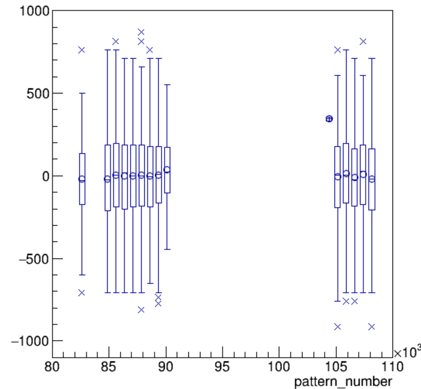
asym_bcm_an_ds3/ppm:pattern_number {ErrorFlag==0}
